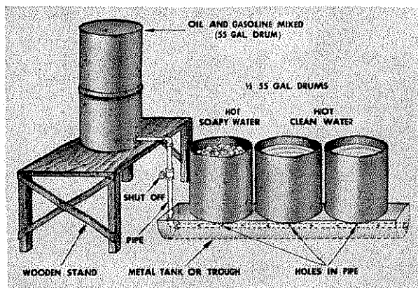
Method of heating mess kit water.
