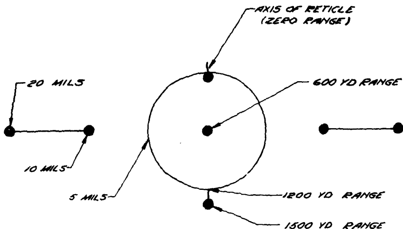
FIGURE 11.—Reticle telescopic sight M19.
