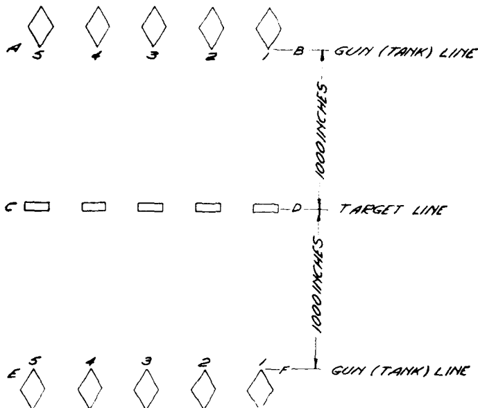
FIGURE 21.—Tank and target arrangement for initial preparatory marksmanship training for two tank platoons.
