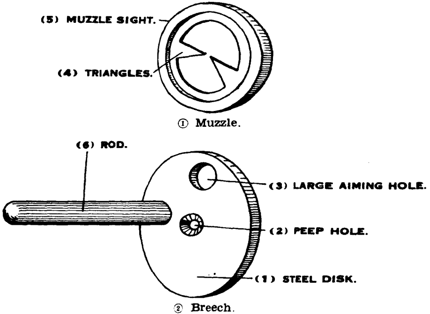
FIGURE 12.—Bore sights.
