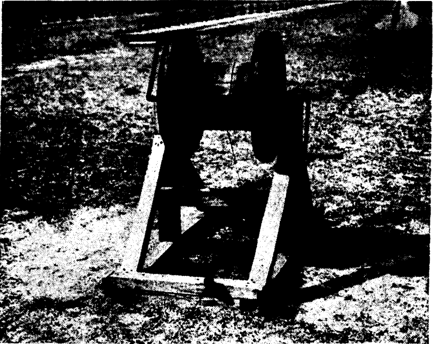
FIGURE 28.—Hand-operated drum (reel), 1,000-inch moving target range.
