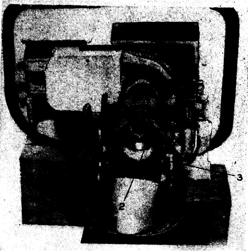
FIGURE 3.—37-mm tank gun M6 in M24 mount, rear view.
