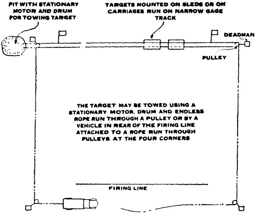
FIGURE 30.—Range for caliber .30 or 37-mm moving field target.
