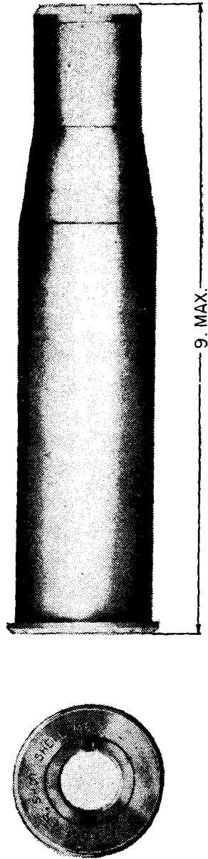
FIGURE 17.—Shot, fixed, TP, M51, with tracer.
