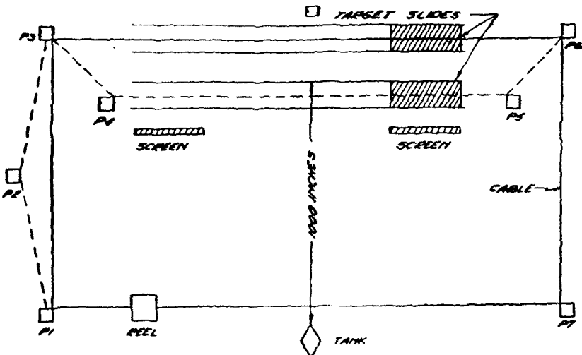
FIGURE 27.—Arrangement of 1,000-inch moving target range unit, showing positions of pulleys and hand-operated drum (reel).
