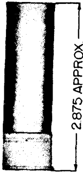
FIGURE 19.—Shell, shotgun, 10-gage, blank (8 grains black powder with dry felt wads).
