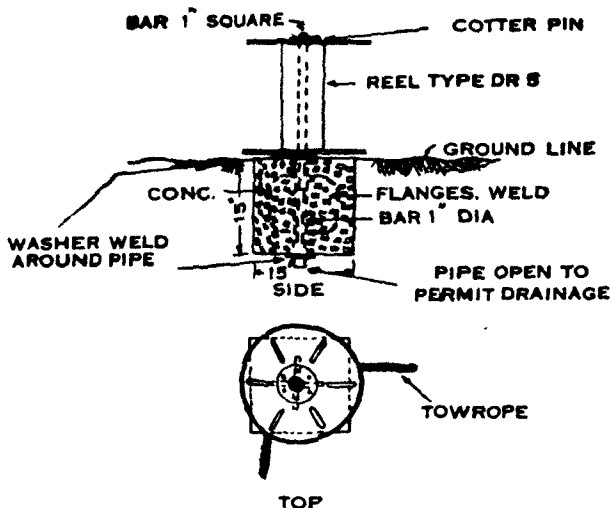
FIGURE 42.—Roadway drum for towed-target range shown in figure 40.
