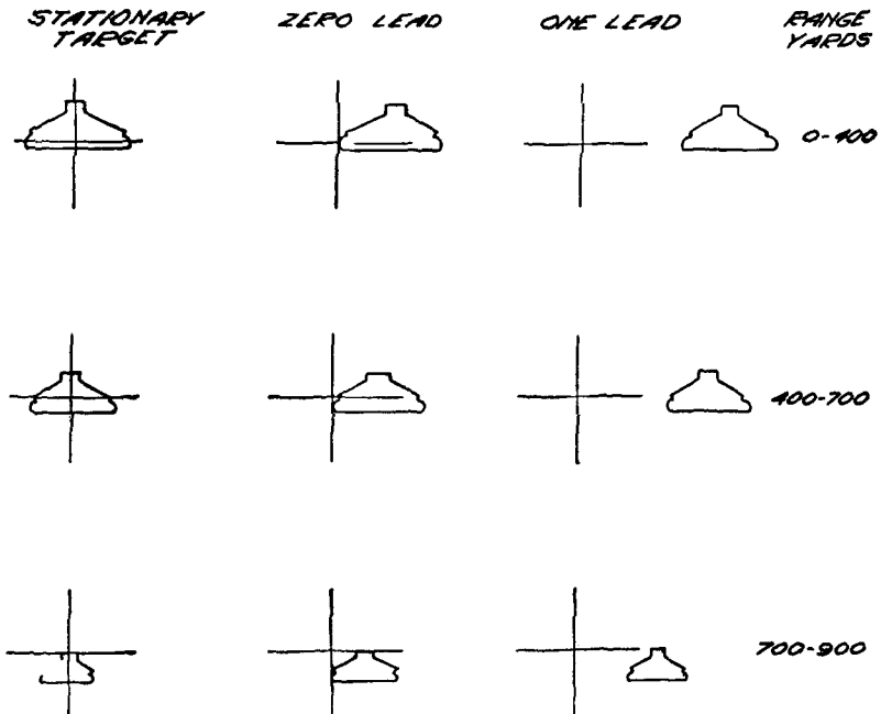
FIGURE 23.—Sight pictures when aiming at stationary and moving targets with the cross hair reticle. (Note change in size of silhouettes as range increases.)
