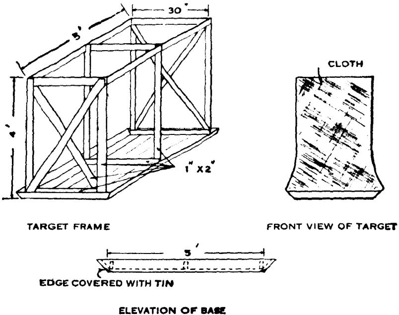
FIGURE 31.—Target frame and sled for towed-target range.
