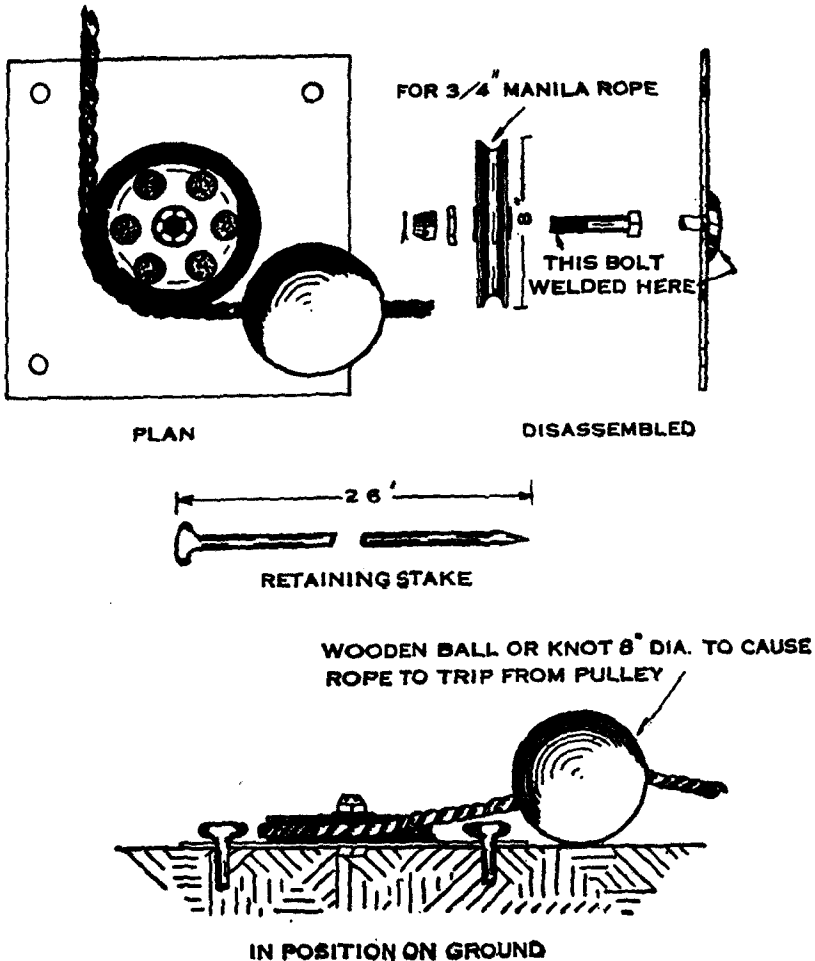
FIGURE 41.—Pulley lay-out for towed-target range shown in figure 40.
