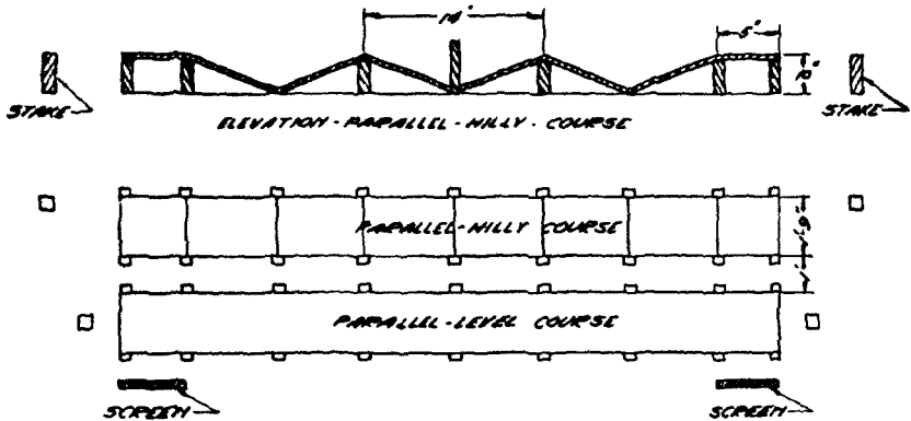
FIGURE 26.—Dimensions and plan of construction; 1,000-inch moving target range.
