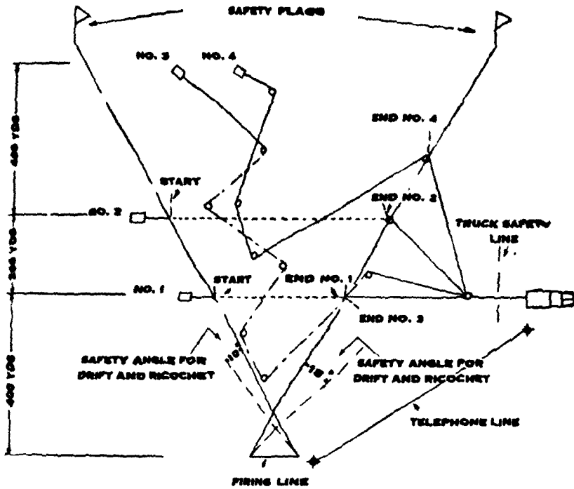
FIGURE 40.—Range for firing 37-mm ammunition at stationary or towed targets.
