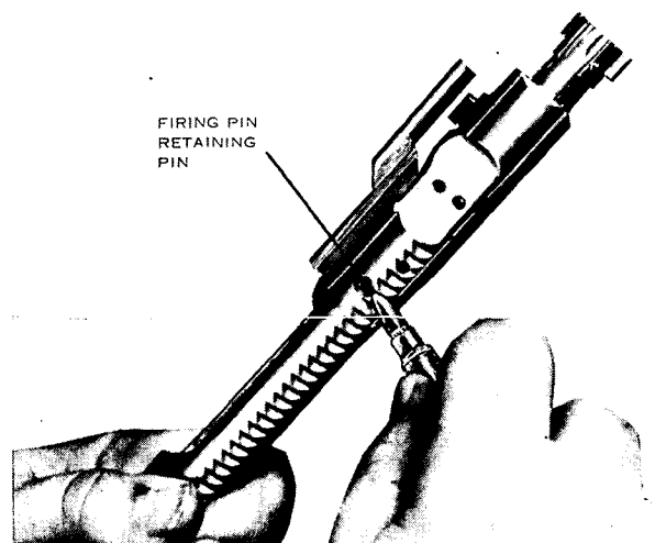
Figure 13. Pressing out firing pin retaining pin.
