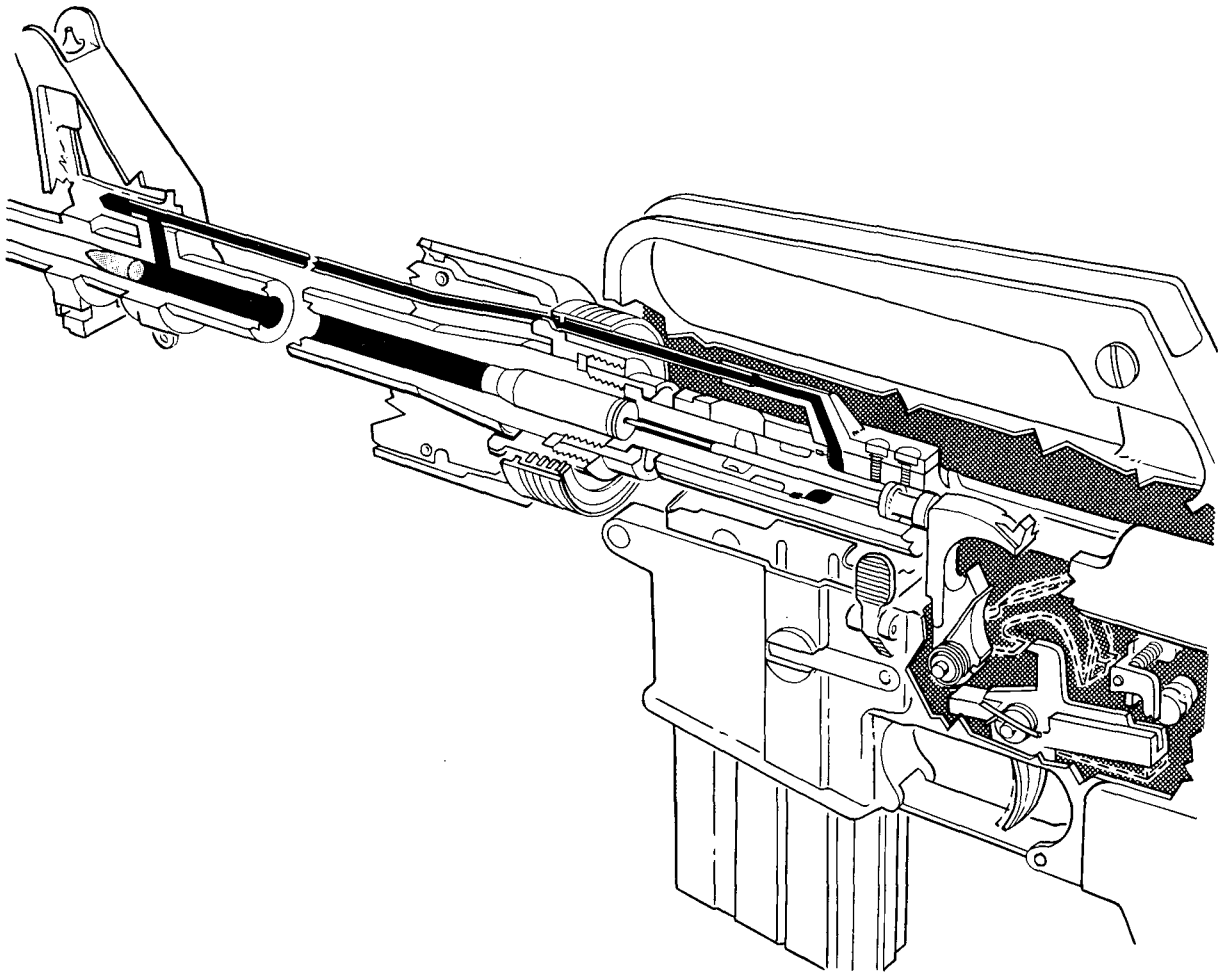
Figure 23. Firing.
