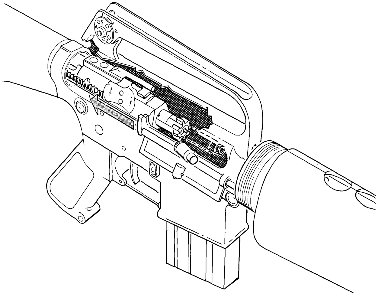
Figure 27. Ejecting.
