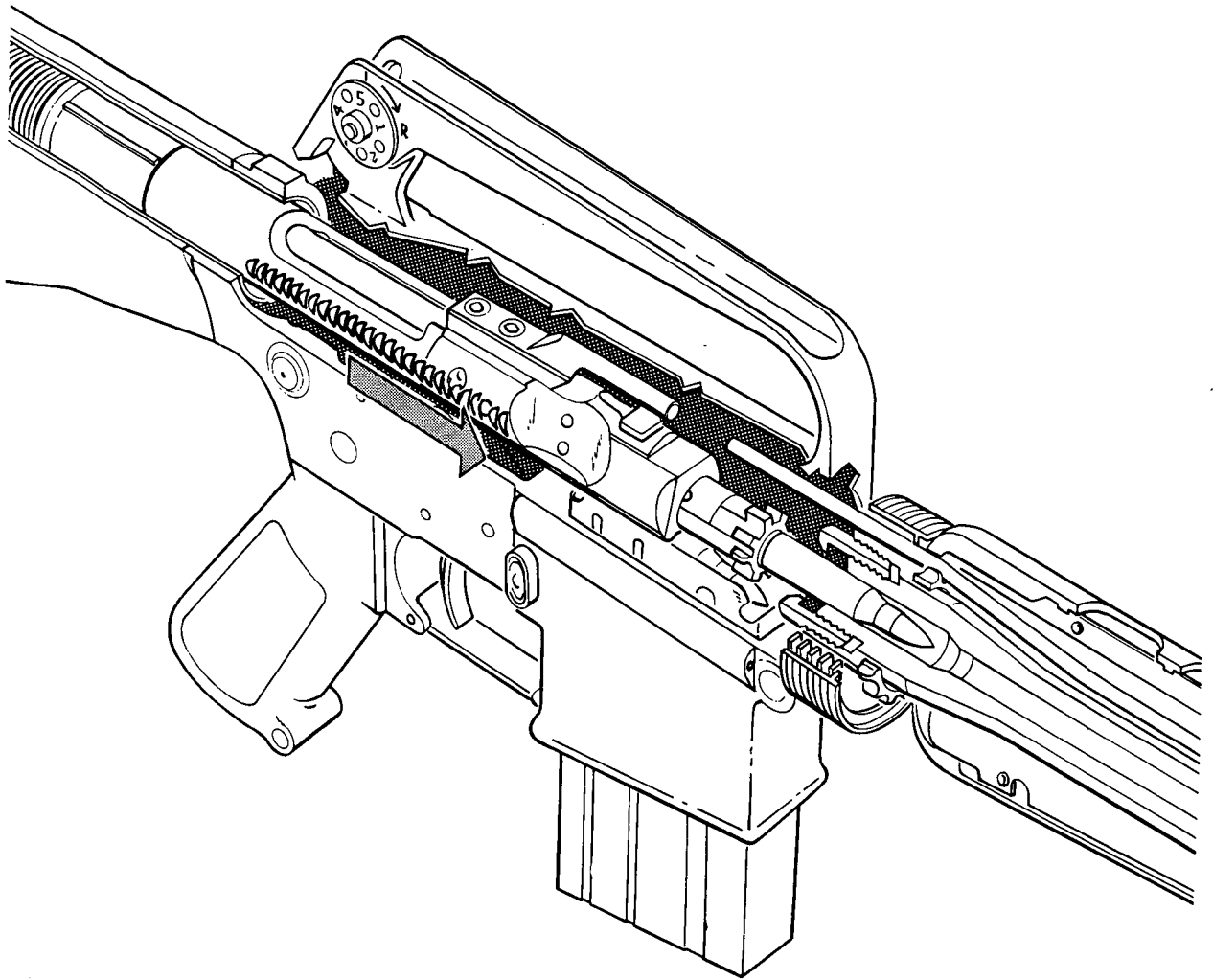
Figure 30. Chambering.
