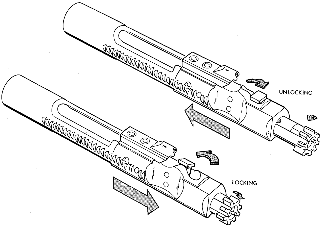
Figure 25. Locking and unlocking.
