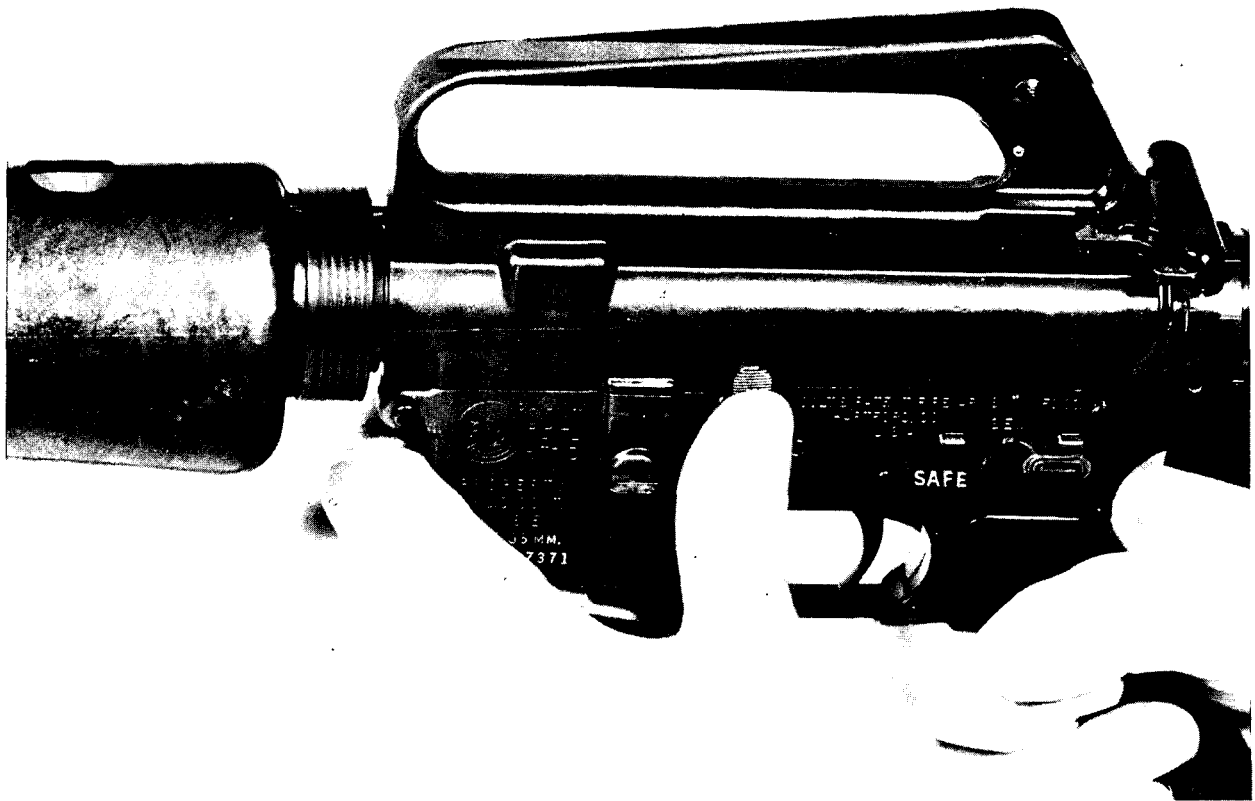
Figure 22. Depressing the upper portion of the bolt catch.
