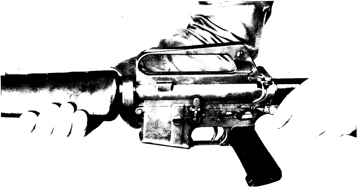
Figure 7. Pressing the takedown pin to the right.
