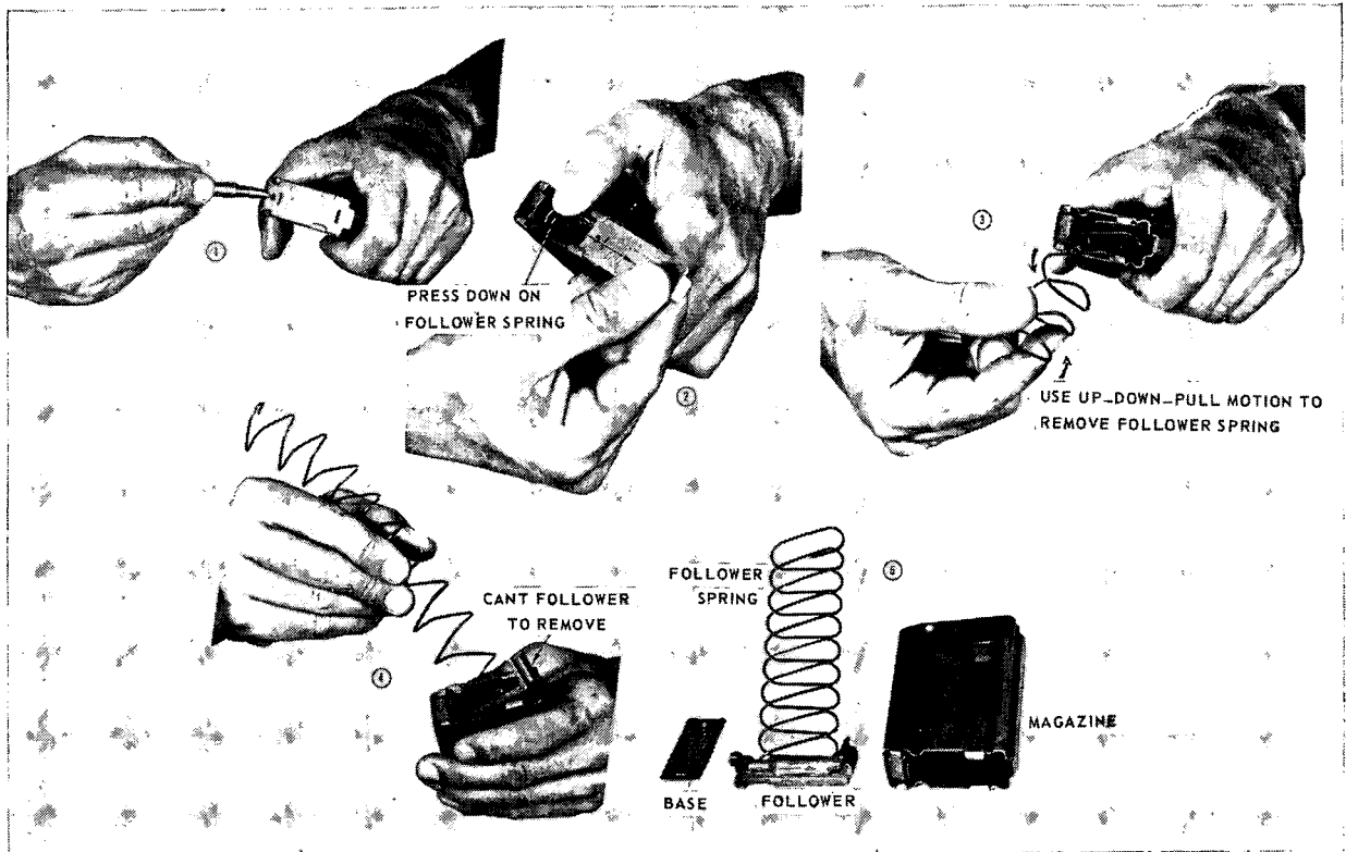
Figure 21.2. Disassembly of the magazine.
