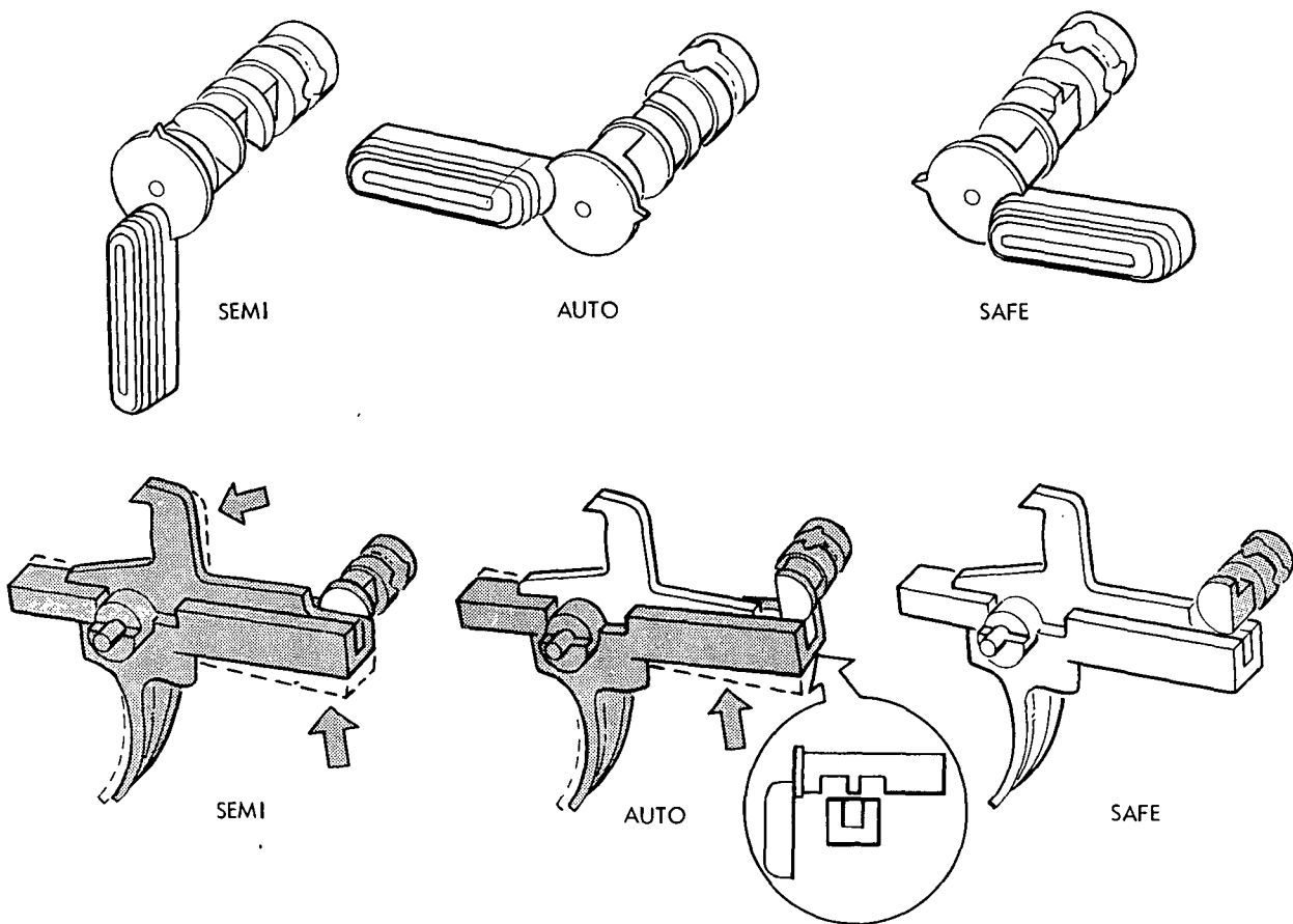
Figure 31. Selector lever.
