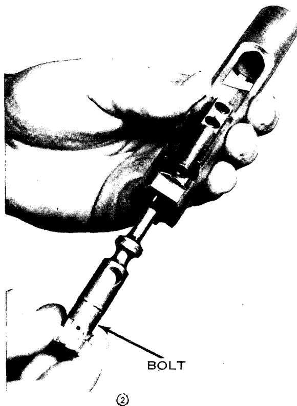
Figure 16. Removing the bolt.
