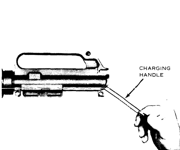
Figure 12. Removing the charging handle.
