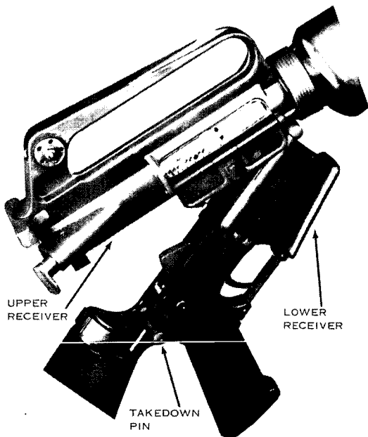
Figure 8. Breaking the upper receiver away from the lower receiver.
