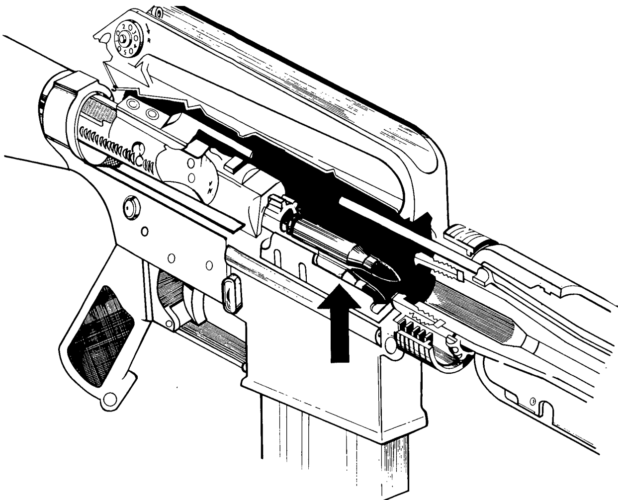
Figure 29. Feeding.
