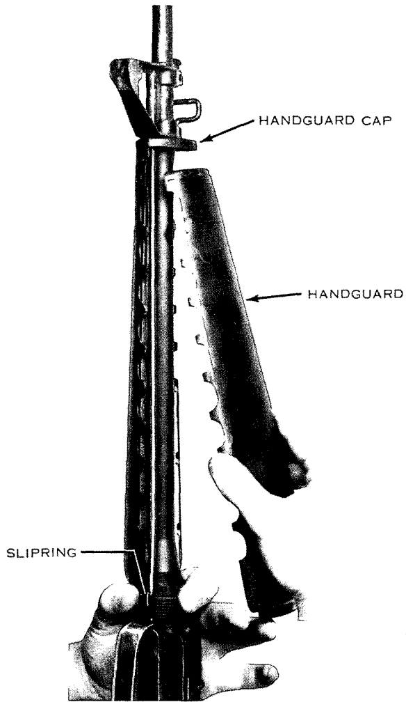
Figure 18. Removing the handguards.
