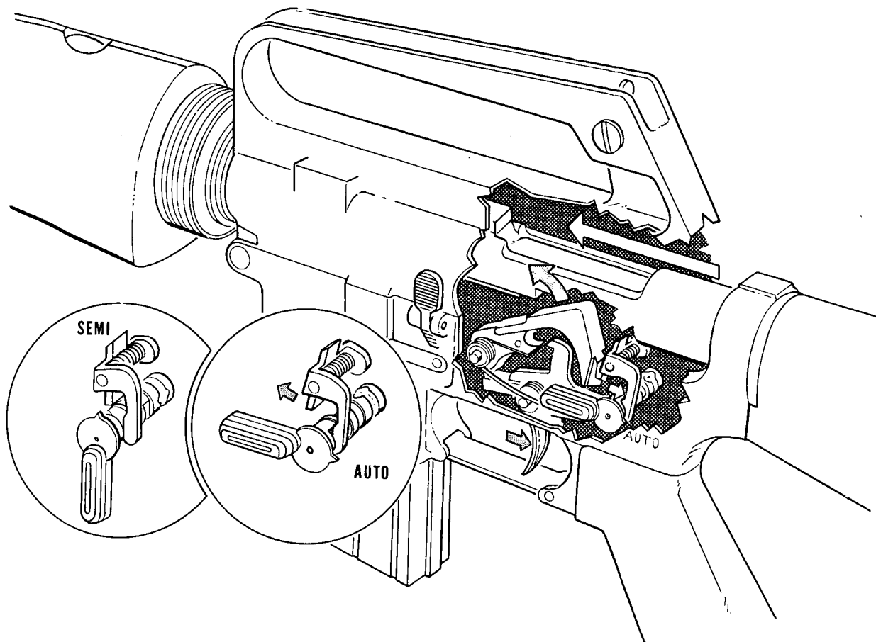
Figure 32. Automatic sear.
