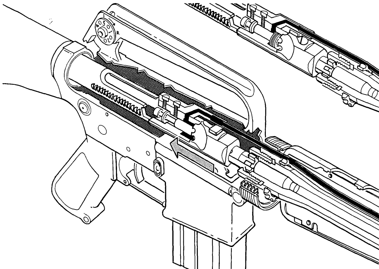
Figure 26. Extracting.
