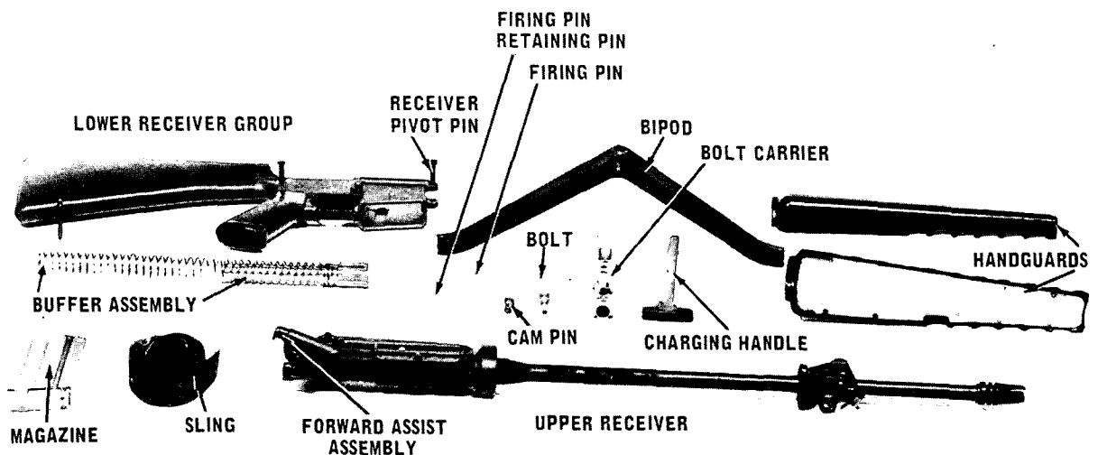
Figure 19. The XM16E1 field stripped.
