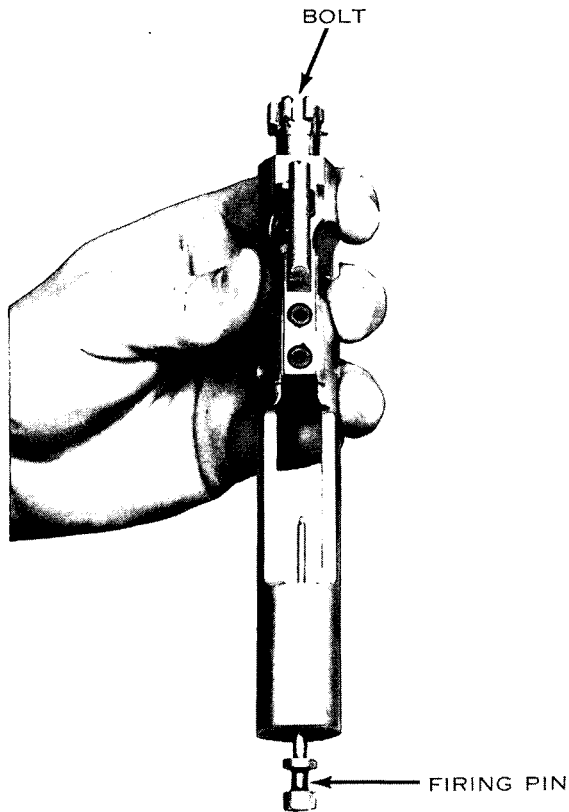
Figure 14. Removing the firing pin.
