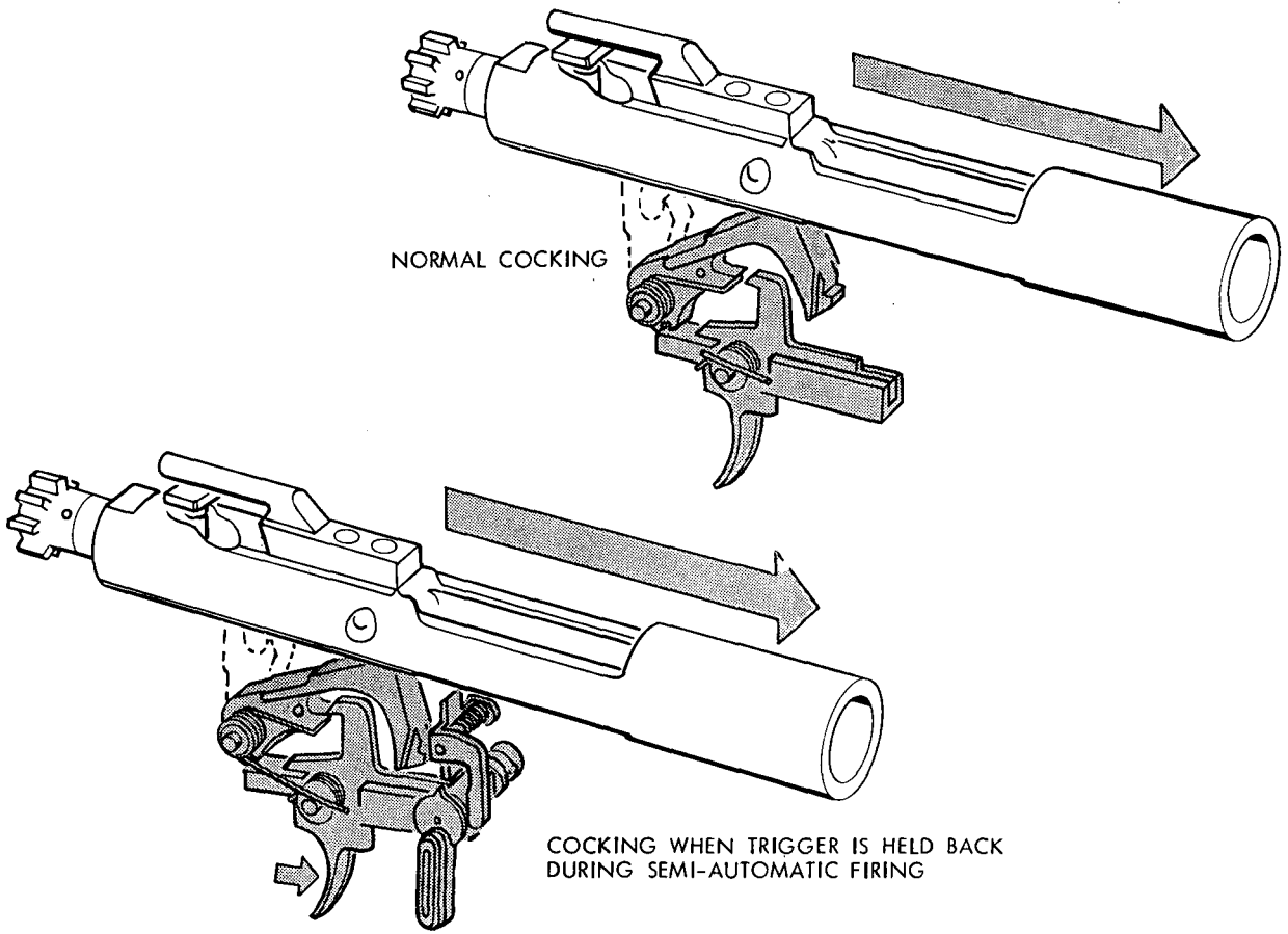
Figure 28. Cocking.
