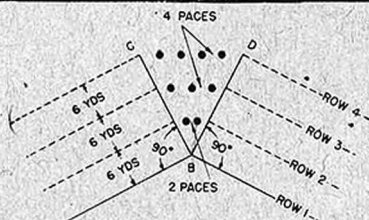
Figure 31.05a. Change of direction, hasty mine belt.
