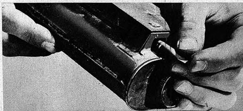
2. Insert fuzes into two pockets under pressure plate, pushing detonator end in first and insuring that red paint is visible in gap.
