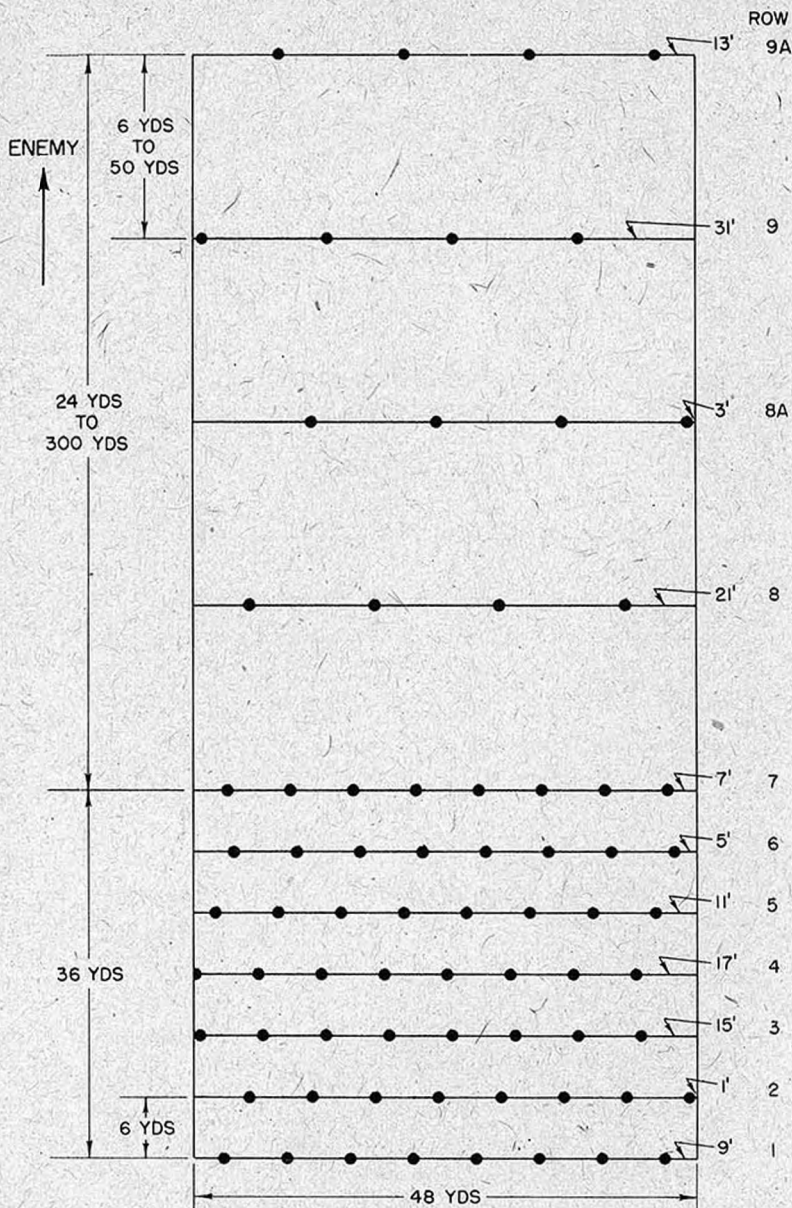
Figure 32.02d. Extended section, deliberate mine belt.
