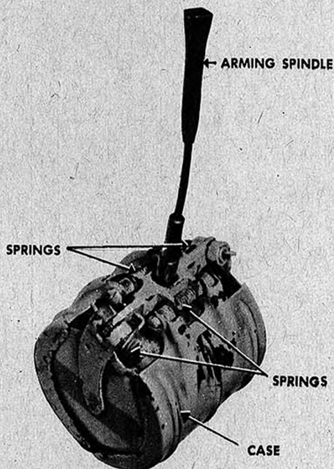
UNARMED BOMB
