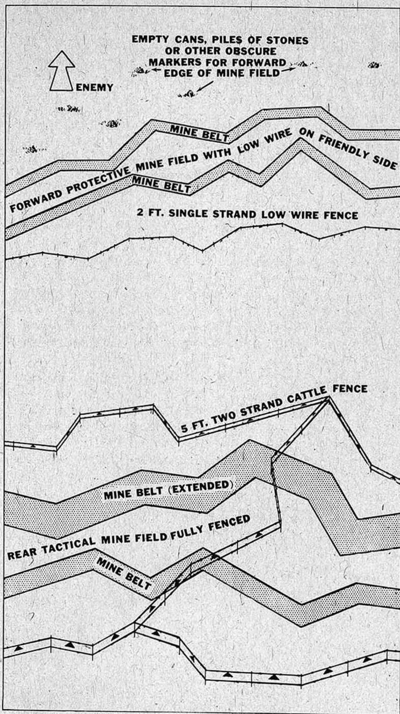
Figure 21.08b. Mine-field marking fences.
