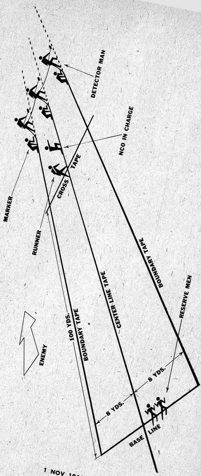
Figure 43.07a. Taping party for breaching mine-field lane.
