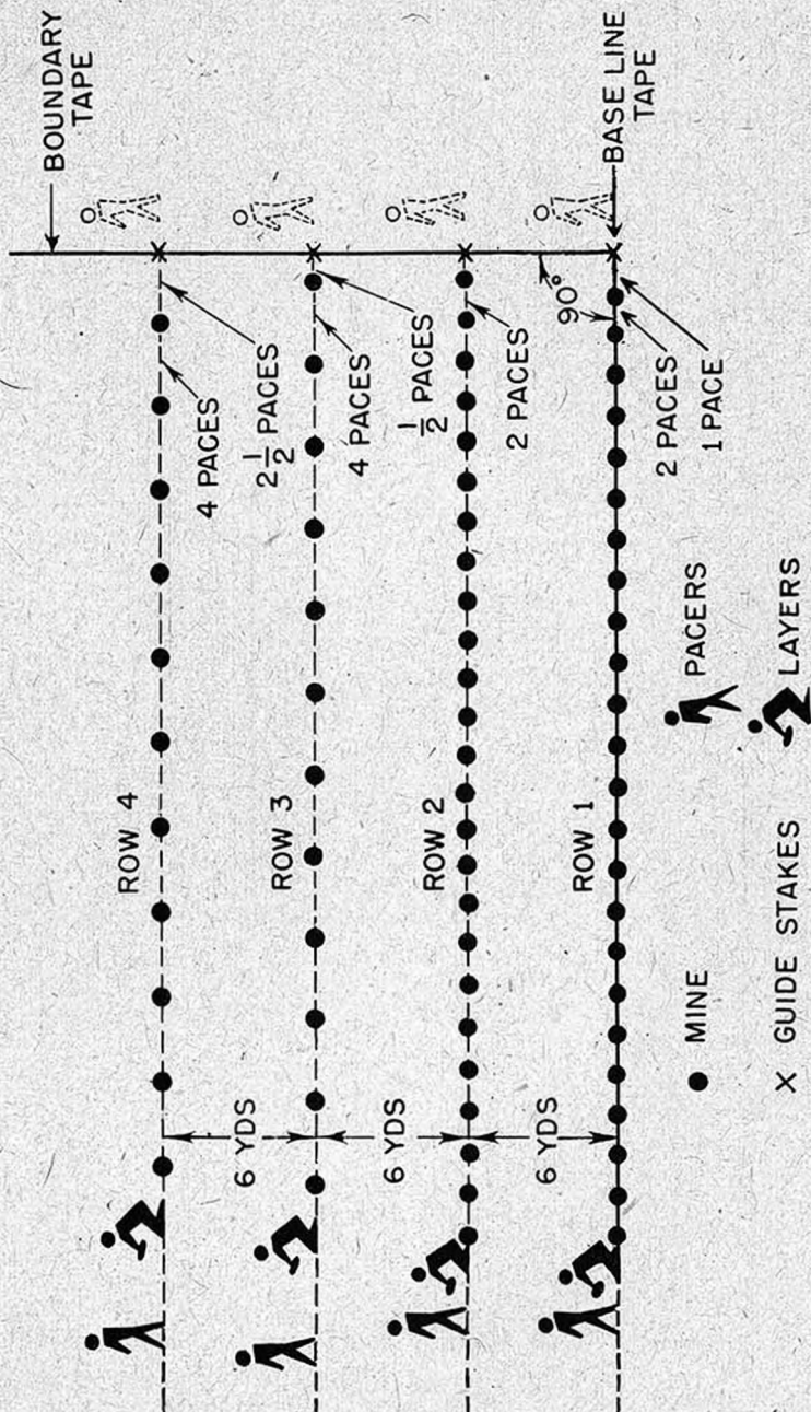
Figure 31.06. Alternate procedure for laying hasty mine belt.
