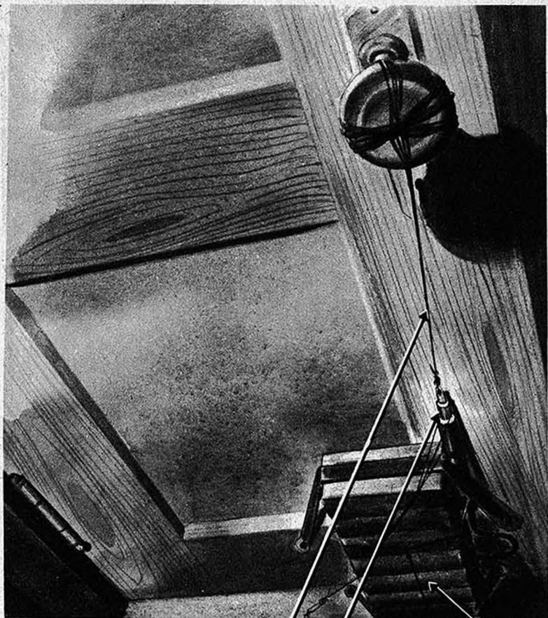
TRIP WIRE (PULLED WHEN KNOB IS TURNED) PULL FUZE Z. Z. 35 CHARGE
