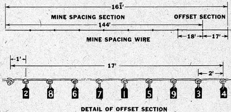
Figure 32.03. Mine-spacing wire.
