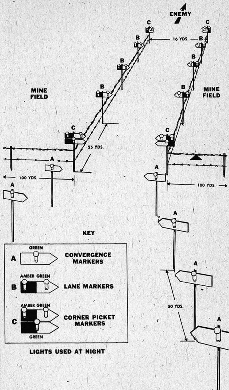
Figure 43.09a. Mine-field lane marking.
