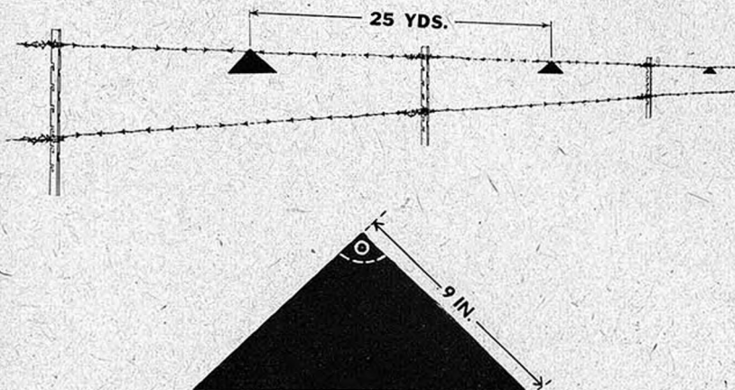
Figure 21.08a. Mine-field fence marker signs.
