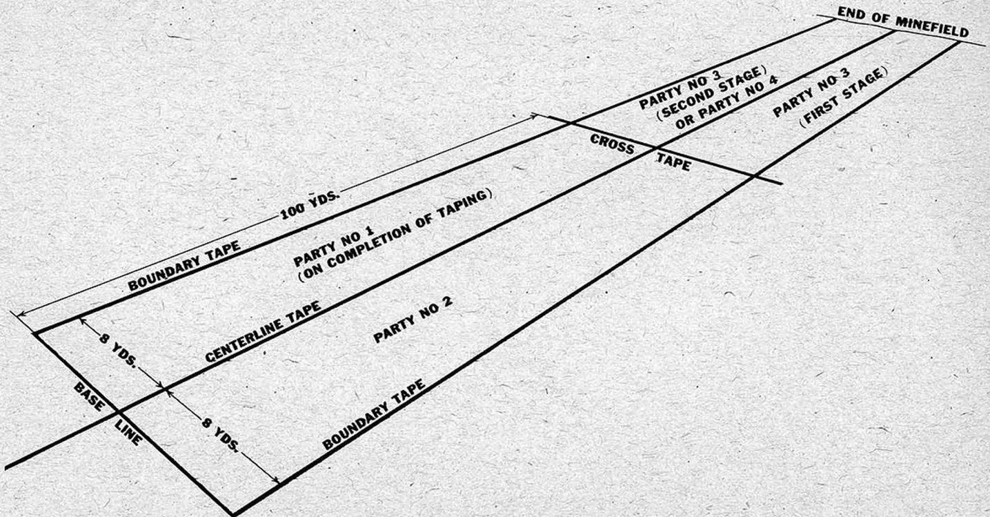
Figure 43.07c. Breaching mine field—lane widening.
