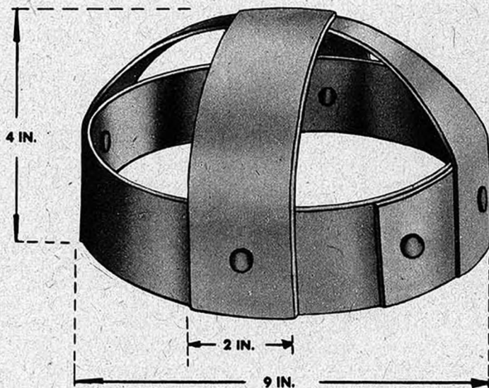
Figure 21.08d. Individual mine marker.
