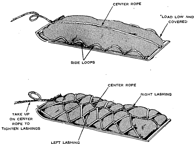
Figure 24. Loop, lashings, and their equipment.
