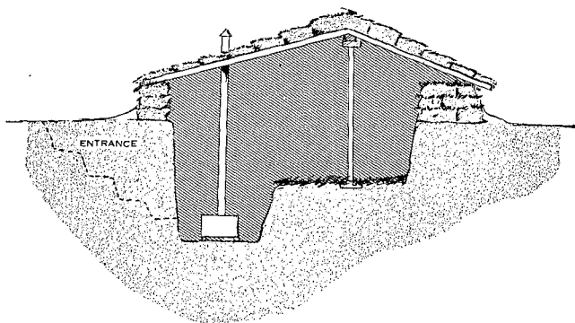
Figure 9. Sod house: cut and cover type.
