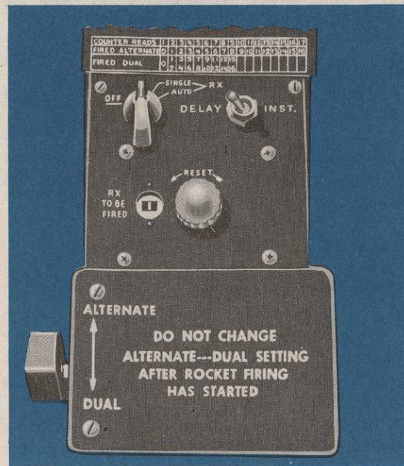
INSTRUMENT PANEL NO. 26
