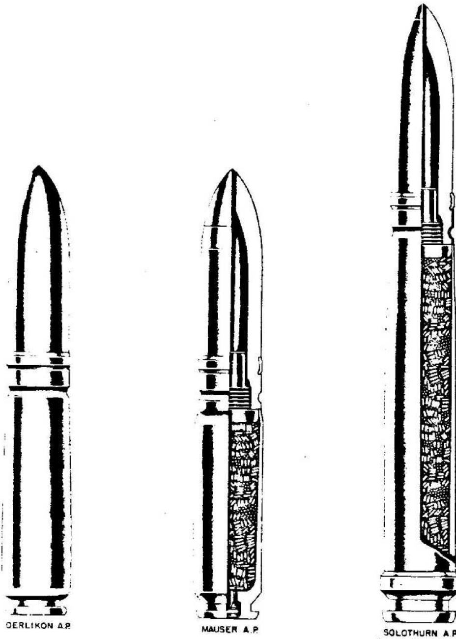
Figure 324A—20-mm Ammunition
