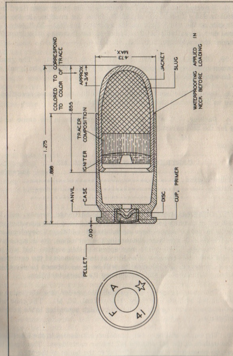
FIGURE 18. - CARTRIDGE, TRACER, CAL..45, M1.
