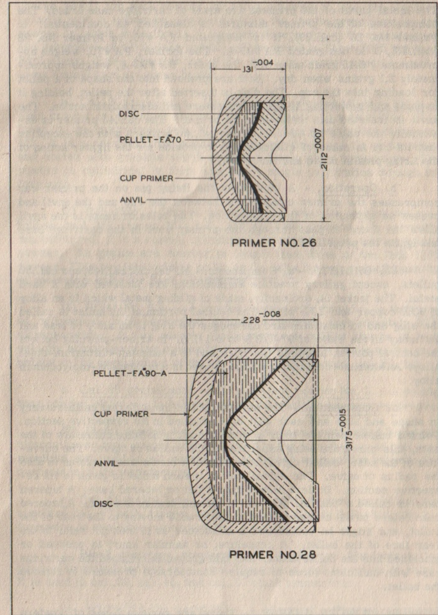
FIGURE 1. - CAL..30 AND CAL..50 PRIMERS.
