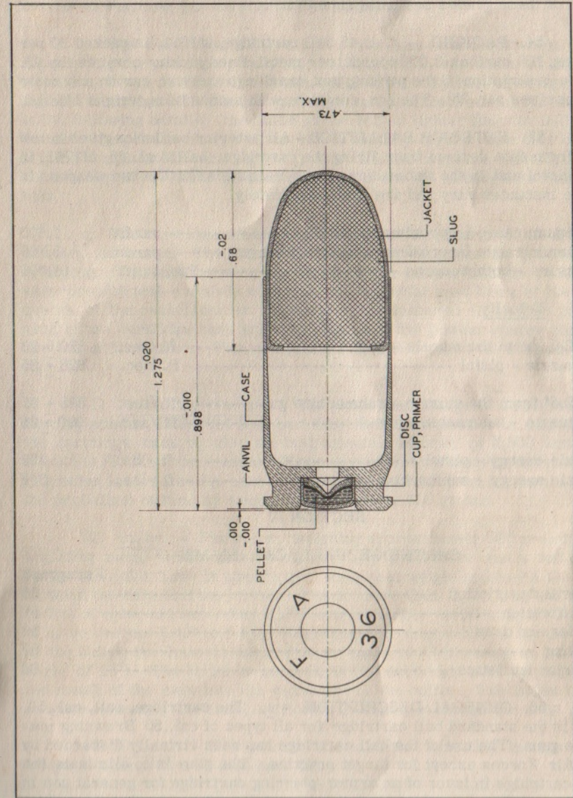
FIGURE 14. - CARTRIDGE, BALL, CAL..45, M1911.
