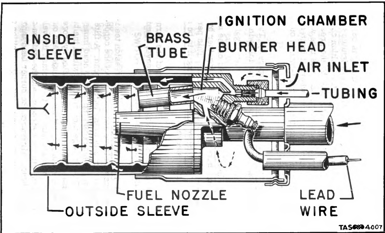
Figure 9. Gas Burner Assembly, Newer Type, Cross Section.
