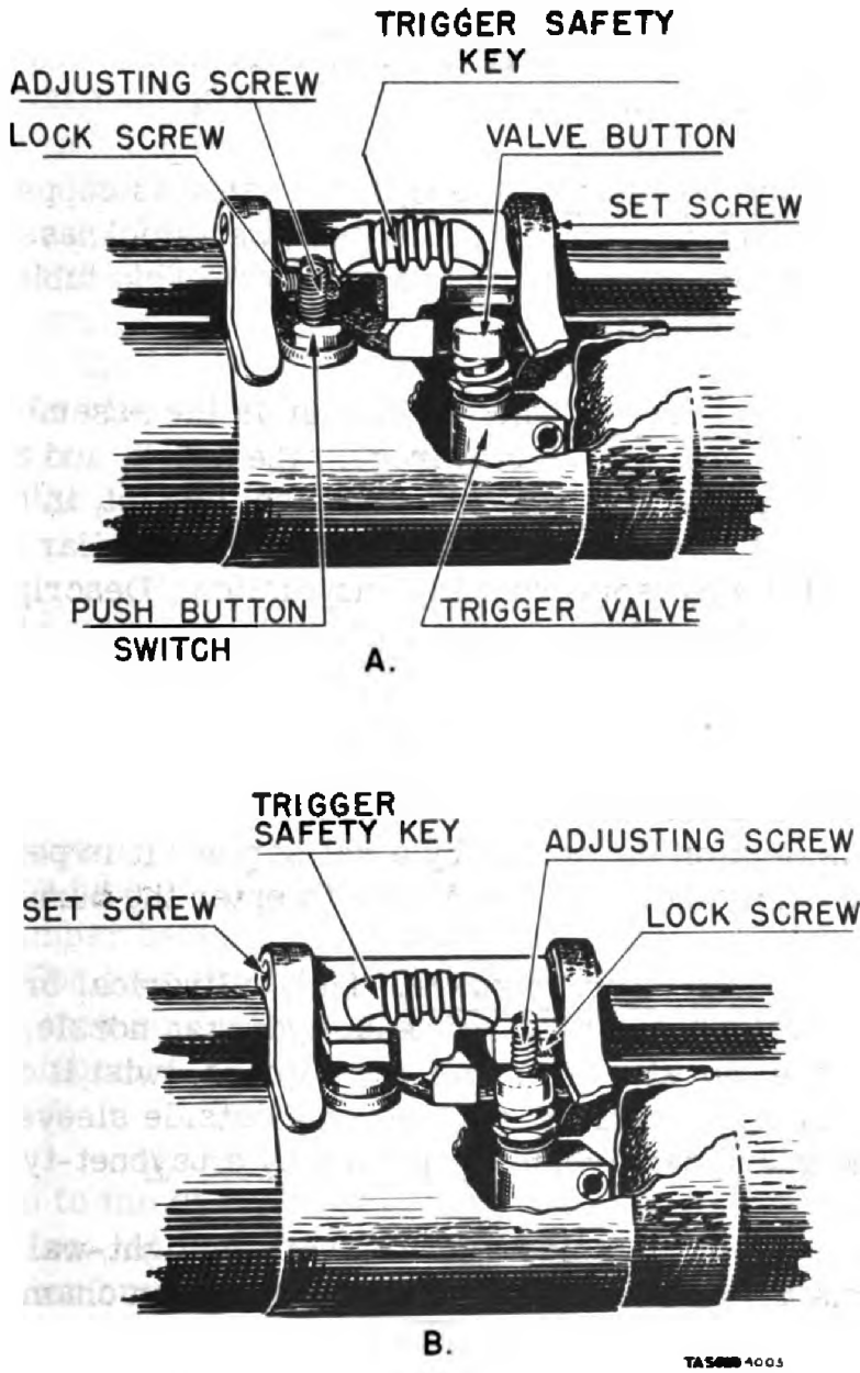
Figure 7. Trigger Assembly, Showing Trigger Safety Key in (A) The Normal Position and (B) The Forward and Depressed Firing Position.
