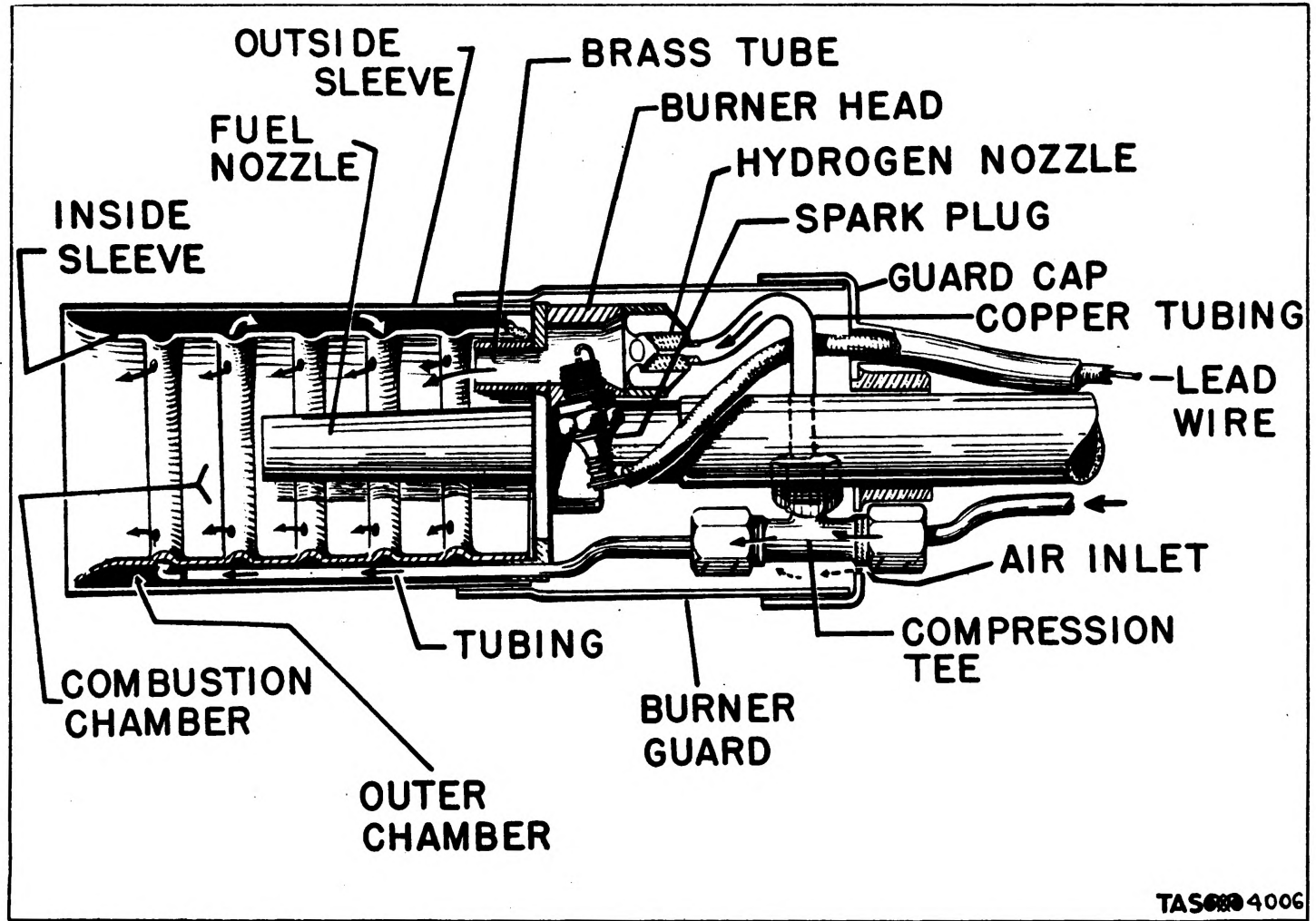
Figure 8. Gas Burner Assembly, Older Type, Cross Section.
