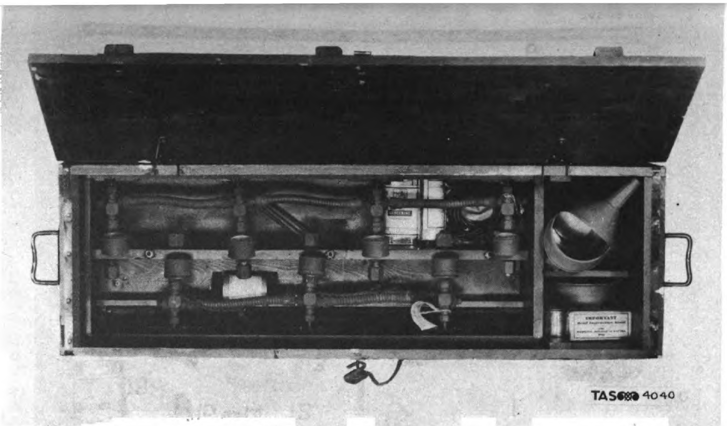
Figure 50. M1A1 Service Kit, with Tray Removed, Showing Filling Manifold Assemblies for Hydrogen and Pressure Cylinders. (See Paragraph 61.)
