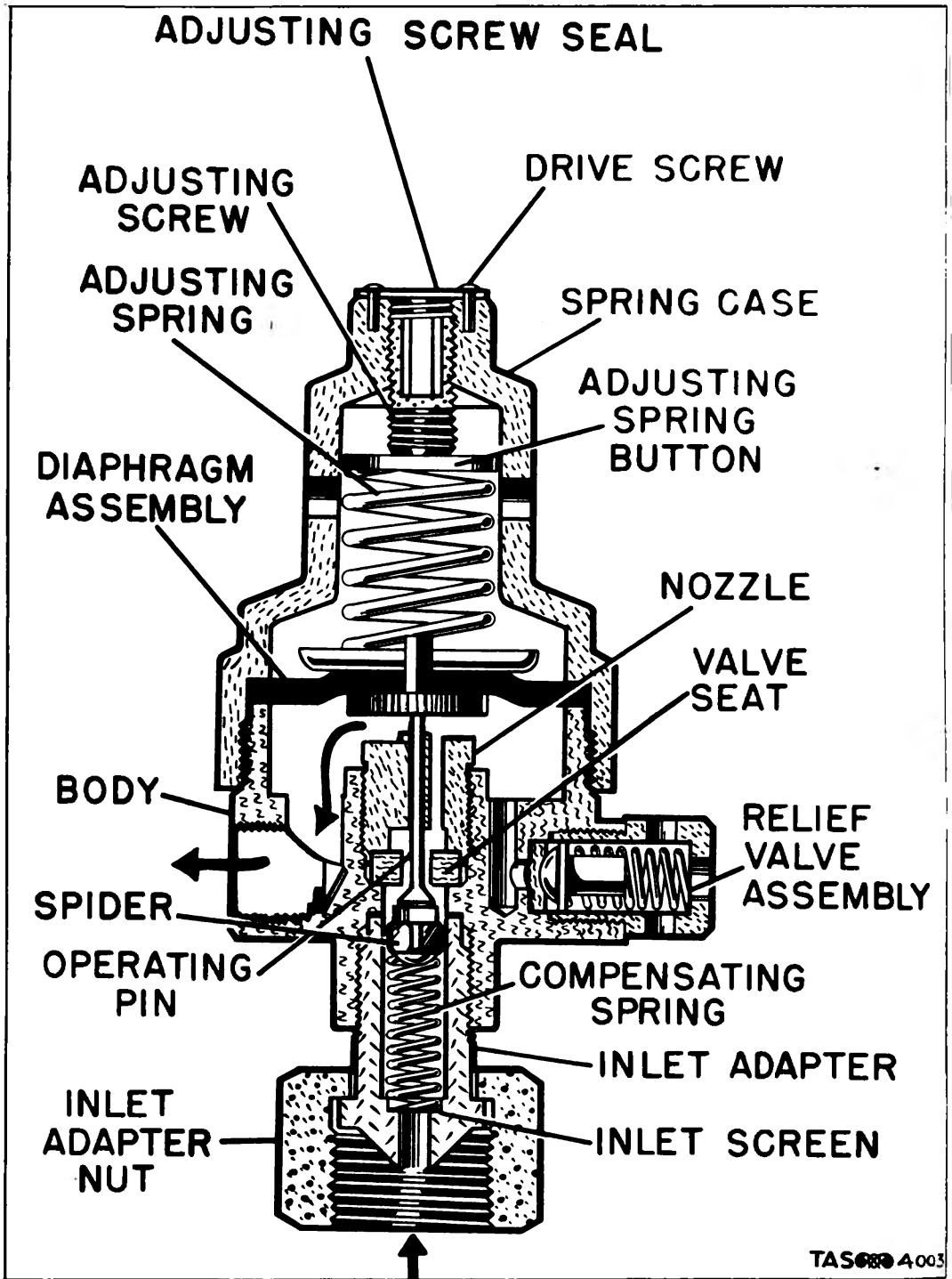
Figure 6. Pressure Regulator Assembly, in Cross Section.
