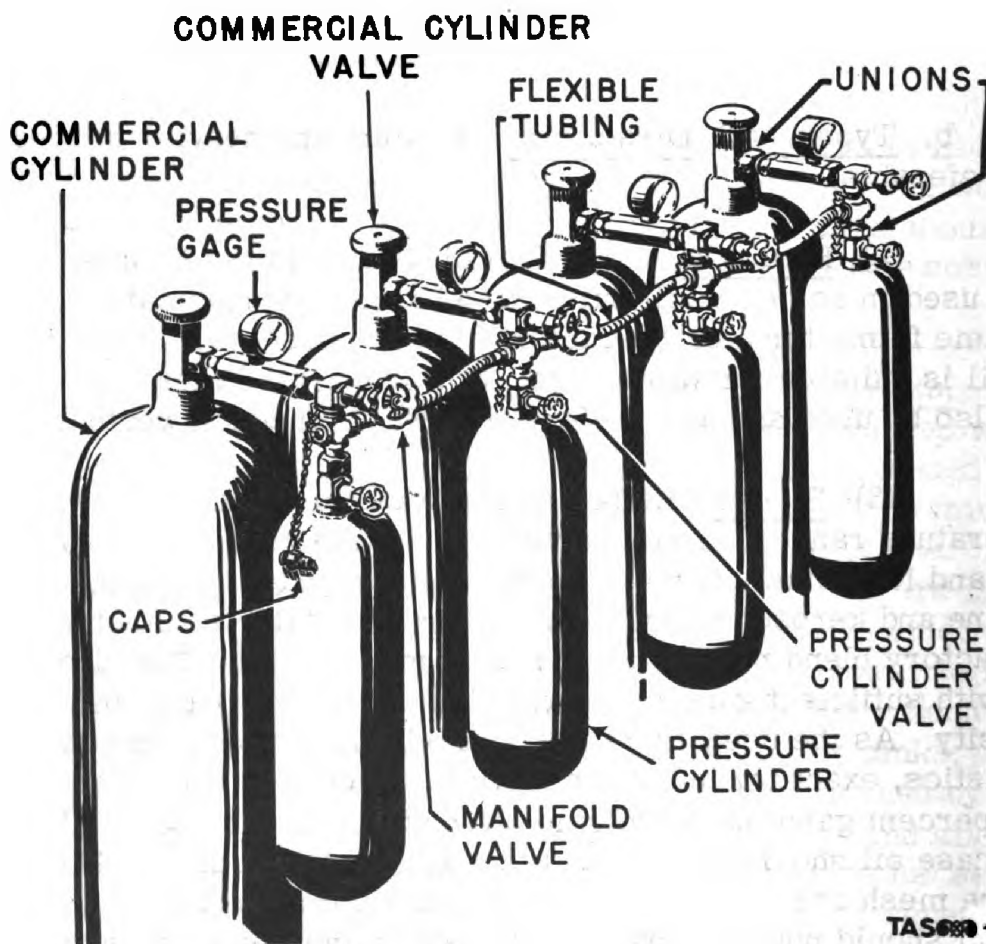
Figure 29. Commercial Cylinders, Pressure Manifold, And Pressure Cylinders, Mounted for Charging.
