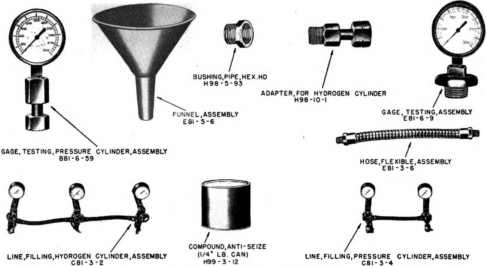
FIGURE 47. Accessories Supplied in Kit, Service, for Portable Flame Thrower M1A1.
