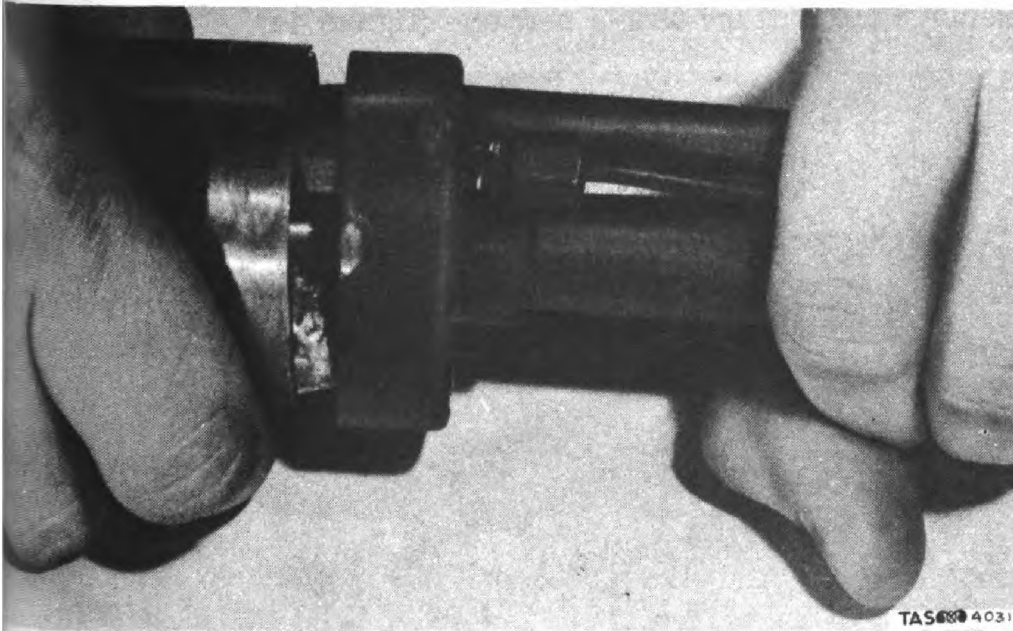
Figure 41.. Burner Guard Twisted by Hand from Guard Cap and over Outer Sleeve.
