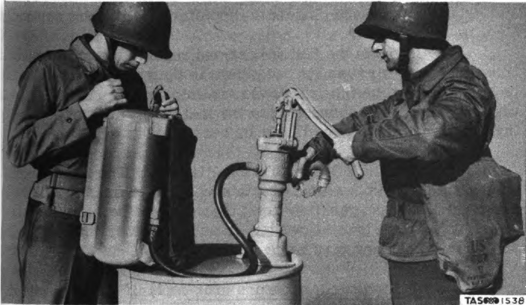
Figure 27. Transferring "Aged" Fuel to Flame Thrower from Shipping Drum.
