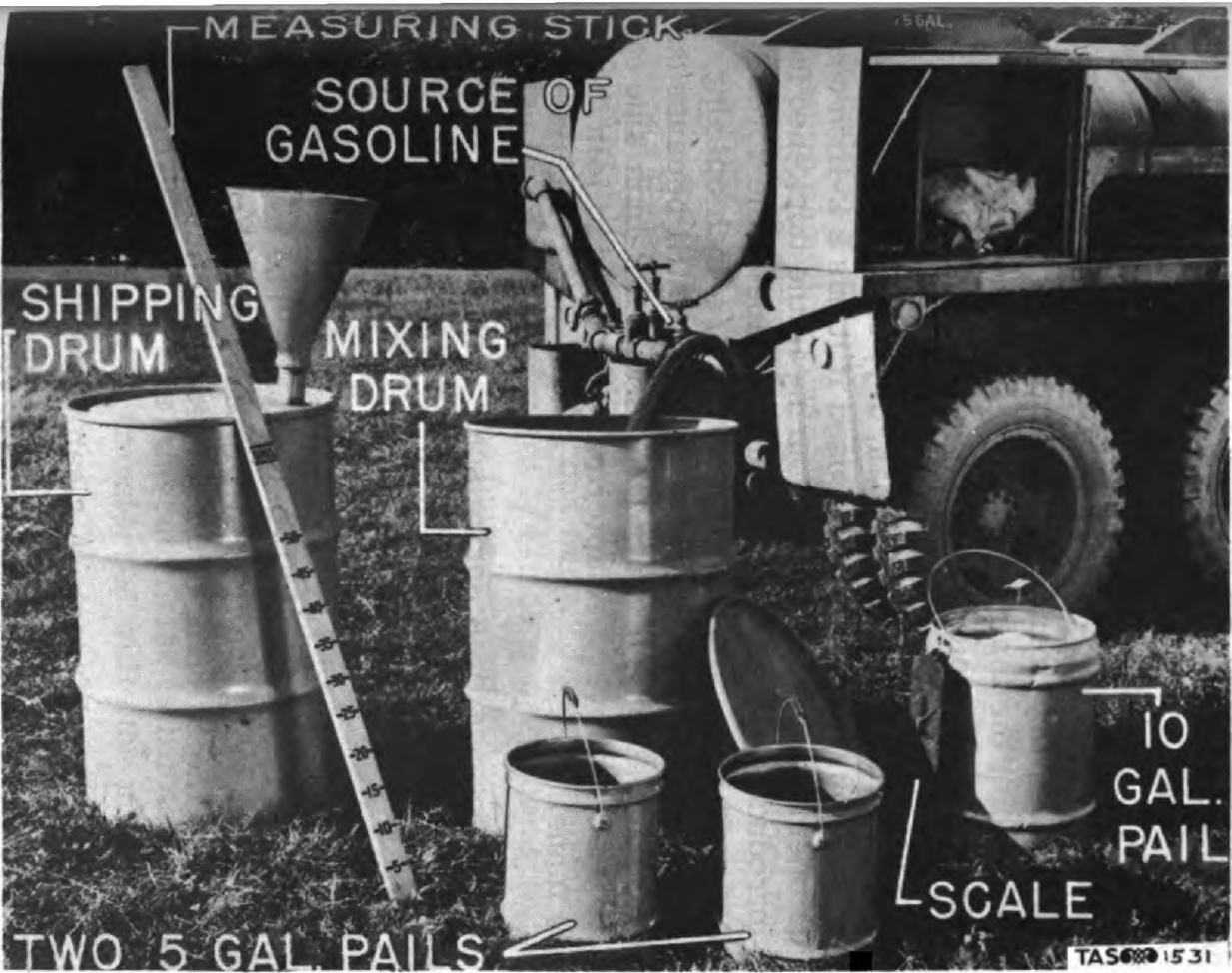
Figure 32. Apparatus Used for Fuel Mixing.
