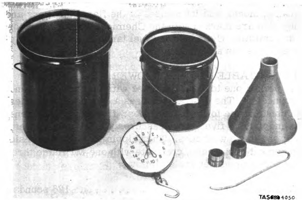
Figure 57. Partial Contents of Fuel Mixing Kit.
