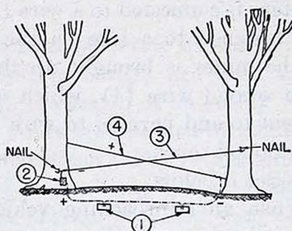
FIGURE 48.—Elektrischemine (electrically operated mine, type C).
