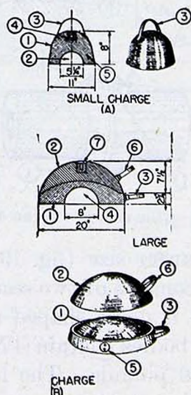
FIGURE 19.—Demolition charges for armored structures.
