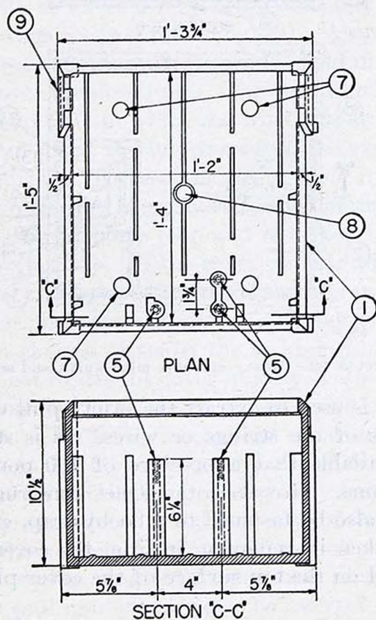
FIGURE 28.—Heavy antitank mine—plan and section of box.
