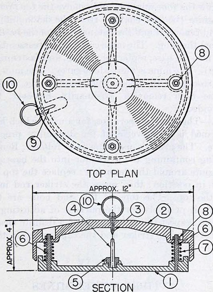
FIGURE 81.—Land mine, railway type.
