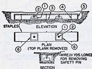
FIGURE 39.—Druckbohlemine (pressure plank mine).
