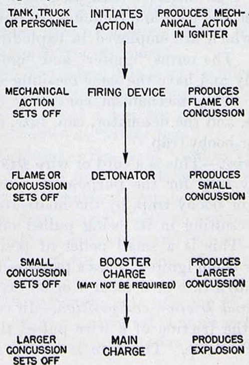
FIGURE 1.—Diagram of firing action.
