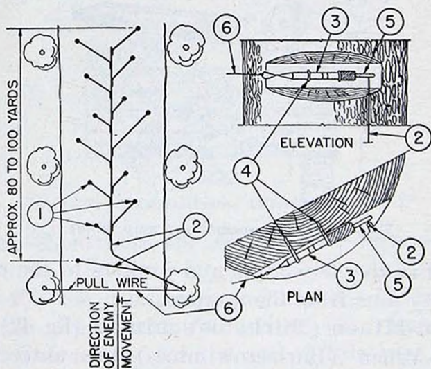
FIGURE 42.—Burbenn-Minen (Burhenn's mines).
