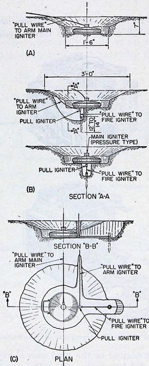
FIGURE 23.—Tellermine in place—sectional views showing antilifting devices.
