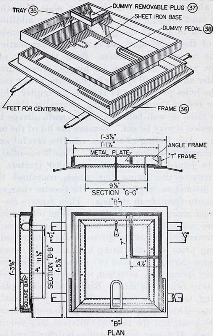
FIGURE 34.—Dummy mine.
