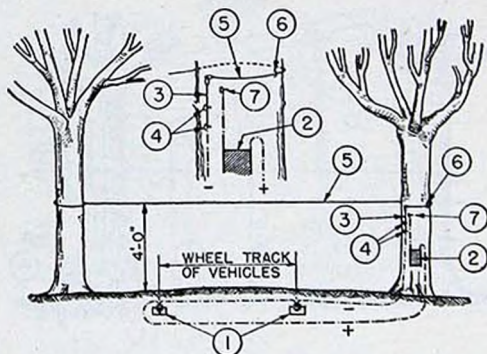
FIGURE 46.—Elektrischemine (electrically operated mine, type A).
