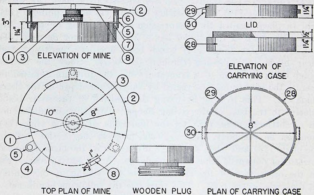
FIGURE 79.—Circular variable pressure mine and igniter carrying case.
