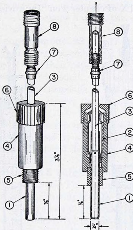
FIGURE 15.—Prepared nonelectric detonator.
