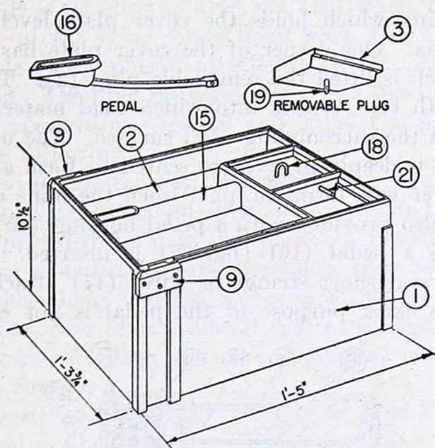
PERSPECTIVE OF BOX AND COVER PLATE
