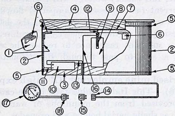
FIGURE 74.—Antitank electric mine, type 2.
