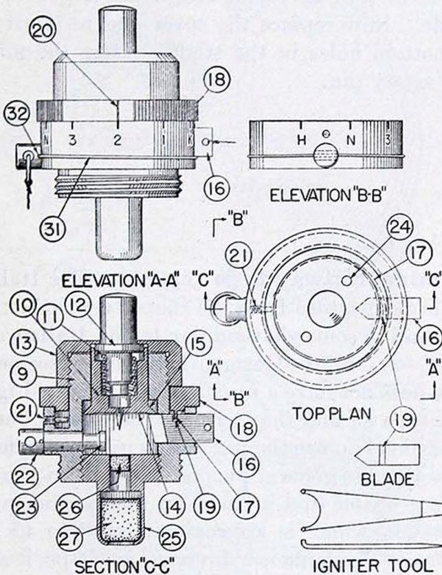
FIGURE 80.—Igniter in circular variable pressure mine—details.
