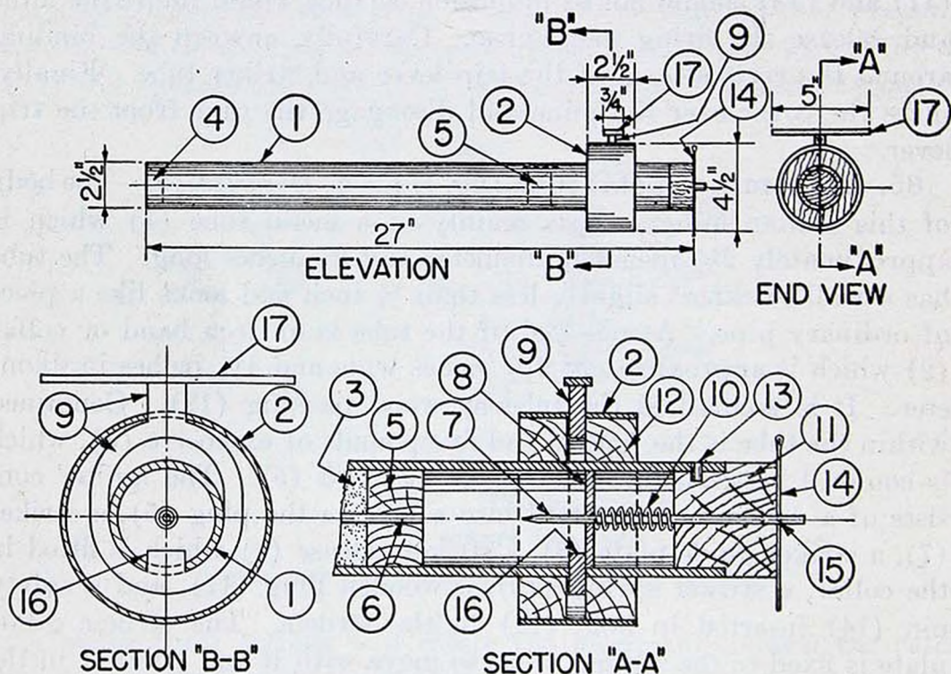
FIGURE 77.—Land mine, metal tube type.
