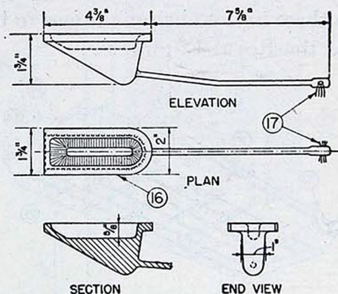
FIGURE 32.—Heavy antitank mine—details of pedal.
