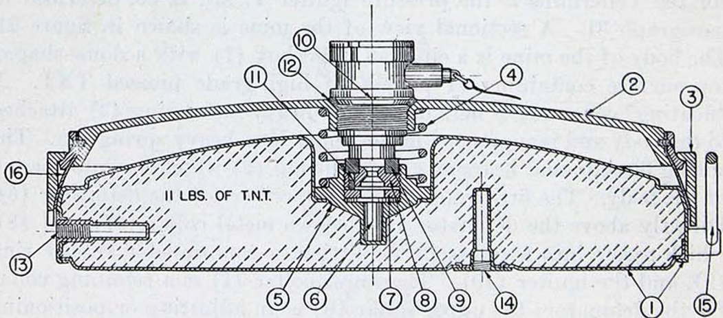
FIGURE 21.—Tellermine—sectional view.
