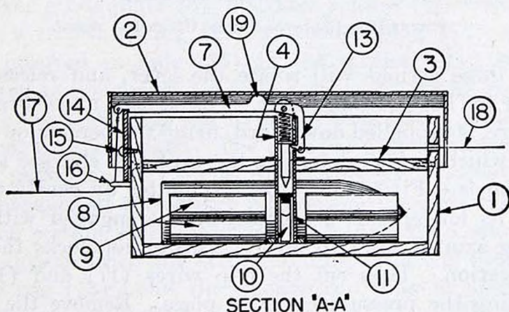
FIGURE 75.—Improvised mine, HE shells.
