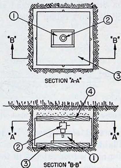
FIGURE 51.—Tretmine (tread mine).
