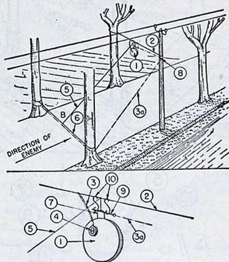
FIGURE 44.—Hangemine (hanging mine).
