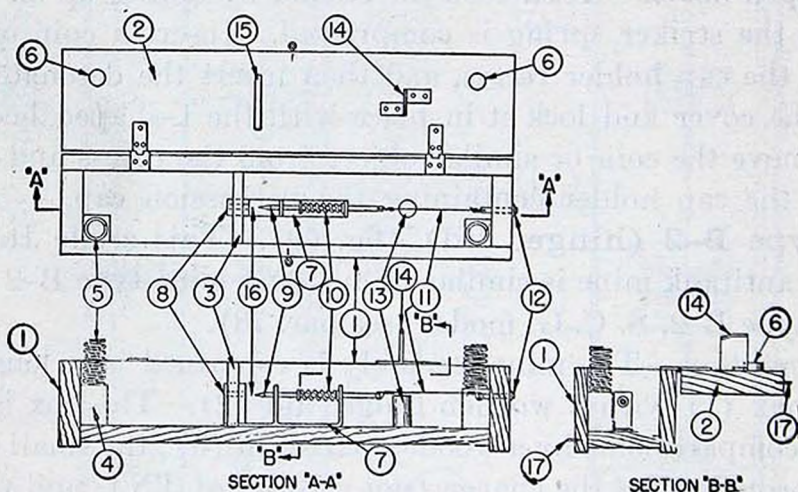
FIGURE 69.—Antitank mine, type B-2 (hinged lid).
