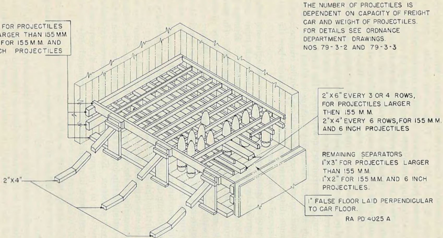
FIGURE 05.—Method of stowing shell in freight car.
