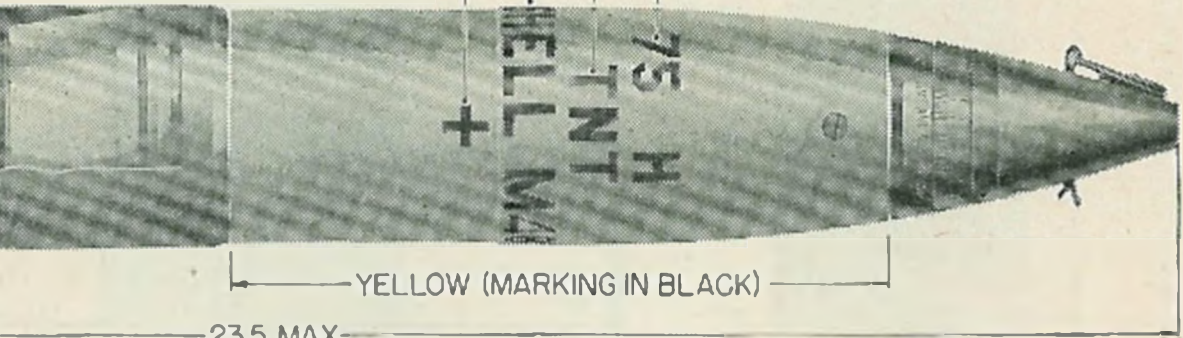
Semifixed ammunition.
