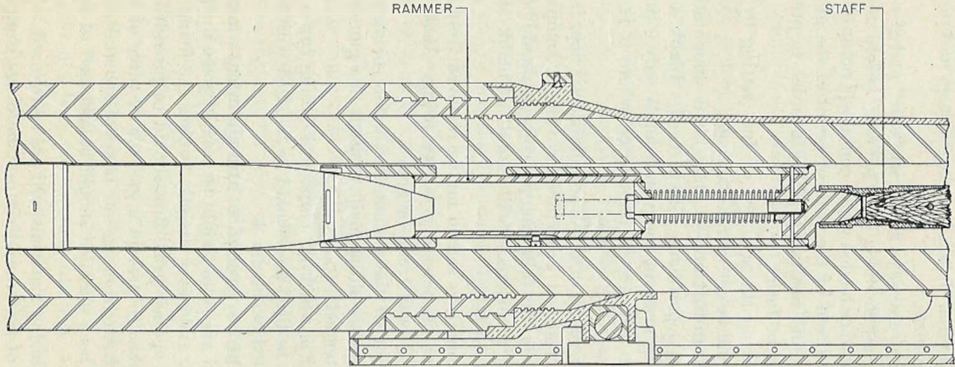
FIGURE 66.—Rammer M1 in use—method of removing shell from gun.
