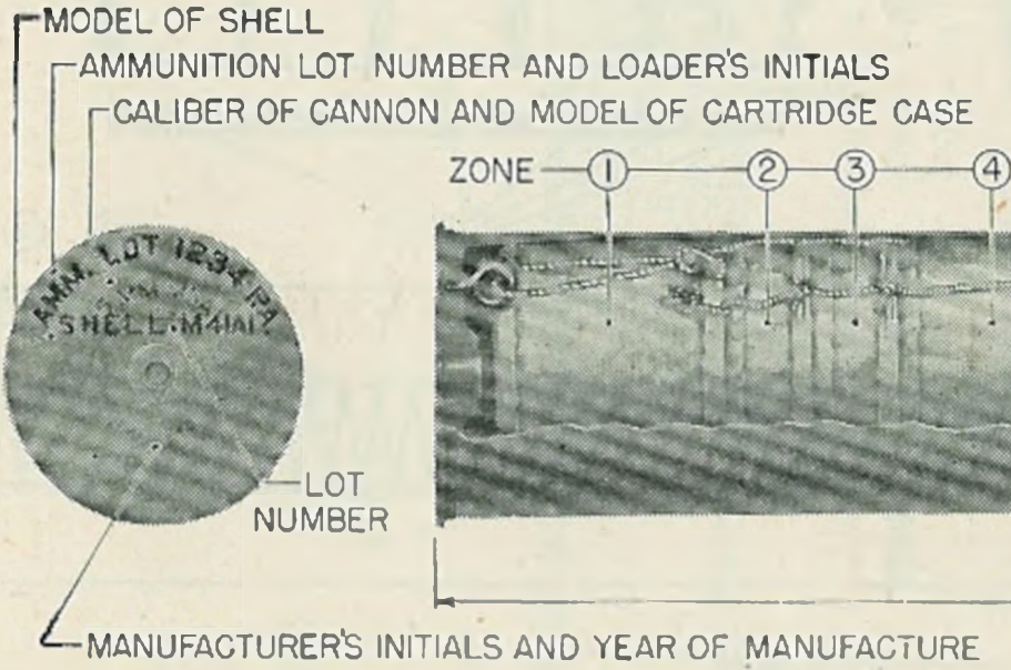
FIGURE 31.—
