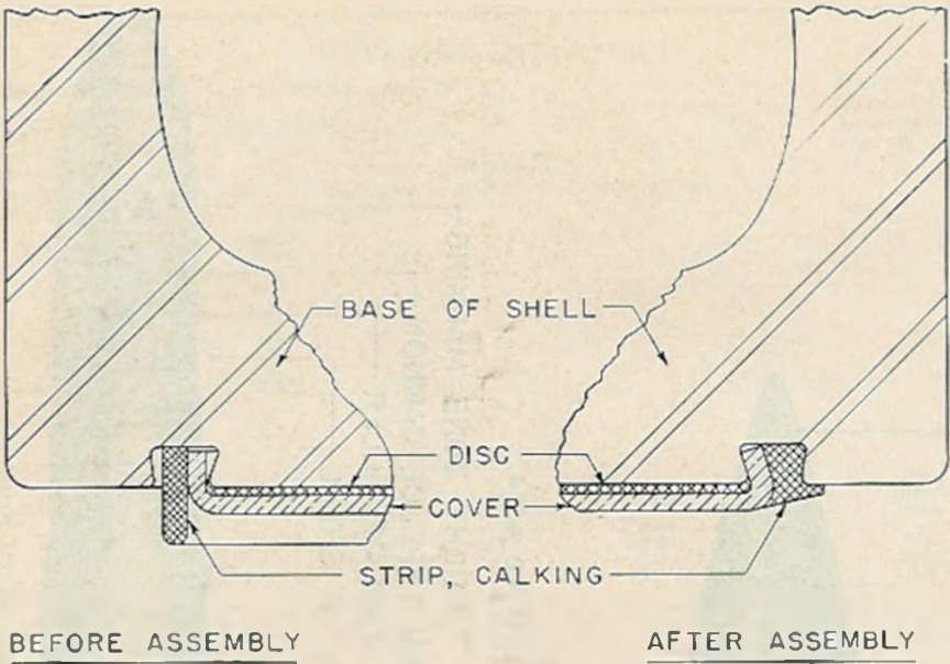
FIGURE 22.—Base cover detail.
