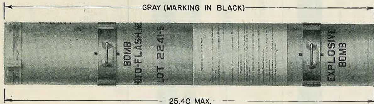
FIGURE 57.—Bomb, photoflash, M23A1.
