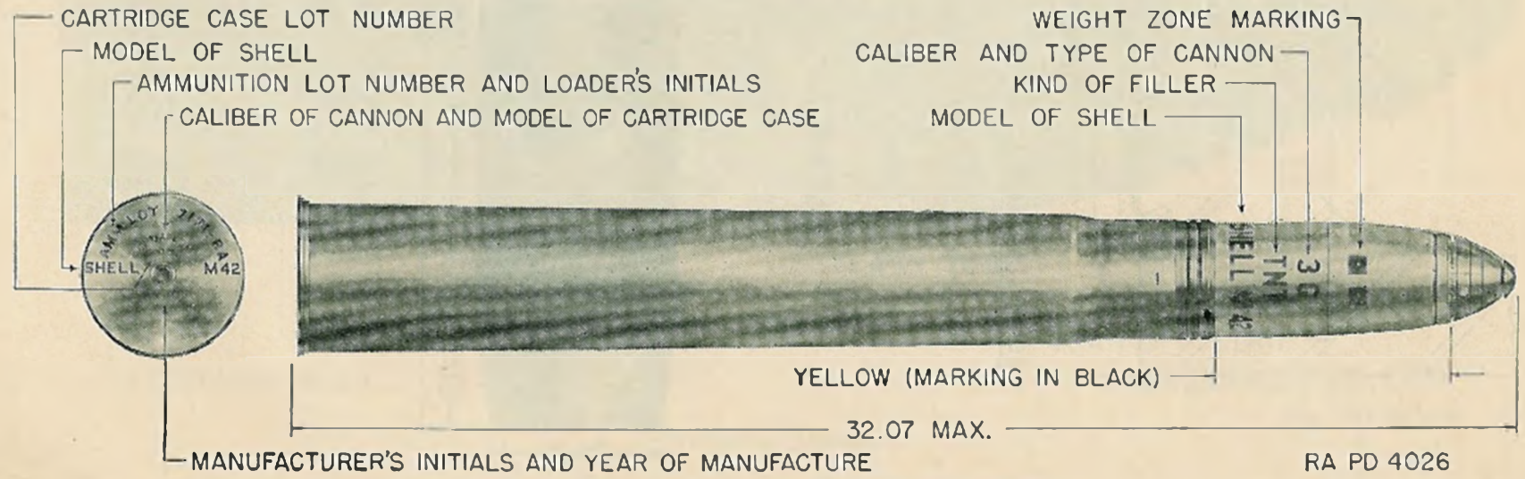
FIGURE 21.—Antiaircraft 3-inch high explosive projectile.
