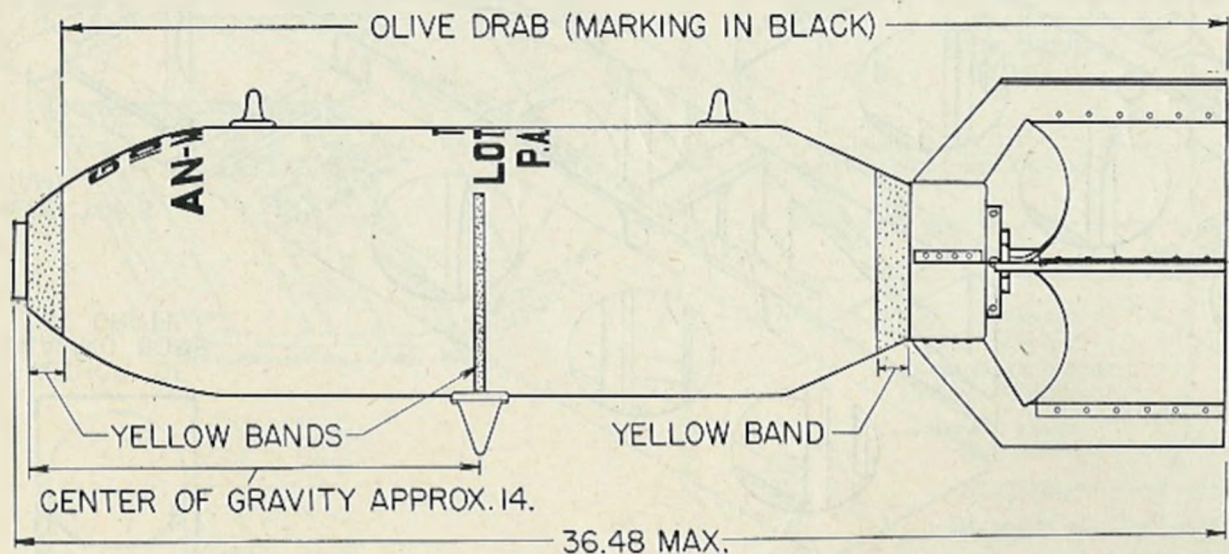
BOMB, GENERAL PURPOSE, 100-LB., AN-M30, UNFUZED
