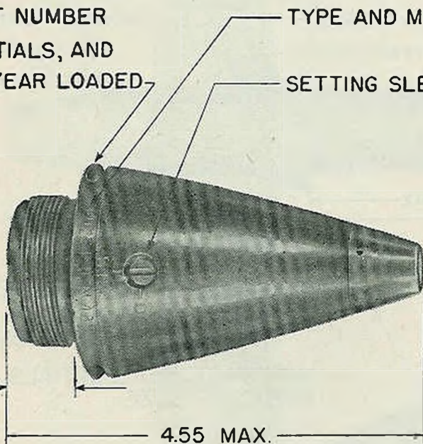
FIGURE 30.—Fuze, point-detonating, M48.
