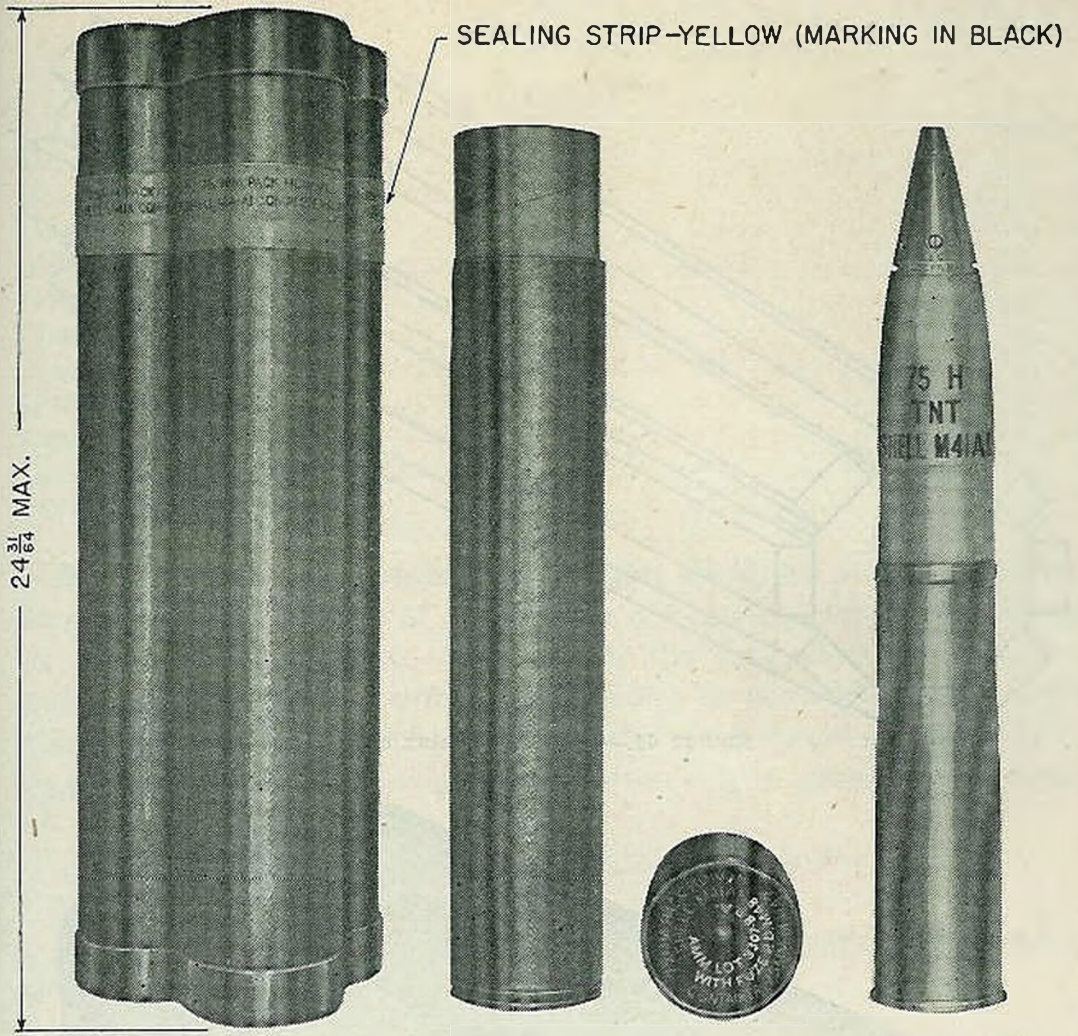
FIGURE 40.—Bundle packing.
