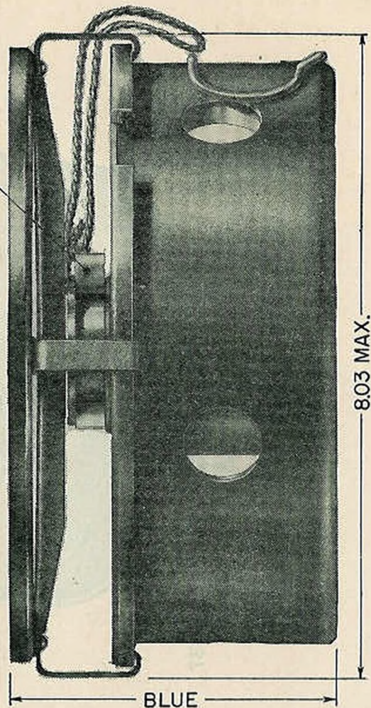
FIGURE 14.—Mine, antitank, practice, M1.
