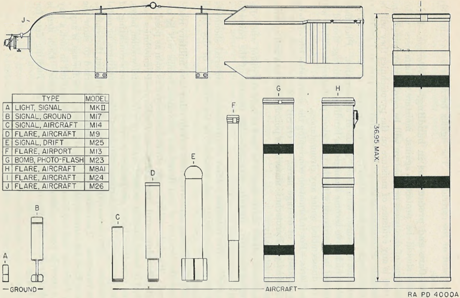
FIGURE 52.—Types of pyrotechnics.
