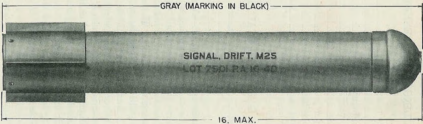
FIGURE 62.—Signal, drift, M25.
