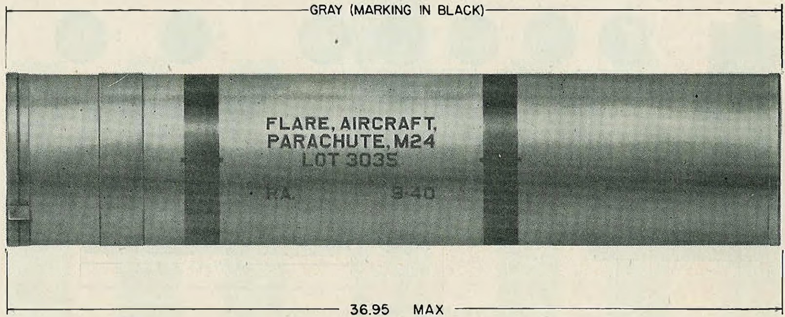
FIGURE 58.—Flare, aircraft, parachute, M24.
