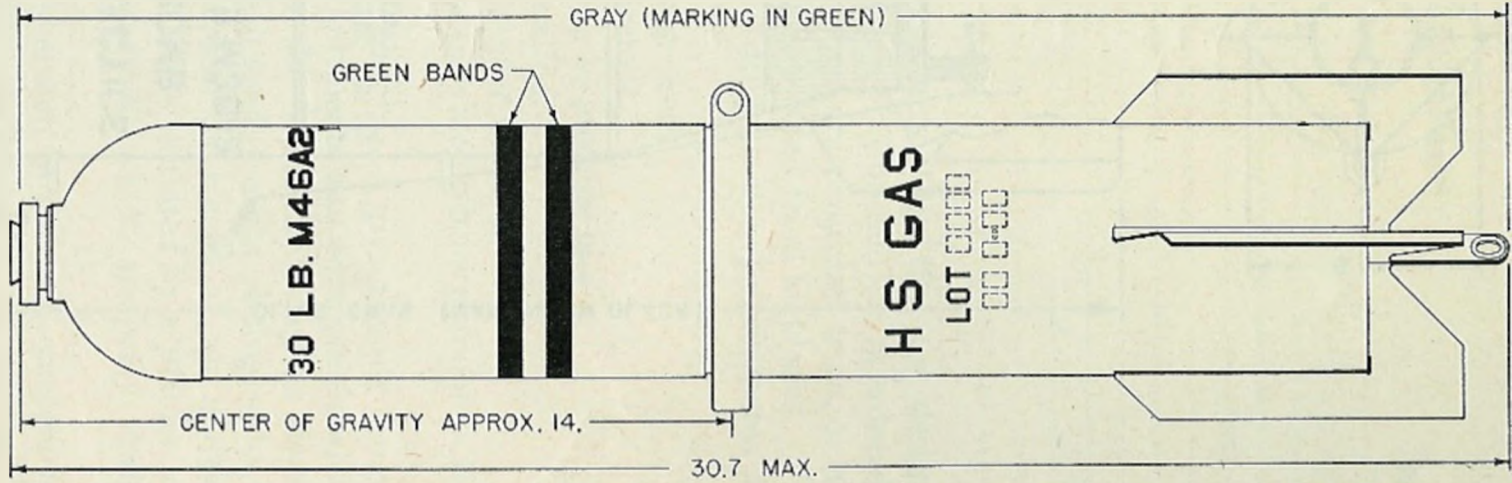
FIGURE 50.—Bomb, gas, persistent, HS, 30-pound.
