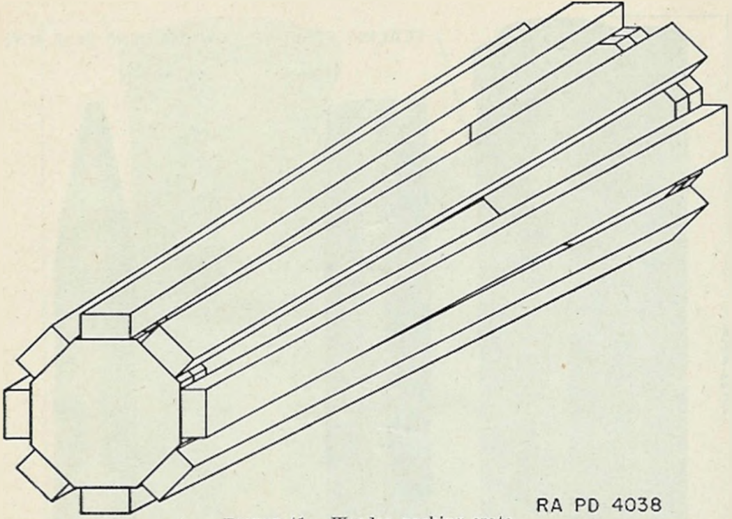
FIGURE 41.—Wooden packing crate.
