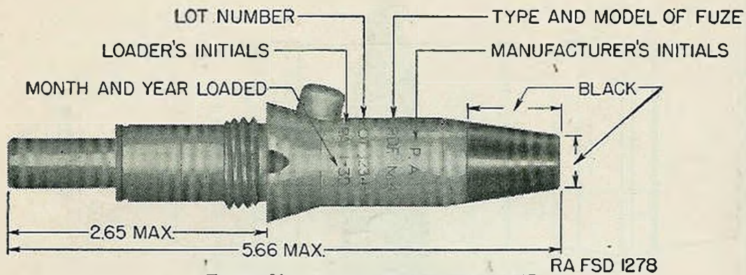
FIGURE 29.—Fuze, point-detonating, M47.
