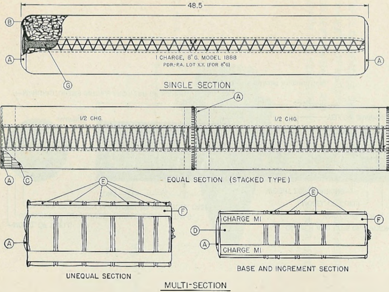
FIGURE 32.—Propellent charges.
