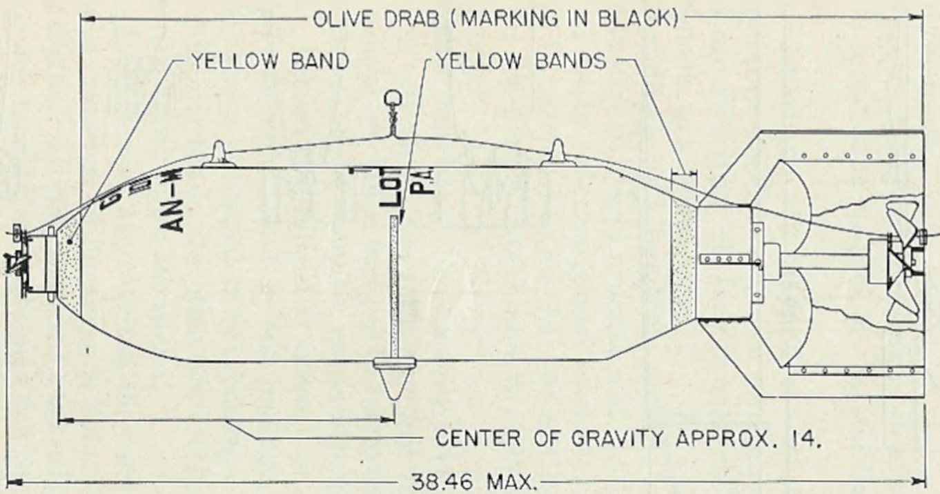
FIGURE 44.—Bomb, demolition, 100-pound, complete round.
