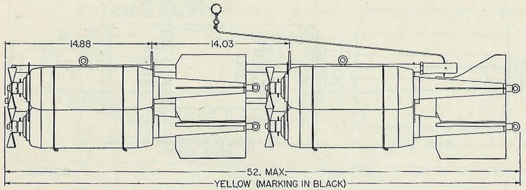
FIGURE 49.—Fragmentation bomb cluster.
