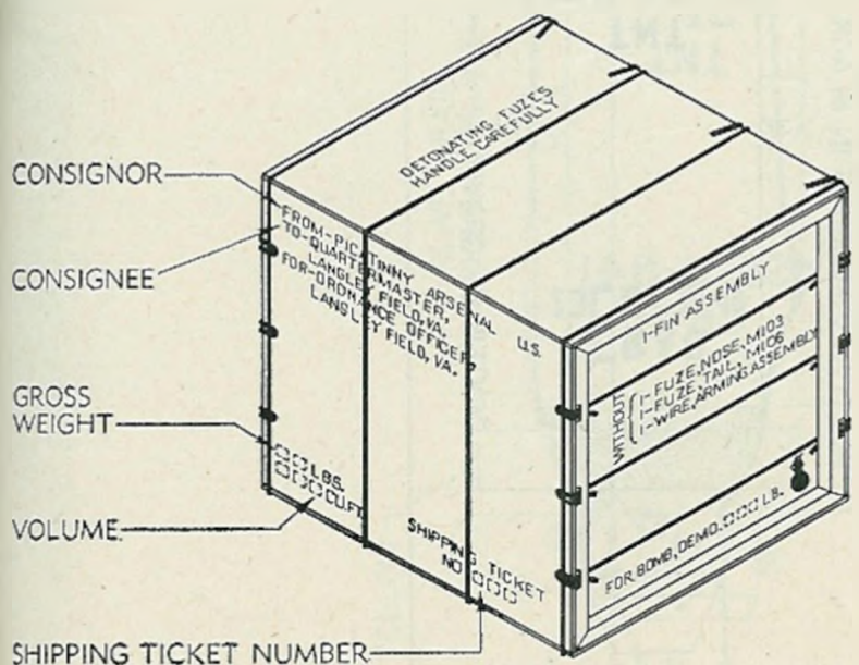
FIGURE 47.—Bomb, demolition, 1,000-pound (as shipped).
