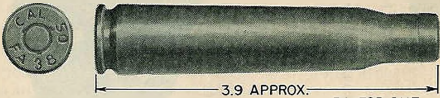
FIGURE 7.—Cartridge, blank, caliber .50.
