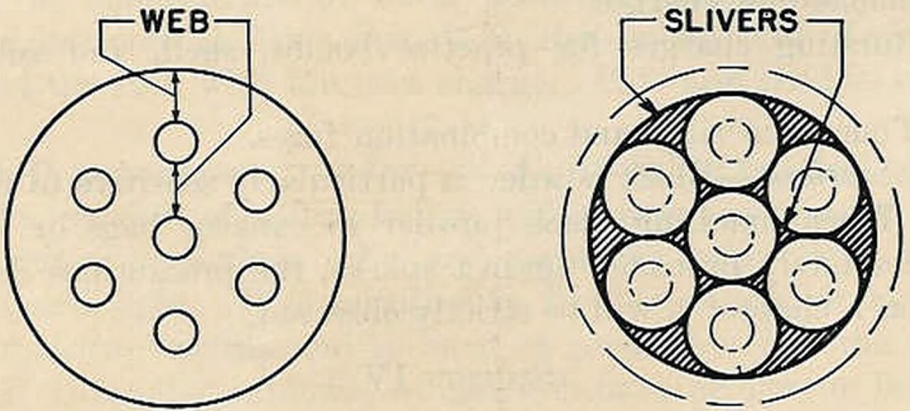
FIGURE 2.—Burning of powder grains.
