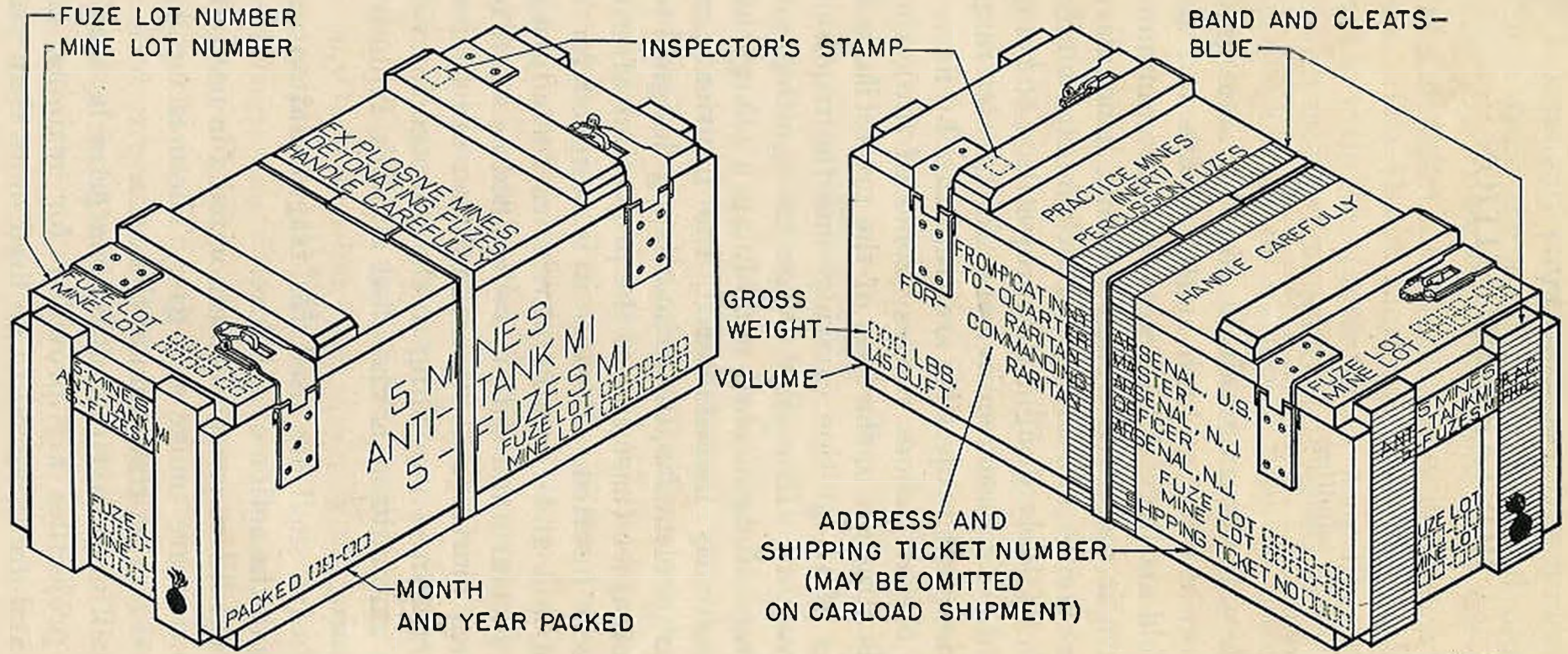
FIGURE 16.—Packings for antitank mines.
