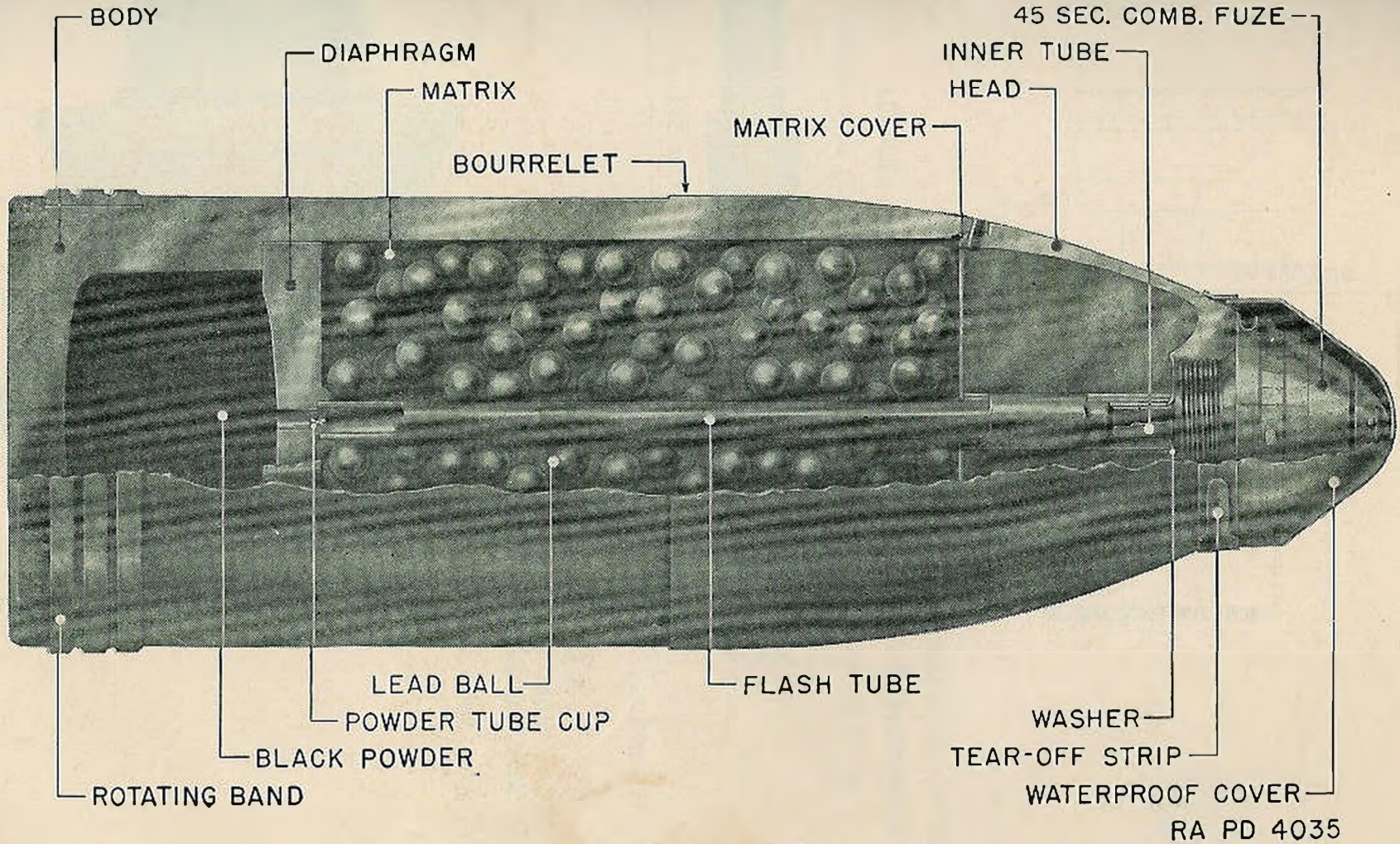
FIGURE 24.—Shrapnel.
