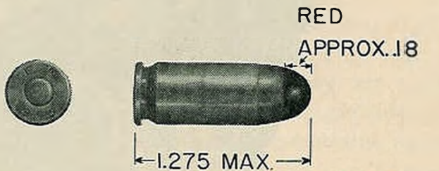
FIGURE 9.—Cartridge, tracer, caliber .45.
