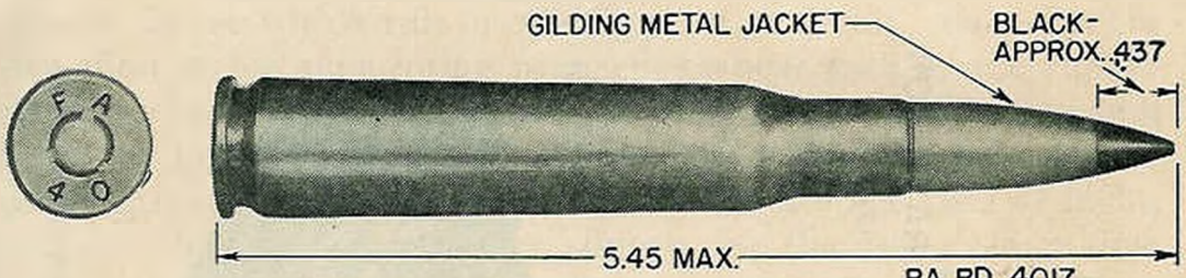
FIGURE 6.—Cartridge, armor-piercing, caliber .50.
