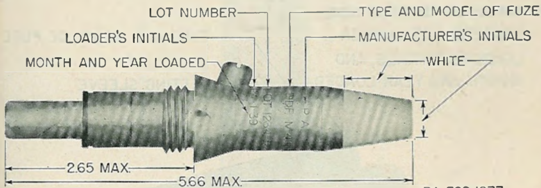
FIGURE 27.—Fuze, point-detonating, M46.
