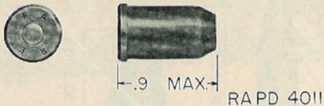
FIGURE 10.—Cartridge, blank, caliber .45.
