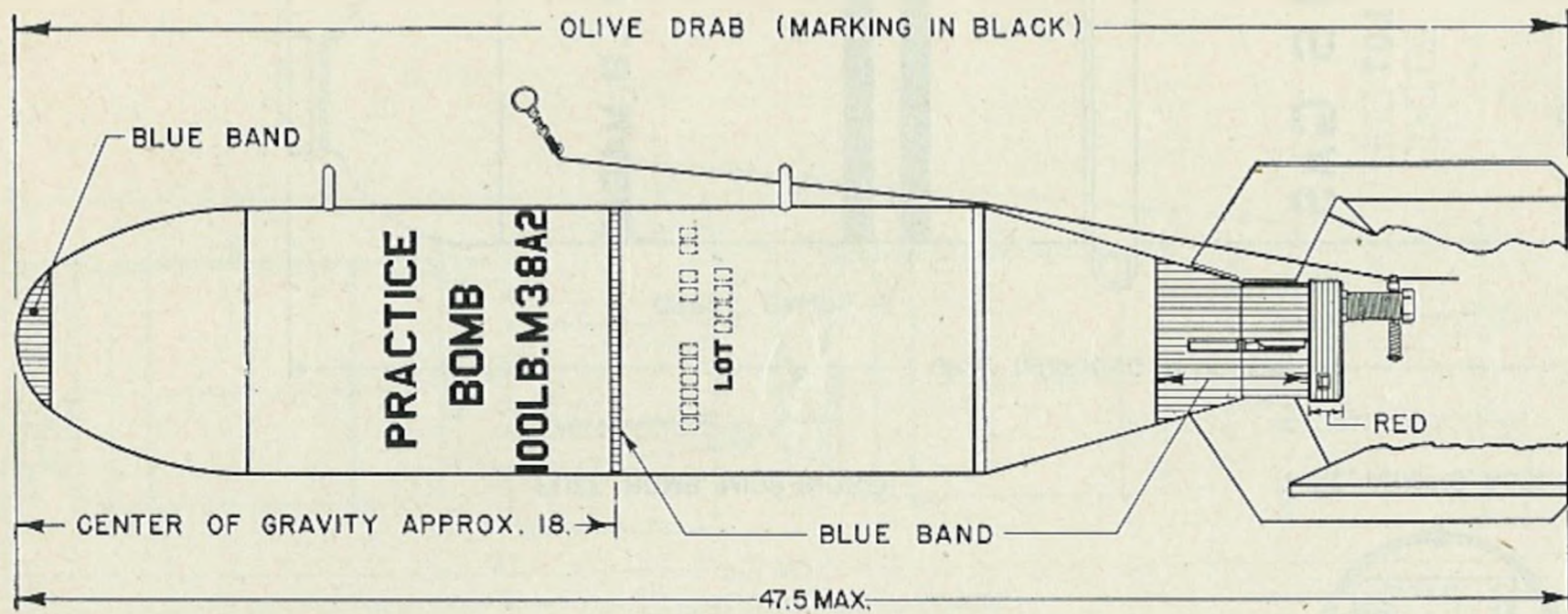
FIGURE 51.—Bomb, practice, 100-pound.
