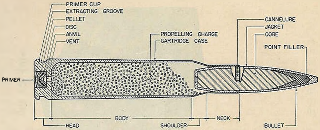
FIGURE 5.—Section of ball cartridge, caliber .50.
