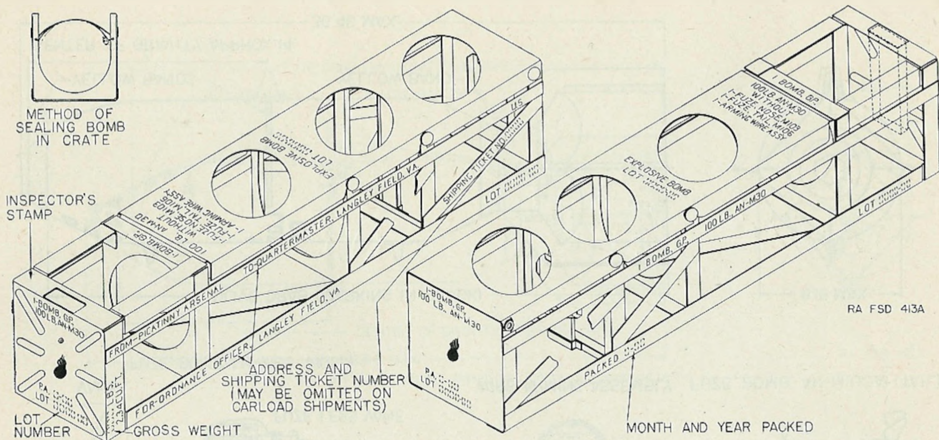
FIGURE 46.—Bomb, demolition, packing and marking of crate.
