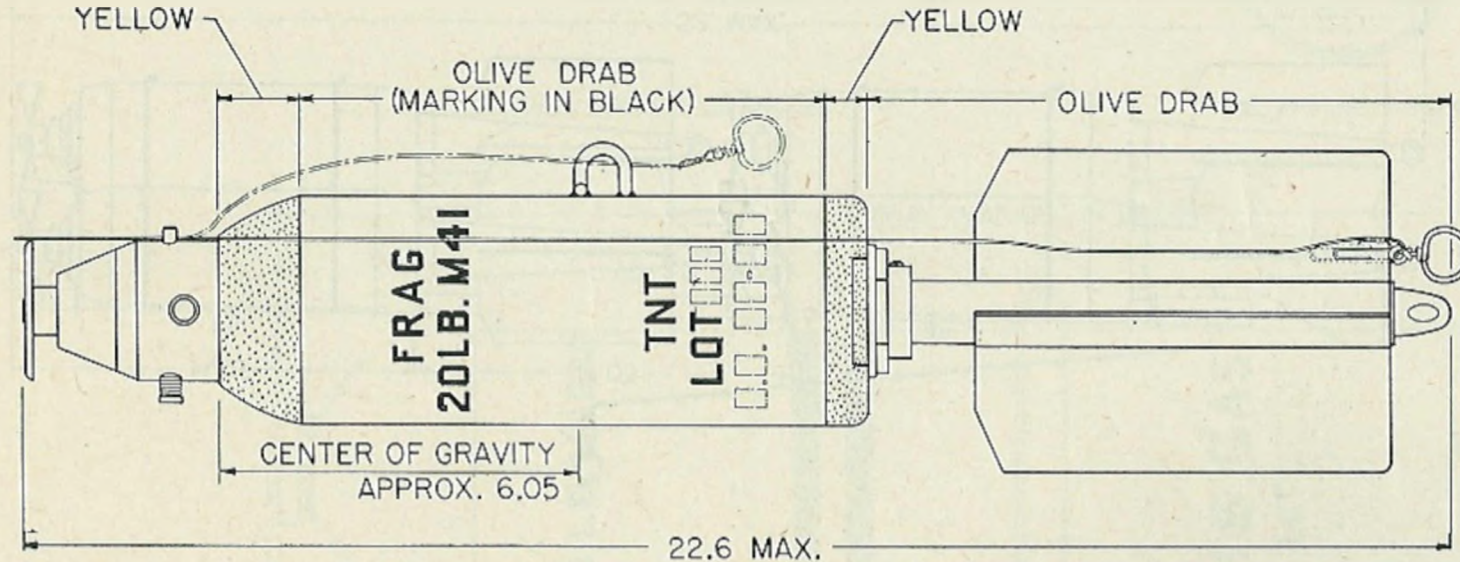
© Bomb, fragmentation, 20-pound.
