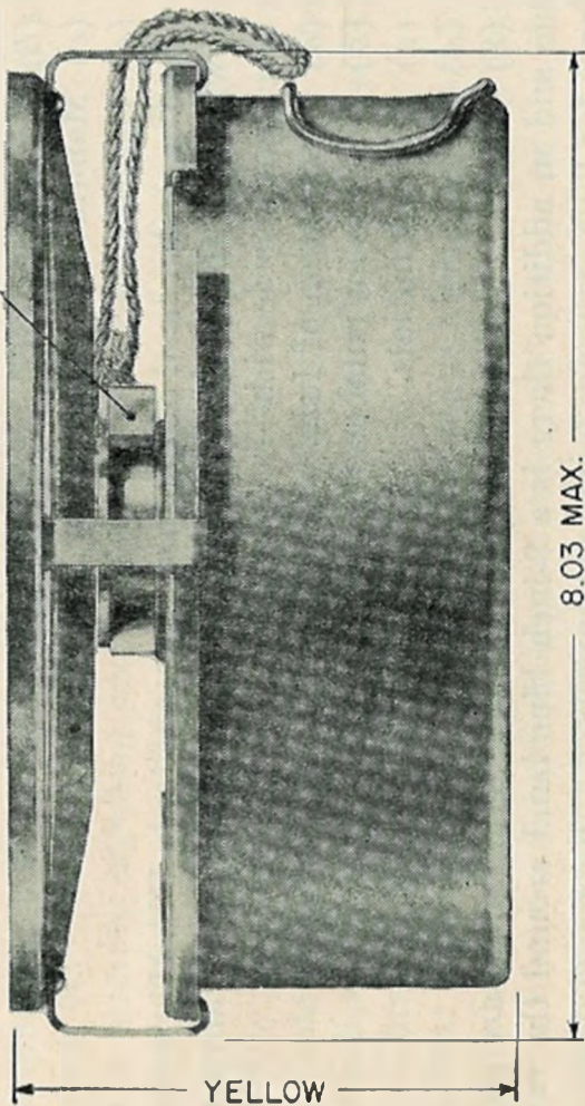
FIGURE 13.—Mine, antitank, high explosive, M1.
