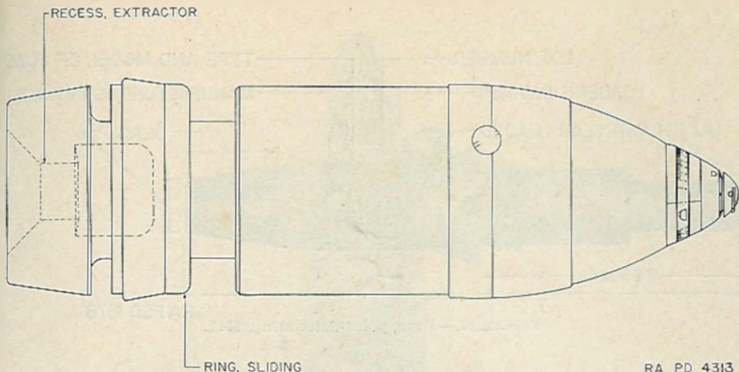
FIGURE 26.—Dummy shell.
