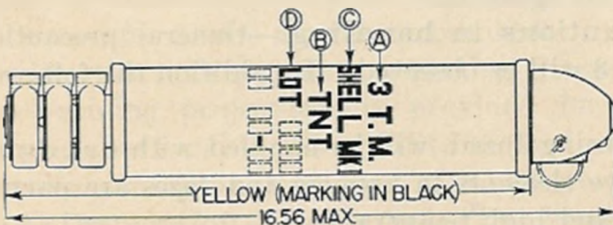
FIGURE 17.—Types of mortar shell.
