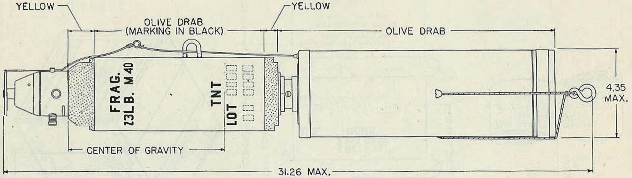
① Bomb, fragmentation, 23-pound.
