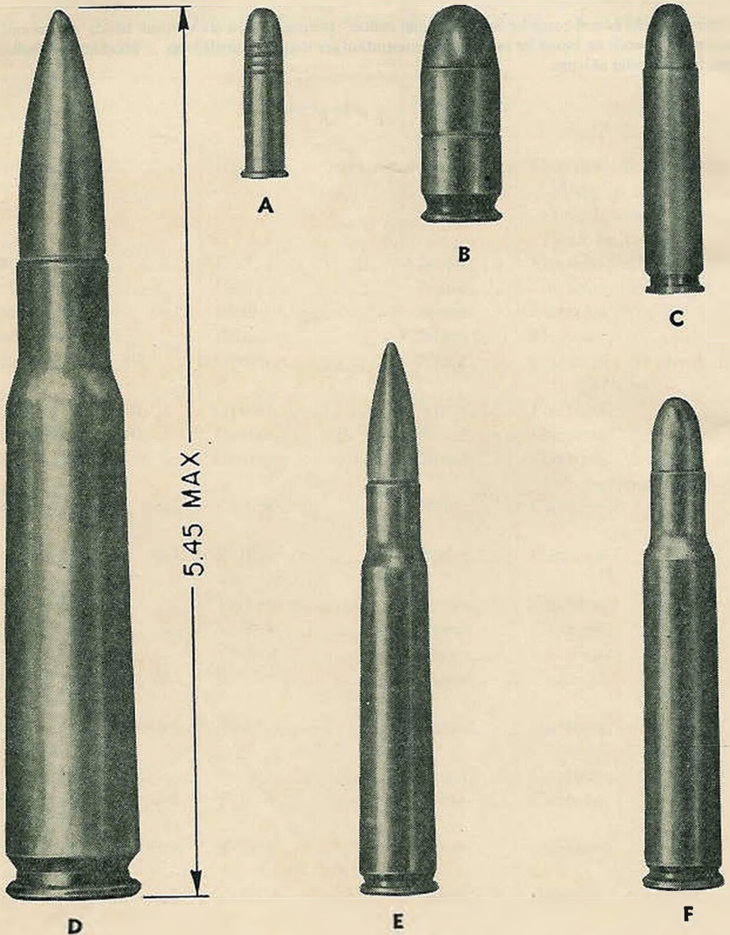
FIGURE 4.—Typical ball cartridges.
