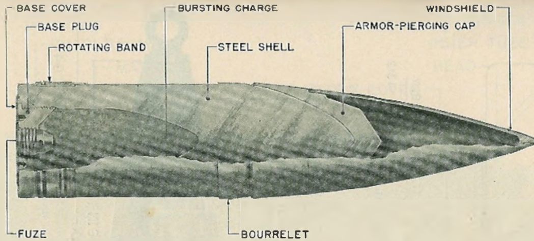
FIGURE 20.—Armor-piercing projectile.
