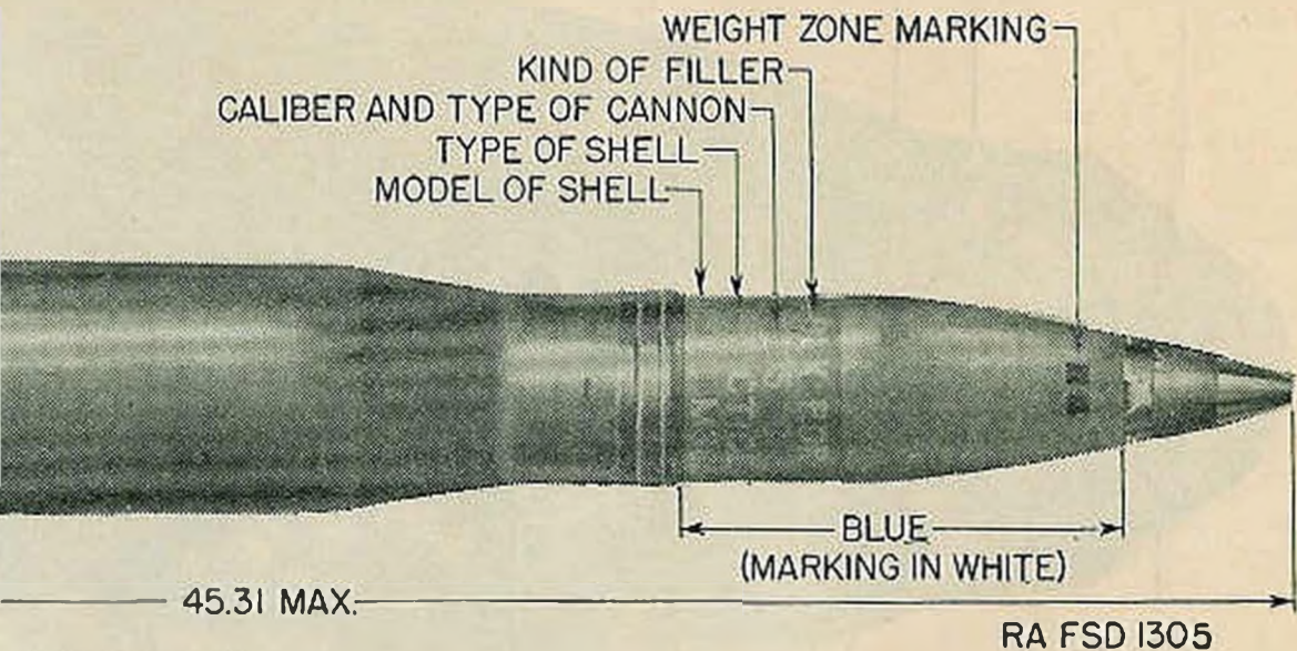
-Practice shell.
