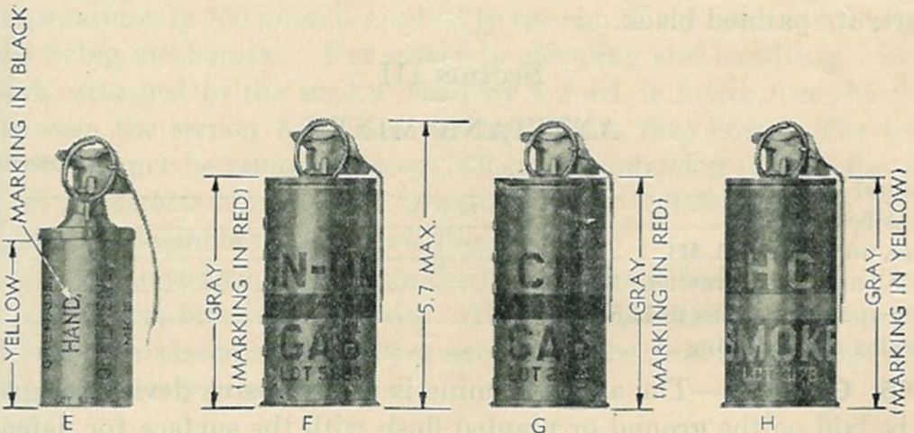
FIGURE 12.—Typical grenades.
