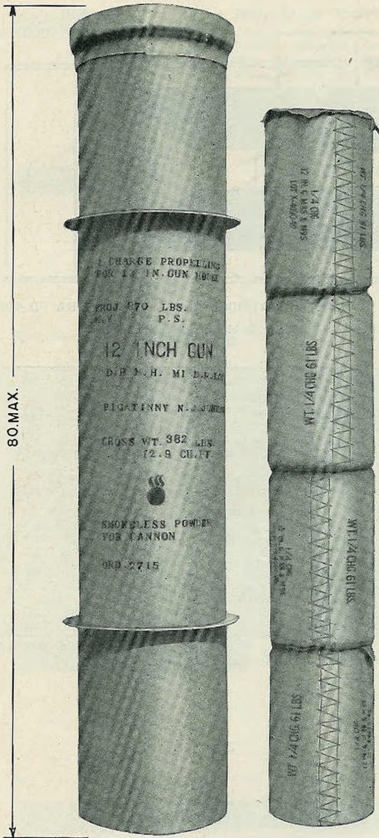
FIGURE 39.—Cartridge storage case and charge. RA PD 4315
