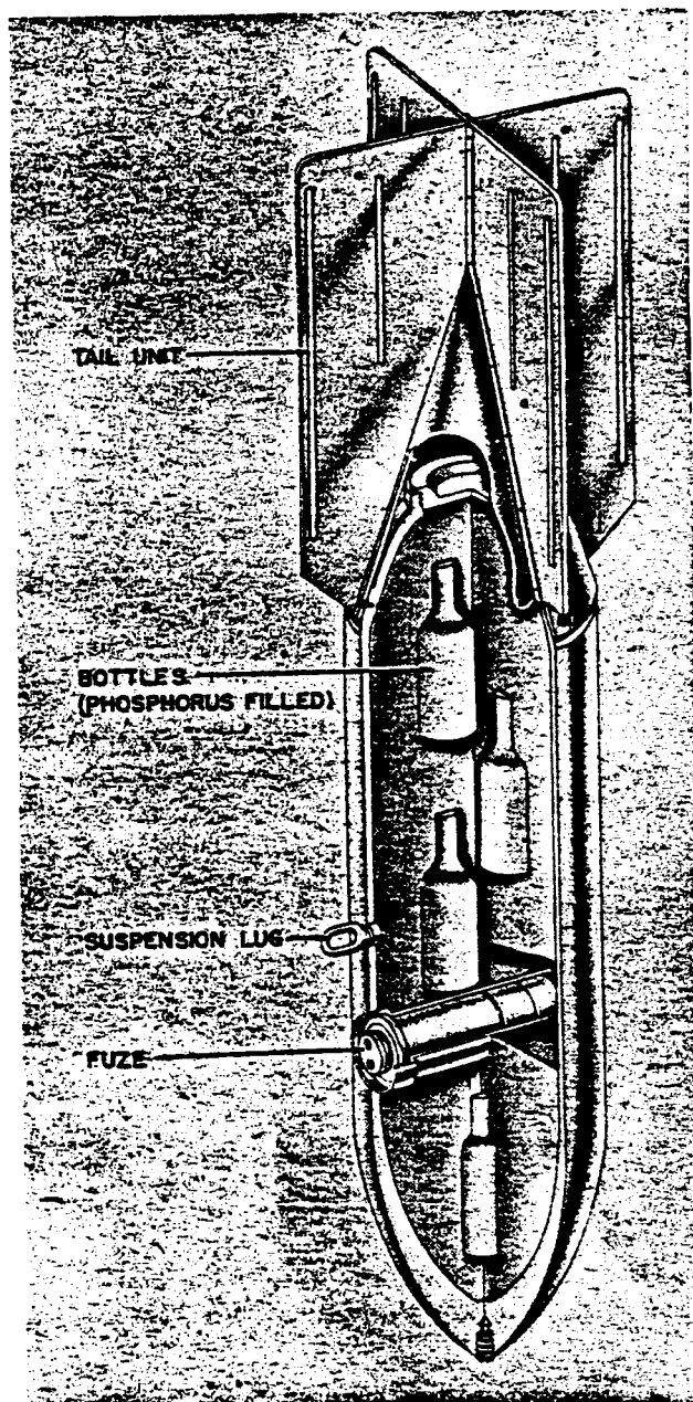
Figure 58—Brand C 50 A Bomb
