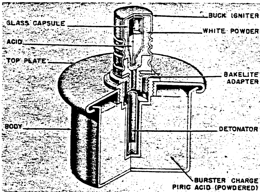
Figure 248—Mustard Pot Mine—Antipersonnel
