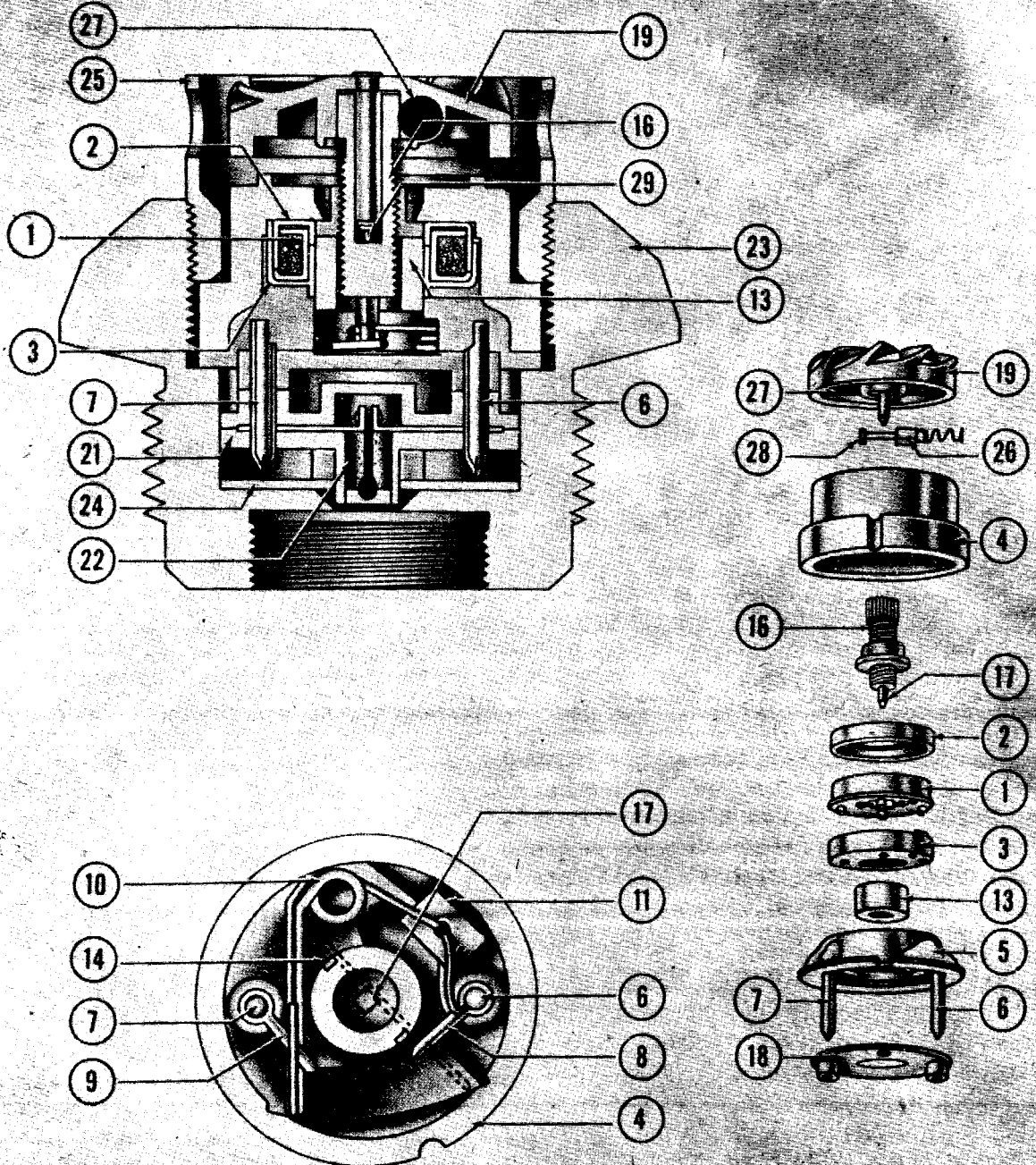
Figure 149—(66) Special Impact Fuze
