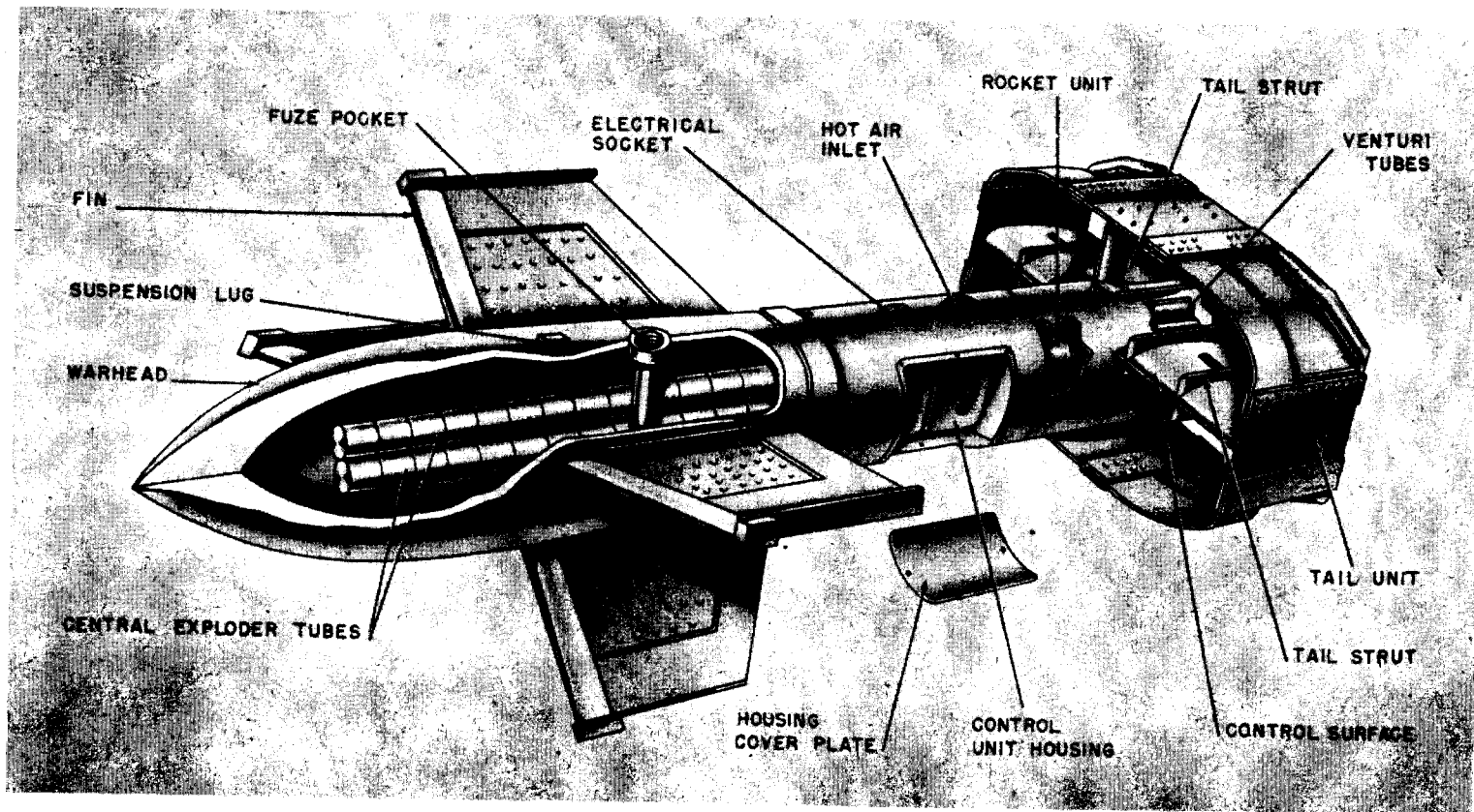
Figure 192—1400 FX
