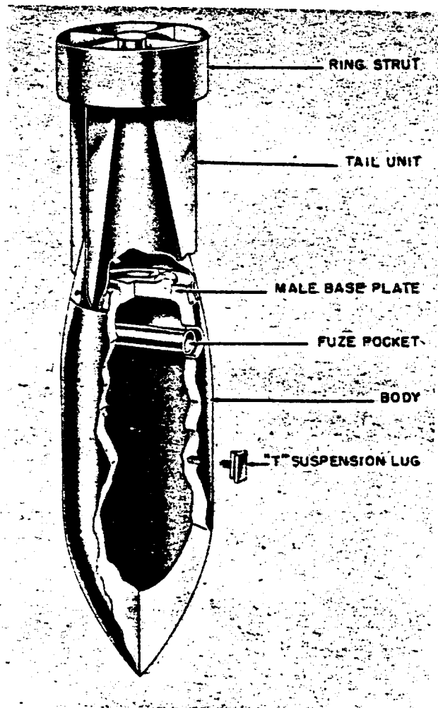
Figure 29—PC 500-Kg Bomb
