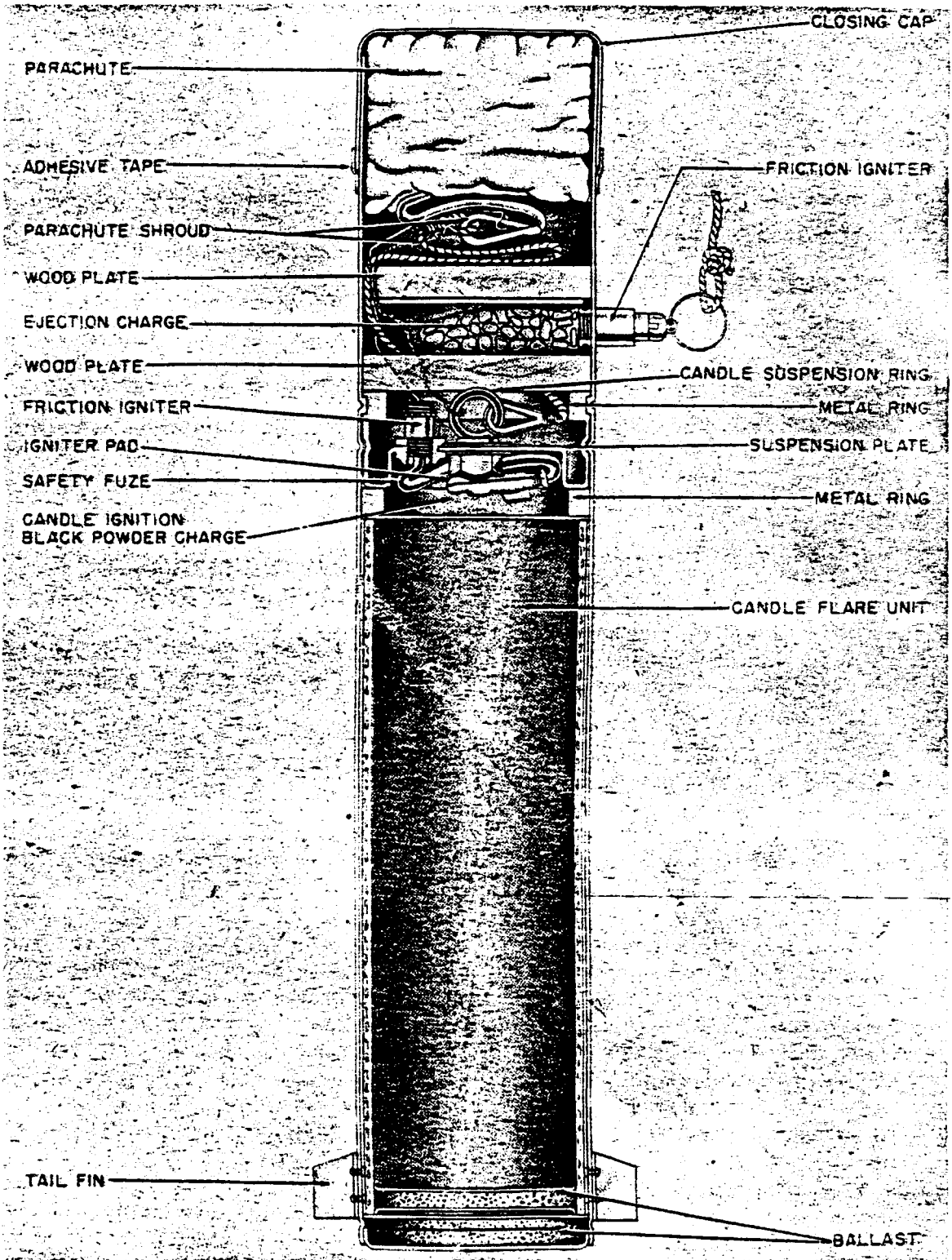
Figure 79—Parachute Flare (Red)—Single Unit
