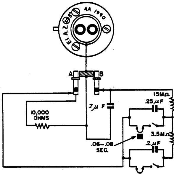
Figure 162—(28)B e Electrical Impact Fuze
