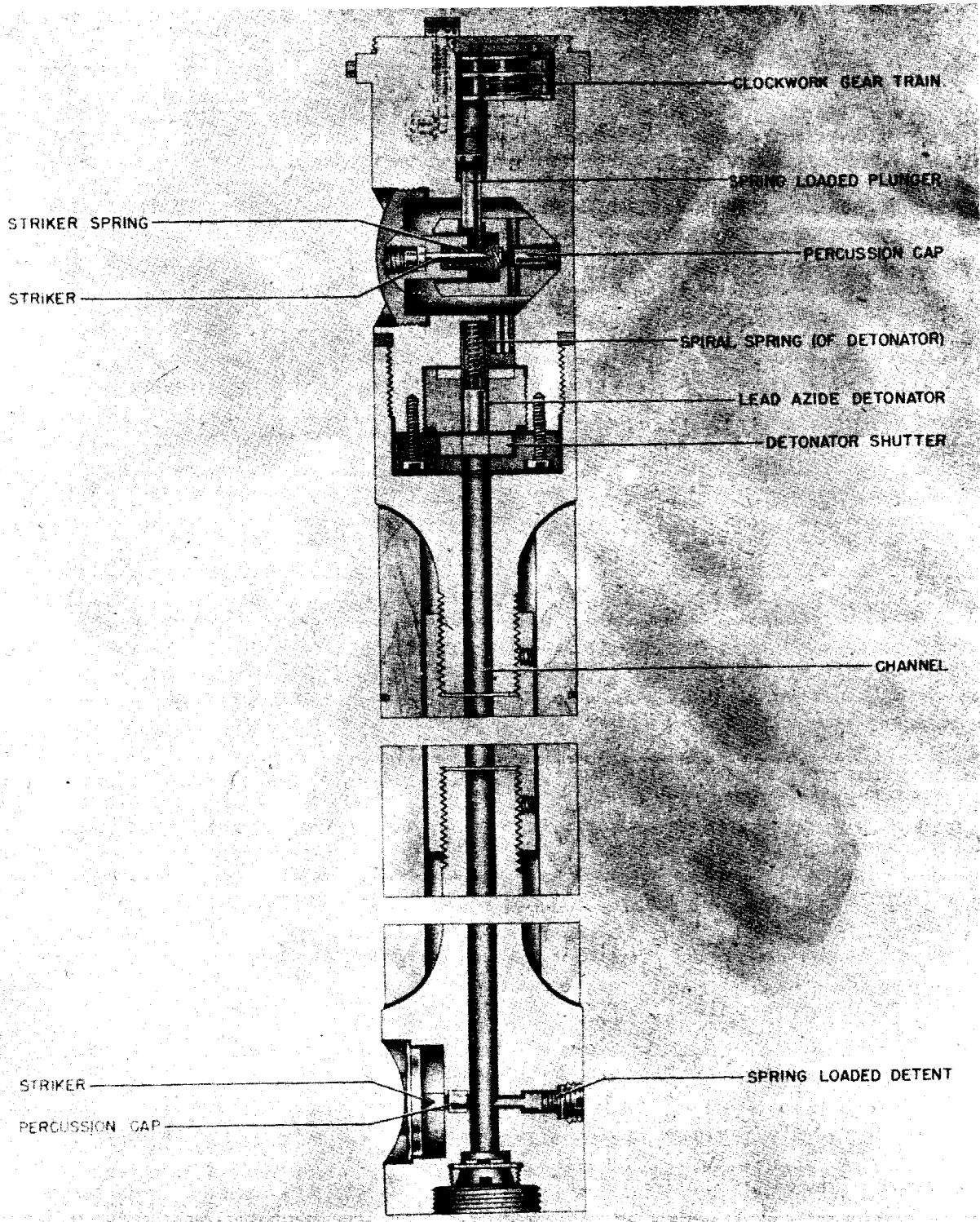
Figure 135—(24) Mechanical Antibreak-up Fuze
