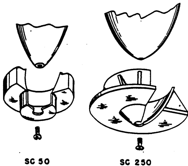
Figure 6—Antiricochet Plates
