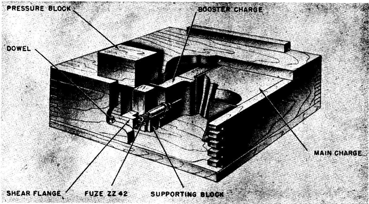
Figure 227—Holzmine 42 Antitank Mine
