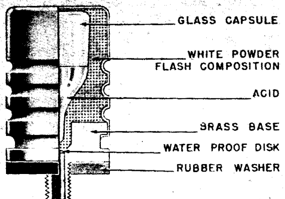
Figure 276—Buck Igniter—Chemical Pressure
