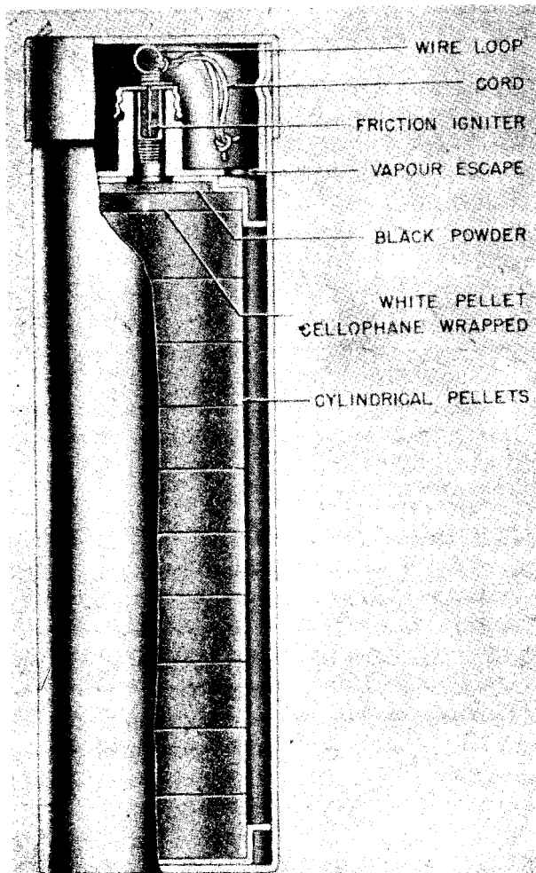
Figure 297—Lachrymatory Hand Grenade
