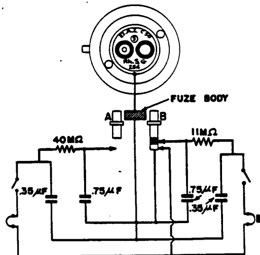
Figure 138—(5) Electrical Impact Fuze
