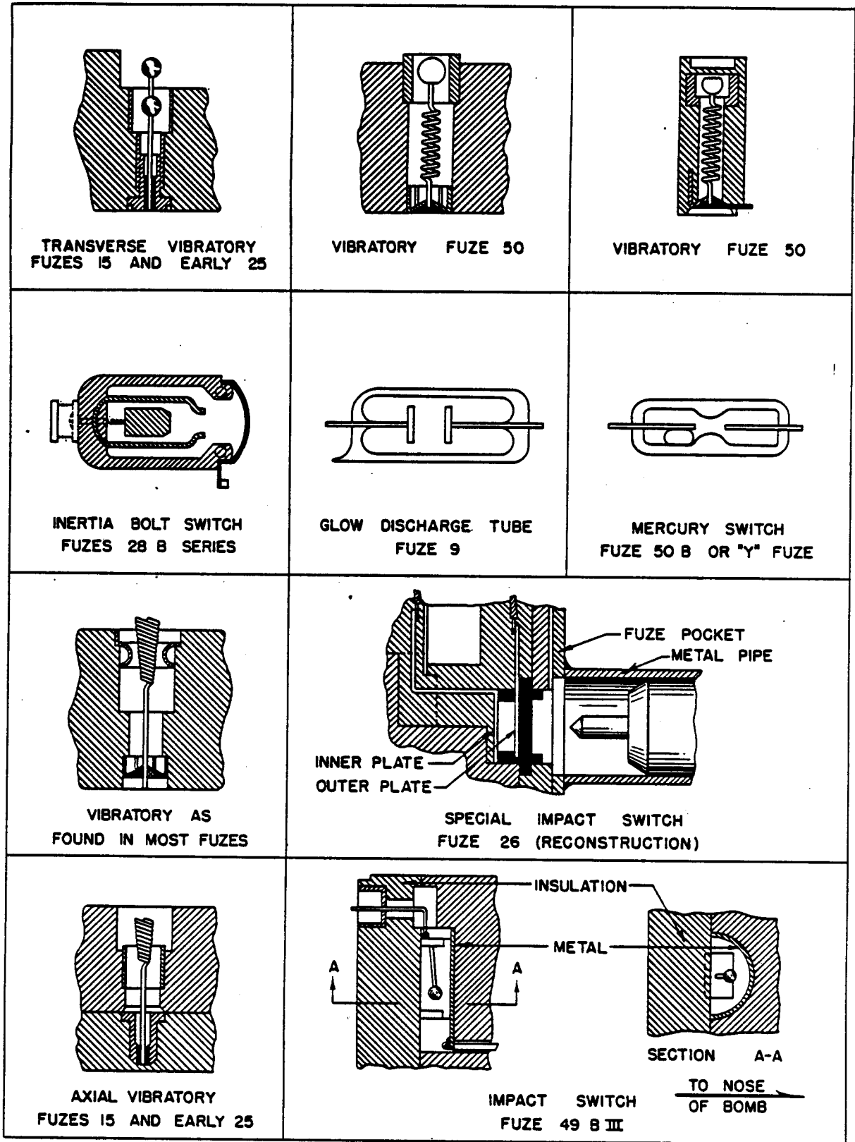
Figure 122—Types of Trembler Switches
