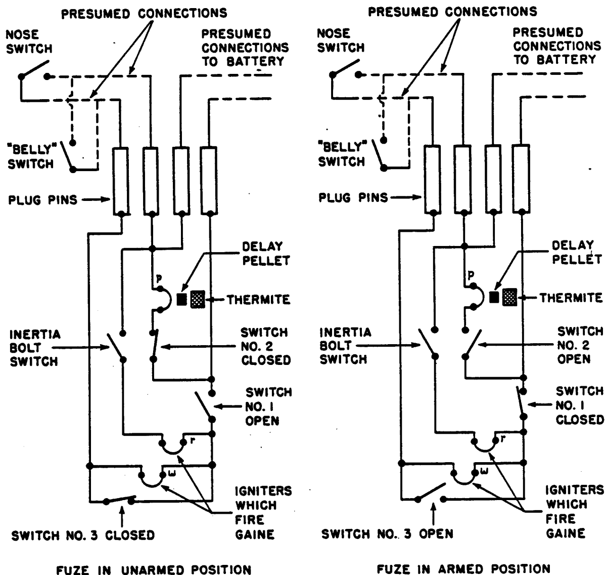
Figure 151B—(106)* Electrical Impact Fuze Wiring Diagram
