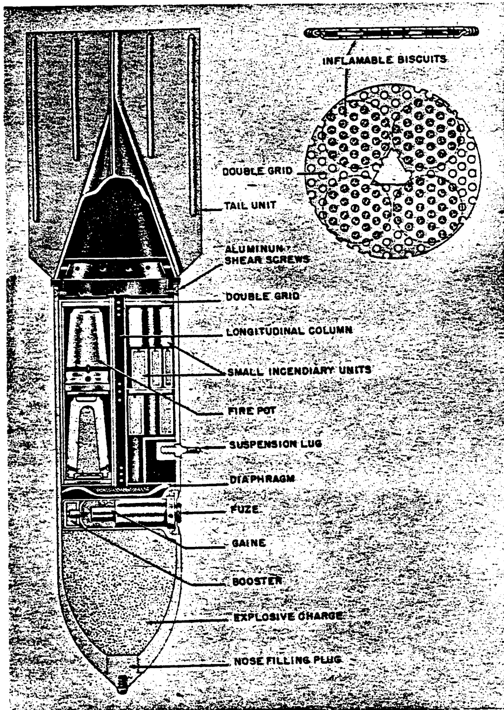
Figure 54—Sprengbrand C 50 Bomb
