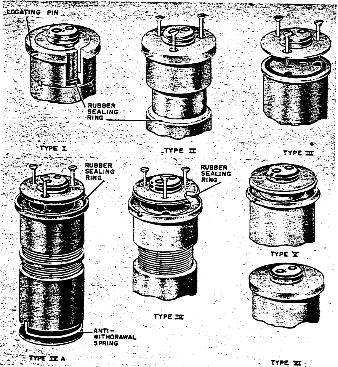
Figure 119—Types of Fuze Construction
