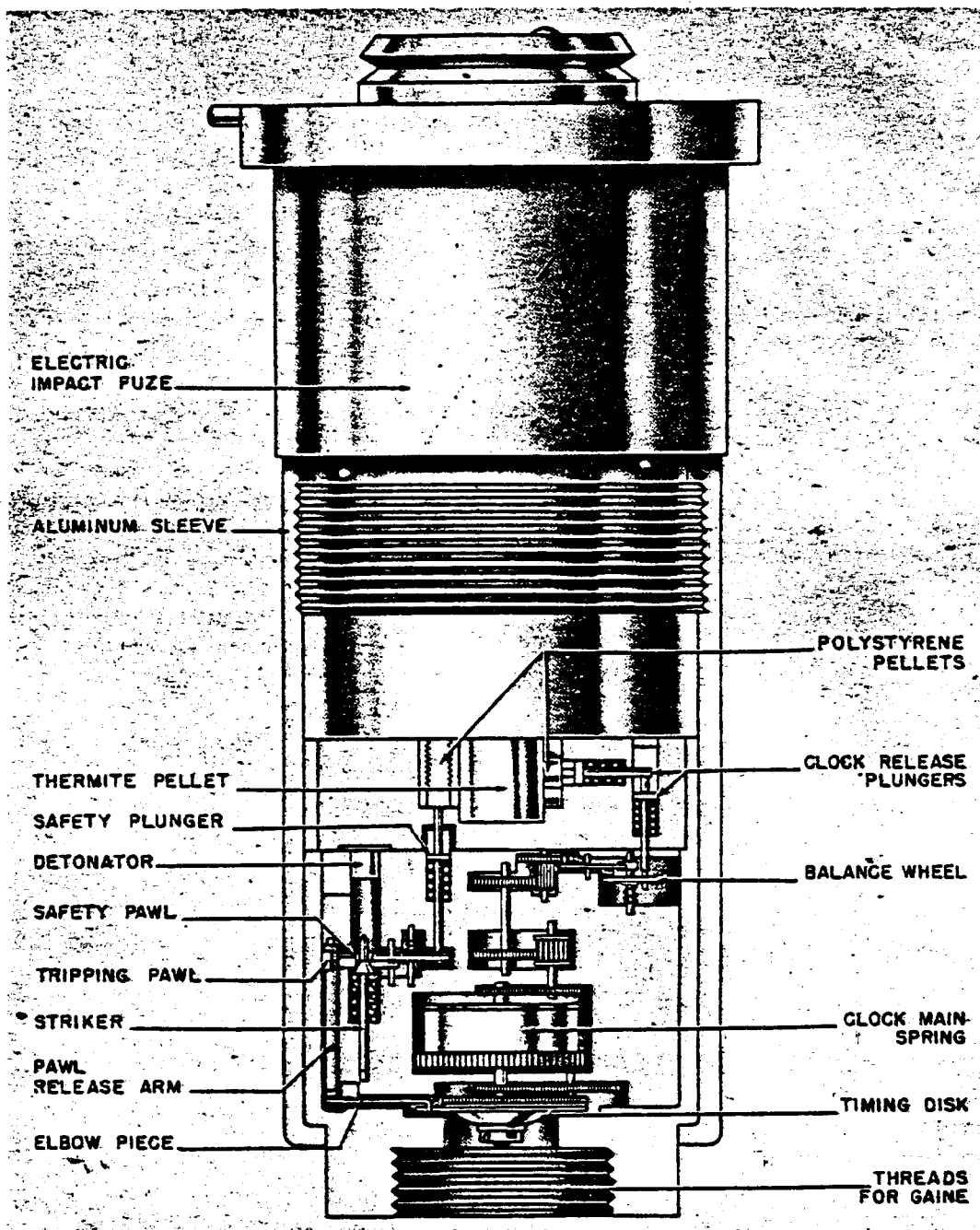
Figure 153A—(17)A Electrical Clockwork Time Fuze
