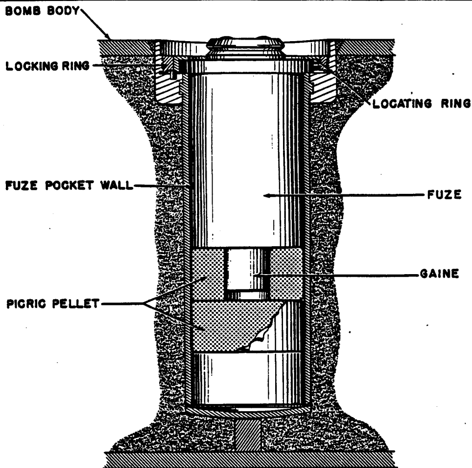
Figure 3—Fuze Pocket in Bomb
