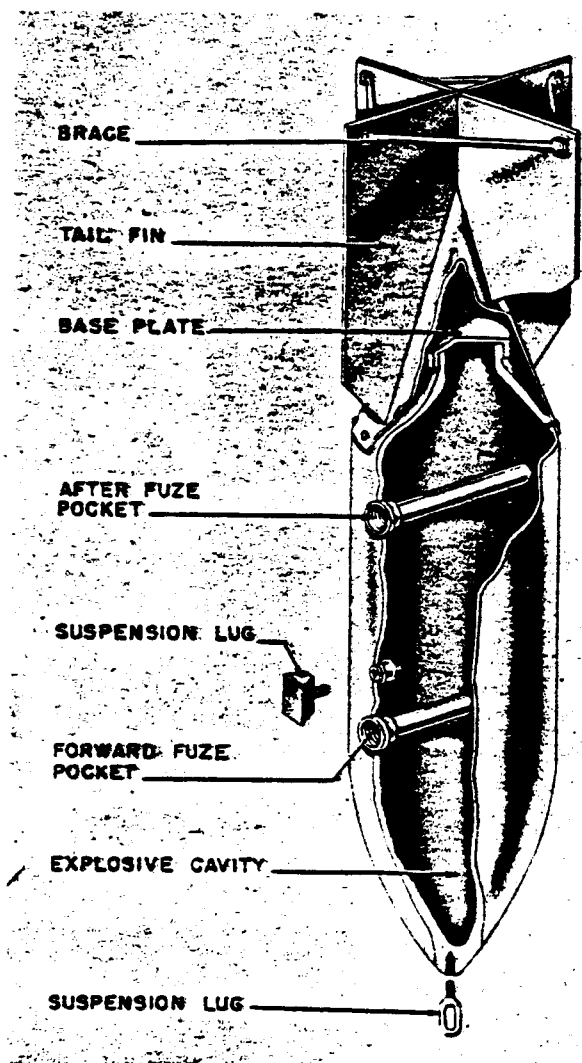
Figure 12—SC 250 Bomb; types 1, 2, and 3
