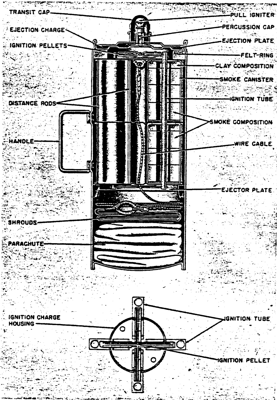
Figure 92—Parachute Recognition Smoke Generator
