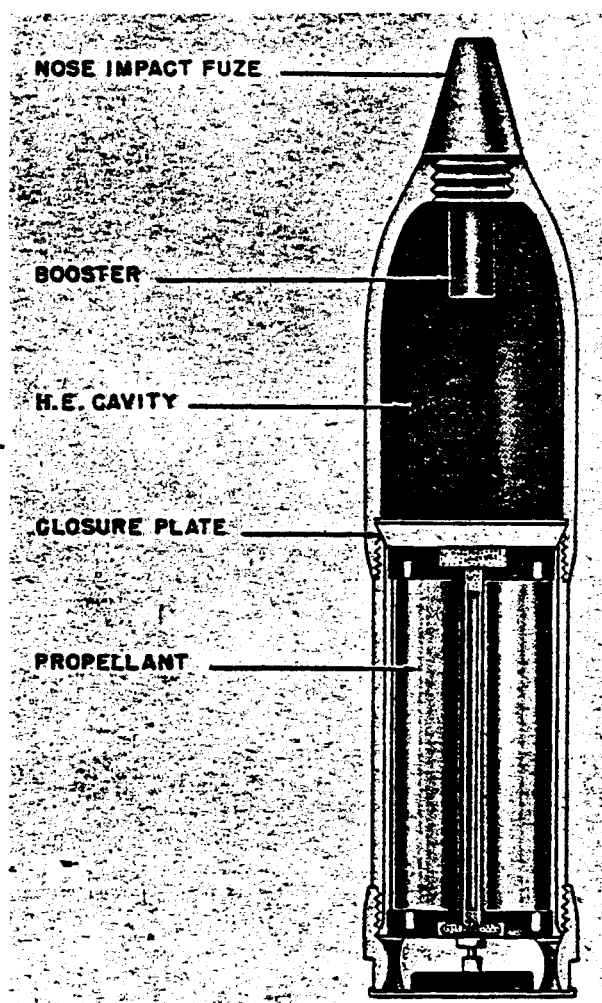
Figure 222—8.6-cm R. Spgr L/4.5 Rocket
