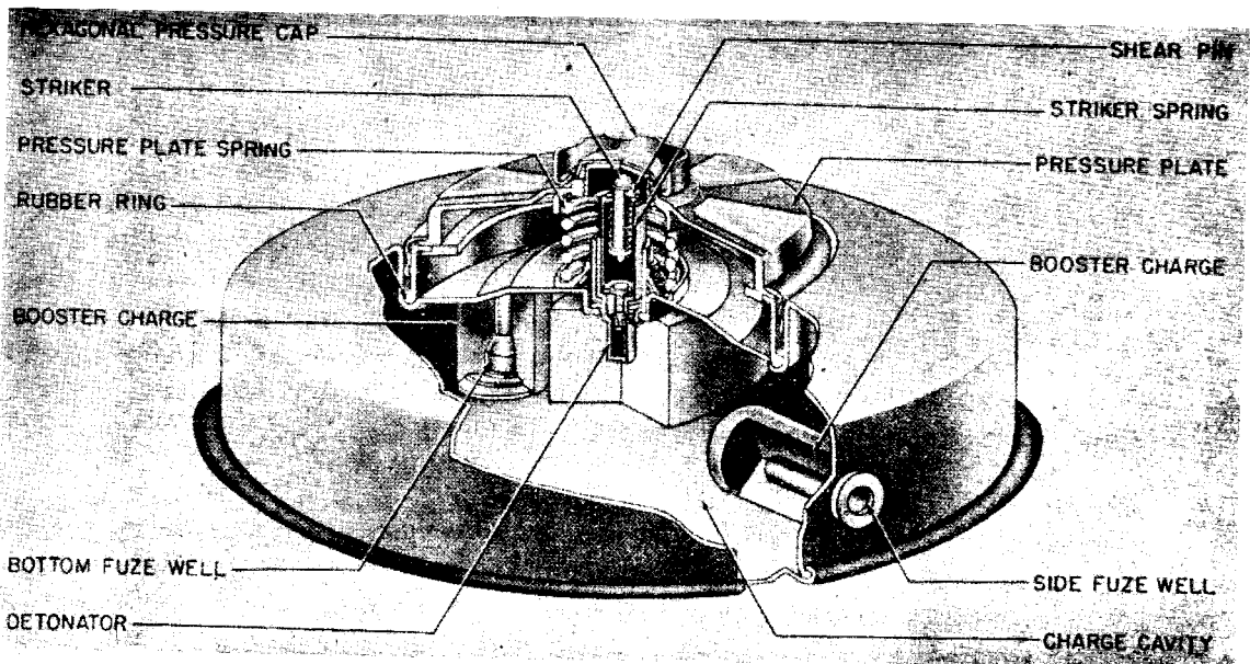
Figure 232—Tellermine 42—Antitank
