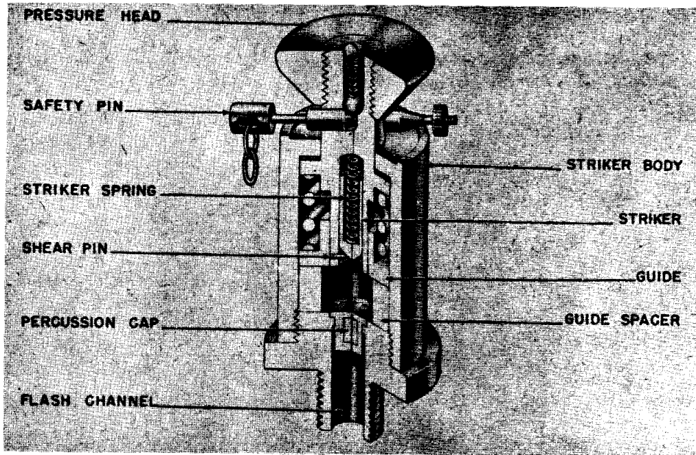
Figure 263—D. Z. 35 (B) Pressure Igniter
