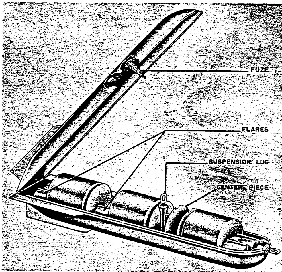
Figure 102—AB 70-1 Container
