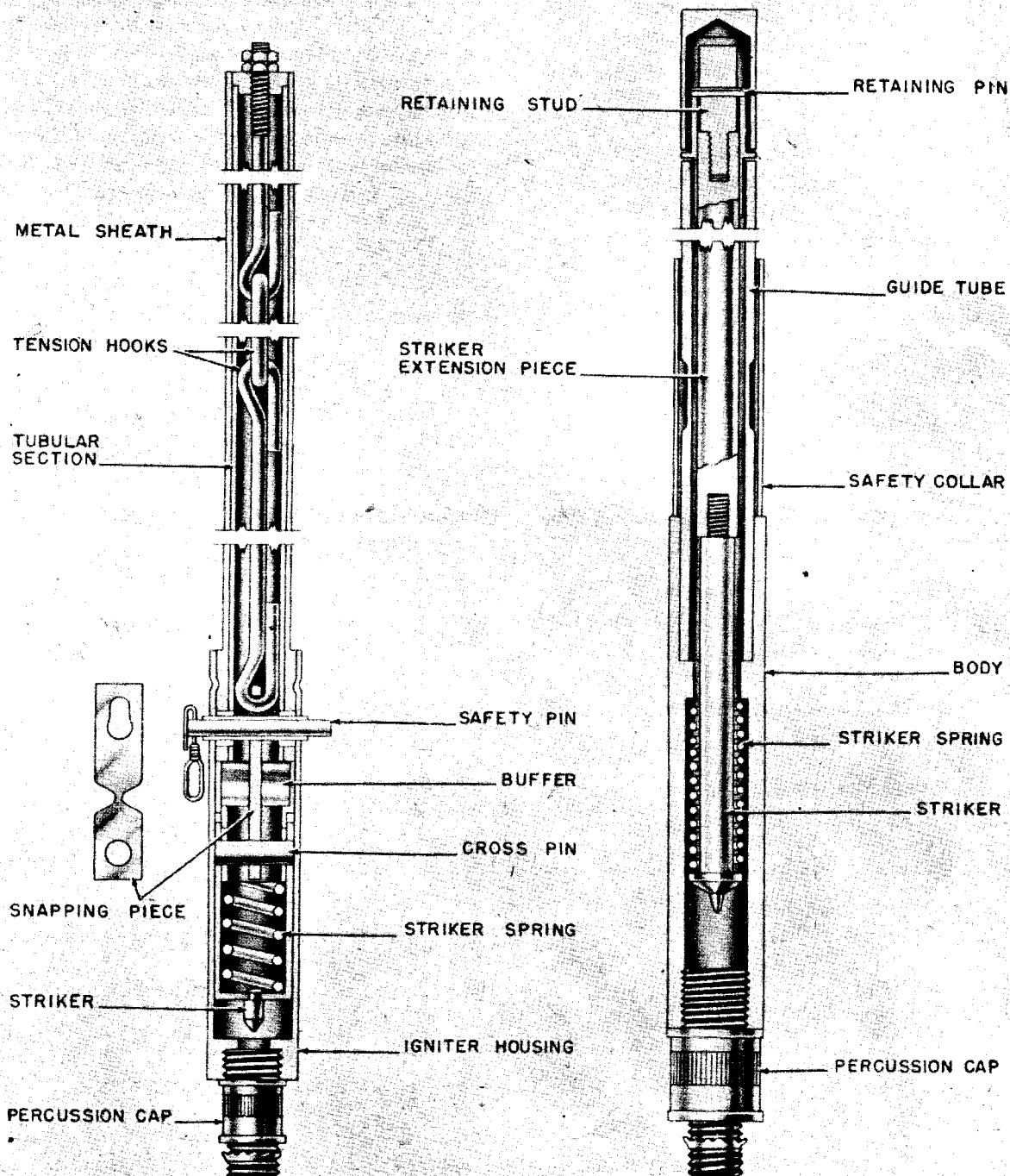
Figure 282—Knickzunder 43, Types I and II, Snap Type
