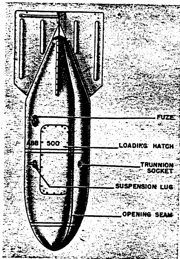
Figure 114—ABB 500 Container
