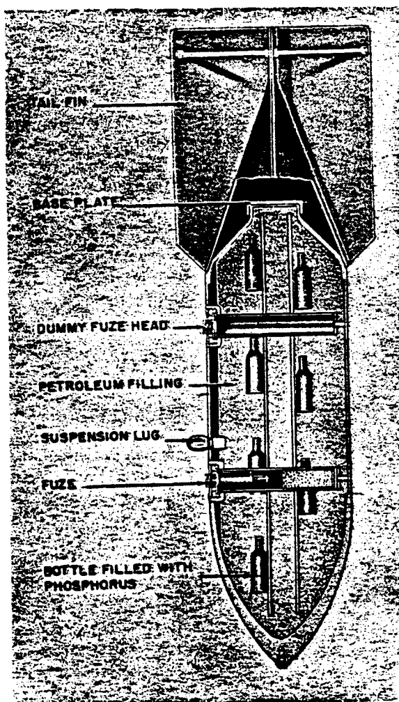
Figure 60—Brand C 250 A Bomb, Types I and II
