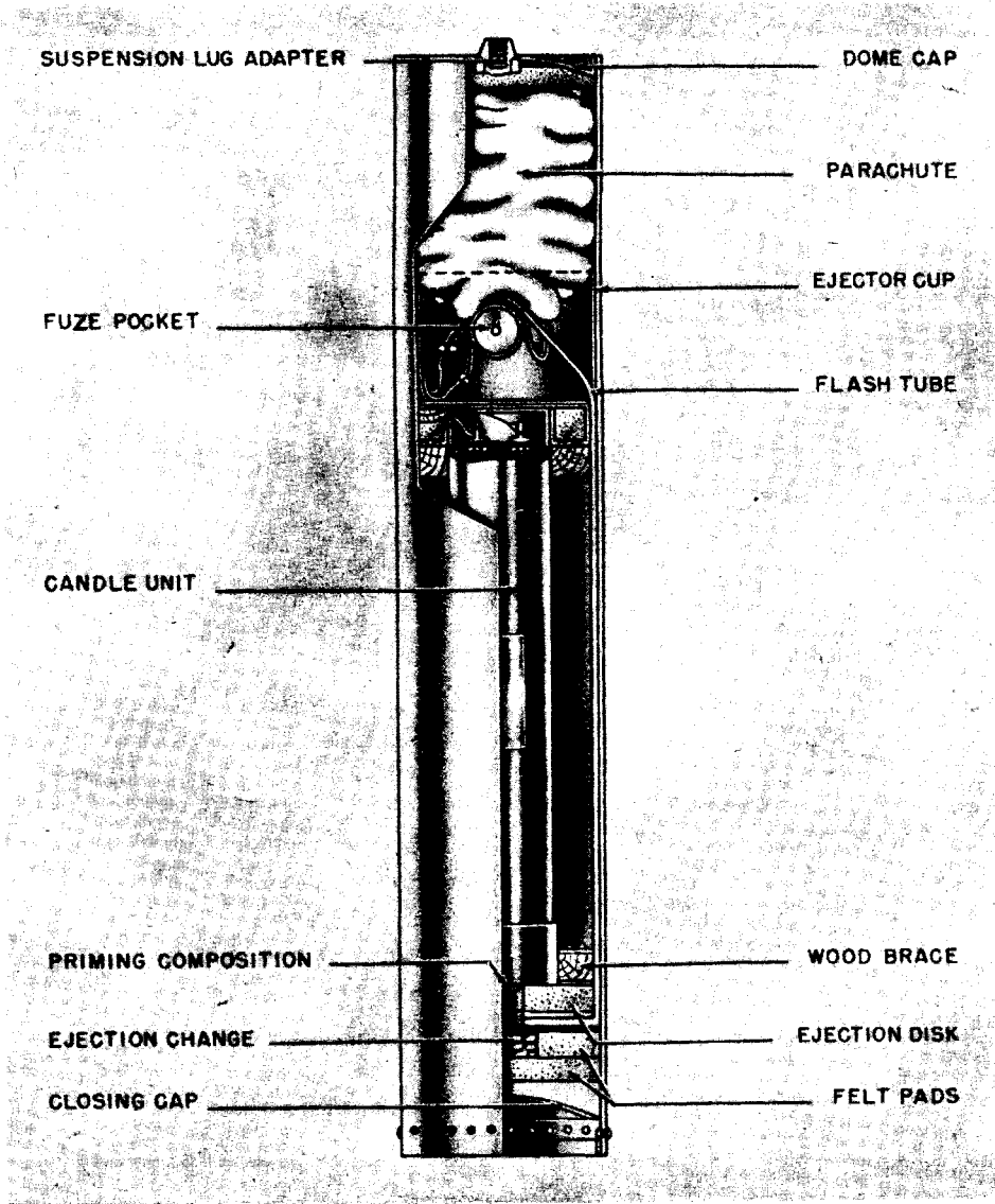
Figure 75—Mark C 50 FA Parachute Flare
