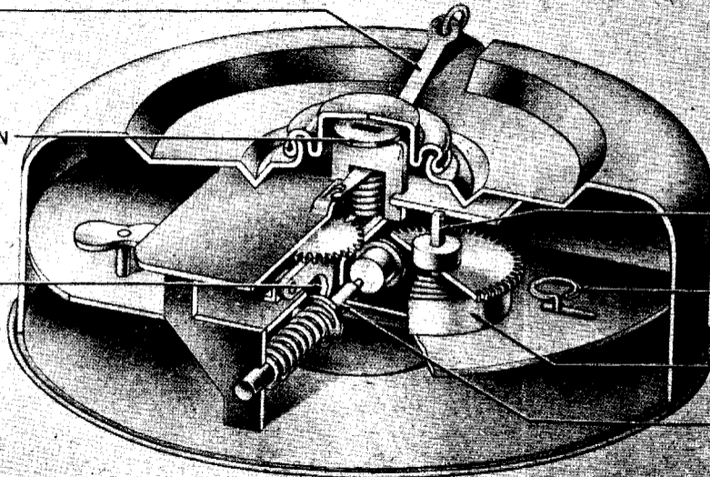
Figure 283—E. Z. 44 Antilifting Device
