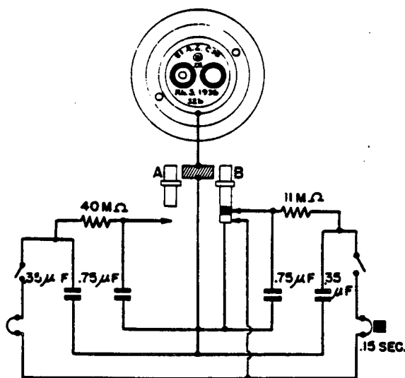
Figure 159—(28)* Electrical Impact Fuze
