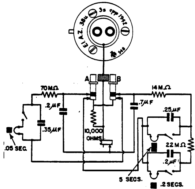
Figure 167—(38 u) Electrical Impact Fuze
