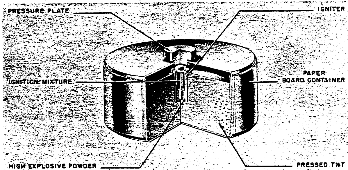
Figure 224—Pappmine Antitank Mine
