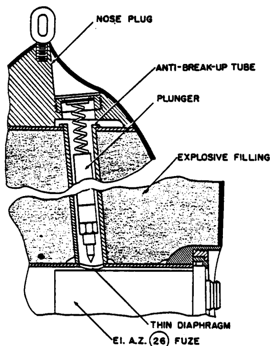
Figure 147A—(26) Electrical Impact (Special)
