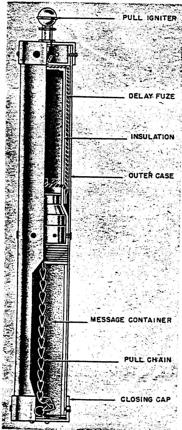
Figure 117—Message Tube (sea)
