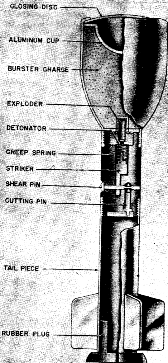
Figure 305—Schuss Gg. P-40 Hollow Charge Rifle Grenade
