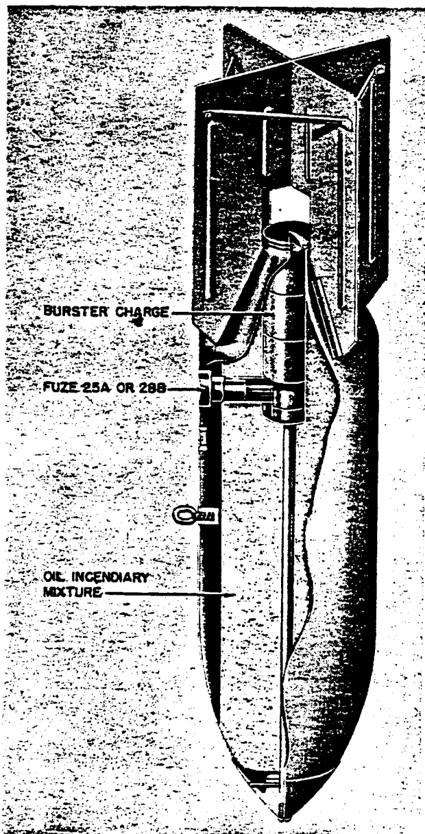
Figure 55—Flam C 250 A Bomb
