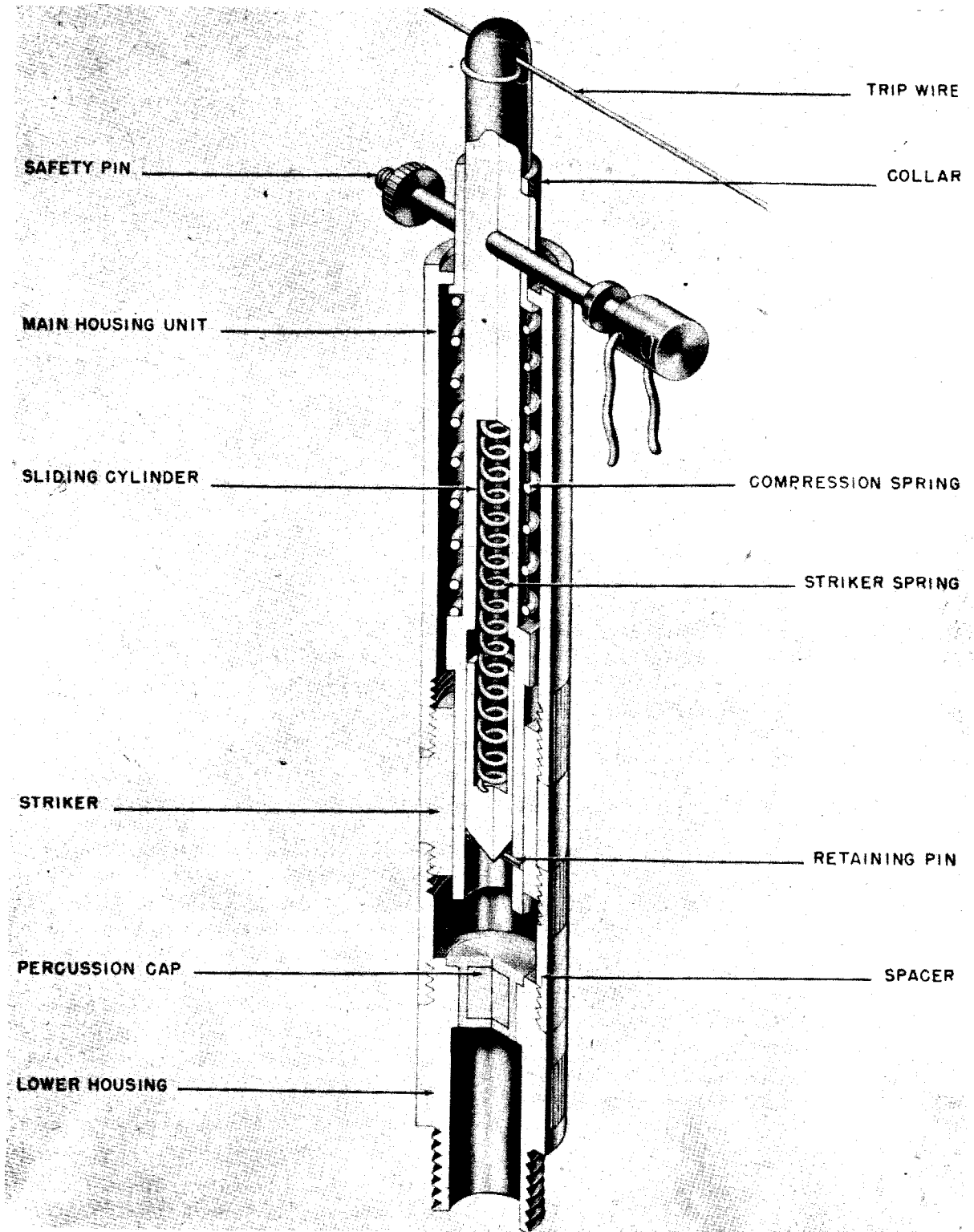
Figure 258—Z. U. Z. 35 Pull and Tension Release Igniter
