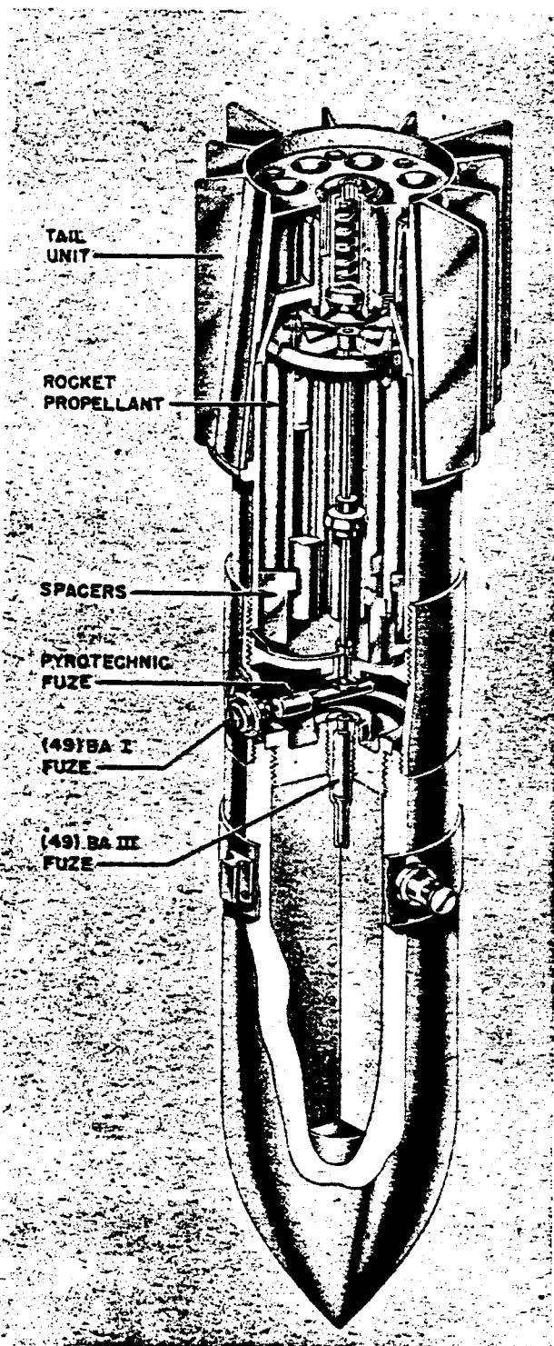
Figure 34—PC 1000 RS Bomb
