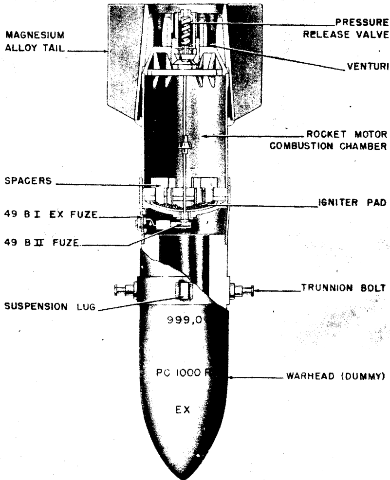
Figure 68—PC 1000 RS EX Practice Bomb
