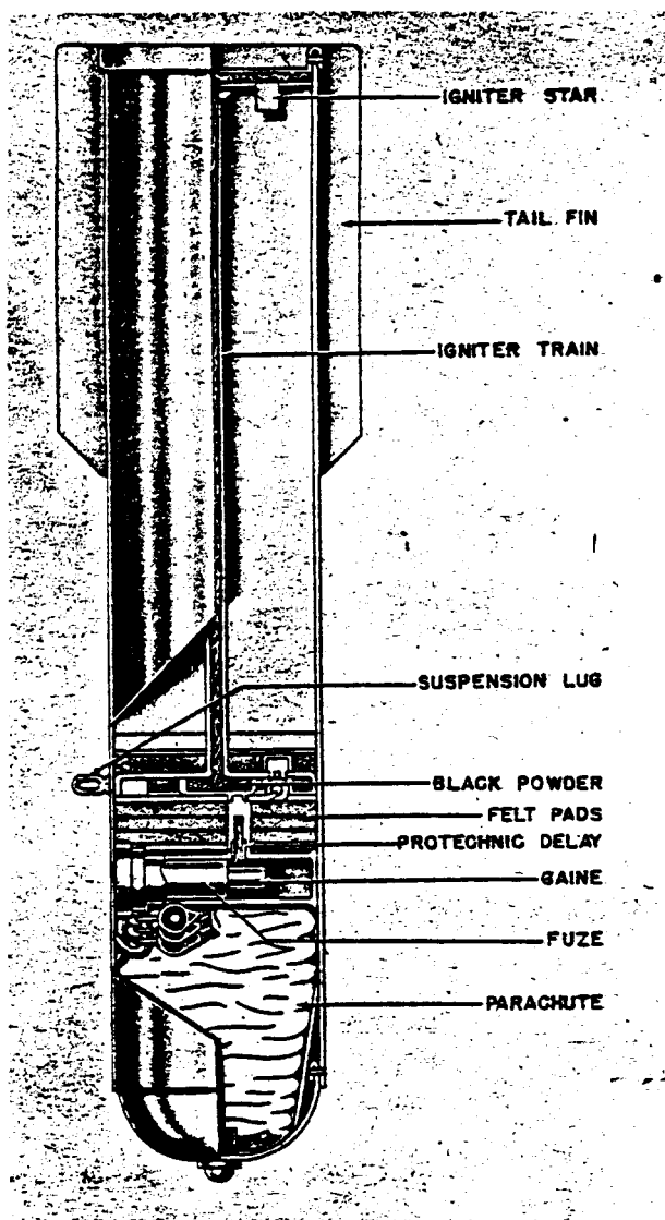
Figure 74—LC 50 F Ausf. G Parachute Flare
