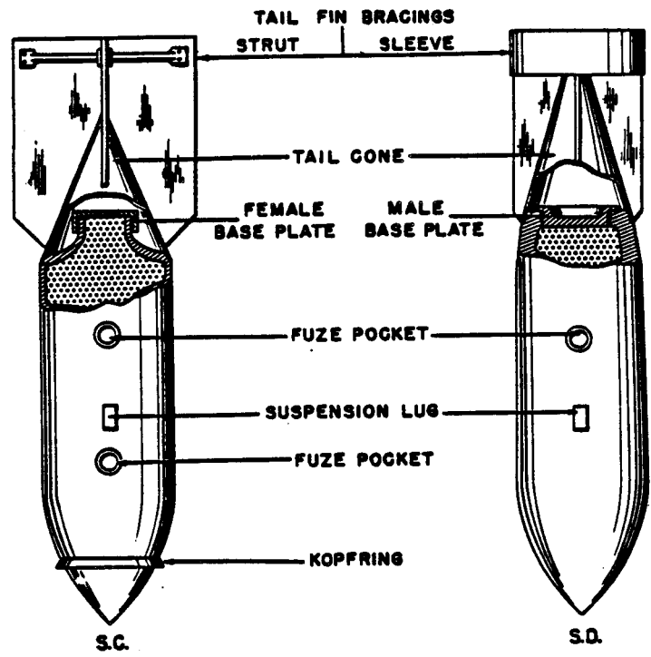
Figure 1—Bomb Component Positions
