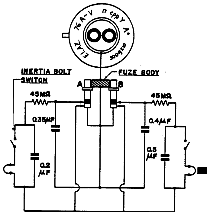
Figure 150—(76)A Electrical Impact Fuze
