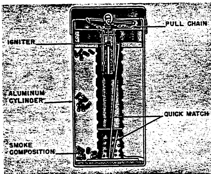
Figure 82—Smoke Flare, Orange, 80
