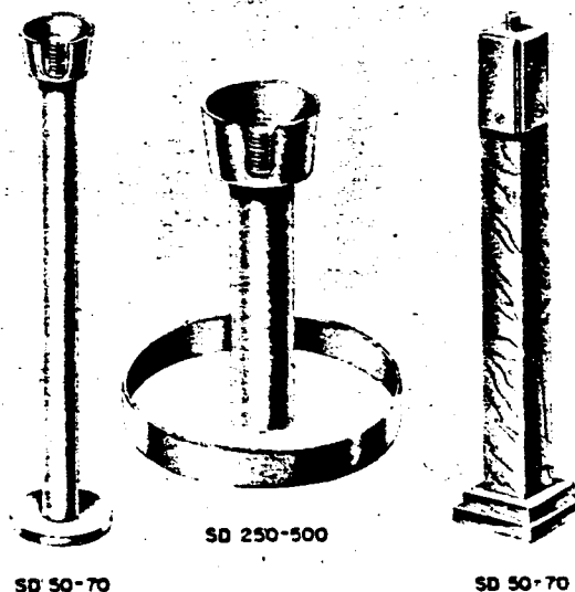
Figure 7—Dinort Rods
