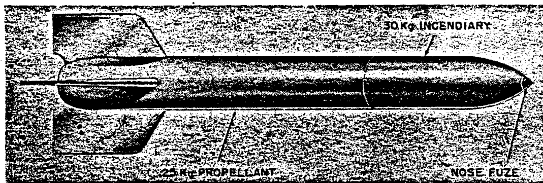
Figure 220—R 100 BS Rocket
