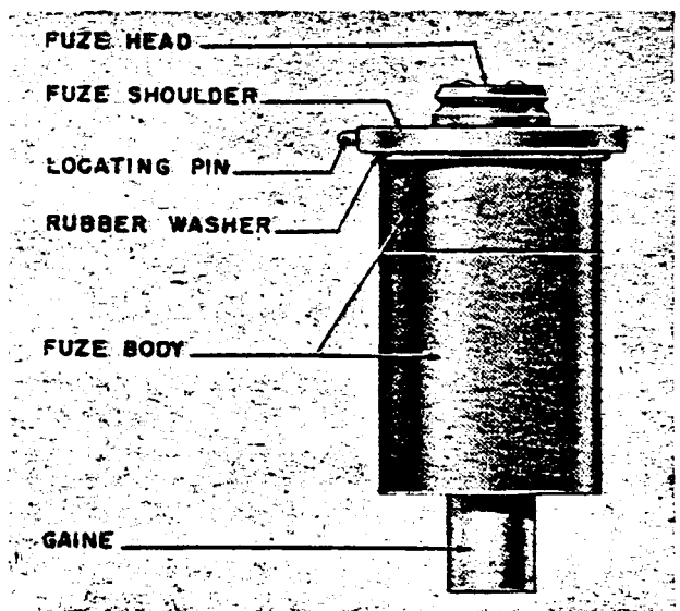
Figure 120—Typical Electrical Bomb Fuze
