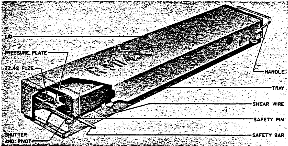
Figure 236—R Mine 43—Antitank
