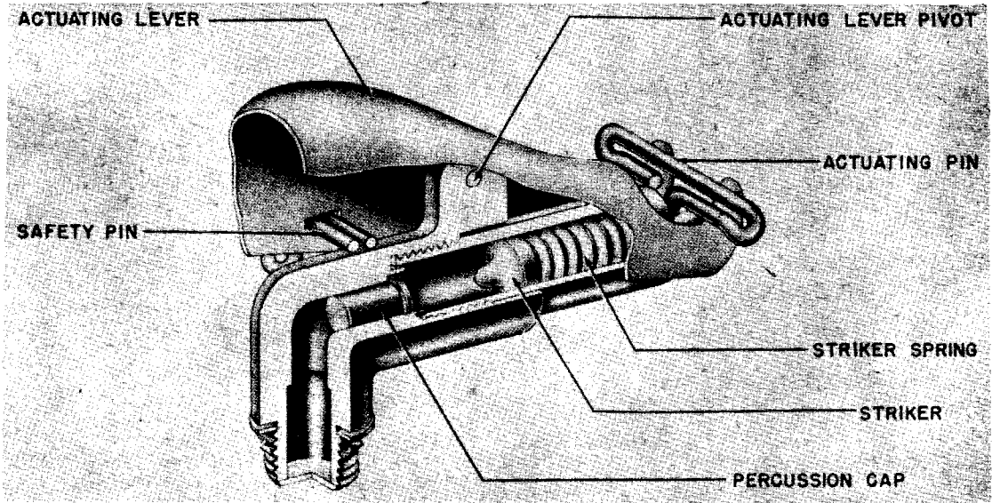
Figure 264—Schuko Pressure Igniter
