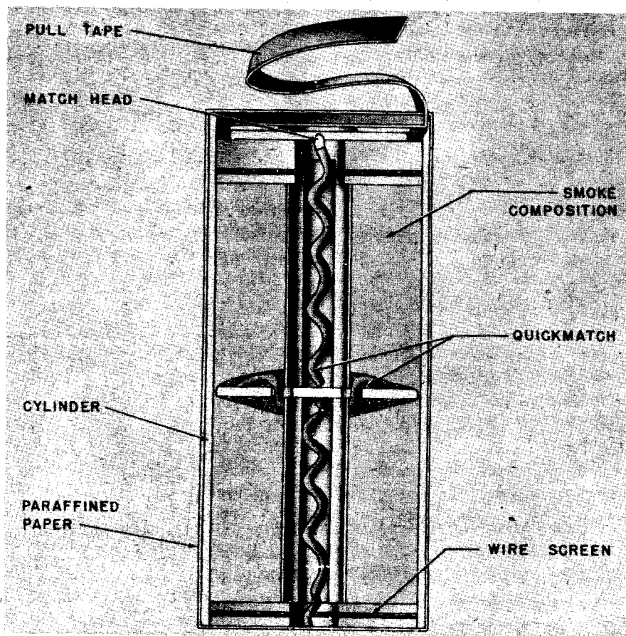
Figure 296—Red Smoke Signal Hand Grenade
