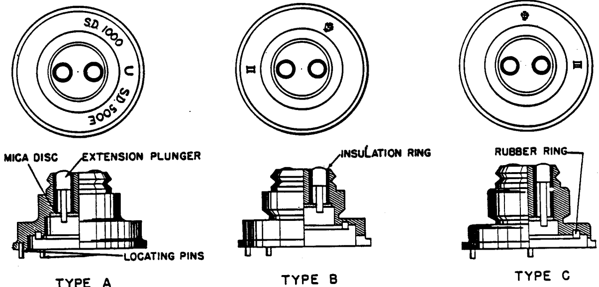
Figure 126—Extension Caps
