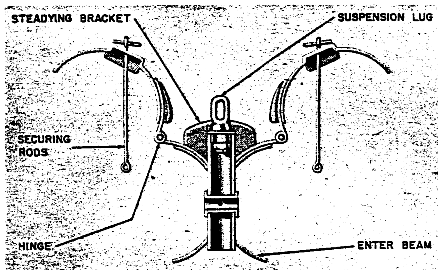
Figure 103C—AB 70-3 Container
