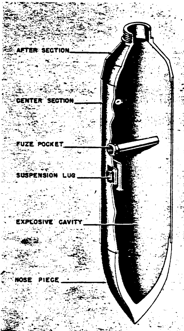
Figure 16—SC 1800-Kg Bomb
