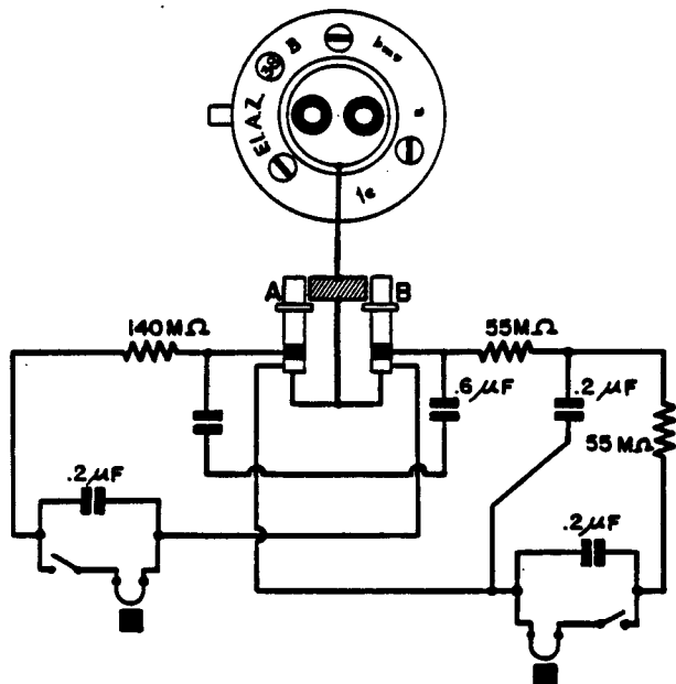
Figure 168—(38)B Electrical Impact Fuze
