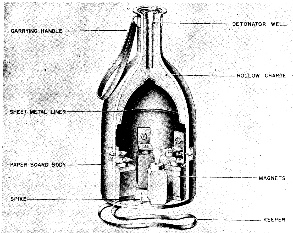
Figure 226—Panzerhandmine 3 Antitank Magnetic Charge Mine
