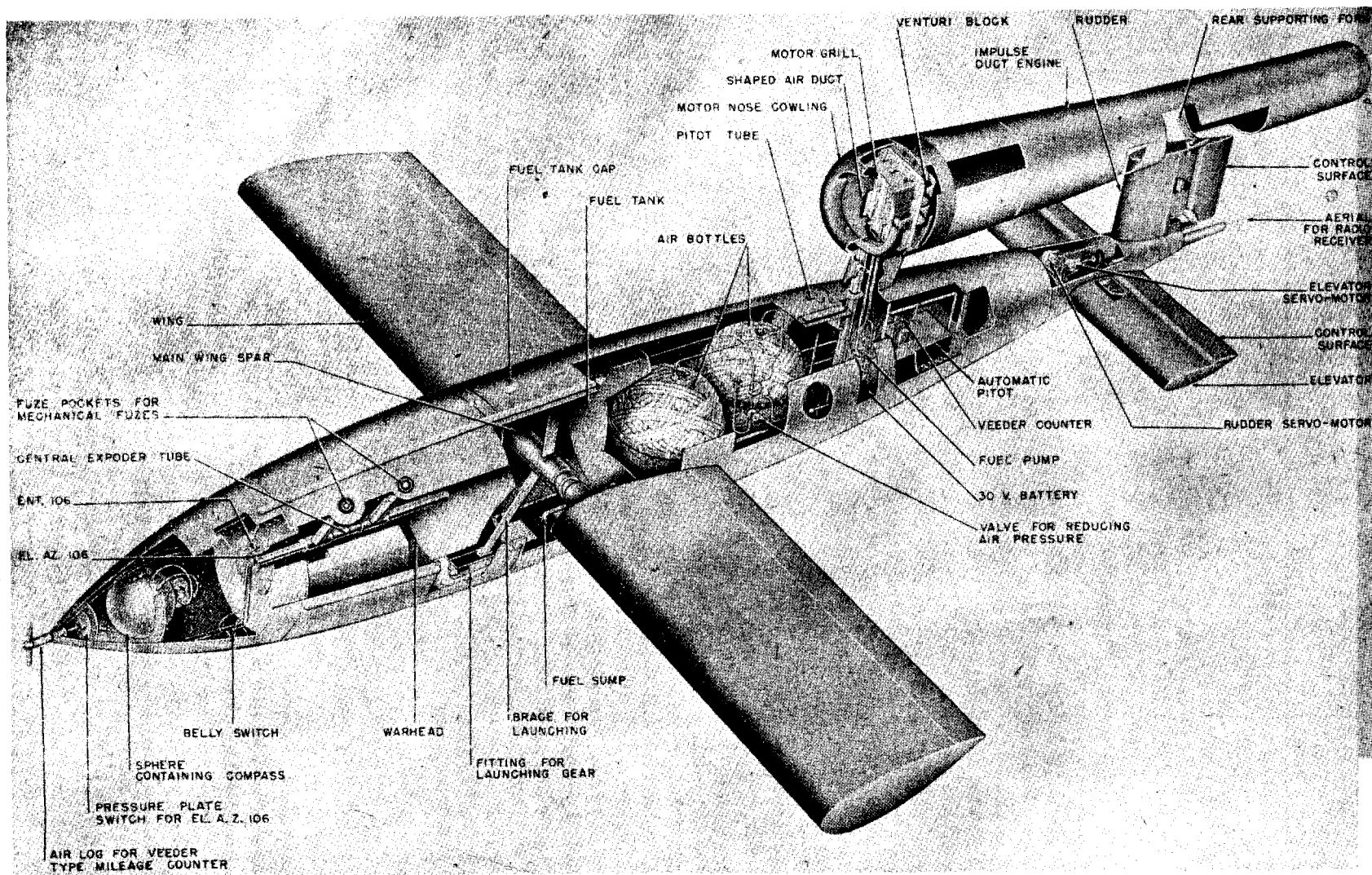
Figure 195—F. Z. G. 76 "V-1" Flying Bomb
