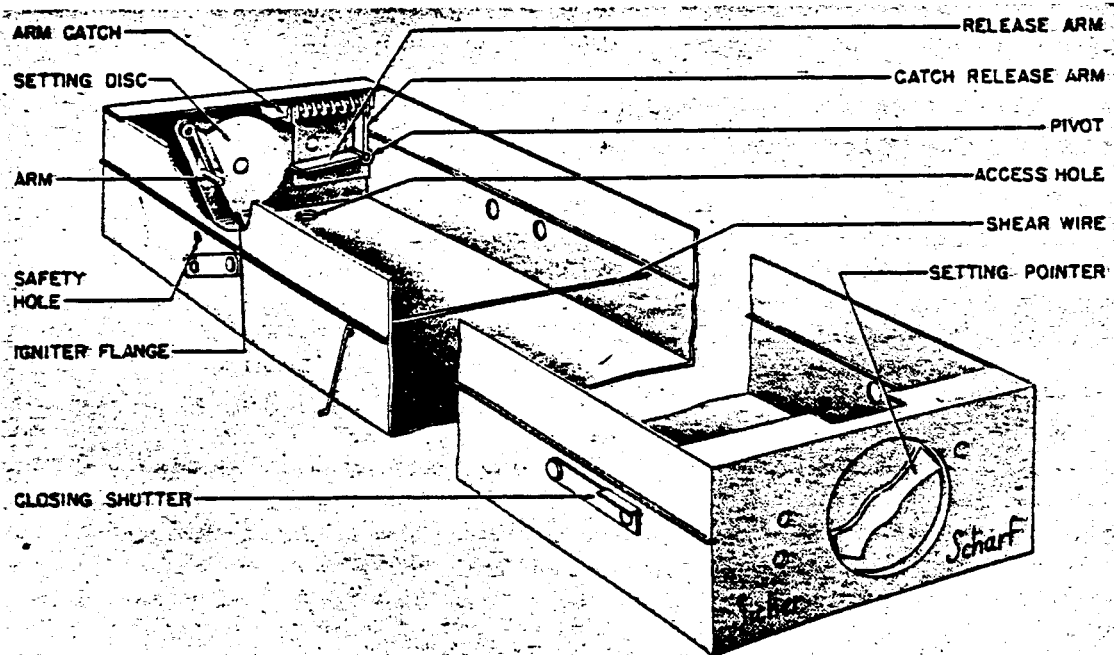
Figure 228—Spreng Riegel 8-Kg Antitank Mine
