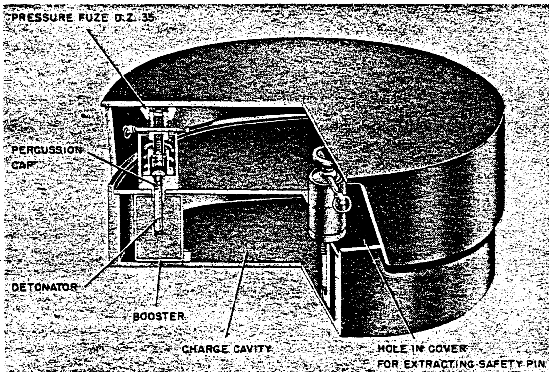
Figure 237—Aluminum Antitank or Antipersonnel Mine
