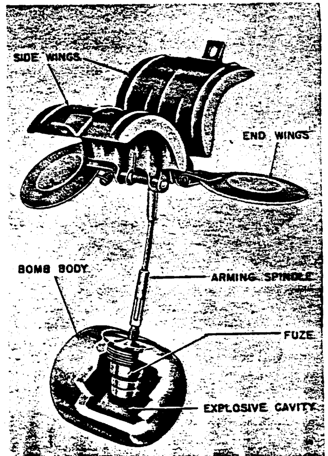
Figure 39B—SD 2-Kg "Butterfly" Bomb
