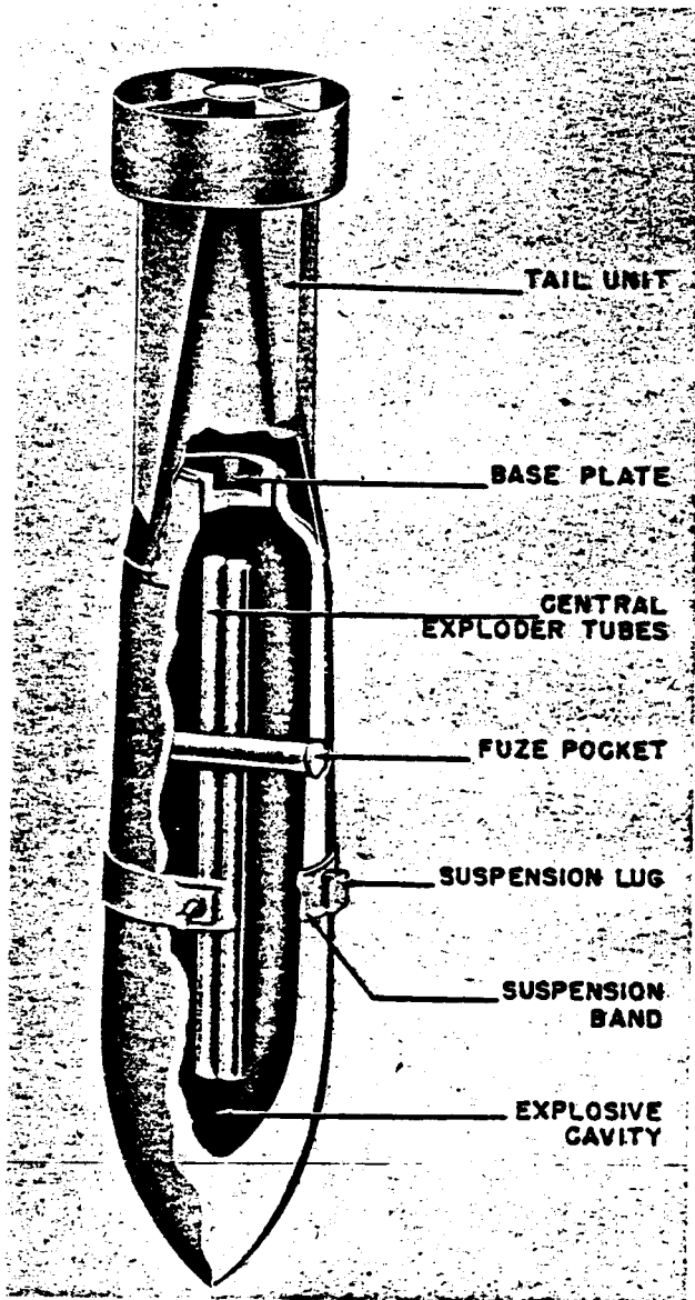
Figure 31—PC 1400-Kg Bomb
