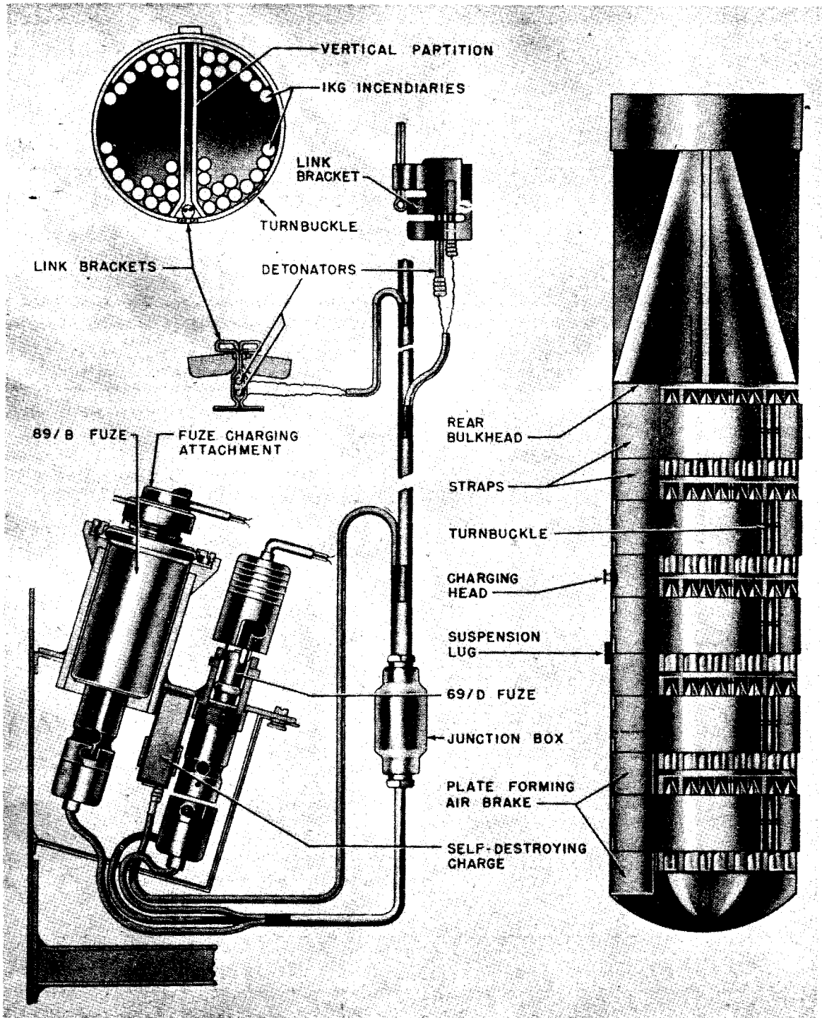
Figure 116—AB 1000-2 Container
