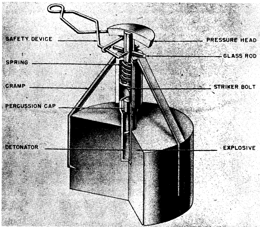
Figure 266—Weissman Pressure Igniter
