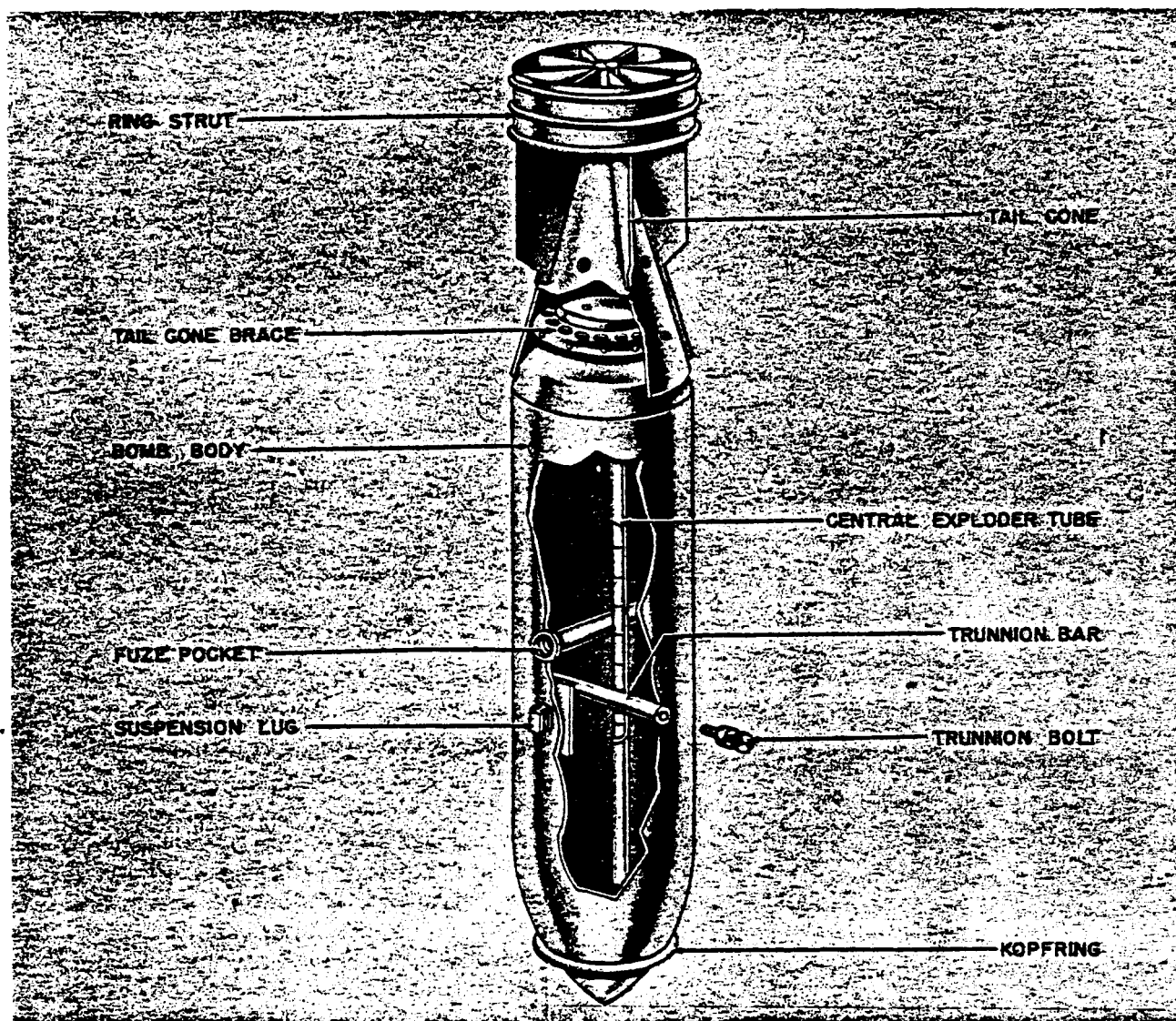
Figure 17—SC 2000-Kg Bomb
