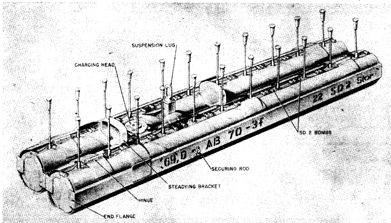
Figure 103A—AB 70-3 Container
