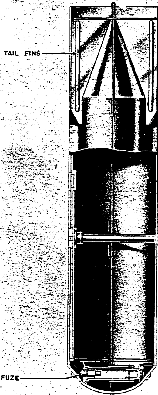
Figure 106—AB 250-2 Container
