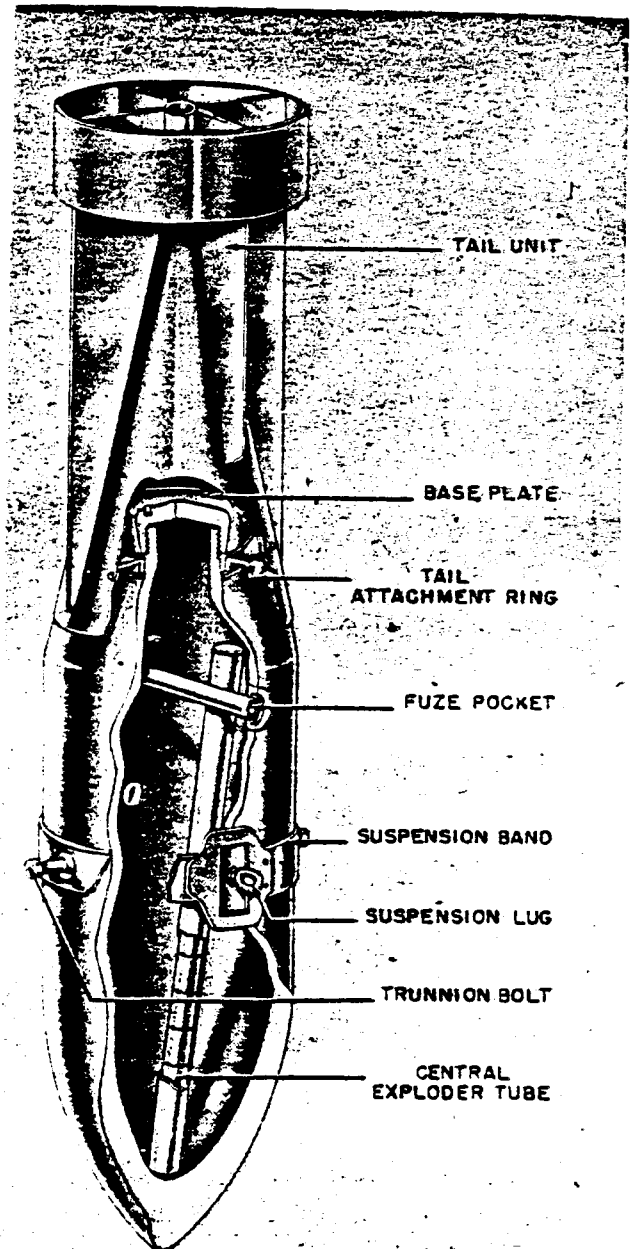
Figure 27—SD 500-Kg Bomb
