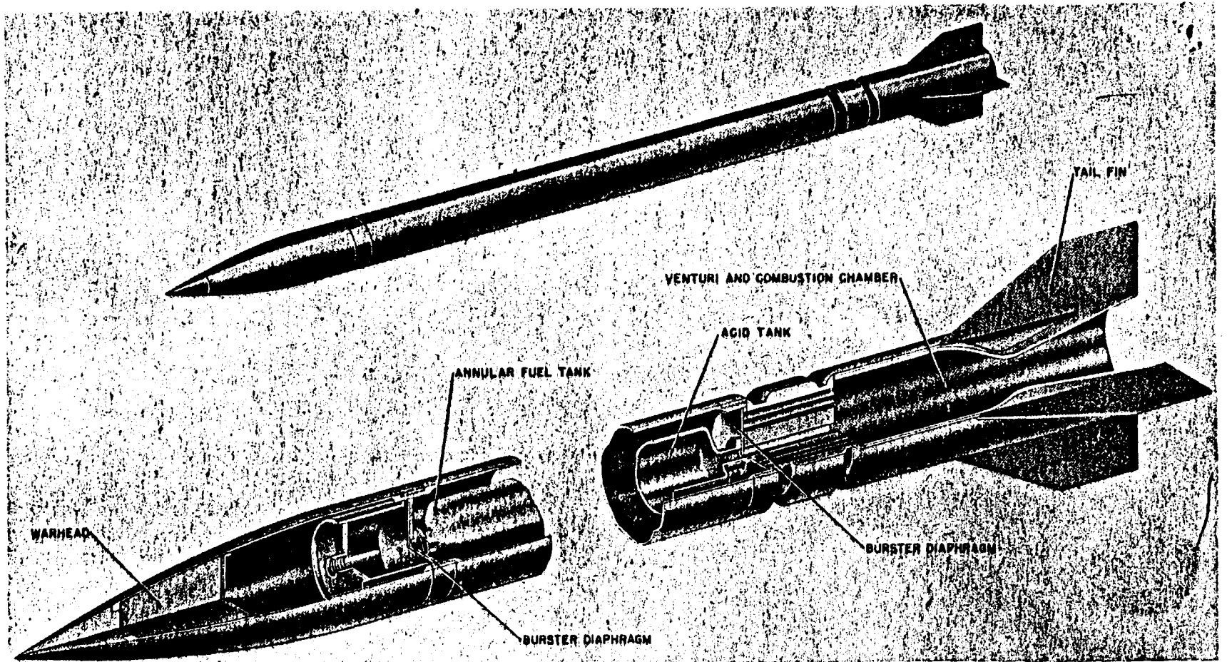
Figure 199—Taifun
