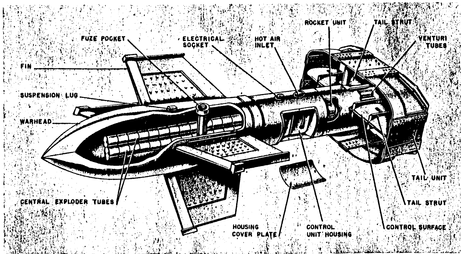
Figure 192—1400 FX
