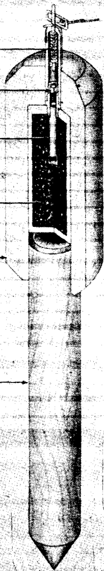
Figure 241—Stockmine—Antipersonnel
