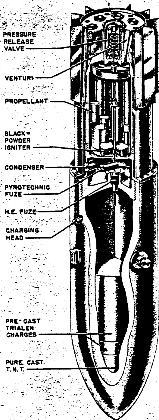
Figure 35—PC 1800 RS Bomb
