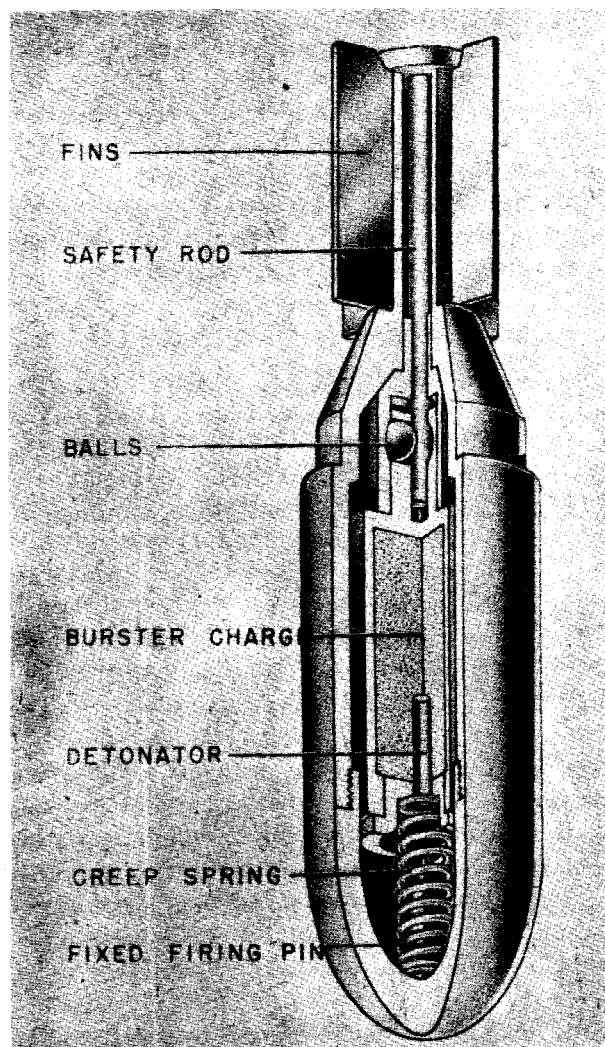
Figure 311—26-mm Pistol Grenade
