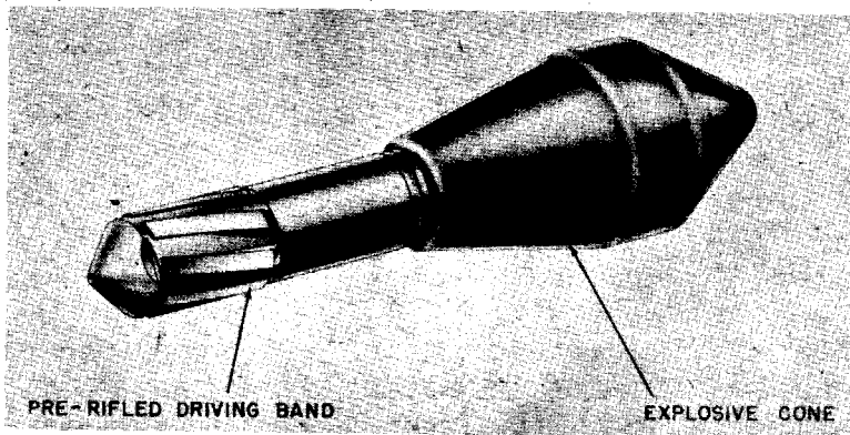
Figure 299—61-mm Hollow Charge Rifle Grenade
