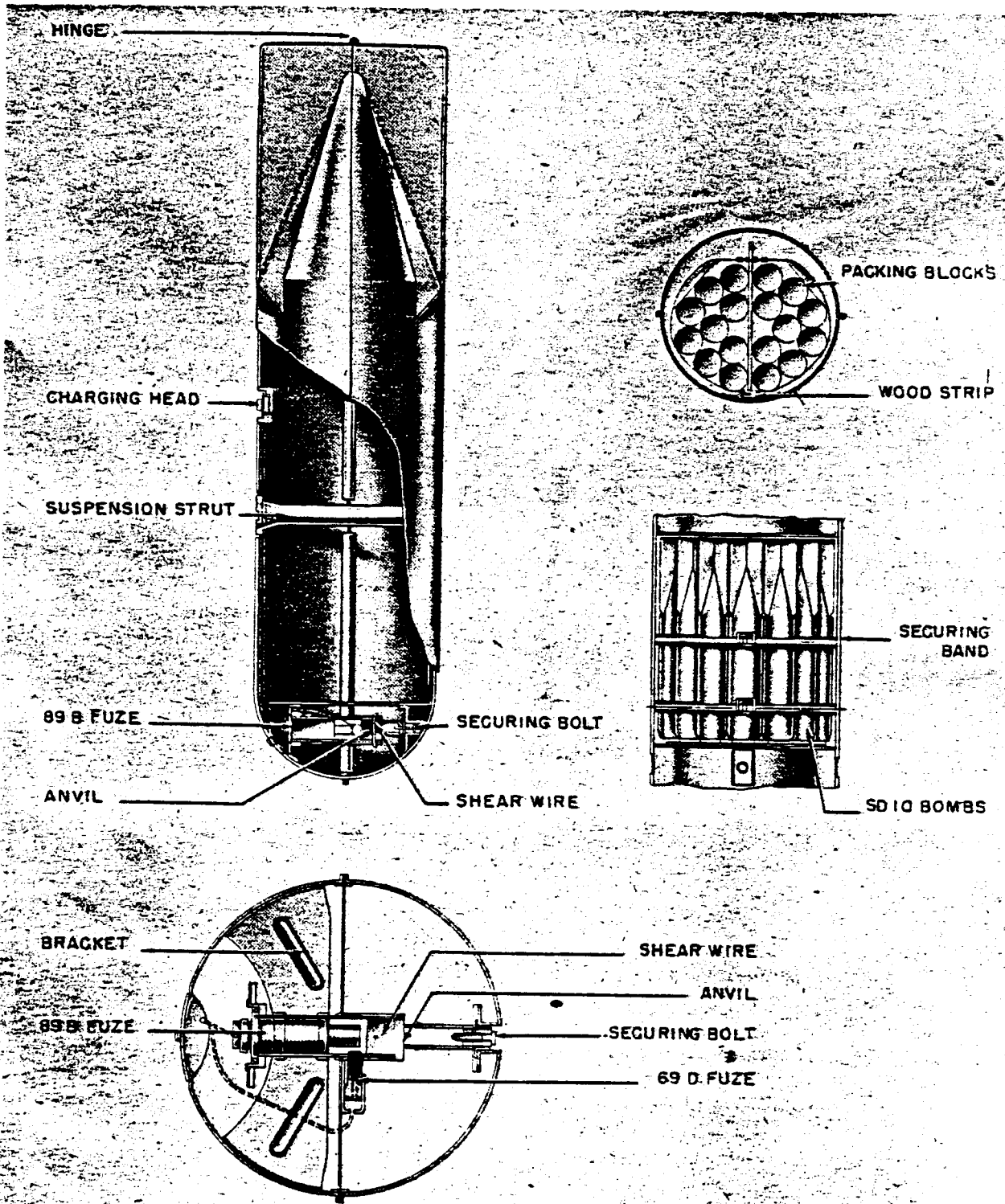
Figure 111—AB 500-1 Container
