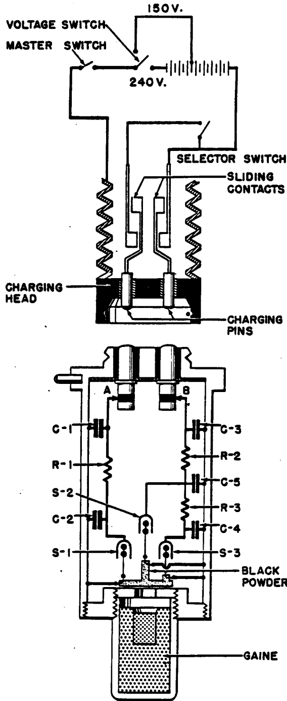
Figure 123—Wiring Diagram of Three Circuit Electrical Fuze
