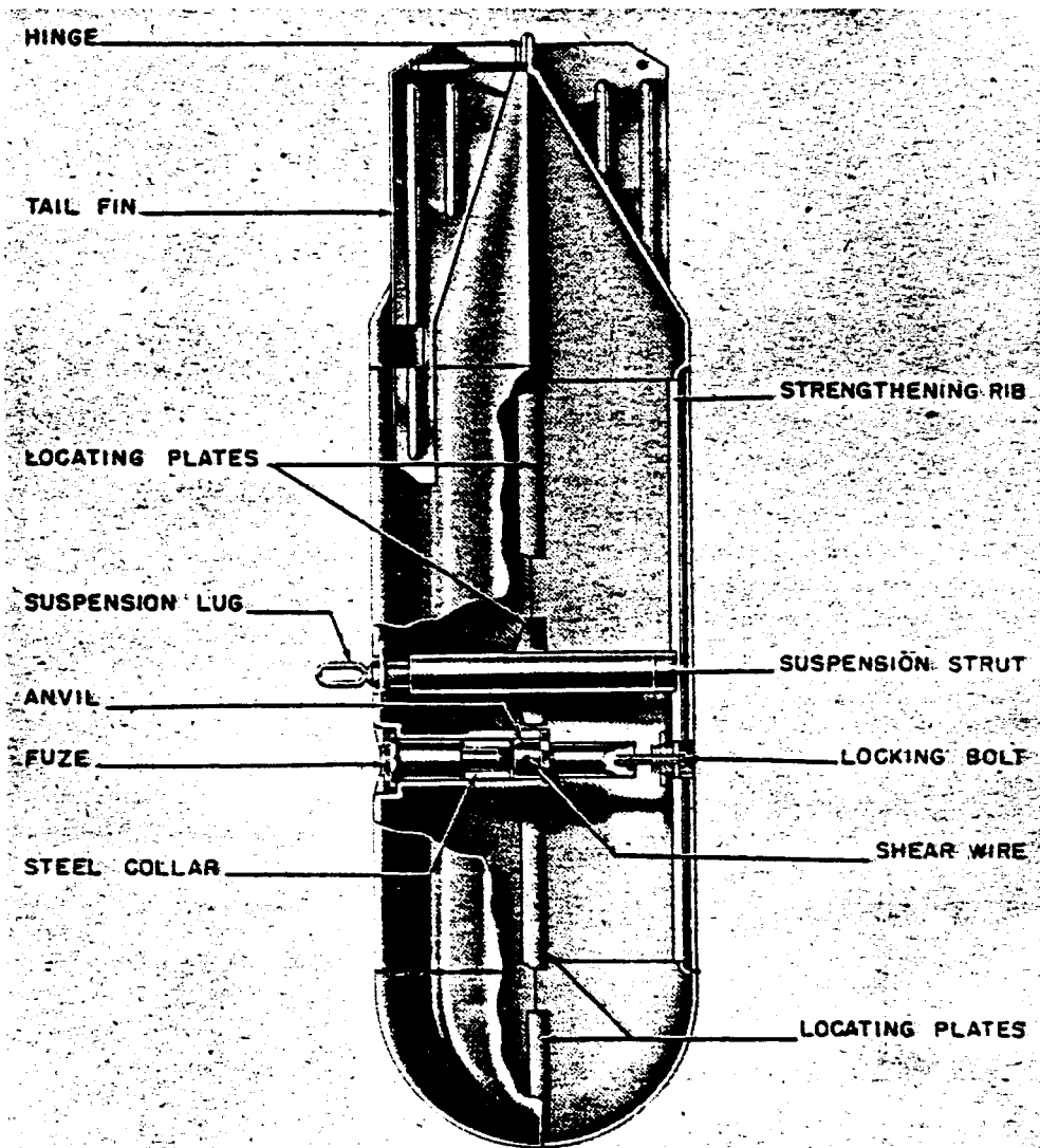
Figure 109—Mark 250 LK Container
