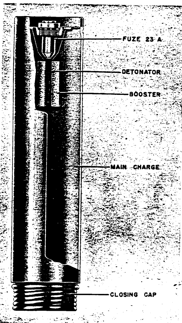
Figure 40—SB 3-Kg Bomb
