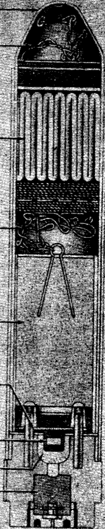
Figure 307—Illuminating Rifle Grenade
