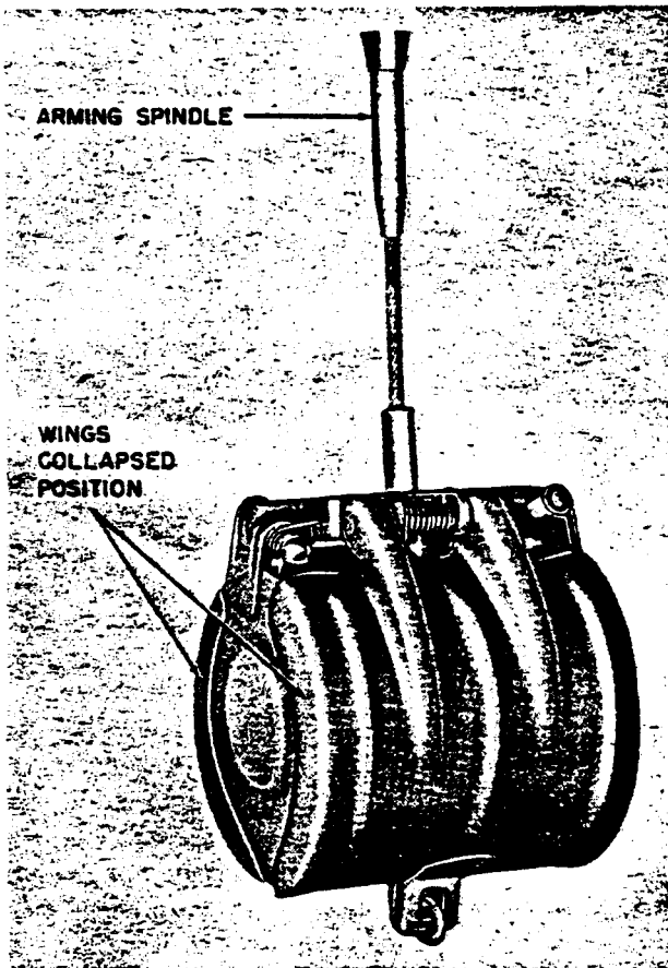
Figure 39A—SD 2-Kg "Butterfly" Bomb
