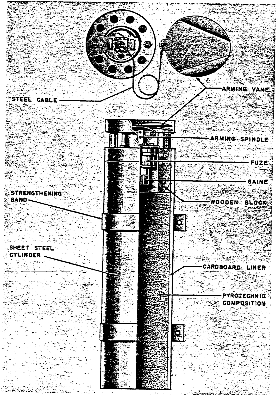
Figure 91—Mark 3 Single Unit Ground Marker (Green)
