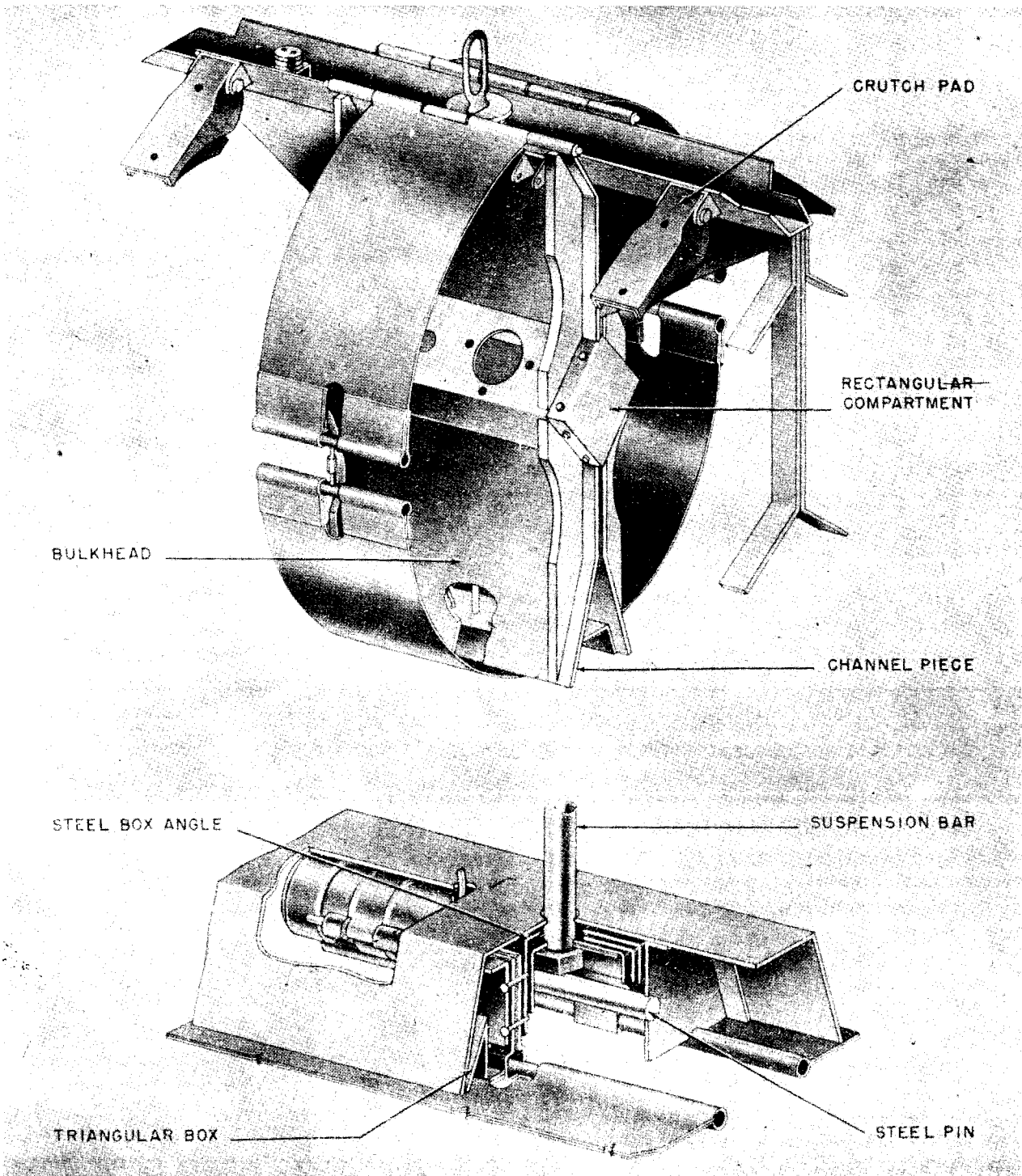
Figure 112—AB 500-3A Cluster Adapter
