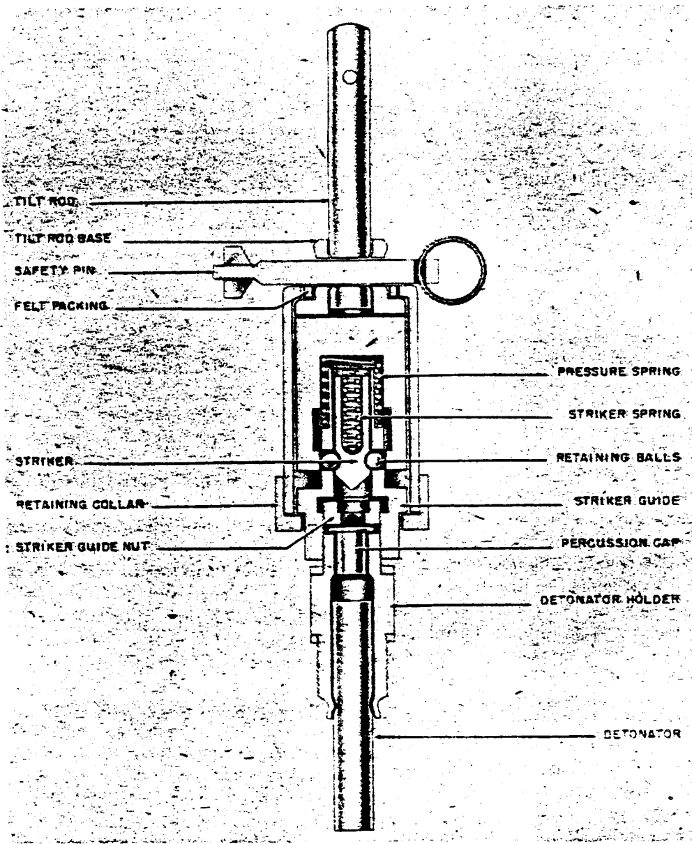
Figure 281—New Type Tilt Igniter (Pressure Tilt Type)
