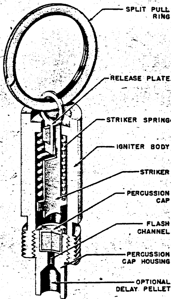
Figure 255—Type 2 Pull Percussion Igniter
