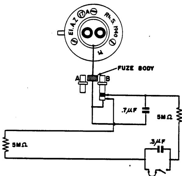
Figure 153B—(17)A Electrical Clockwork Time Fuze Wiring Diagram
