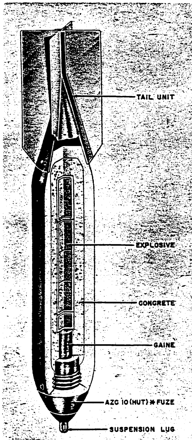
Figure 44—12-Kg SC 10 Concrete Bomb
