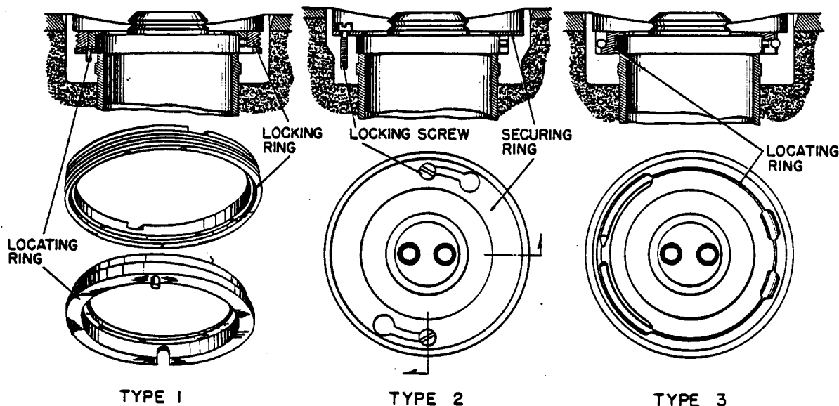
Figure 124—Methods of Securing the Fuze in the Bomb
