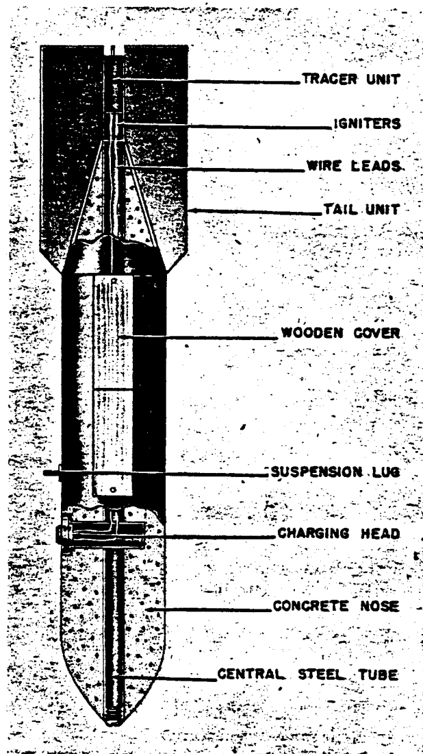
Figure 67—ZC 50-Kg Concrete Practice Bomb, Types I and II
