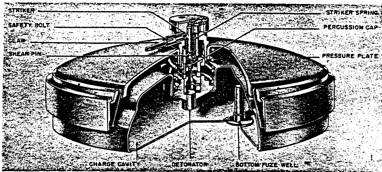
Figure 230—Tellermine 35—Antitank
