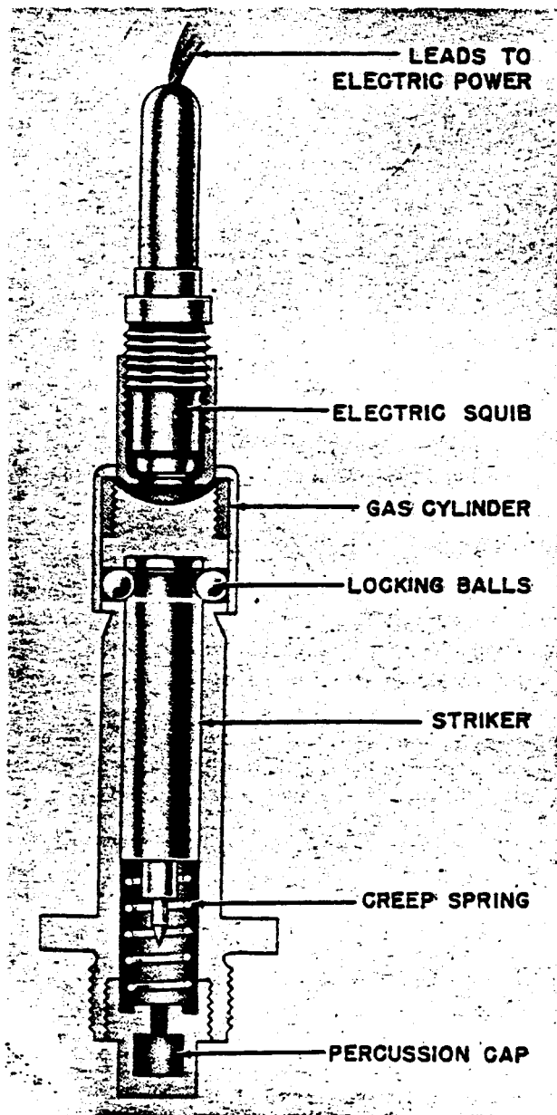
Figure 148—(46) Electrical Impact Tail Fuze
