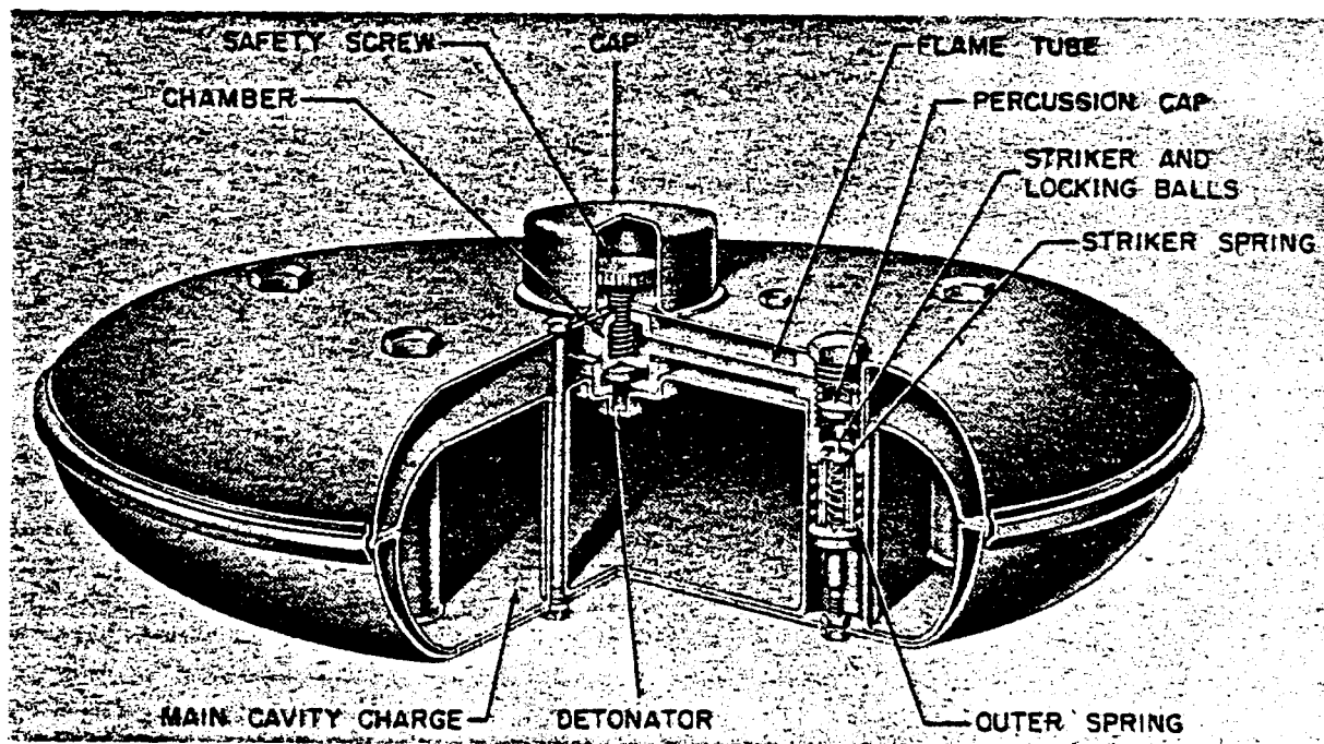
Figure 238—L. P. Z. Light Antitank or Antipersonnel Mine
