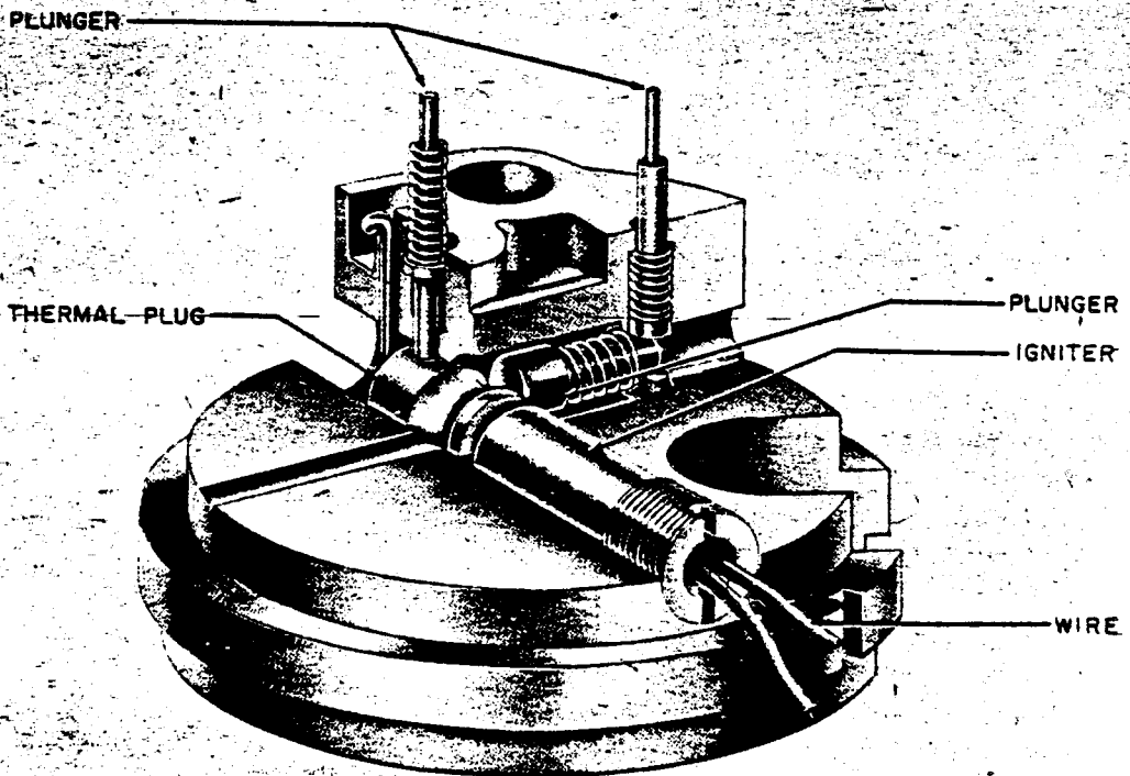
Figure 179—(89)B Clockwork Aerial Burst Fuze
