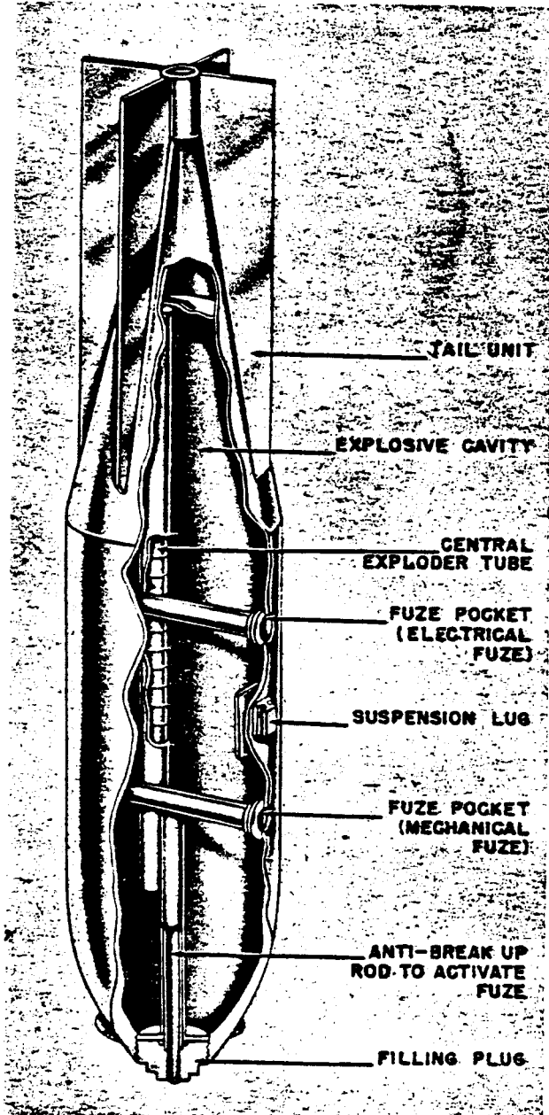
Figure 22—SB 2500-Kg Bomb
