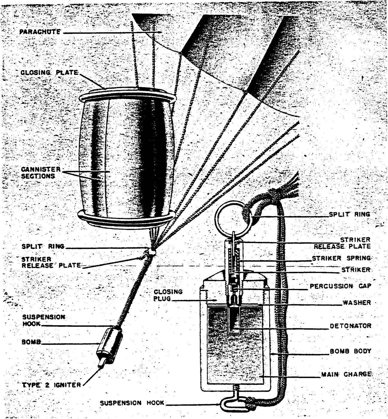
Figure 37—1/2 Kg Antipersonnel Parachute Bomb
