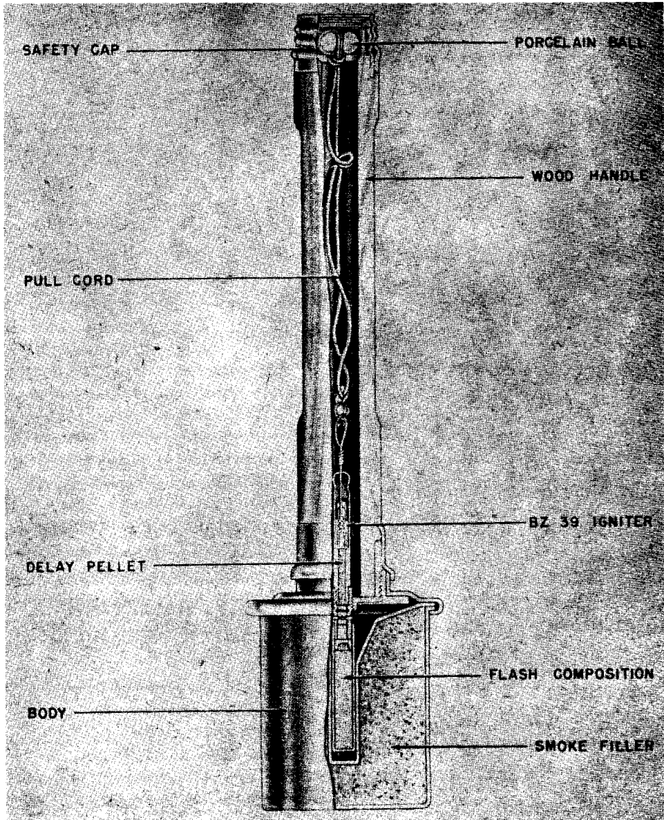
Figure 292—Type 39 Smoke Hand Grenade
