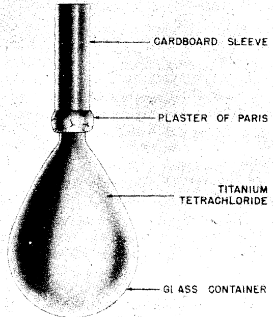
Figure 293—Blendkorper 14 Smoke Hand Grenade
