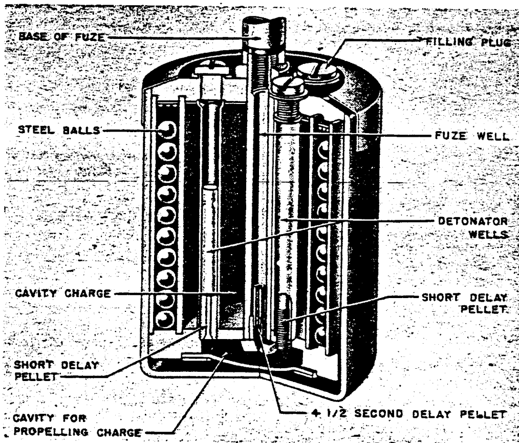
Figure 246—S-Mine 35—Antipersonnel
