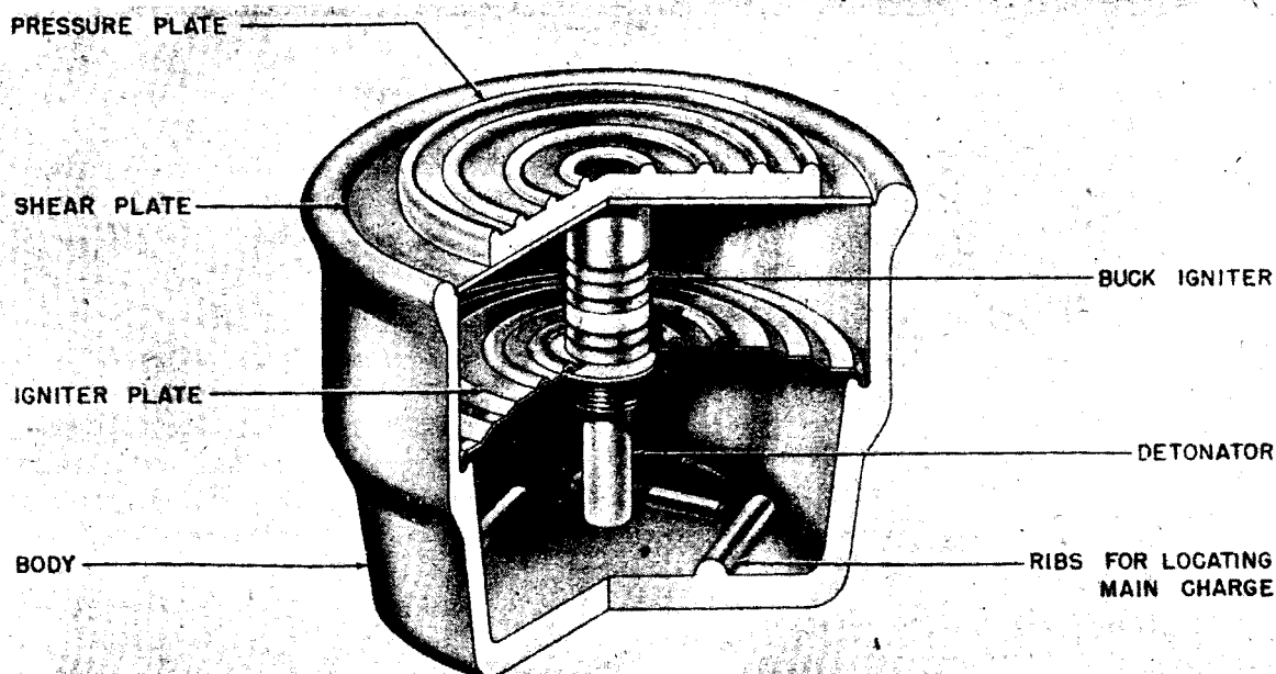
Figure 239—Glassmine 43 (f)—Antipersonnel
