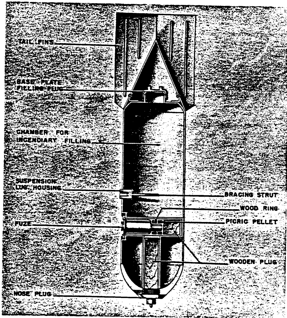
Figure 59—Brand C 50 B Bomb
