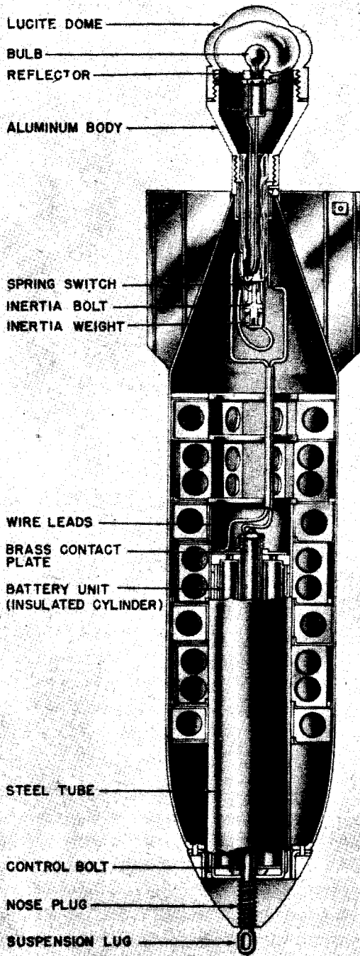
Figure 89—Sea Marker Bomb
