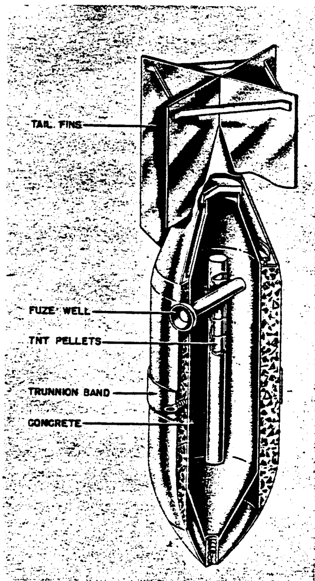
Figure 47—SBe 250-Kg Concrete Bomb
