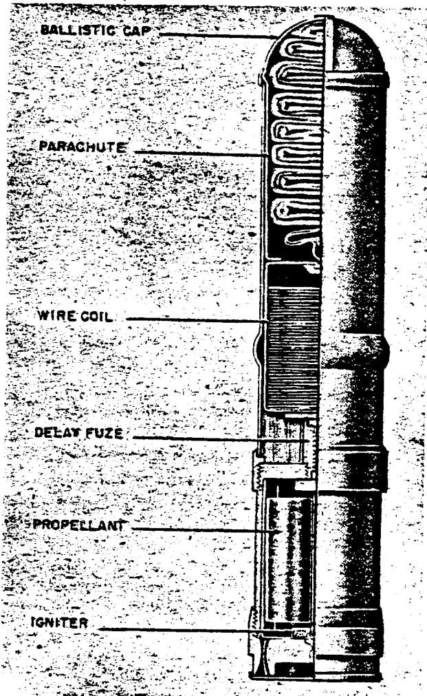
Figure 208—8.6-cm Illuminating Rocket (Naval)
