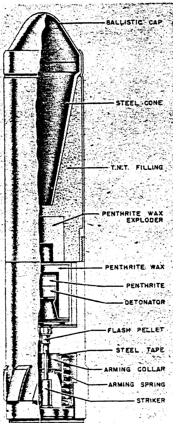
Figure 302—Antitank Hollow Charge Rifle Grenade
