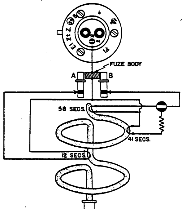
Figure 175—(59)B Electrical Aerial Burst Fuze
