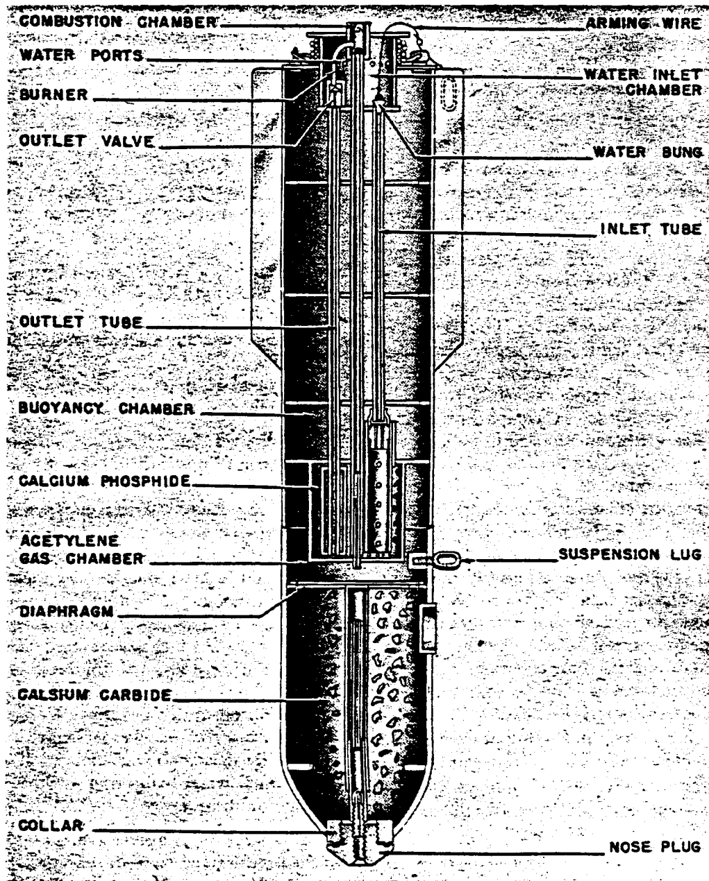
Figure 93—Lux N Flame Float
