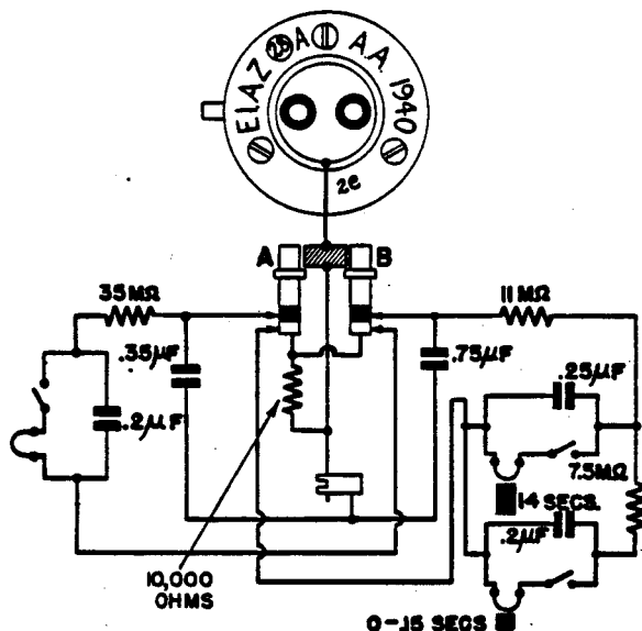
Figure 160—(28)A Electrical Impact Fuze
