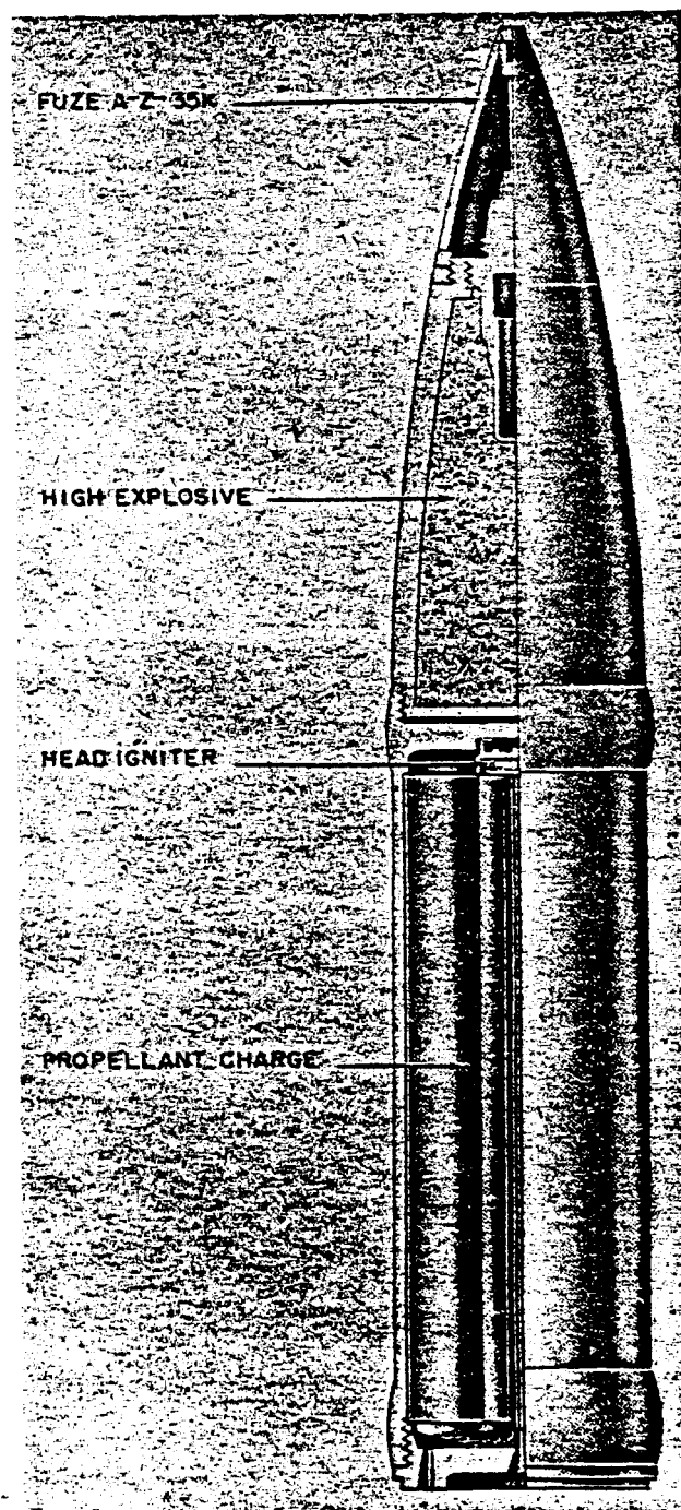
Figure 215—21-cm Aircraft Rocket
