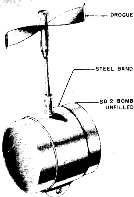
Figure 65—SD 2 Type Practice Bomb
