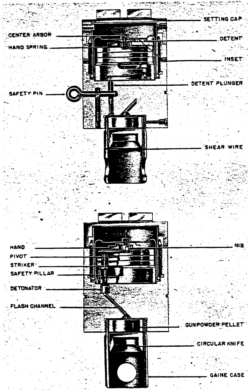
Figure 187—FZ 60 Clockwork Aerial Burst Fuze
