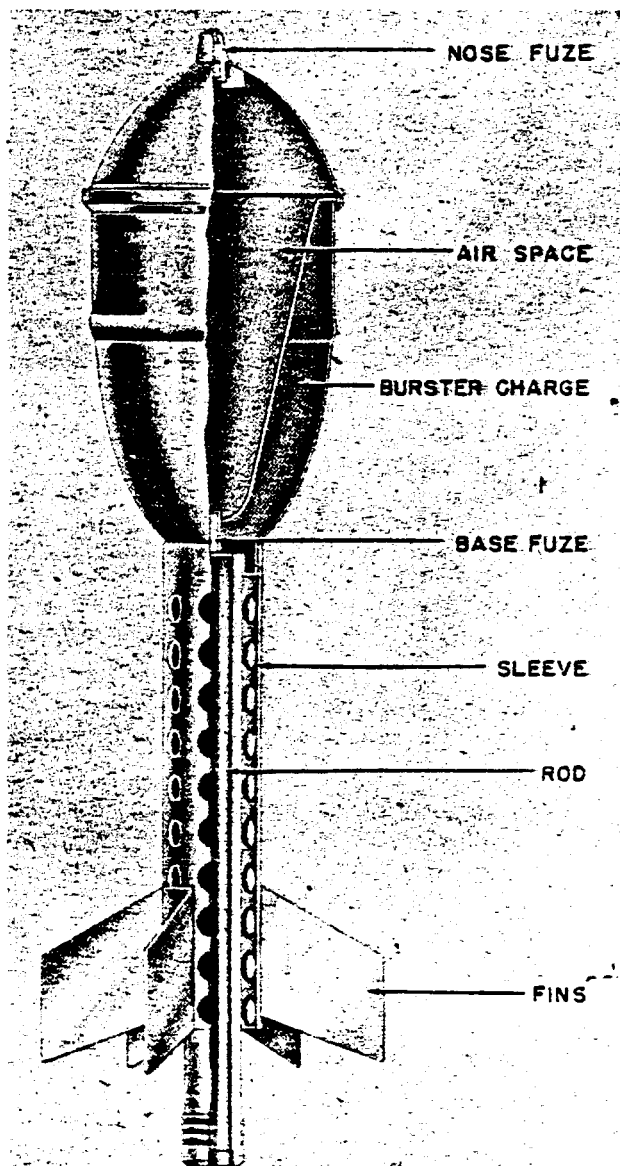
Figure 303—37-mm Hollow Charge Rifle Grenade
