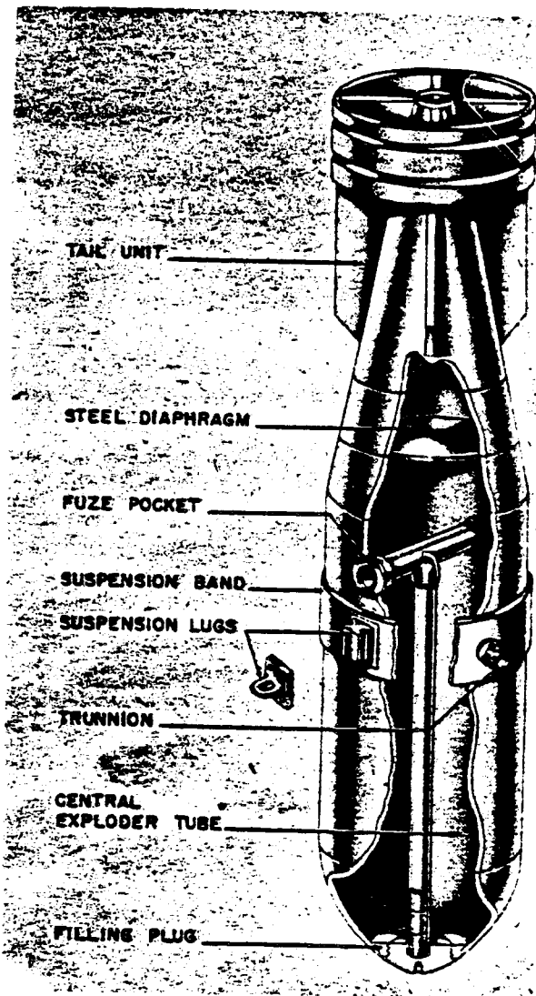
Figure 20—SB 1000-Kg Bomb
