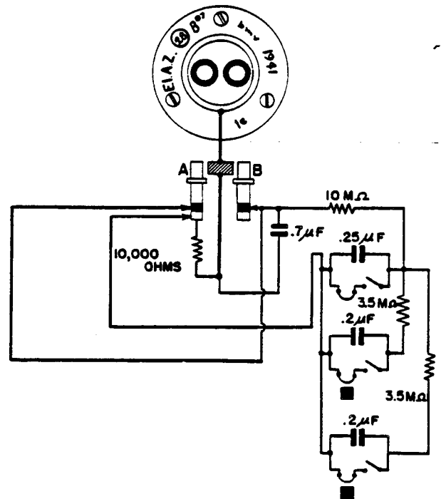
Figure 163—(28)B OT Electrical Impact Fuze
