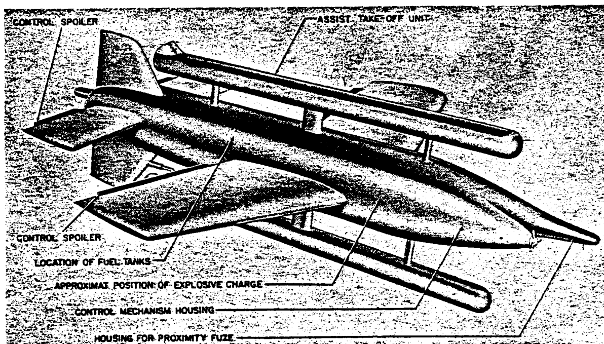
Figure 193—Hs 117 (Hs 297) "Schmetterling"
