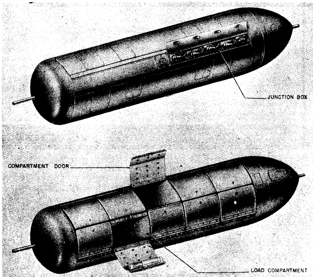
Figure 110—BSB 1000 Container
