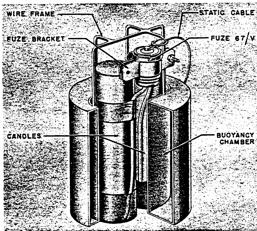
Figure 80—Mark 5 Flare, Types 1 and 2
