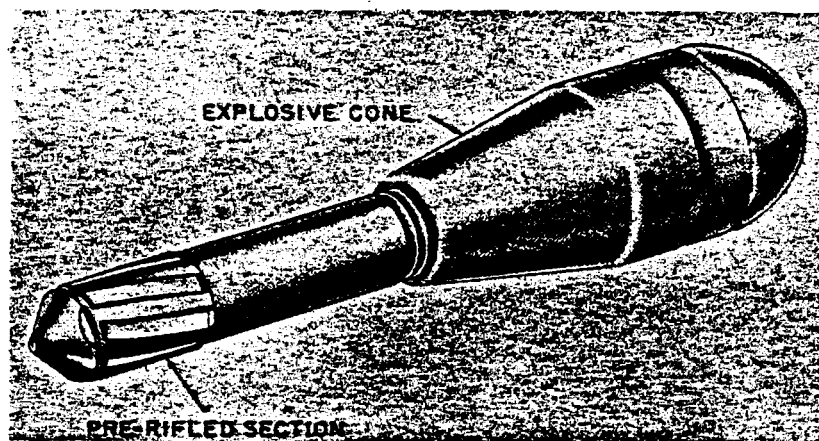
Figure 300—Hollow Charge Rifle Grenade
