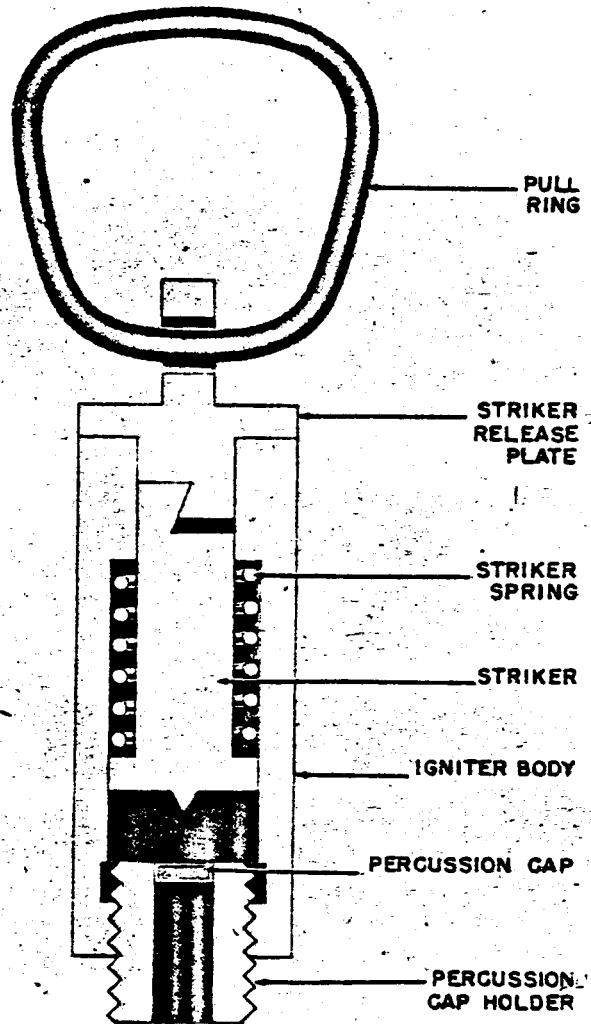
Figure 254—Safety Fuse Igniter, Percussion Type
