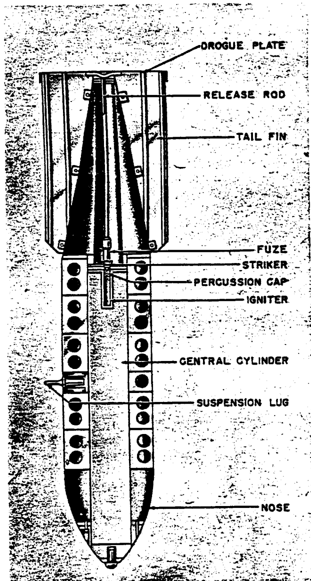
Figure 62—NC 50 W. C. Smoke Bomb
