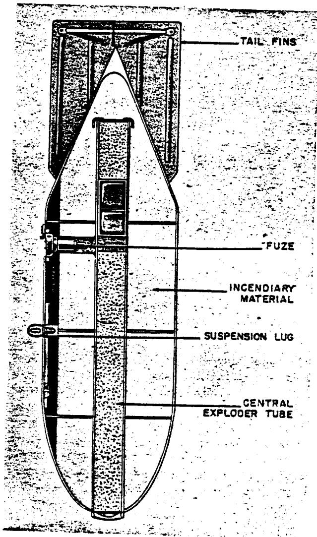
Figure 57—Flam C 500 Bomb
