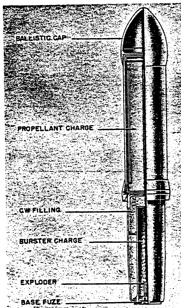
Figure 212—15-cm Smoke and Chemical Rocket
