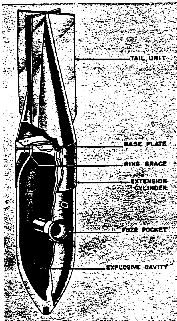
Figure 23—SD 50-Kg Bomb
