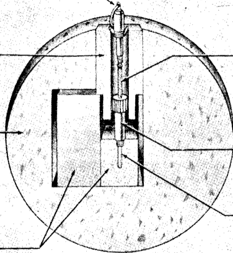
Figure 242—Concrete Ball Mine—Antipersonnel
