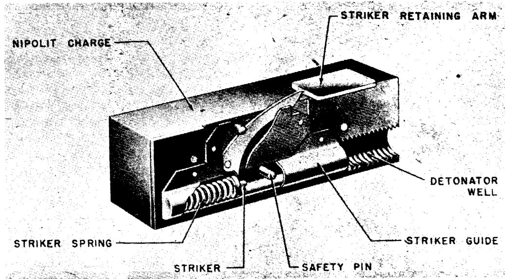
Figure 275—All-Explosive Pressure Release Device
