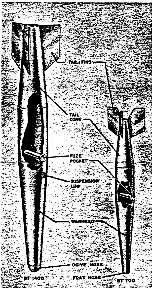
Figure 49—1400-Kg Bomben Torpedo
