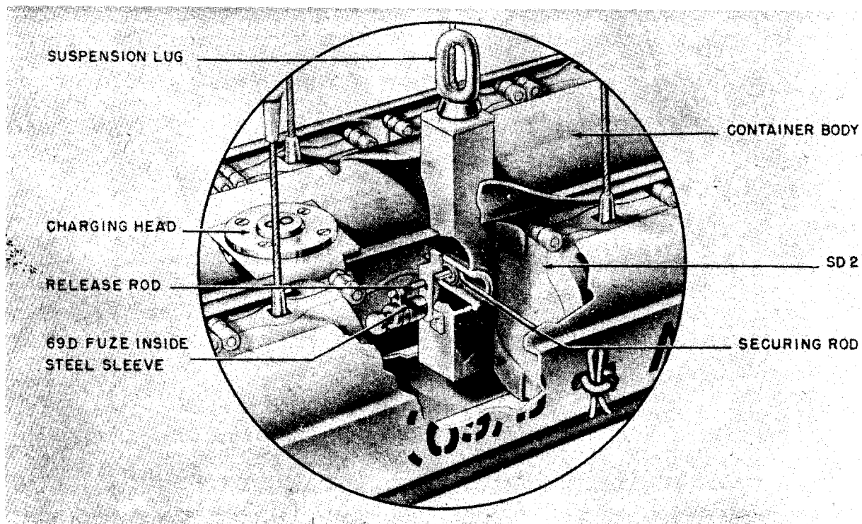
Figure 103B—AB 70-3 Container
