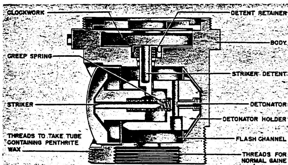
Figure 190—VZ (80) Mechanical All-Ways Action Fuze
