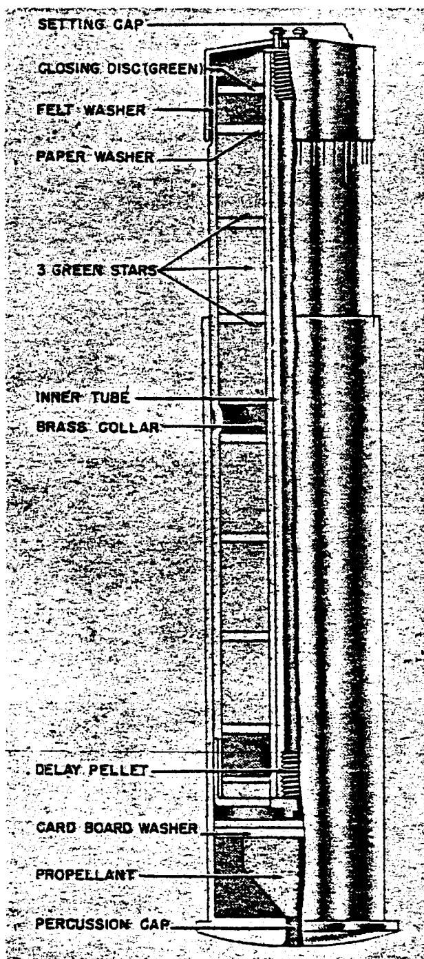
Figure 315—27-mm Multistar Pistol Cartridge
