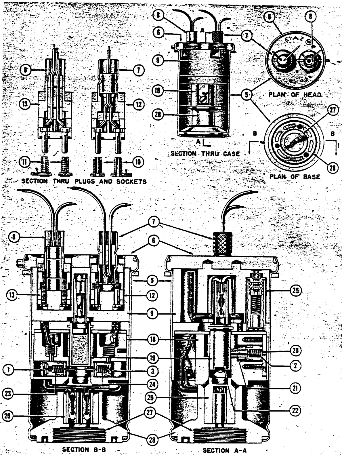
Figure 151A—(106)* Electrical Impact Fuze
