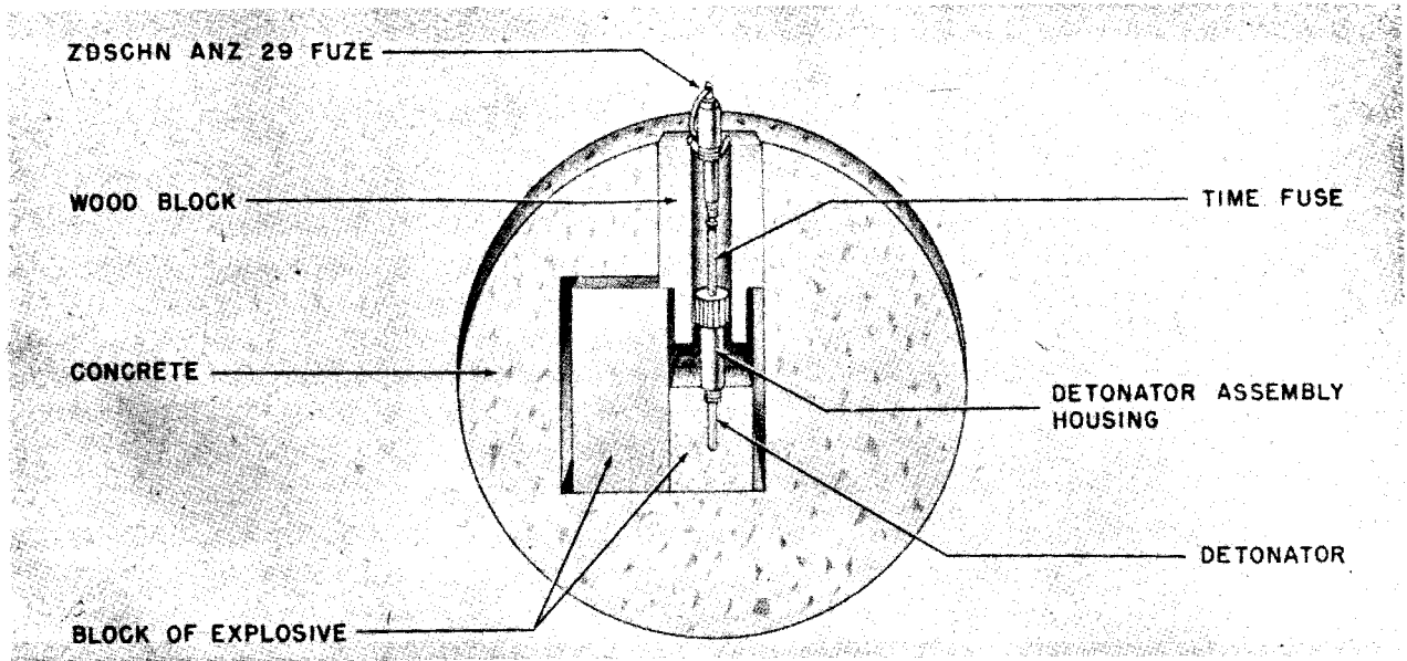
Figure 242—Concrete Ball Mine—Antipersonnel
