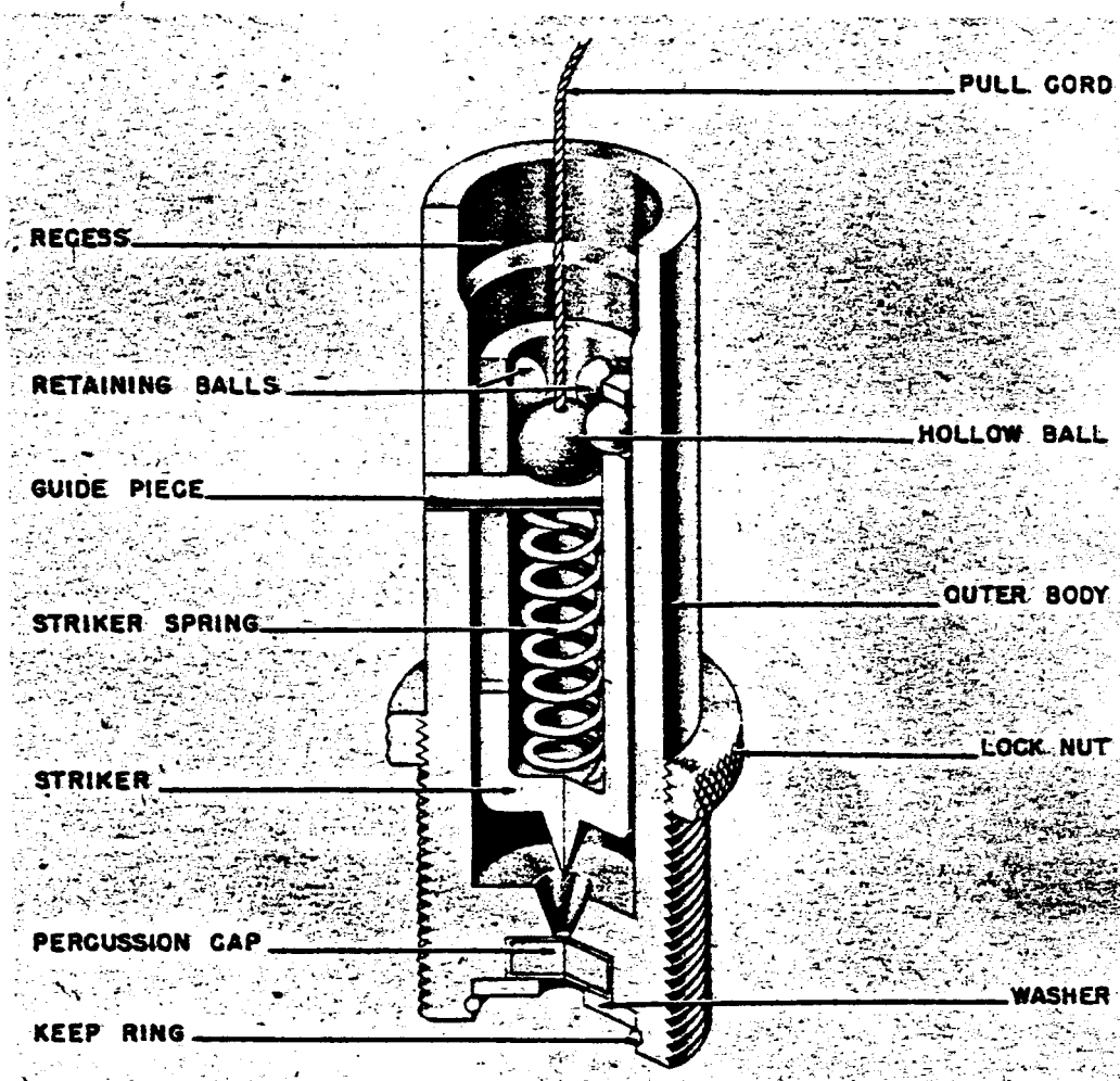
Figure 257—Type 31 Pull Igniter
