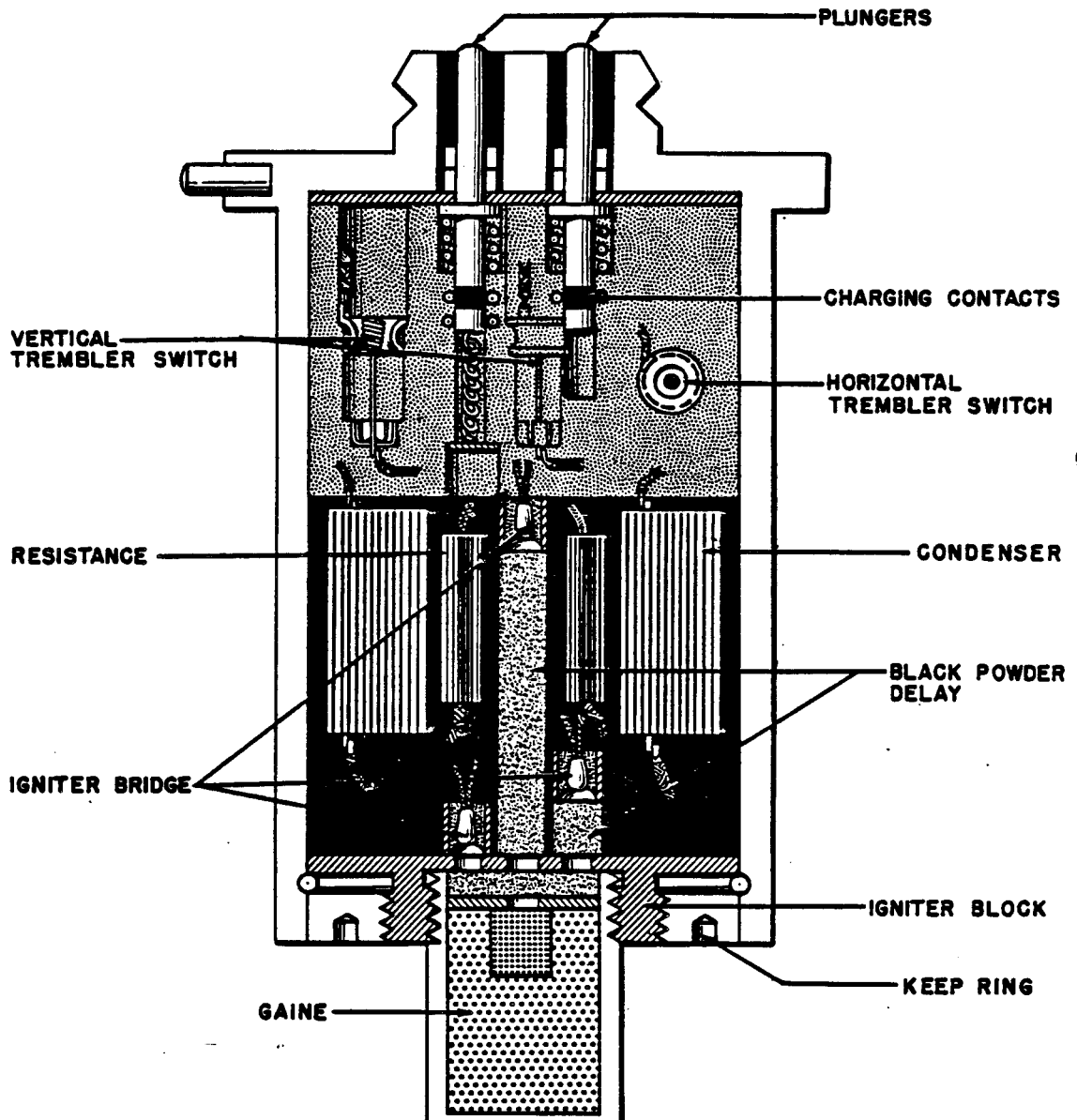
Figure 121—Internal Construction of Electrical Bomb Fuze
