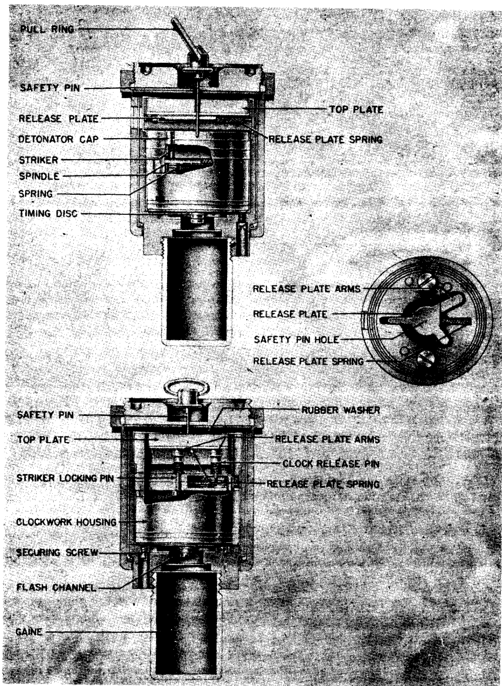
Figure 155—Z 17 Bm. Mechanical Clockwork Fuze
