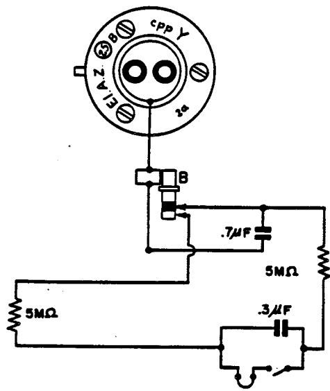
ARMING CIRCUIT DIAGRAM
