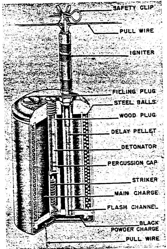
Figure 245—S-Mine 44—Antipersonnel
