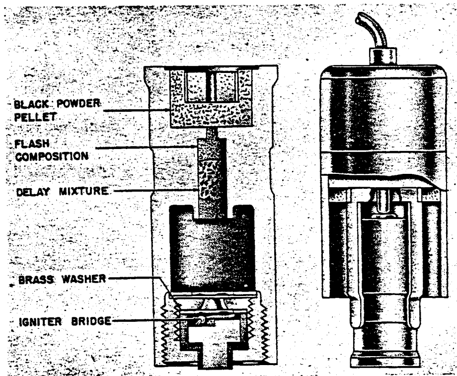
Figure 176—69CII Electrical Aerial Burst Fuze
