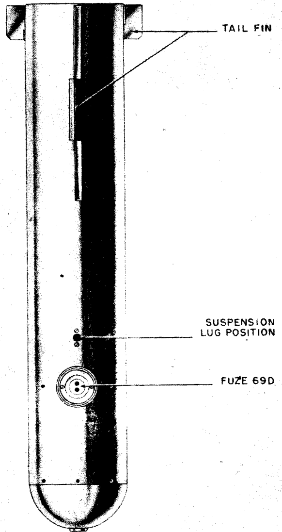
Figure 70—LC 10 Single Candle Parachute Flare
