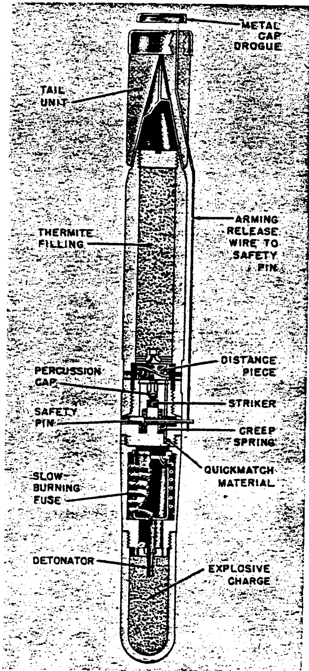
Figure 53—2.2-Kg B2.2EZ Incendiary Bomb
