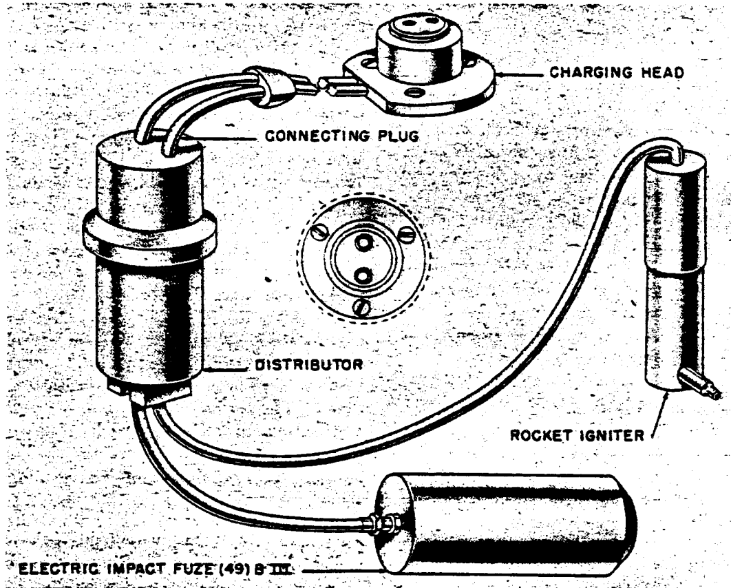
Figure 172—(49)C Rocket Bomb Fuze Assembly
