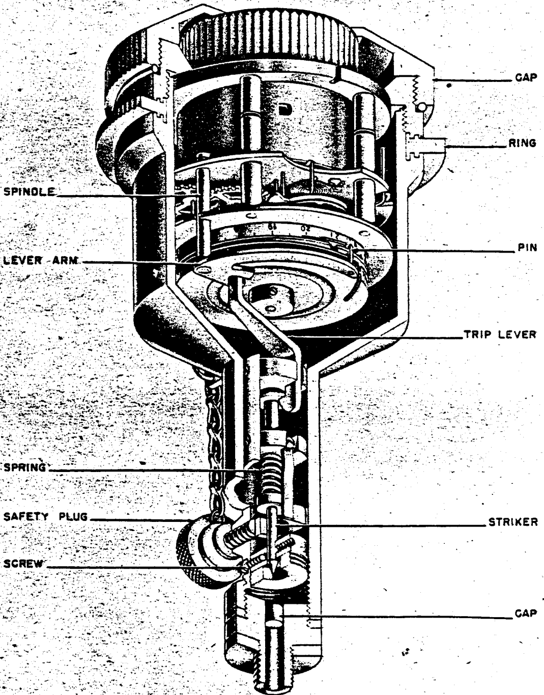
Figure 278—J-Feder 504 Clockwork
