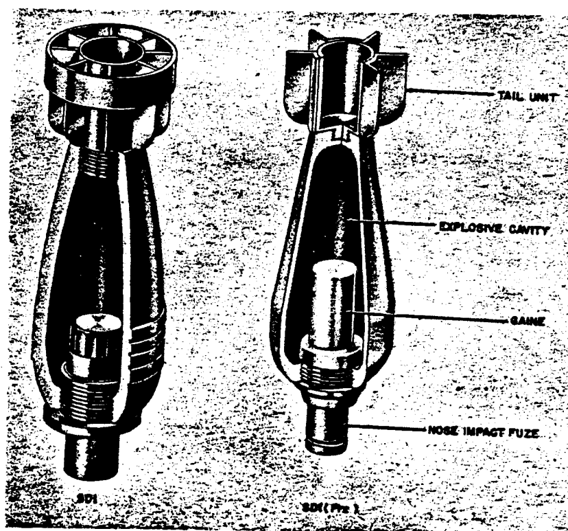
Figure 38—SD 1-Kg Mortar Bomb
