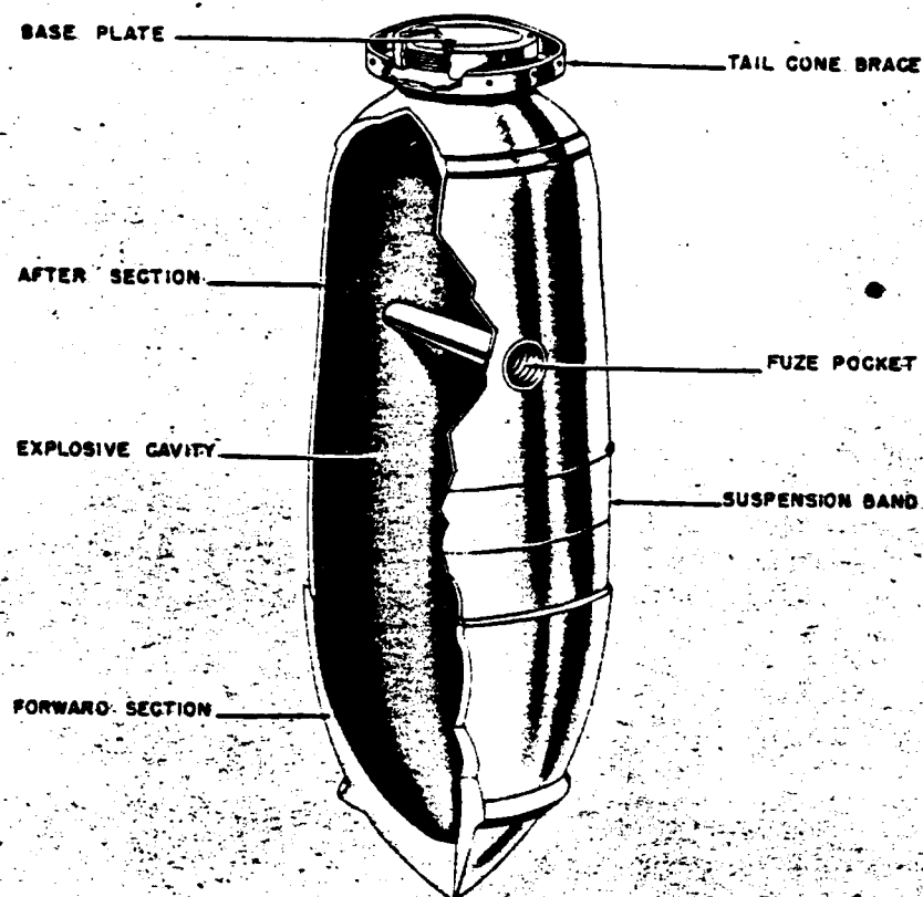
Figure 14—SC 1000-Kg Bomb
