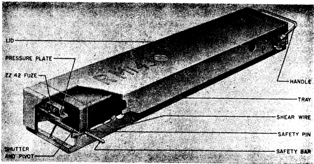
Figure 236—R Mine 43—Antitank
