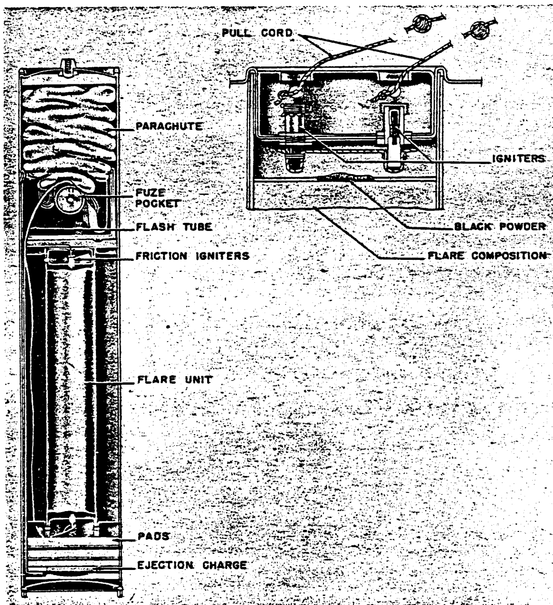
Figure 77—Parachute Flare with Pull Igniter
