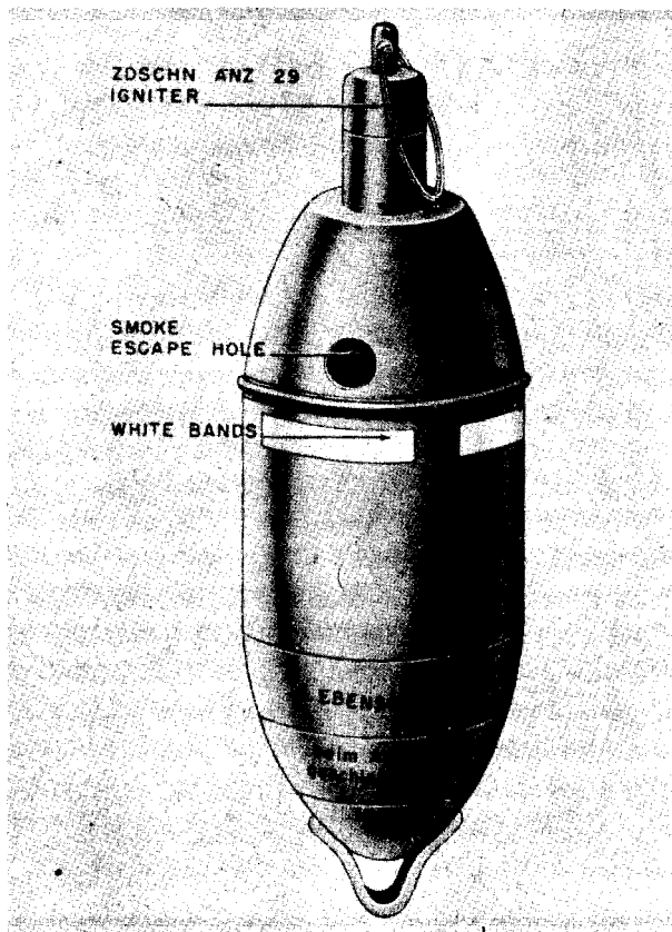
Figure 295—Egg Type Smoke Hand Grenade
