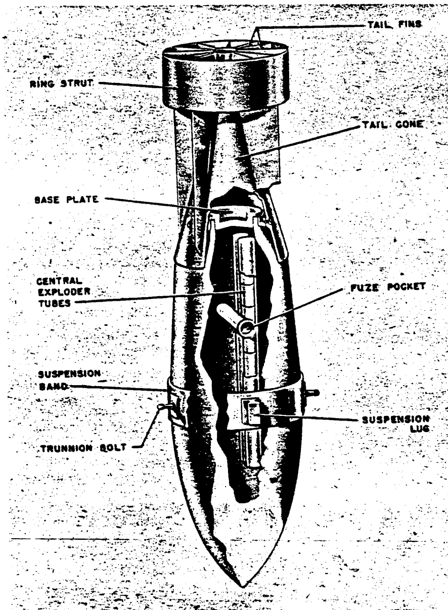
Figure 30—PC 1000-Kg Bomb
