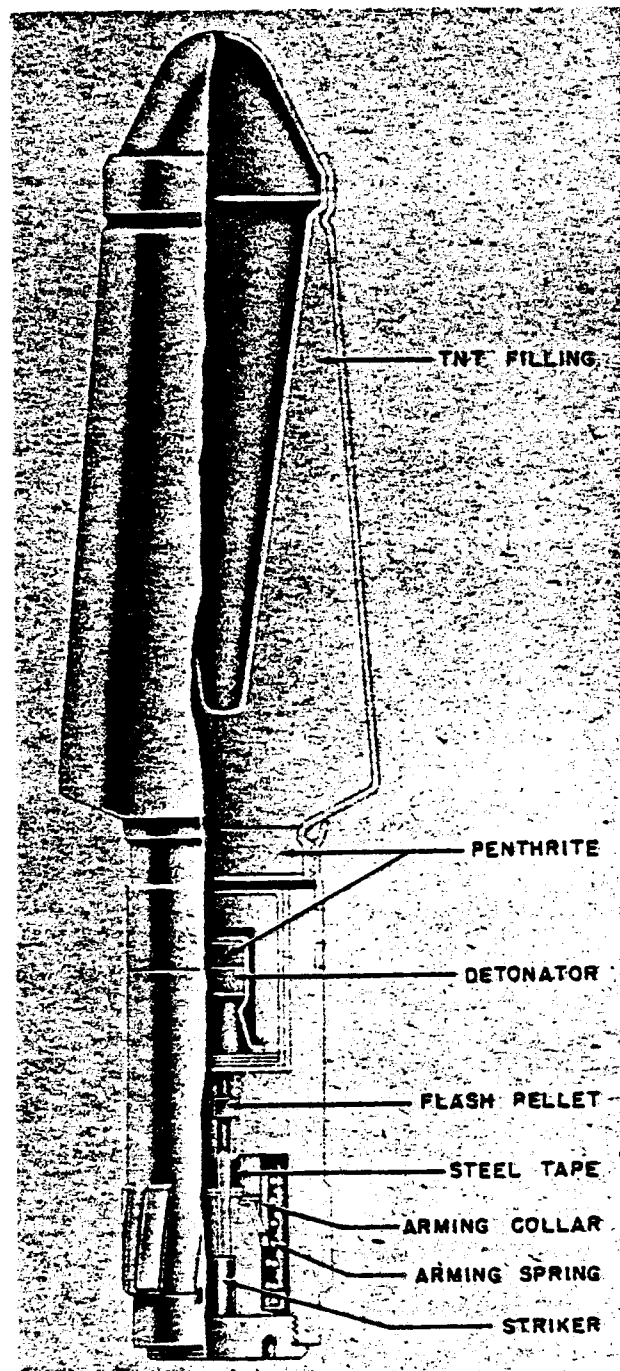
Figure 304—Large Hollow Charge Rifle Grenade
