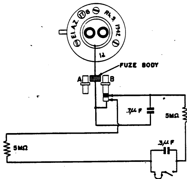
Figure 154—(17)B Electrical Clockwork Time Fuze
