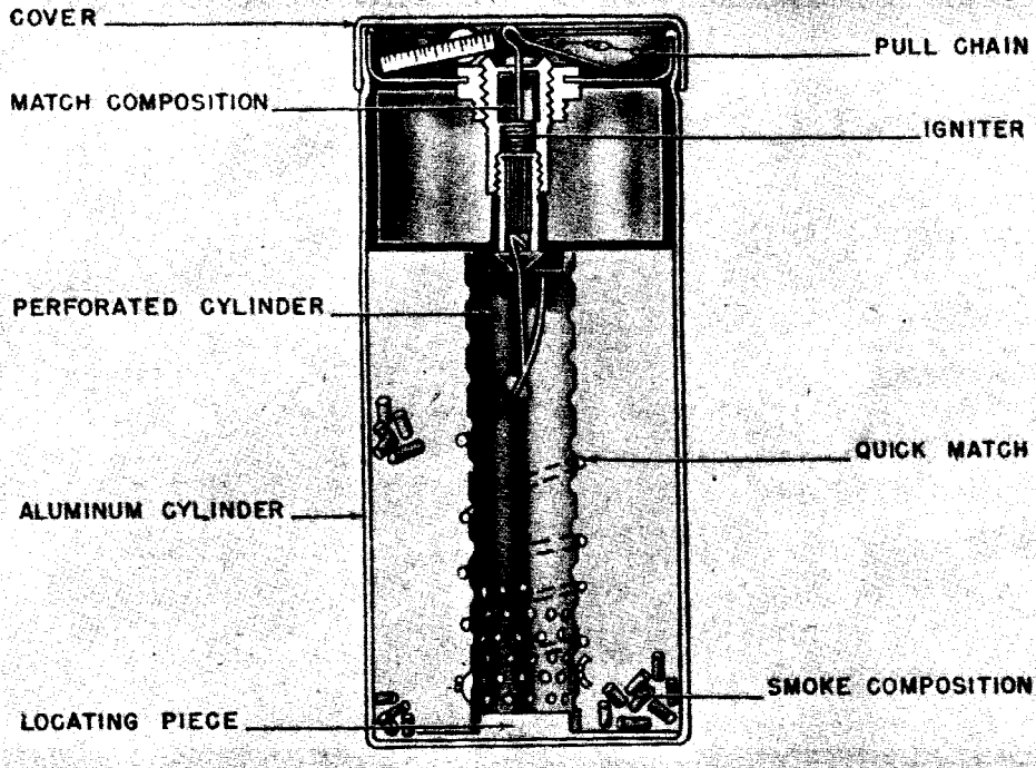
Figure 81—Smoke Flare, Orange, 160
