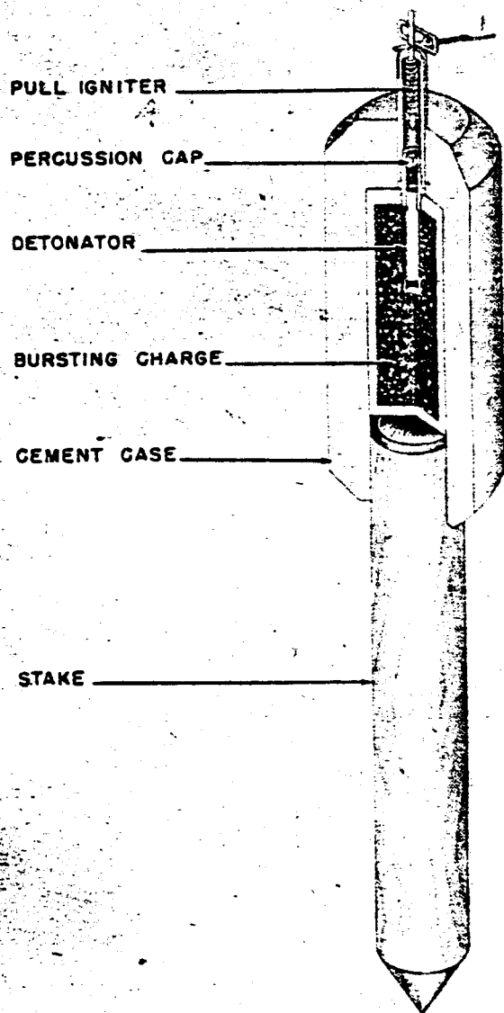
Figure 241—Stockmine—Antipersonnel
