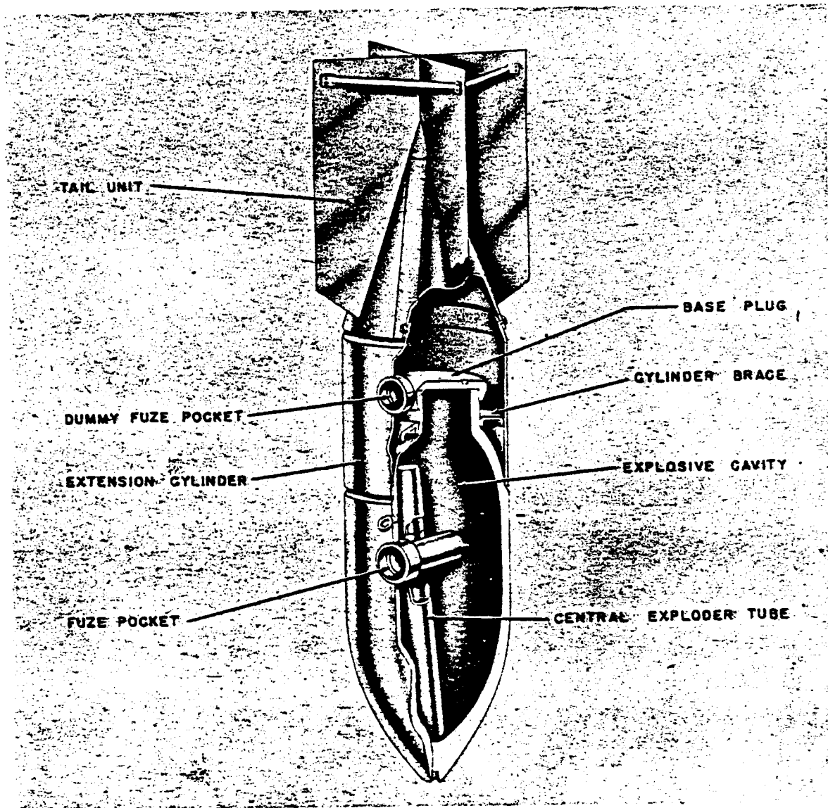
Figure 25—SD 250-Kg Bomb
