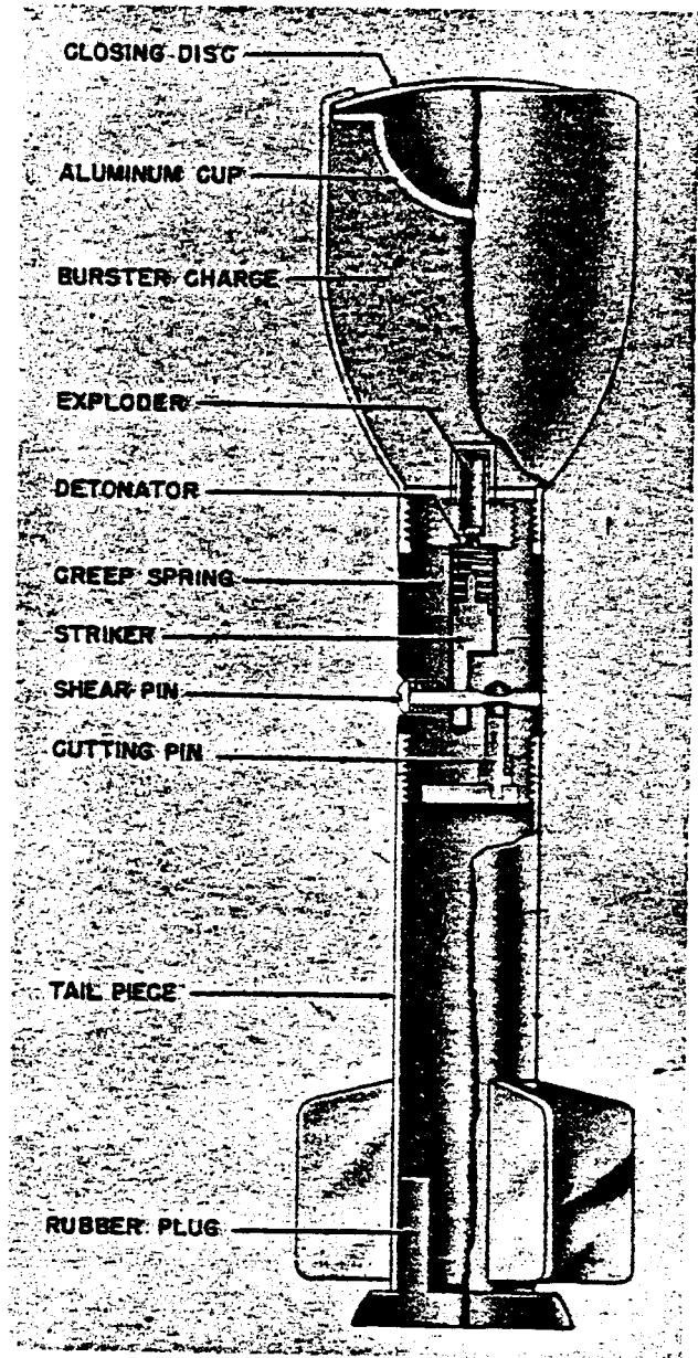
Figure 305—Schuss Gg. P-40 Hollow Charge Rifle Grenade
