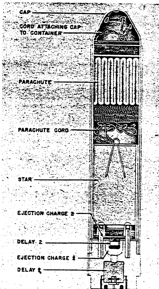
Figure 307—Illuminating Rifle Grenade
