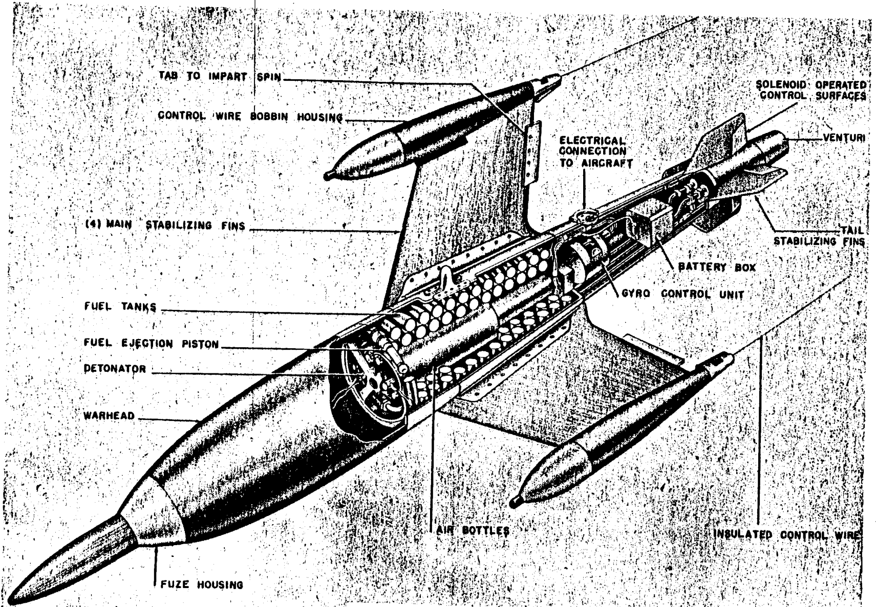
Figure 197A—X-4 Missile
