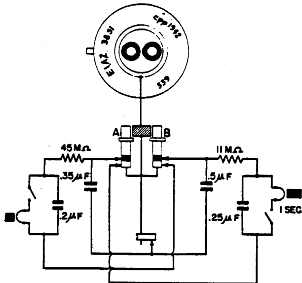
Figure 166—(38 sl) Electrical Impact Fuze
