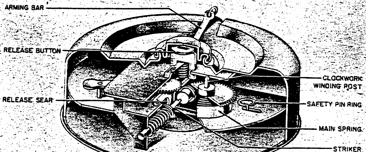
Figure 283—E. Z. 44 Antilifting Device
