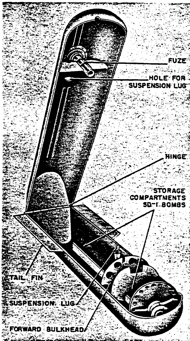
Figure 104—AB 70D1 Container
