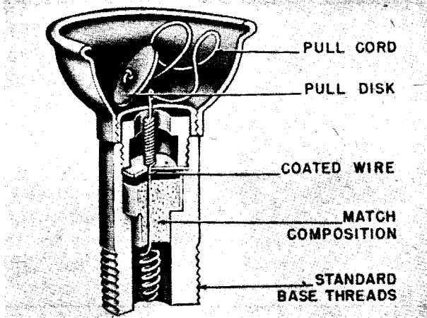
Figure 252—ZDSCHN-ANZ-39 Friction Igniter Pull Type
