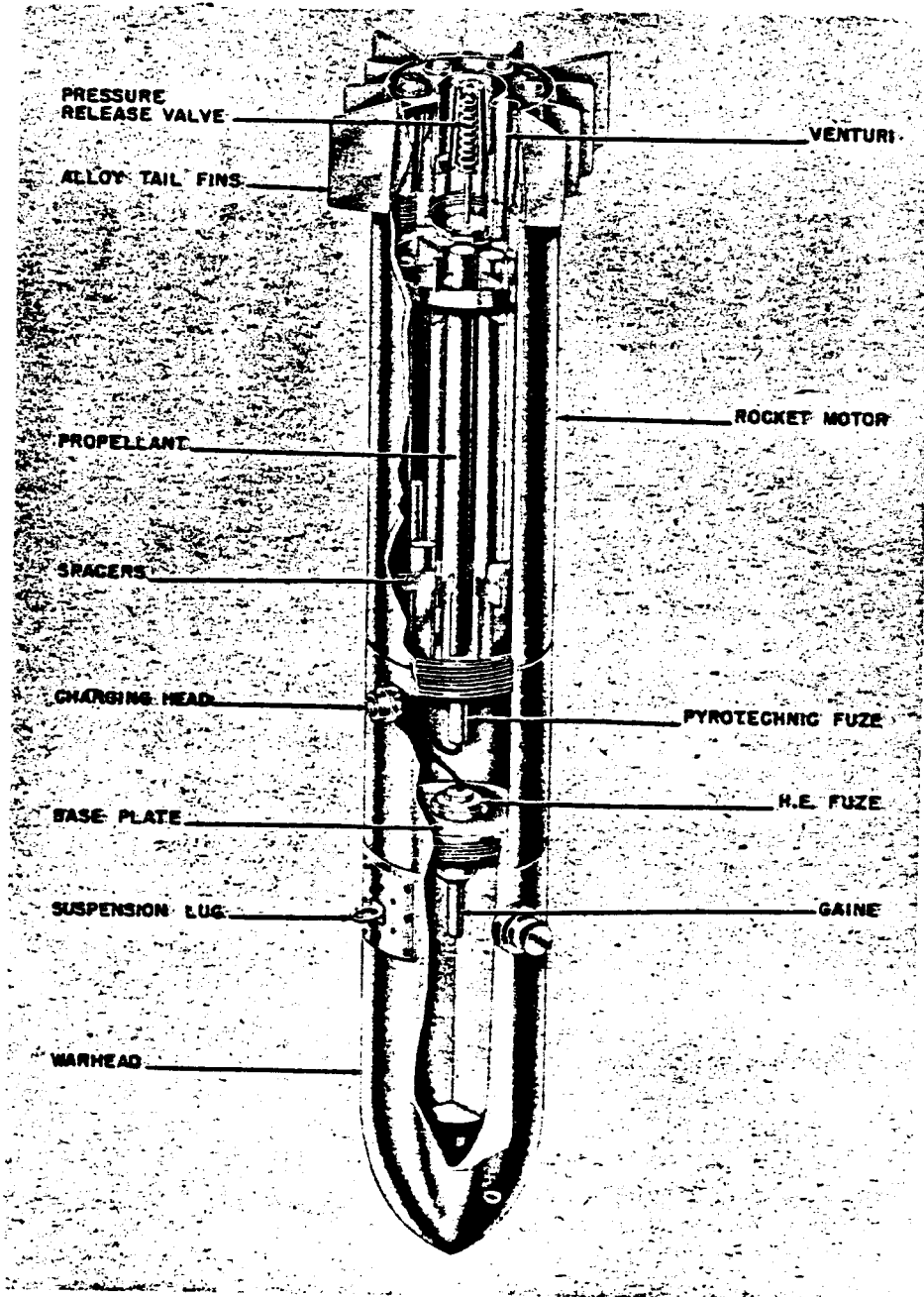
Figure 33—PC 500 RS Bomb
