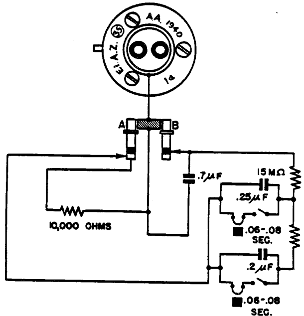
Figure 143—(35) Electrical Impact Fuze
