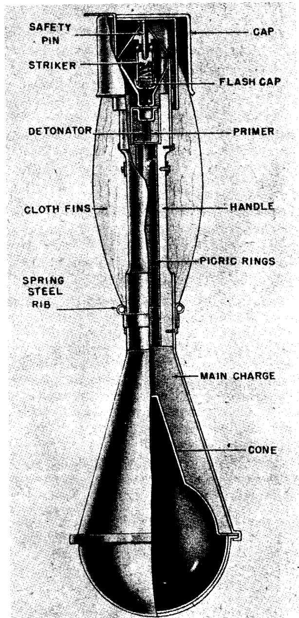
Figure 290—Panzerwurfmine Hollow Charge Hand Grenade
