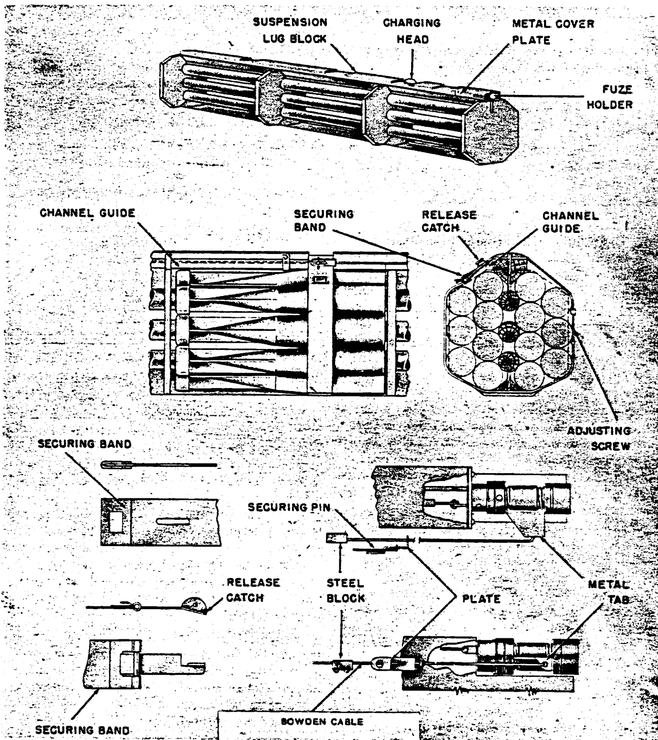
Figure 101—AB 42 Container
