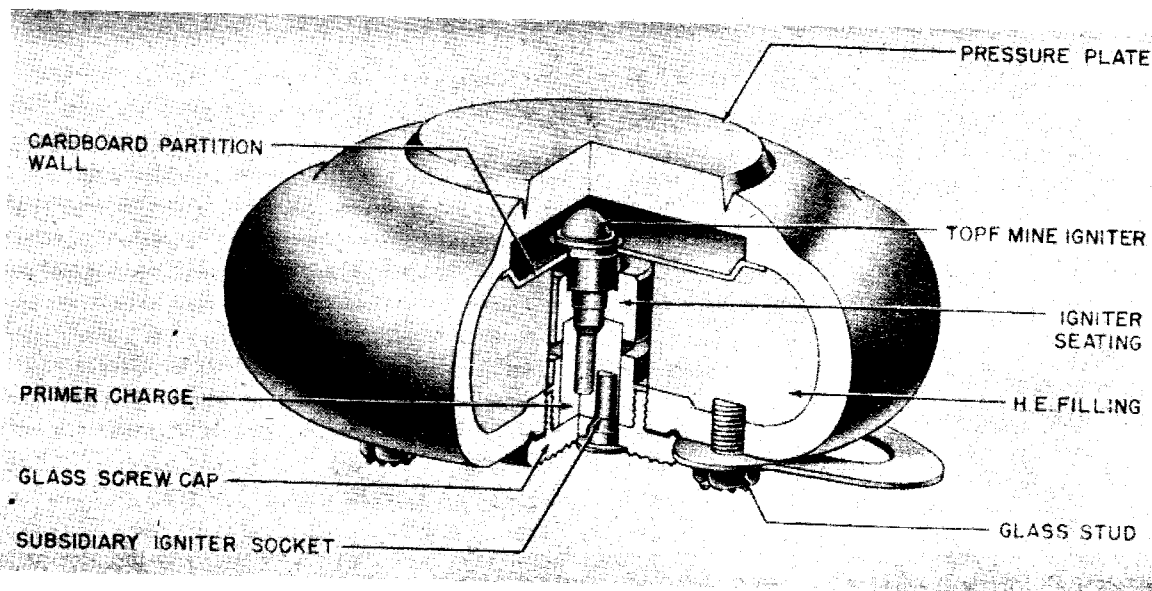
Figure 235—Topf Mine A—Antitank
