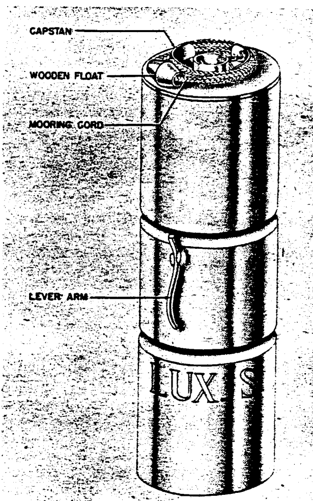
Figure 94—Lux S Flame Float, Types 1, 2, and 3
