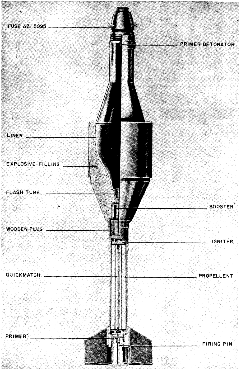
Figure 210—8.8-cm Hollow Charge Antitank Rocket
