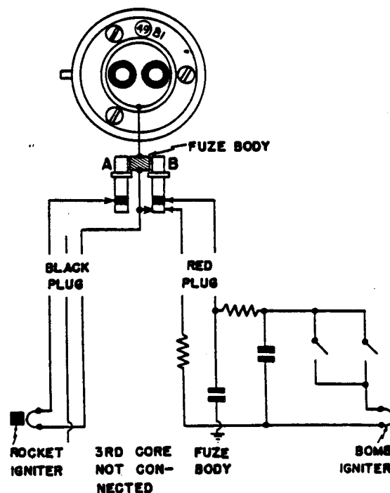
Figure 171—(49)B Rocket Bomb Fuze Assembly
