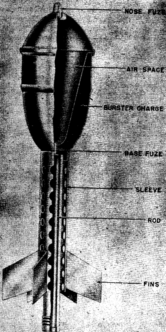
Figure 303—37-mm Hollow Charge Rifle Grenade
