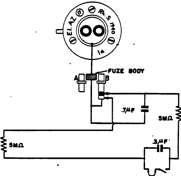
Figure 152—(17) Electrical Clockwork Time Fuze
