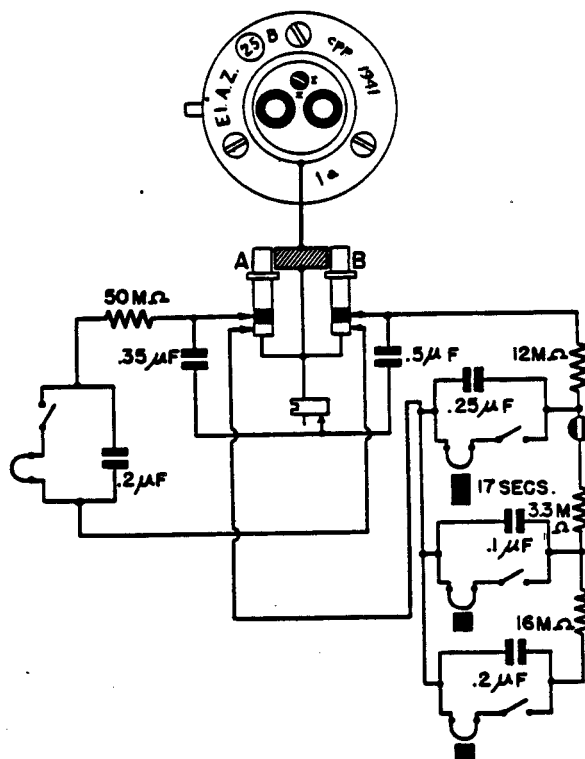
Figure 141—(25)B Electrical Impact Fuze
