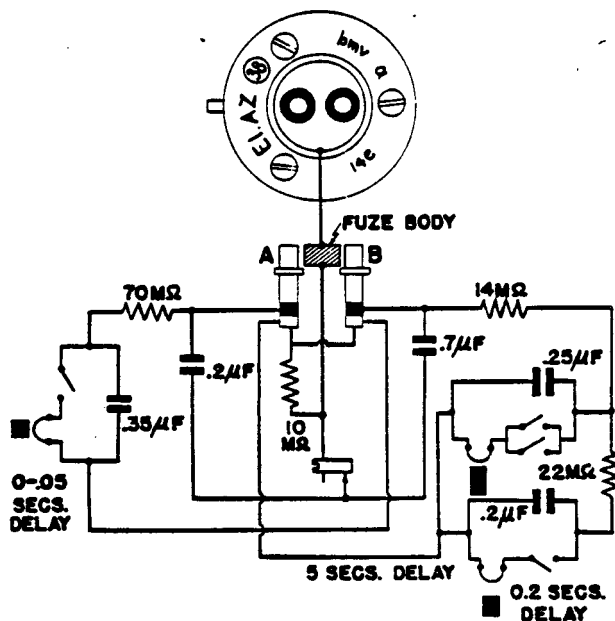
Figure 165—(38) Modified Electrical Impact Fuze
