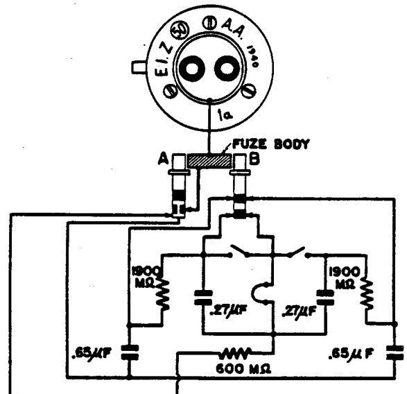
Figure 185—(50) Yellow Top Electrical Antidisturbance Fuze
