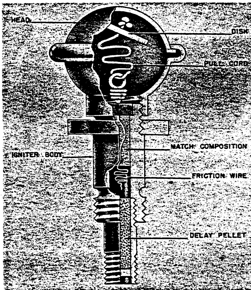
Figure 250—B. Z. E. Friction Igniter Pull Type
