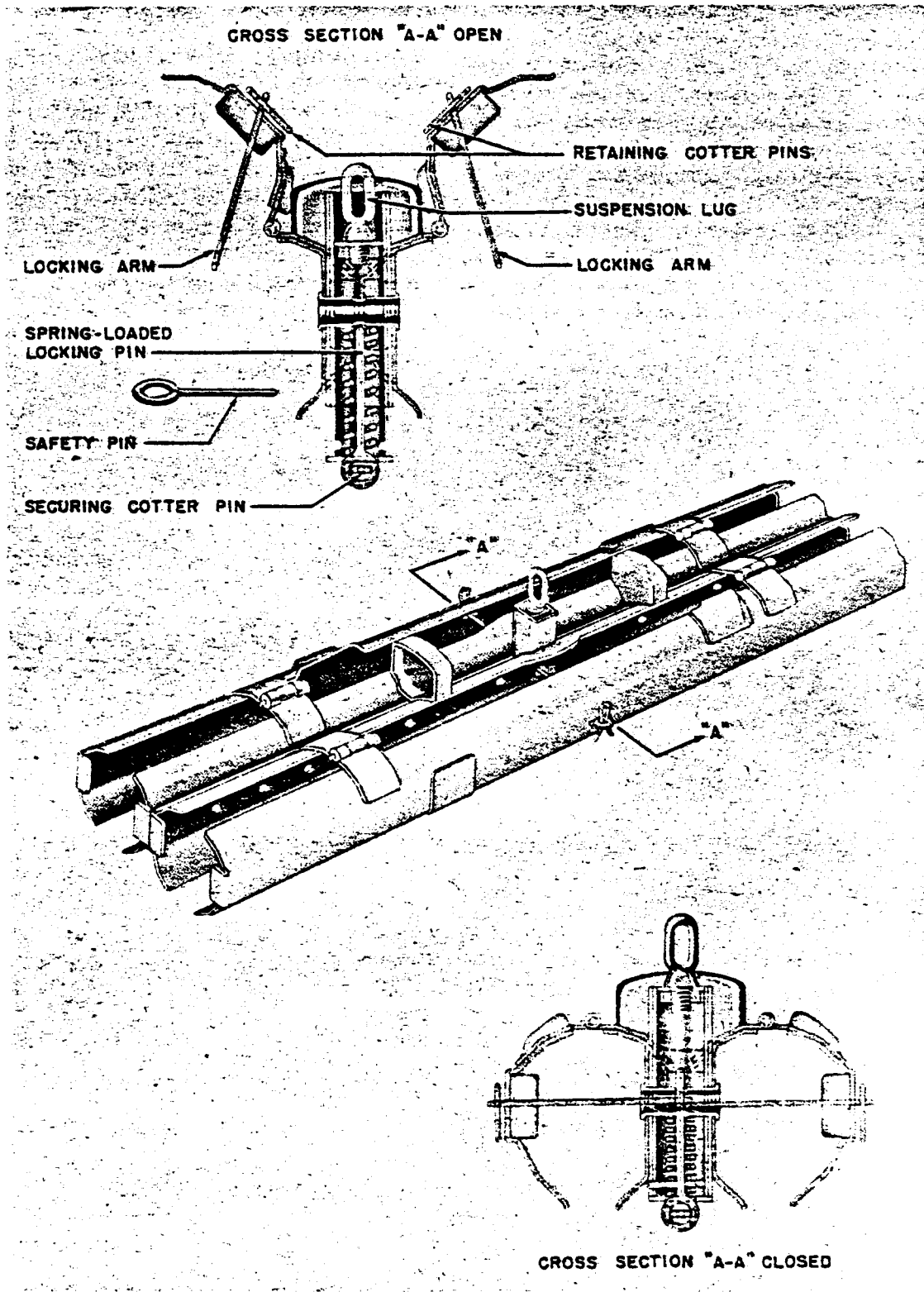
Figure 97—AB 24T SD 2 Container
