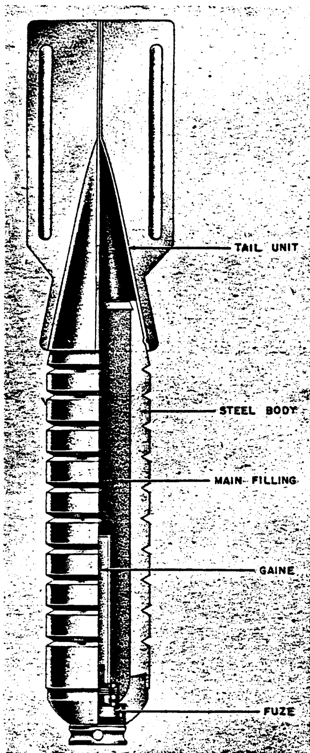
Figure 43—SD 10C Antipersonnel Bomb
