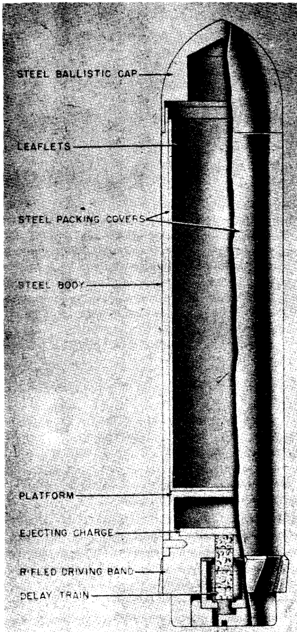
Figure 306—Propaganda Rifle Grenade
