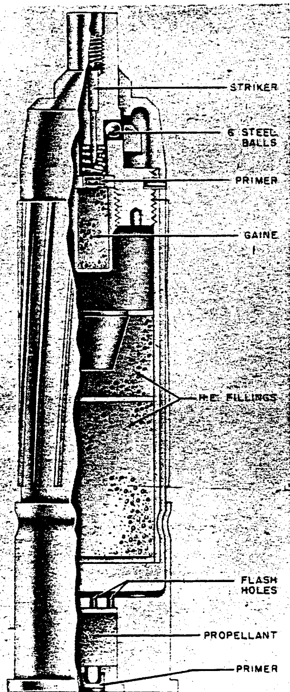
Figure 312—H. E. Cartridge for 27-mm Grenade Pistol
