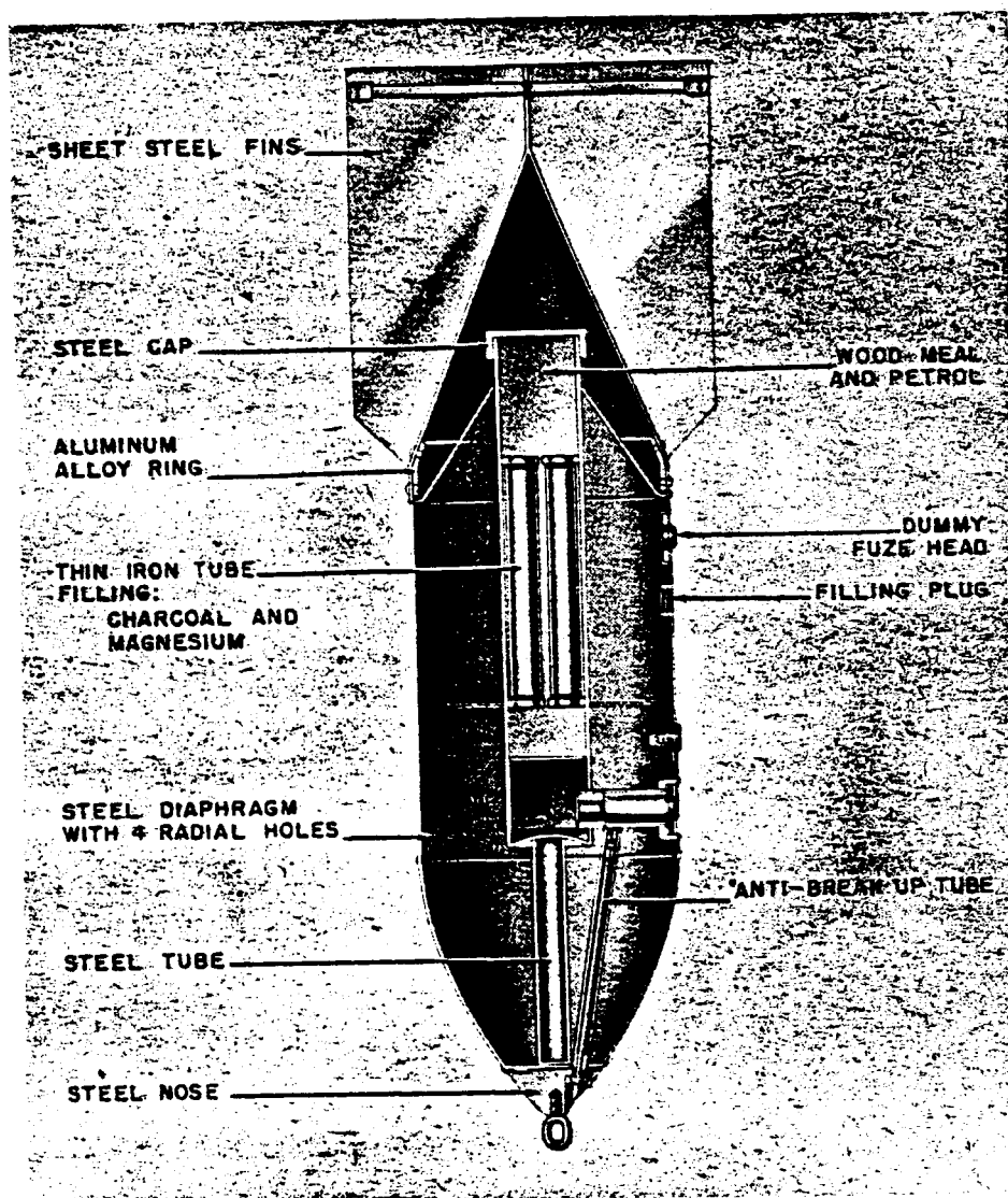
Figure 56—KC 250 Flam Bomb
