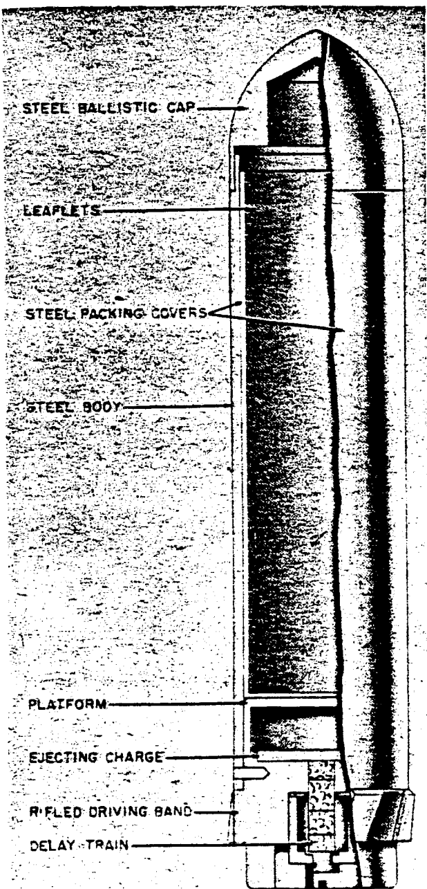
Figure 306—Propaganda Rifle Grenade
