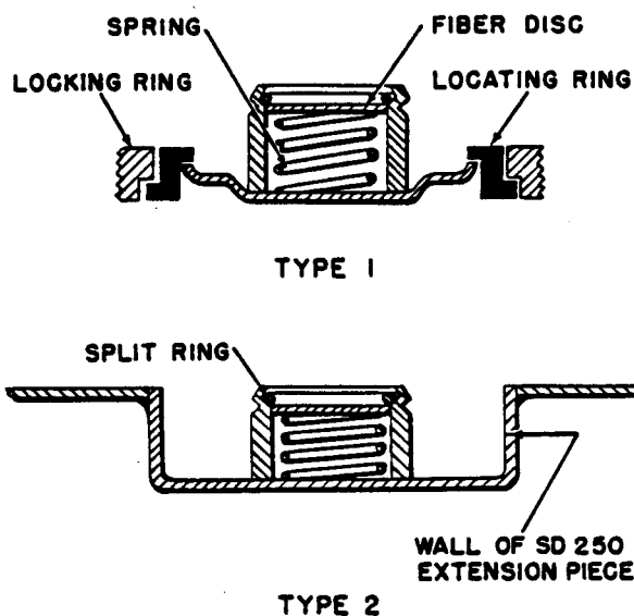
Figure 127—Dummy Fuze Heads
