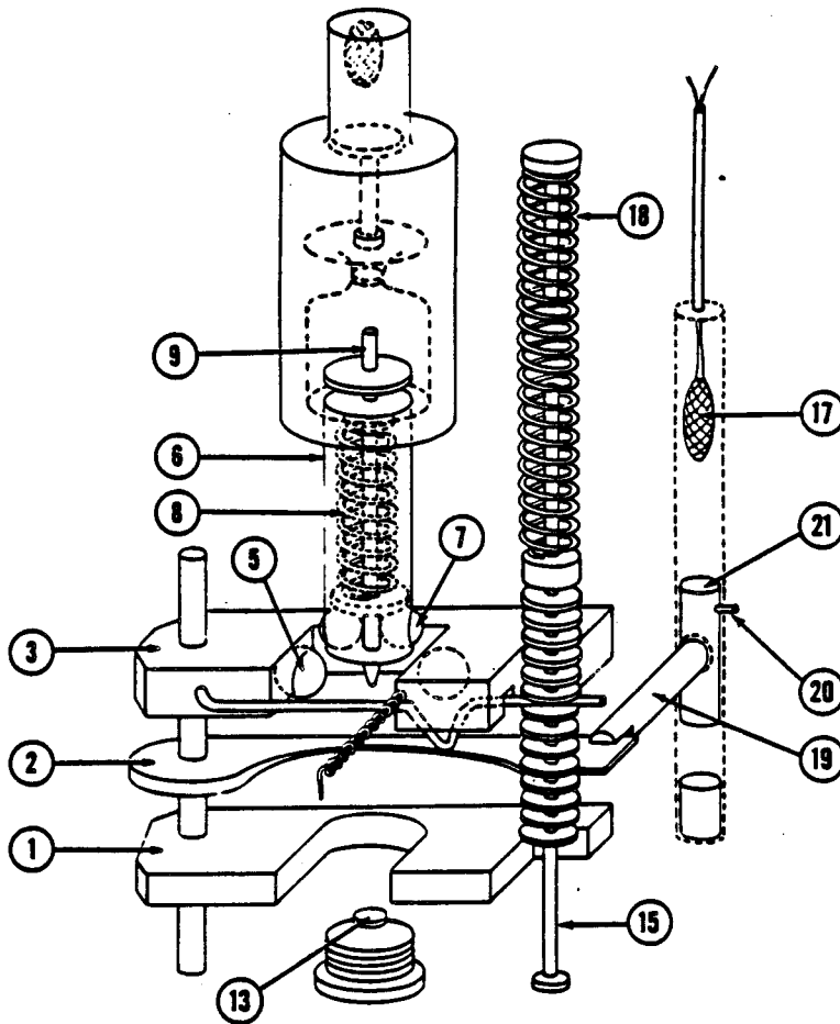
Figure 156B—(57) Electrical Chemical Time Fuze Schematic Diagram
