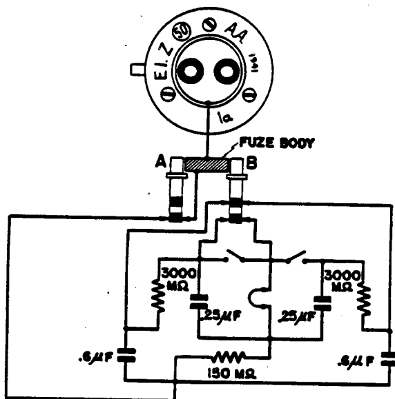
Figure 184—(50) Electrical Antidisturbance Fuze
