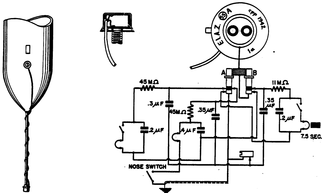
Figure 146—(55)A Electrical Impact Fuze
