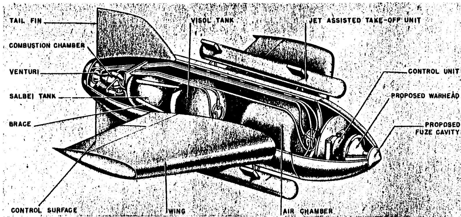
Figure 202—Enzian E-4
