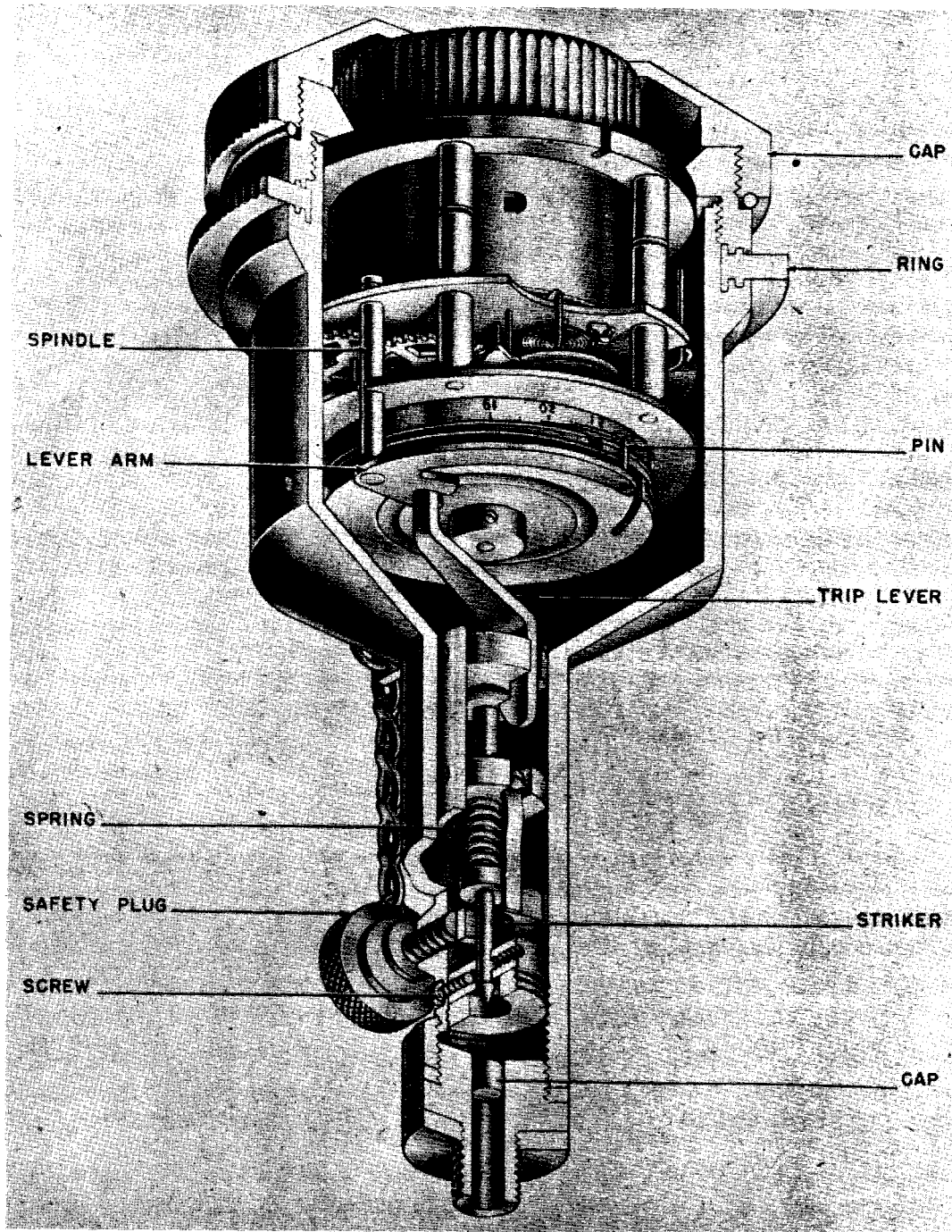
Figure 278—J-Feder 504 Clockwork
