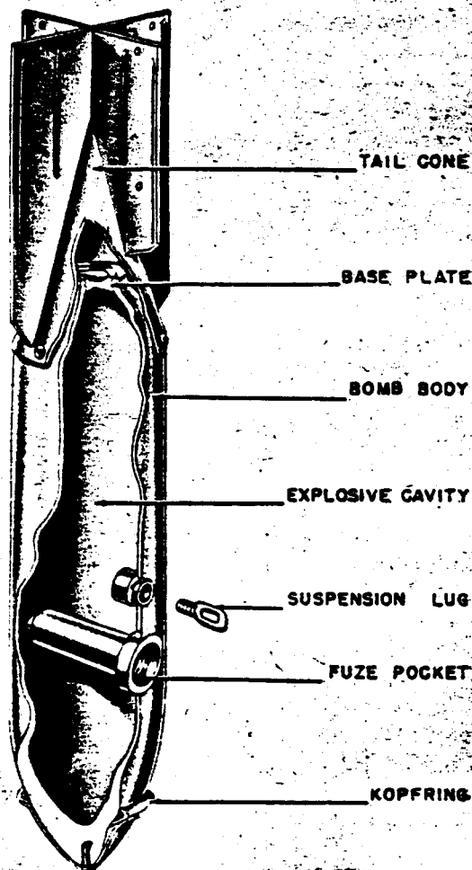
Figure 10—SC 50 Grade I Bomb
