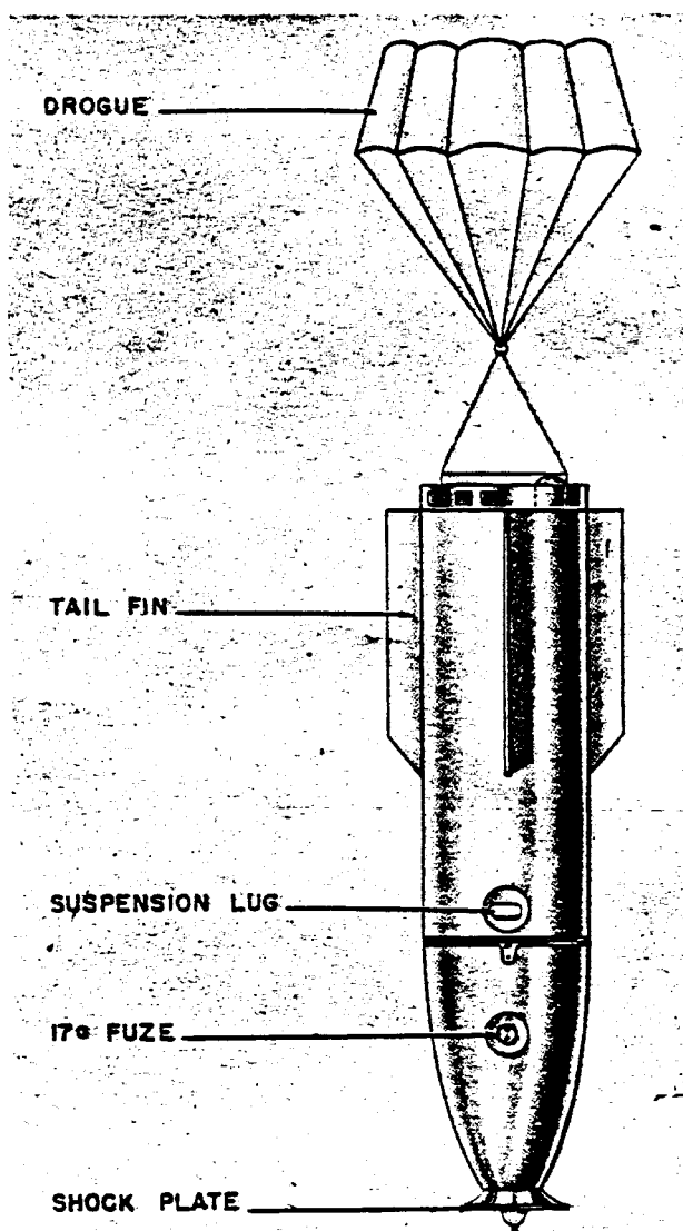
Figure 90—Lux EZ 50 SC Sea Marker
