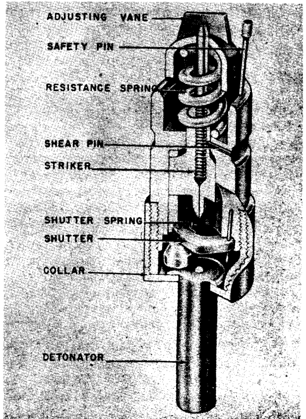
Figure 265—PX 32 Pressure Igniter
