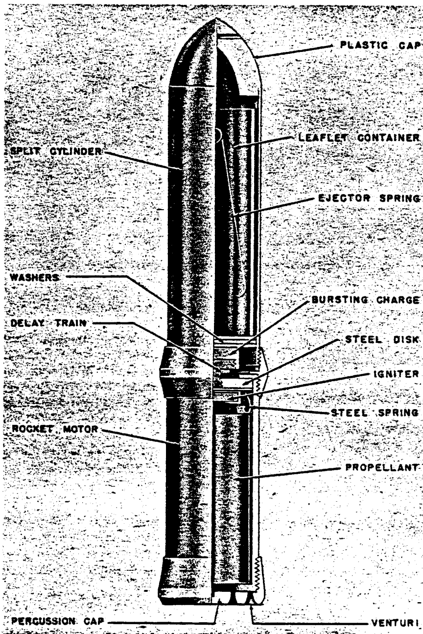
Figure 204—7.3-cm Propaganda Rocket
