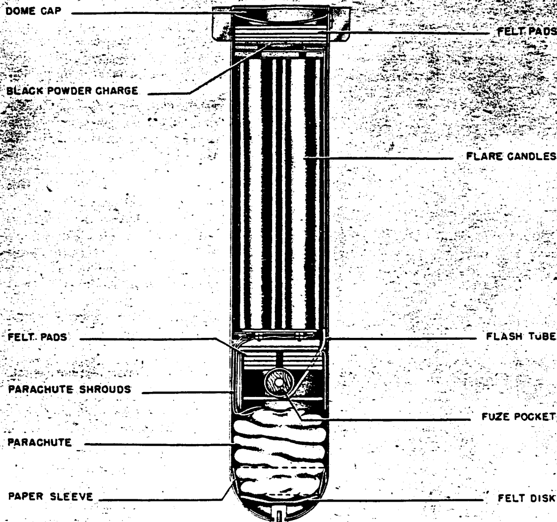
Figure 72—LC 50 F Ausf. C Parachute Flare
