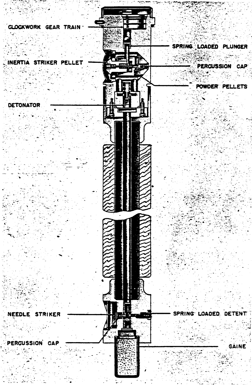
Figure 136—(24)A Mechanical Impact Fuze with Antibreak-up Switch
