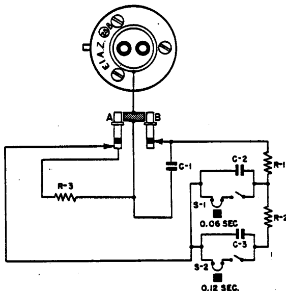
Figure 161—(28)B Electrical Impact Fuze
