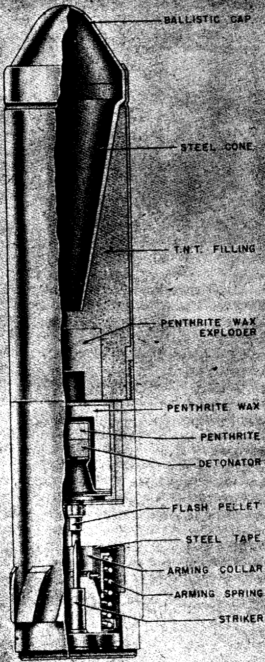
Figure 302—Antitank Hollow Charge Rifle Grenade
