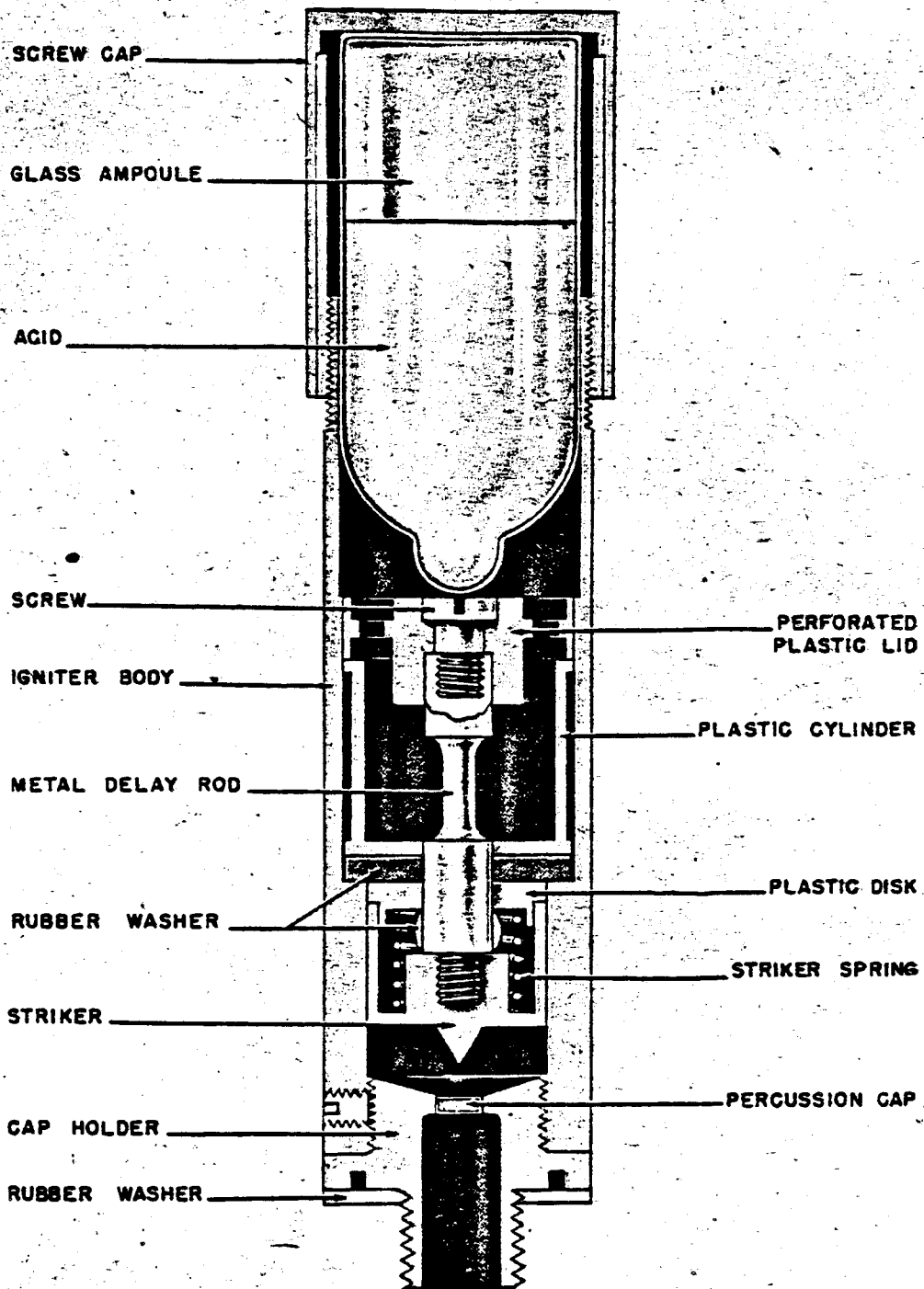
Figure 279—C. M. Z. 41W Chemical Delay Igniter
