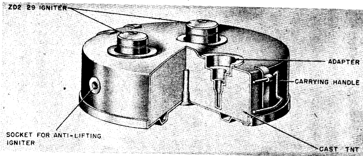
Figure 234—T. Mi. 29 (T-5) Mine—Antitank
