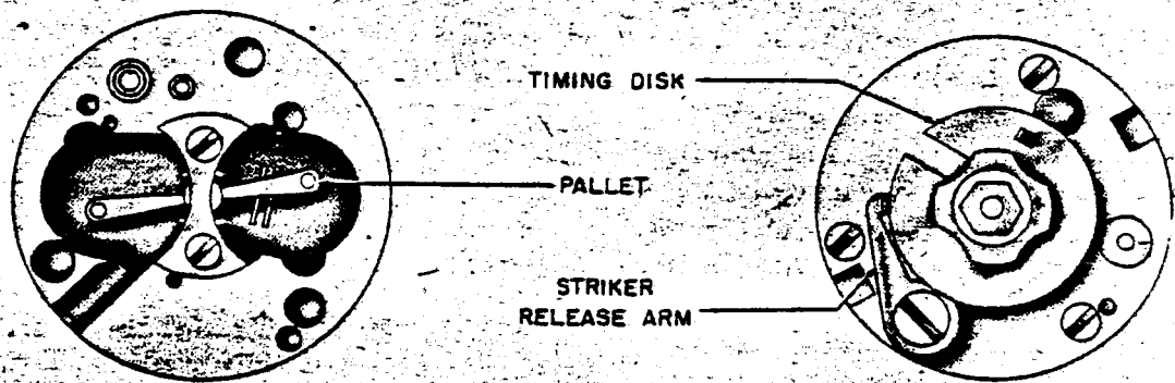
Figure 180—(89)D Clockwork Aerial Burst Fuze
