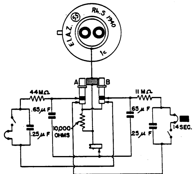
Figure 145—(55) Electrical Impact Fuze
