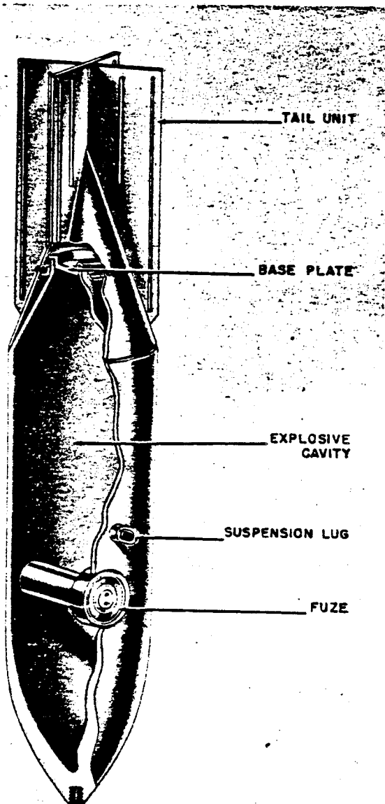
Figure 24—SD 70-Kg Bomb
