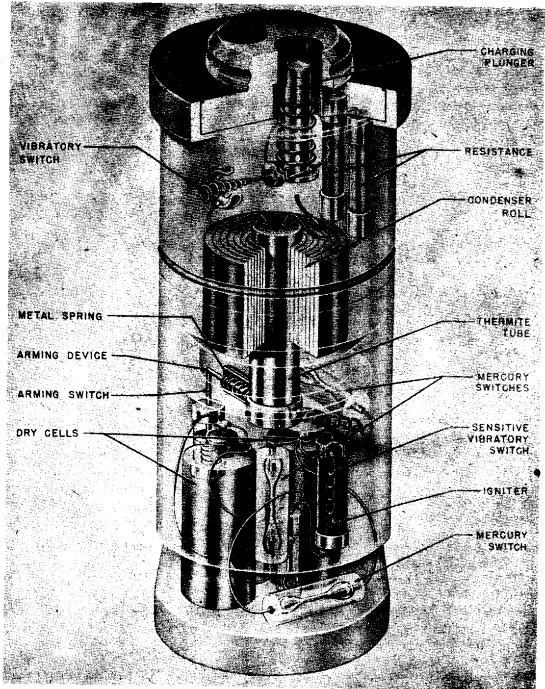
Figure 186A—50 b or "Y" Electrical Antidisturbance
