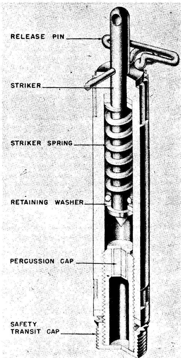
Figure 260—Z. Z. 42 Igniter—Pressure and Pull
