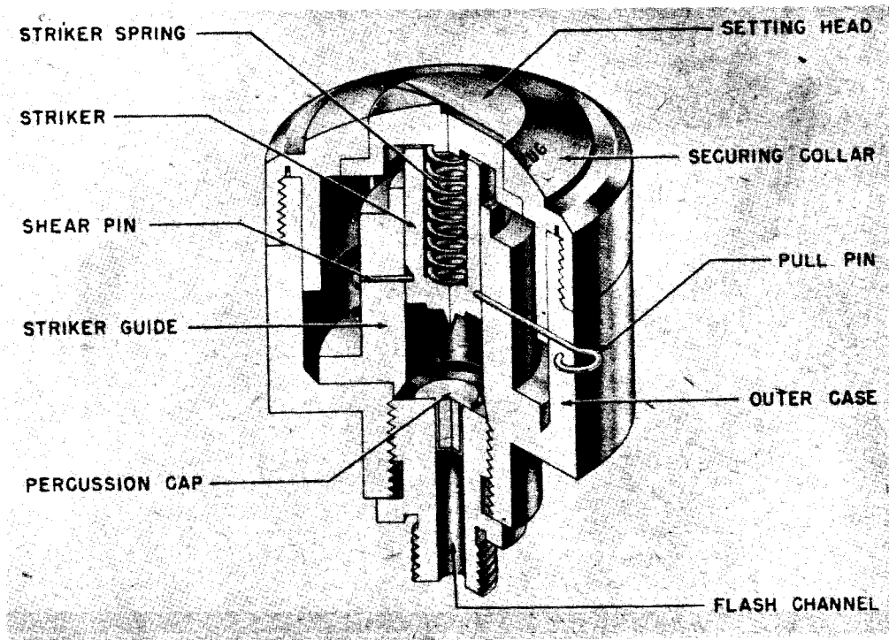
Figure 259—Z. D. Z. 29 Igniter—Pressure and Pull
