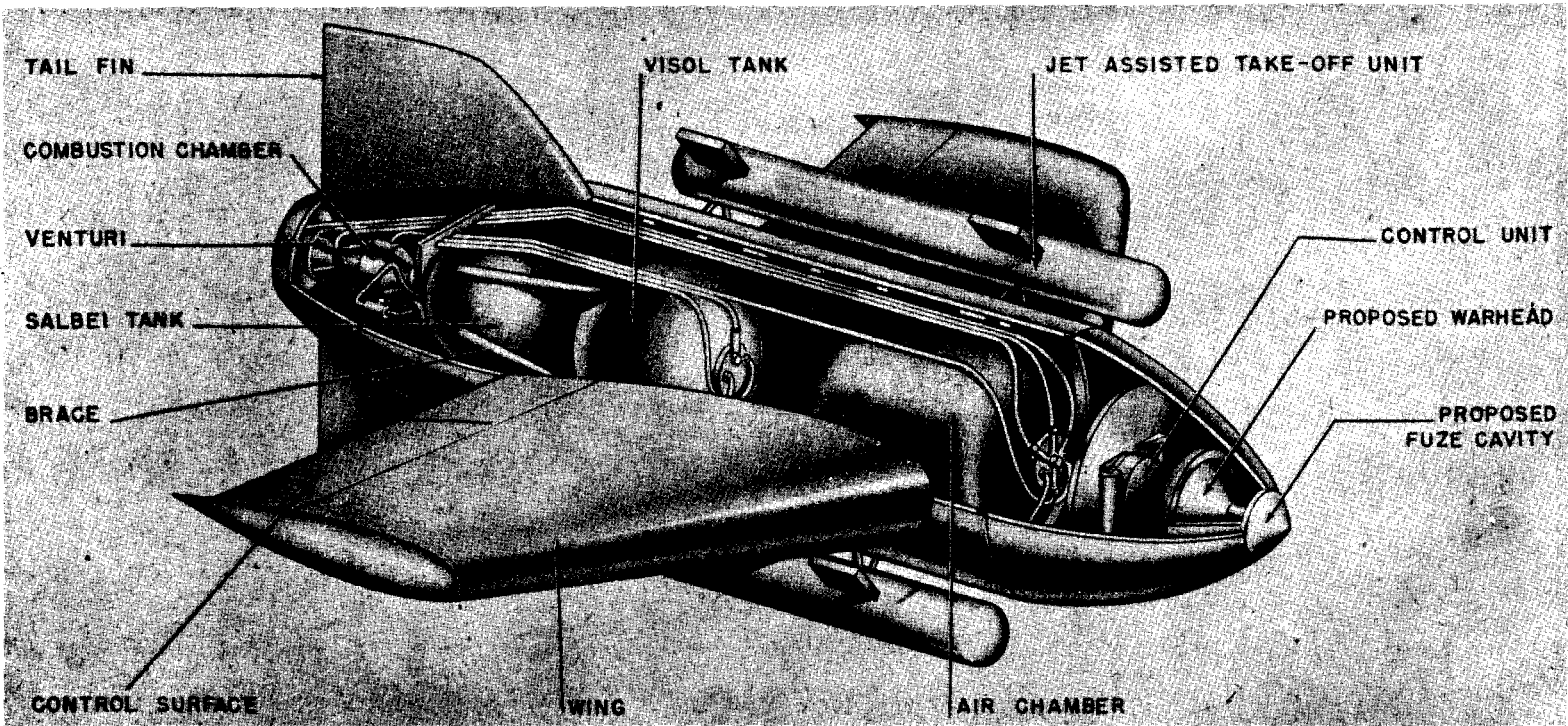
Figure 202—Enzian E-4
