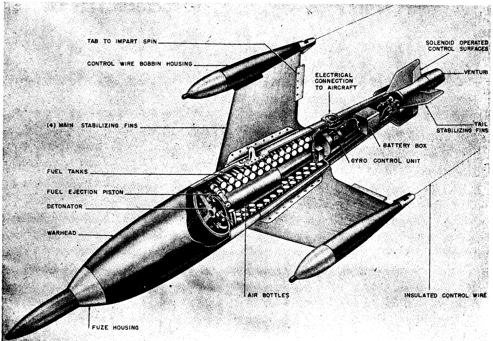
Figure 197A—X-4 Missile
