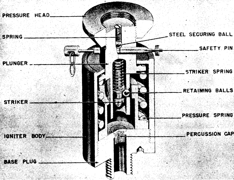
Figure 262—D. Z. 35 (A) Pressure Igniter
