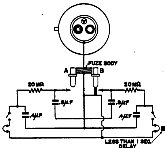
Figure 137—(A) Electrical Impact Fuze
