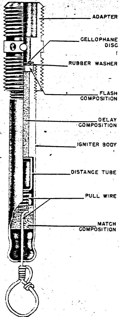
Figure 251—BZ-39 Friction Igniter Pull Type
