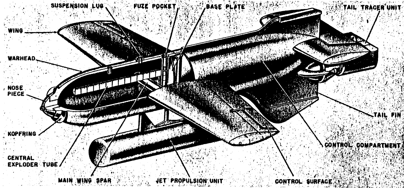
Figure 194—Hs 293 Glider Bomb; Hs 298
