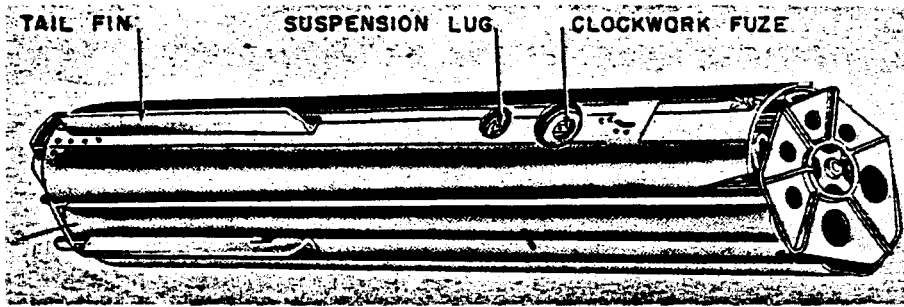
Figure 99—BSK 36 Container
