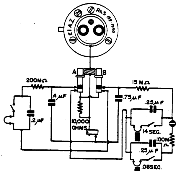
Figure 140—(25) Electrical Impact Fuze
