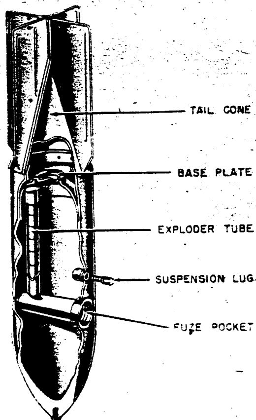
Figure 11—SC 50 Grade II Bomb
