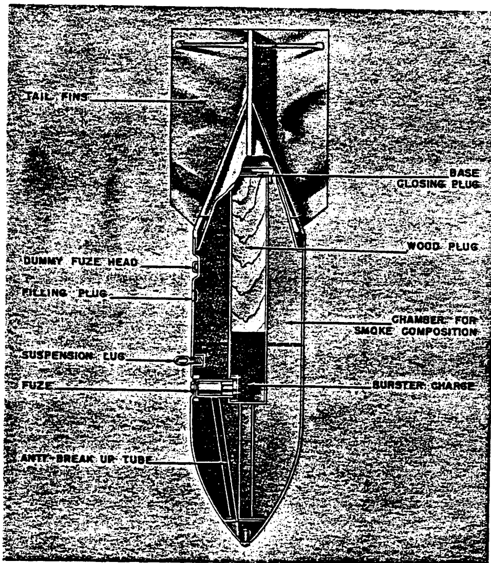
Figure 63—NC 250 S Smoke Bomb
