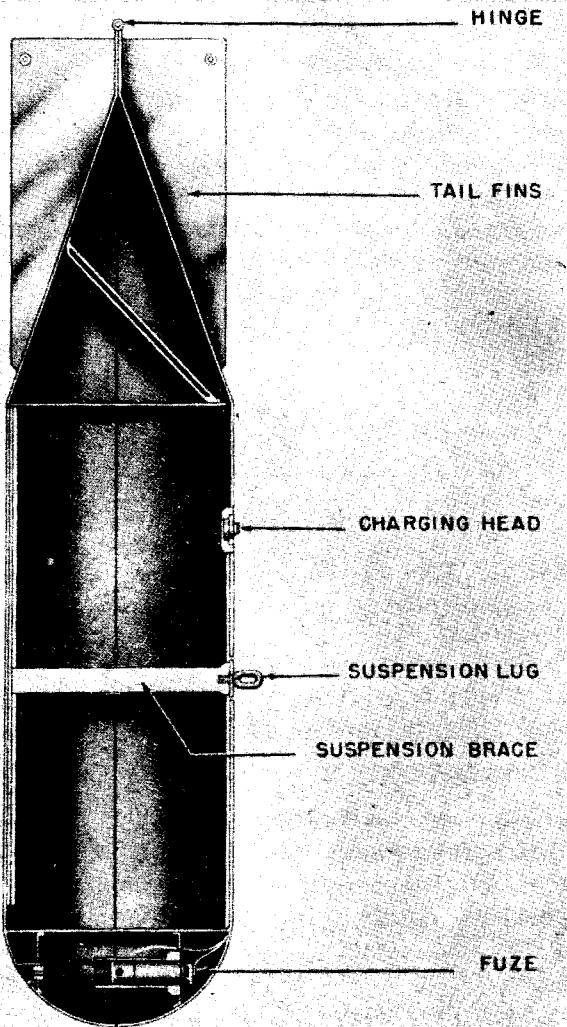
Figure 113—AB 500-1B Container
