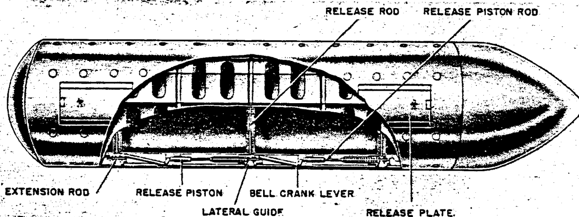
Figure 105—AB 250-1 Container
