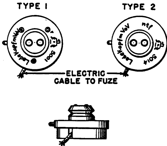
Figure 130—Charging Heads
