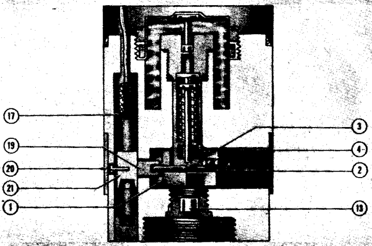
Figure 156A—(57) Electrical Chemical Time Fuze
