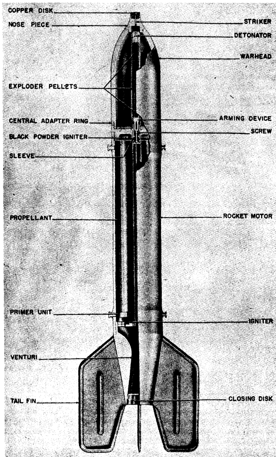
Figure 206—8-cm Aircraft Rocket
