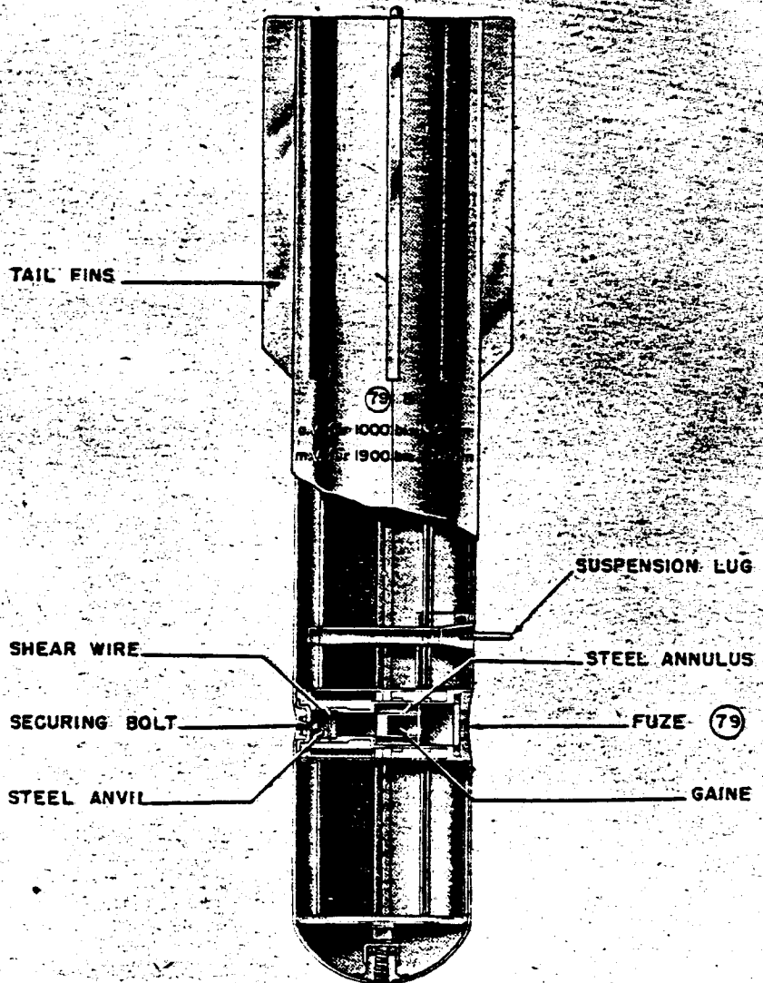
Figure 96—AB 23 SD 2 Container
