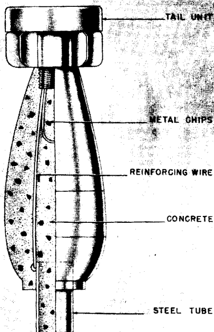
Figure 64—SD 1 Type Practice Bomb
