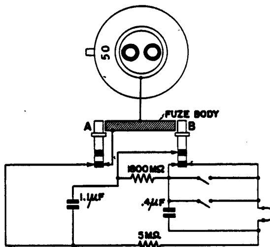
Figure 183—50 Electrical Antidisturbance Fuze
