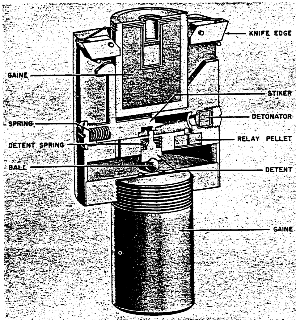
Figure 181—ZUS 40 (Type I) Mechanical Antiwithdrawal
