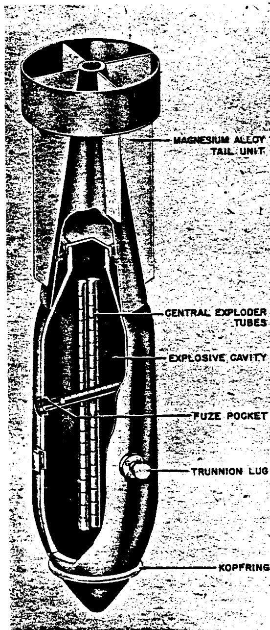
Figure 28—SD 1700-Kg Bomb
