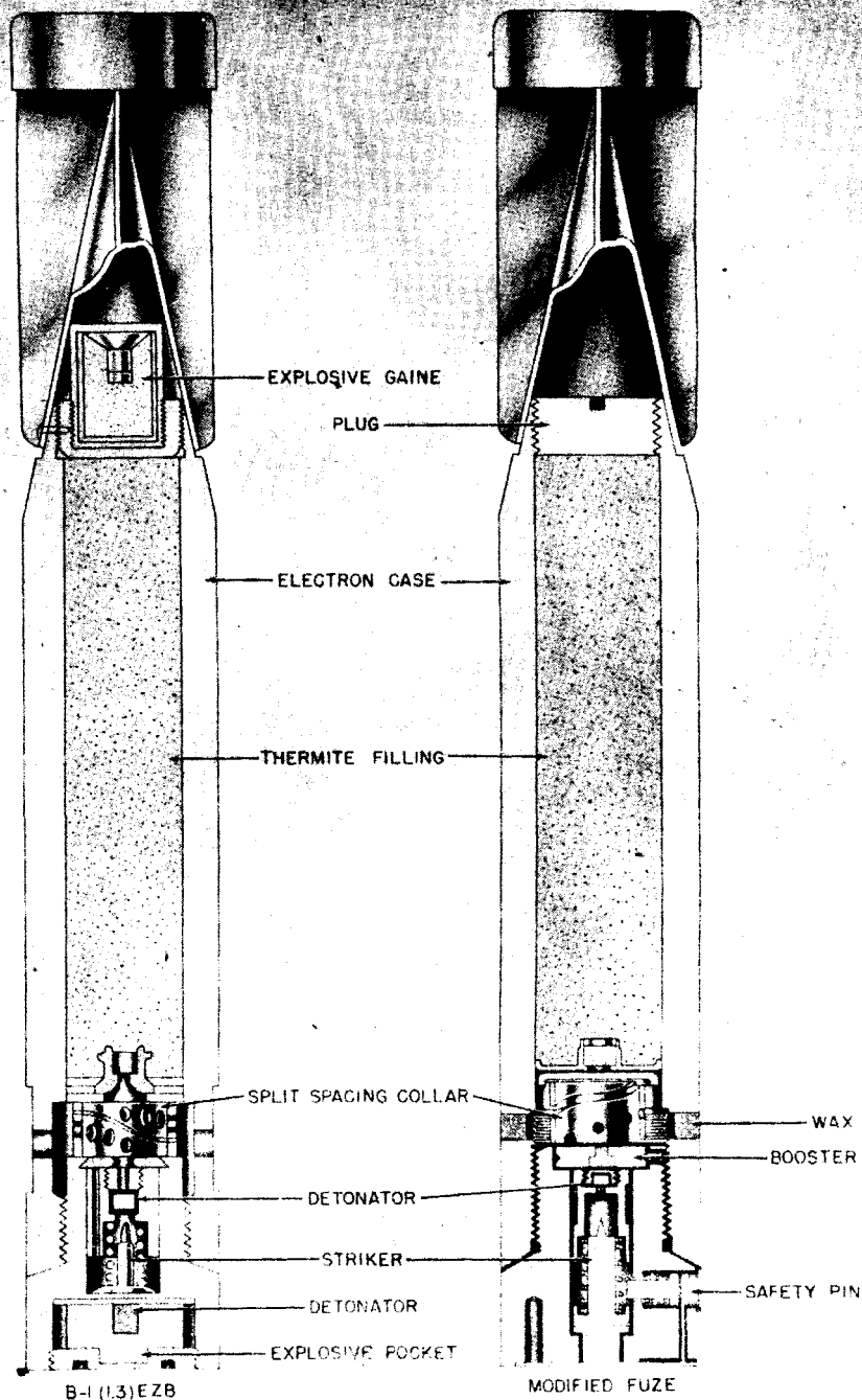
Figure 51—1-Kg B1E, B1EZE, B1EZB Incendiary Bomb
