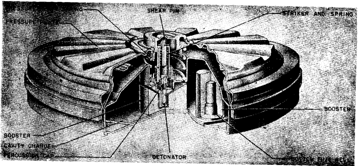
Figure 231—Tellermine 35 (Steel Antitank)
