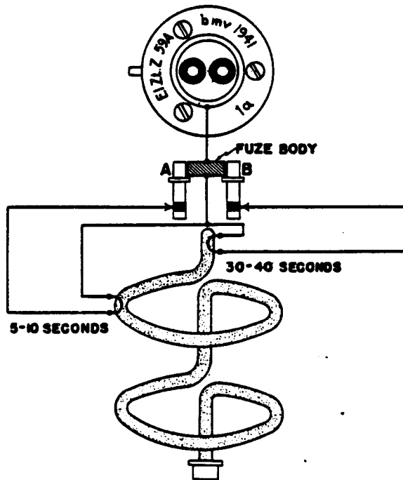
Figure 174—(59)A Electrical Aerial Burst Fuze
