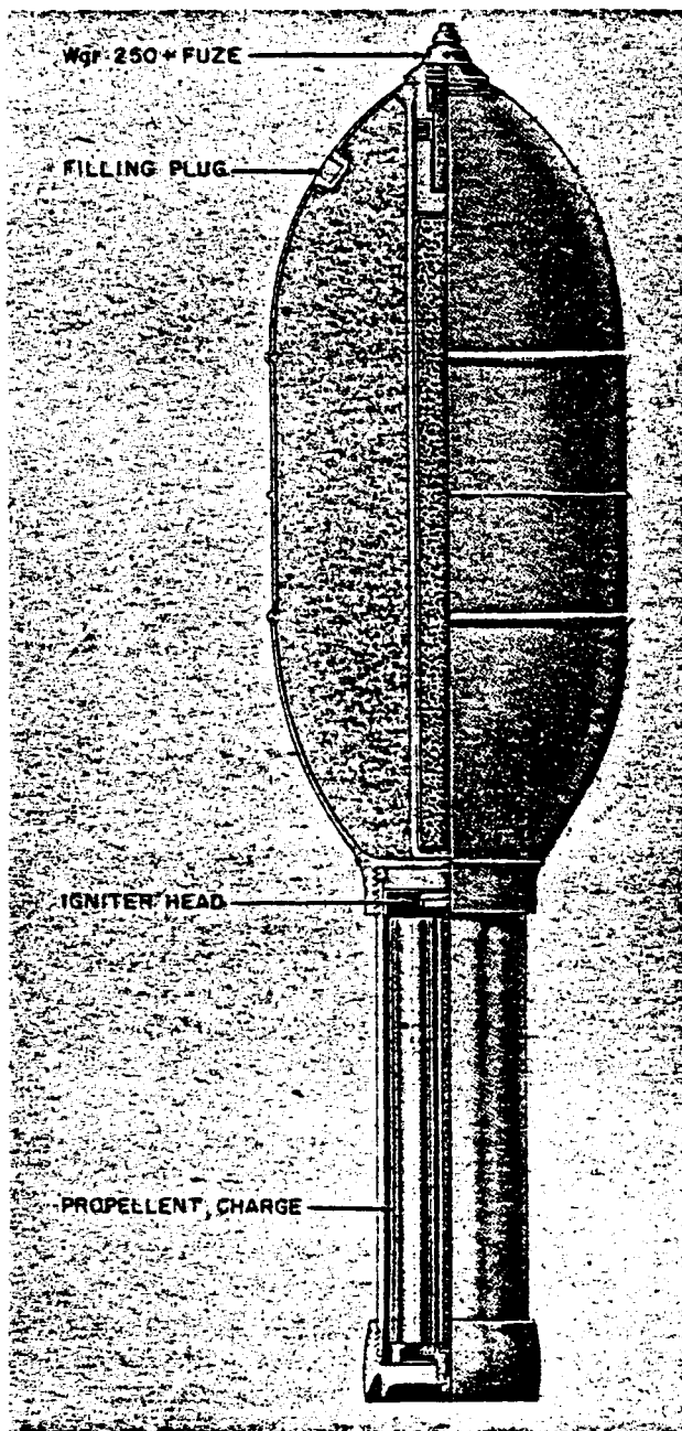
Figure 218—32-cm Incendiary Rocket
