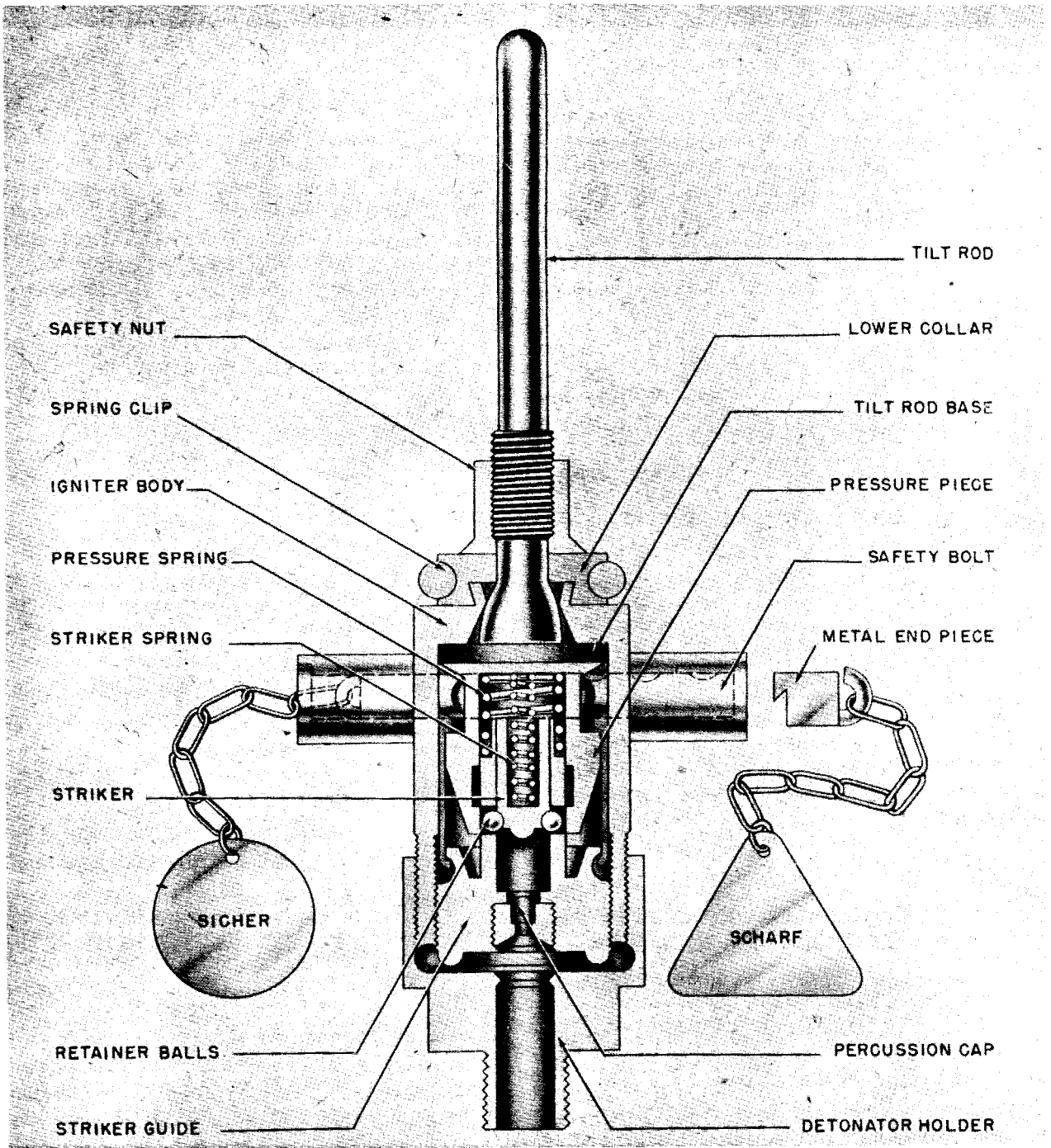
Figure 280—Kippzunder 43, Tilt Type
