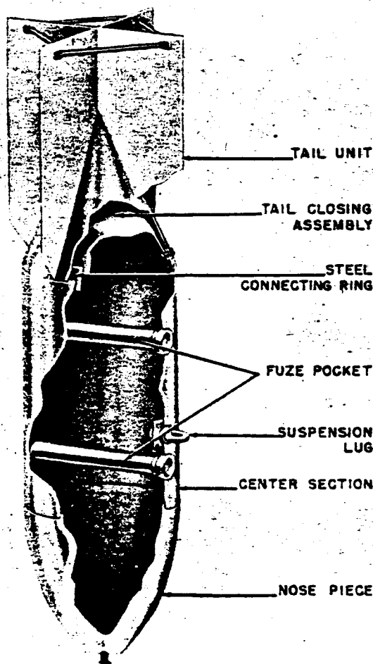
Figure 13—SC 500-Kg Bomb
