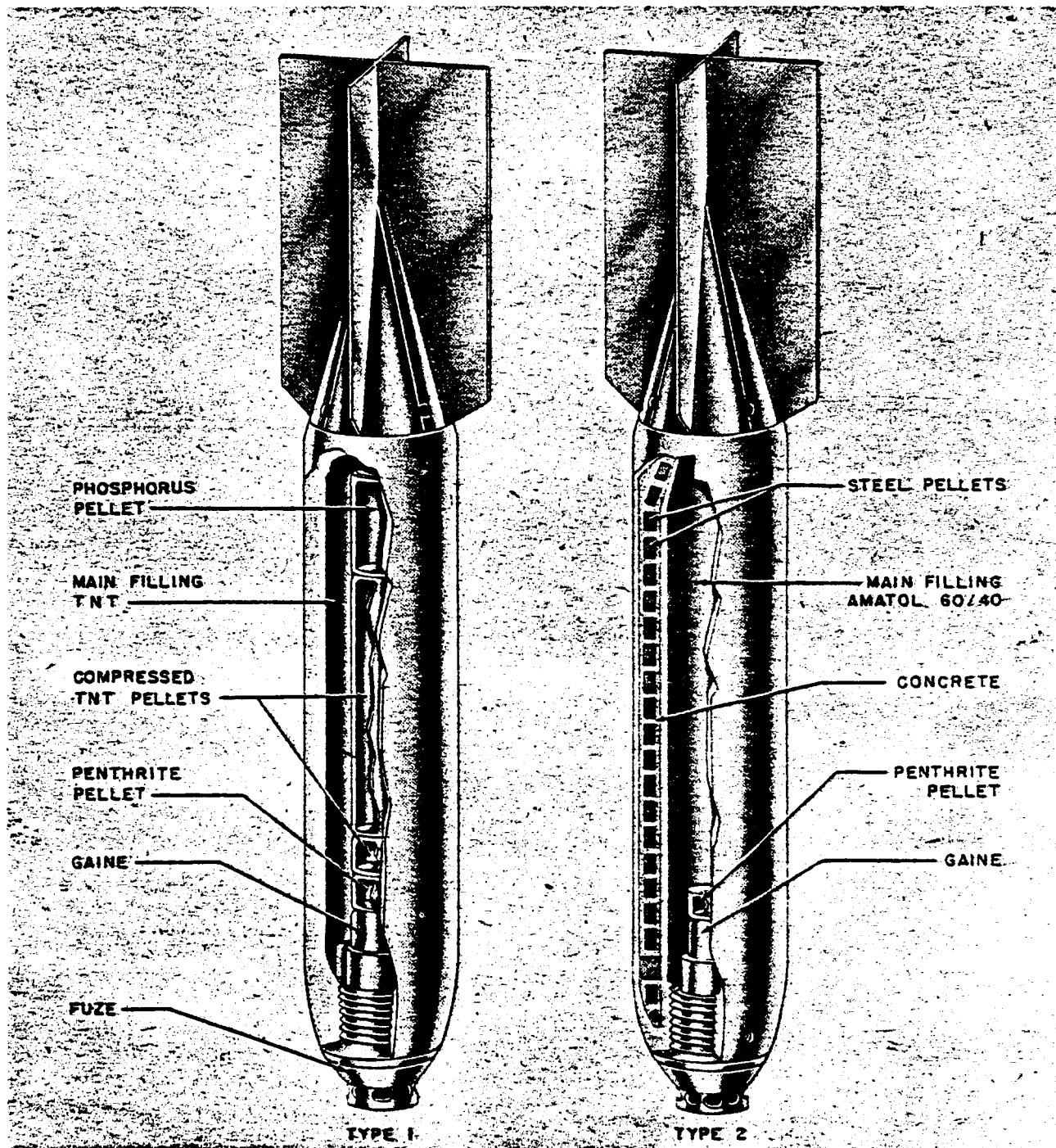
Figure 42—SD 10A Antipersonnel Bomb
