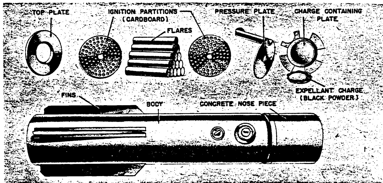
Figure 76—Mark 50 Kask Target Identification Flare
