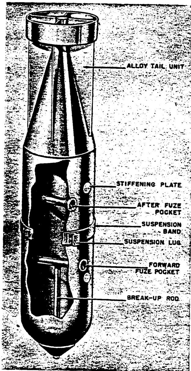
Figure 18—SC 2500-Kg Bomb
