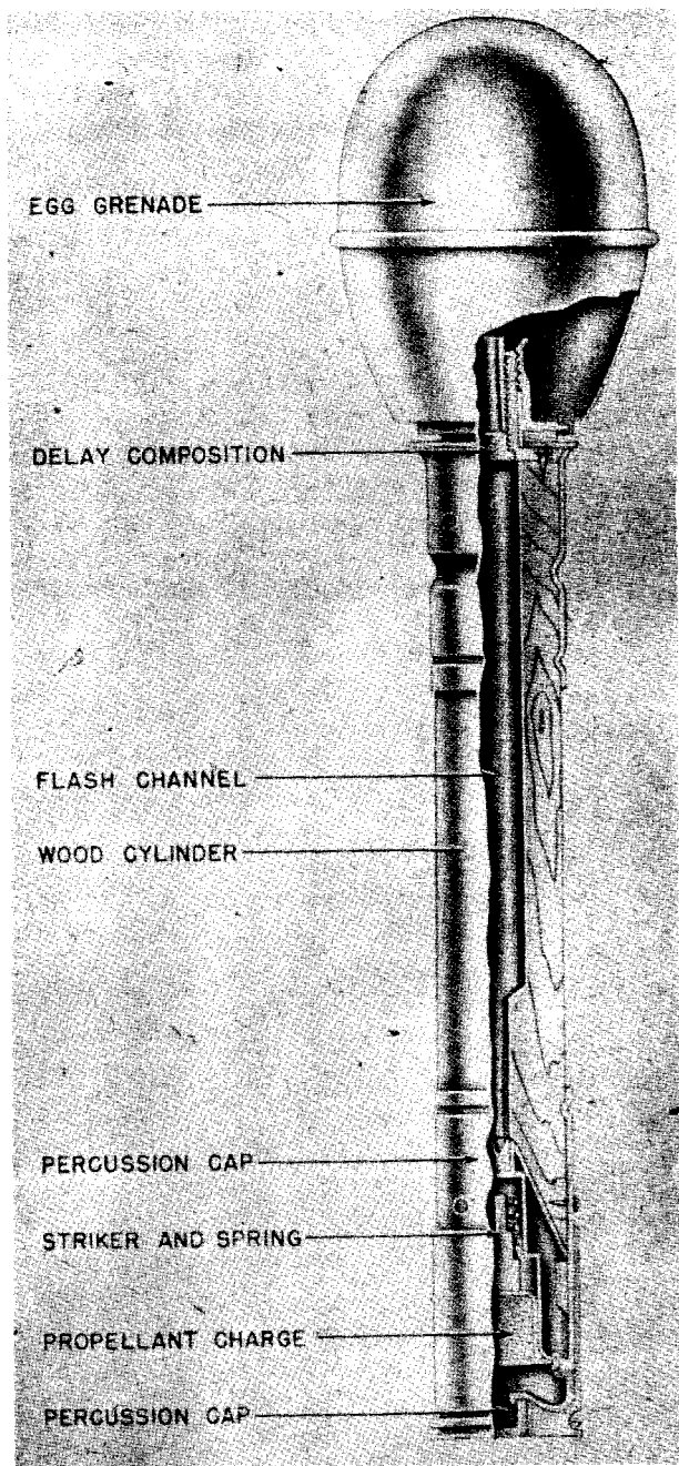
Figure 310—27-mm Egg Type Pistol Grenade
