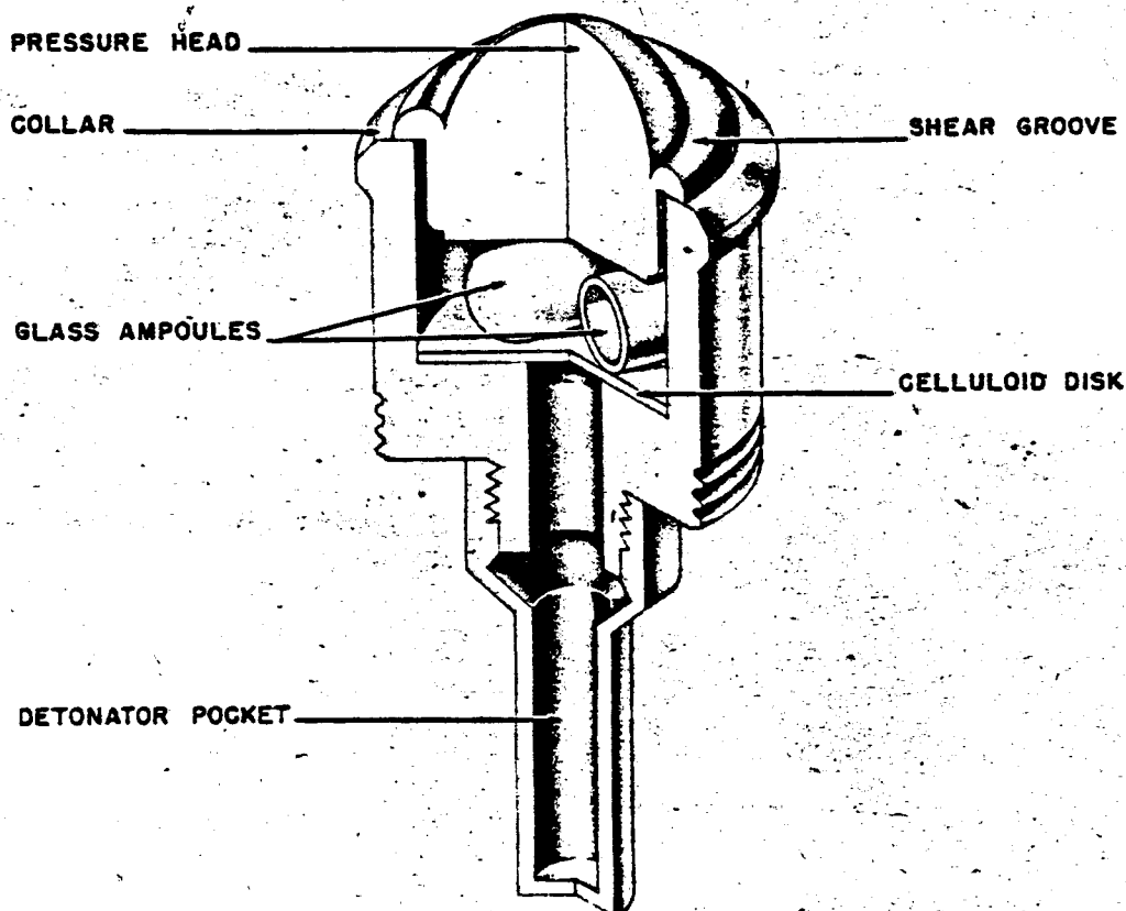
Figure 273—Topf Pressure Igniter
