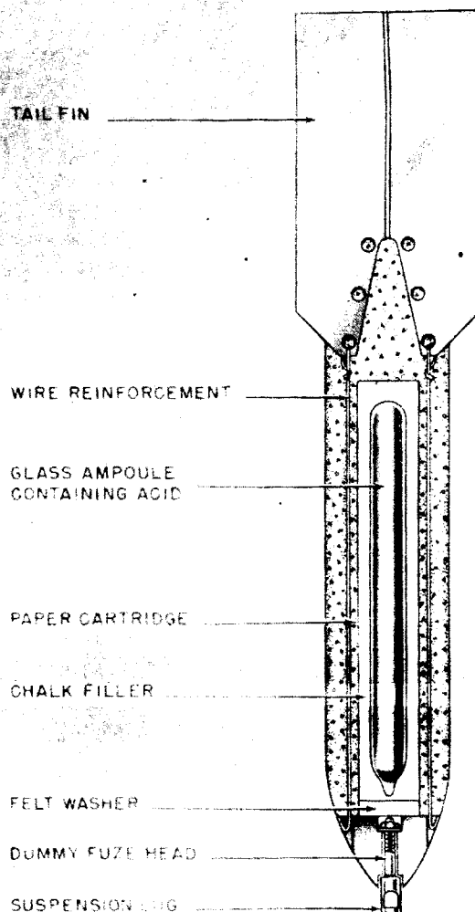
Figure 66—ZC 10-Kg Concrete Practice Bomb
