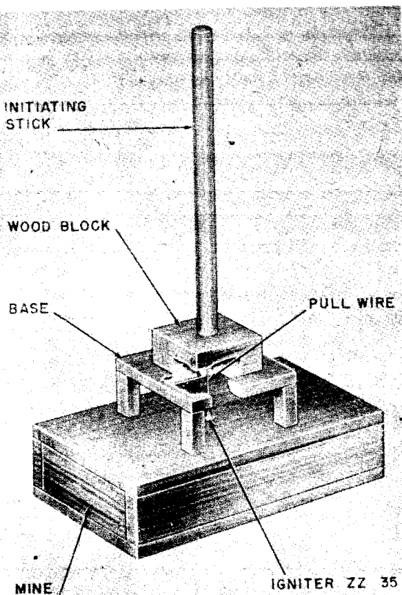
Figure 240—B-Stabmine—Antipersonnel
