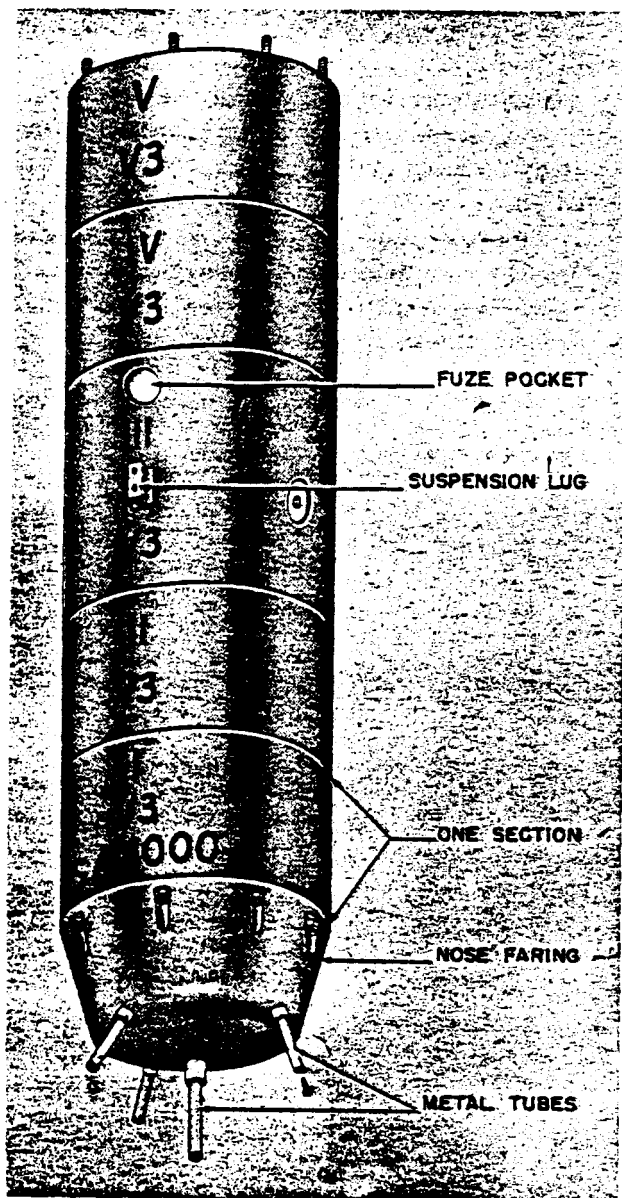
Figure 48—SA 4000-Kg Bomb
