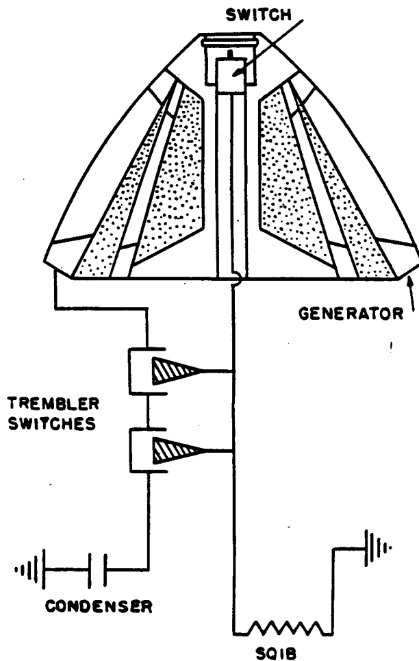
Figure 191B—Dust Fuze for SD 10 Bomb Wiring Diagram
