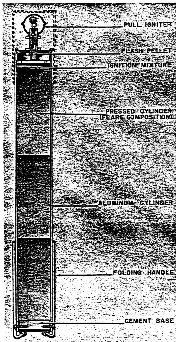
Figure 85—Distress Signal Torch
