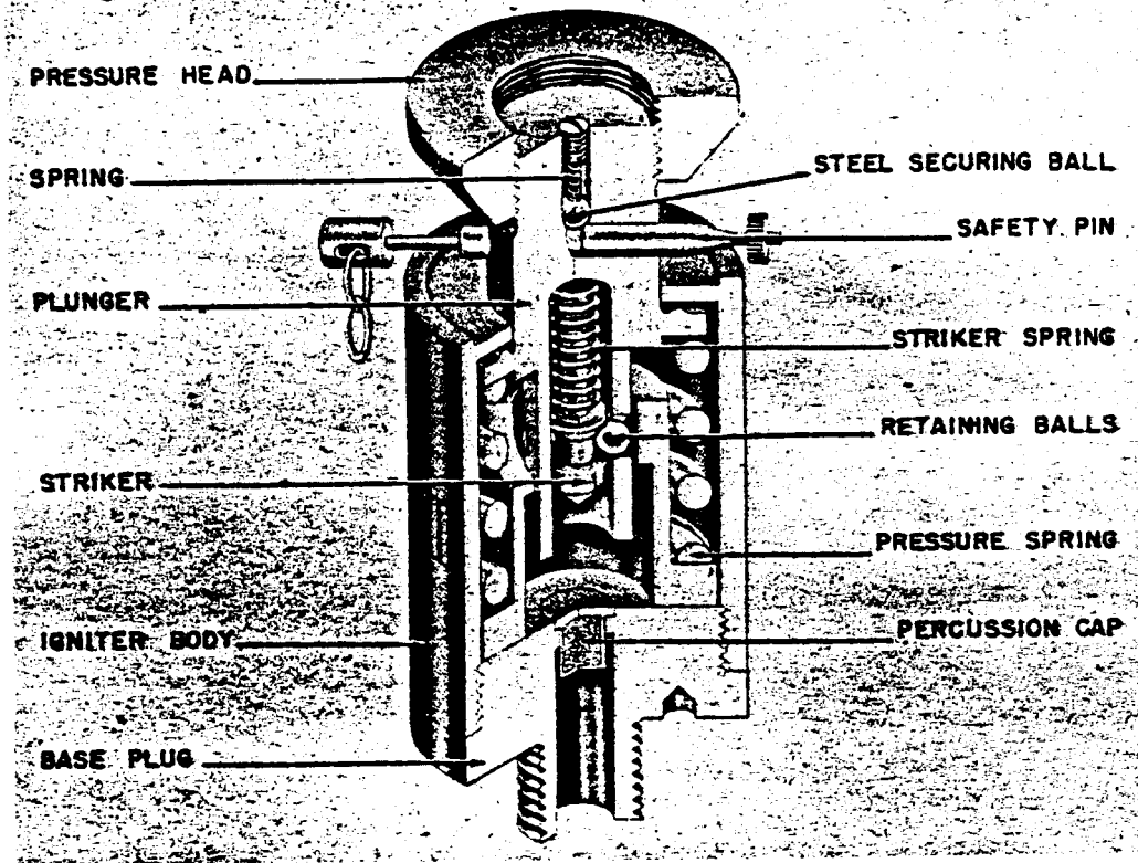
Figure 262—D. Z. 35 (A) Pressure Igniter
