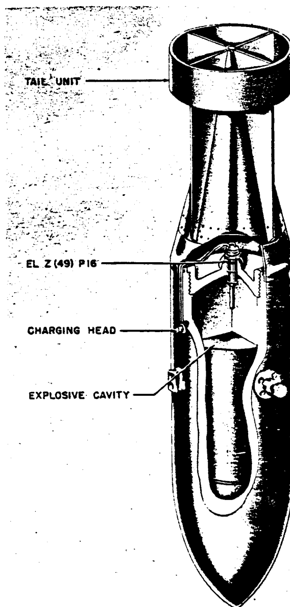
Figure 32—PC 1600-Kg Bomb
