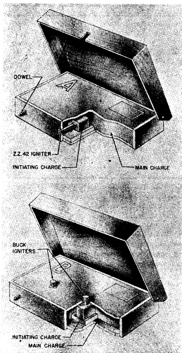
Figure 225—Panzerschnell Antitank Mine
