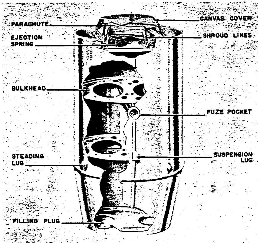
Figure 21—SB 1000-Kg Parachute Bomb
