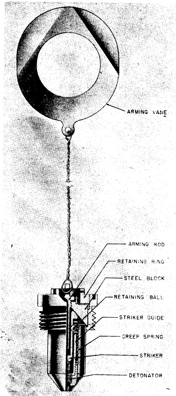
Figure 134—(23)A Mechanical Tail Impact Fuze
