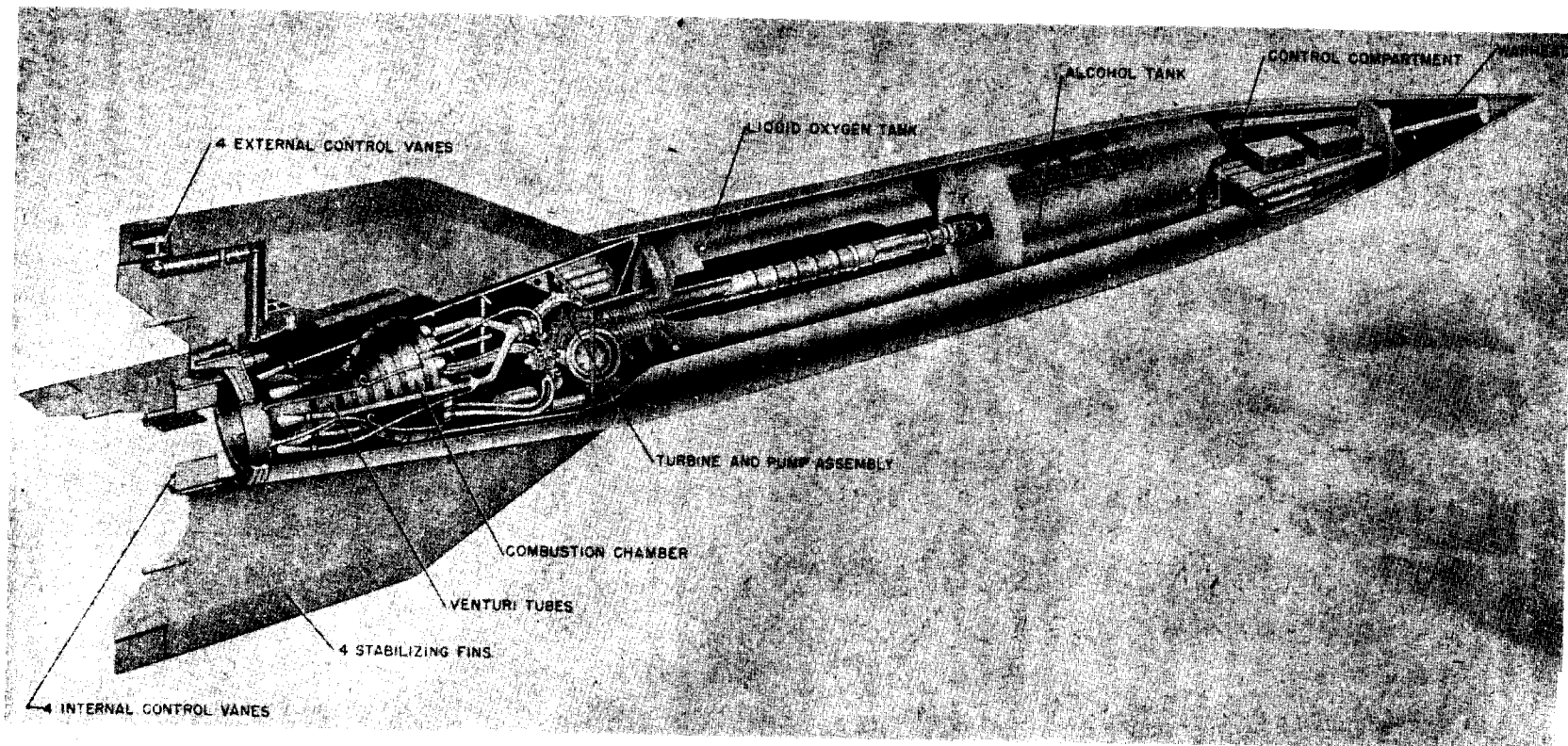
Figure 196—A-4 "V-2" Rocket
