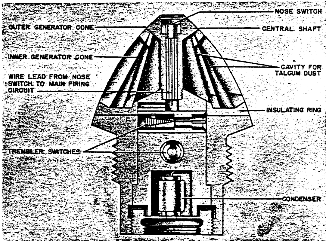
Figure 191A—Dust Fuze for SD 10 Bomb
