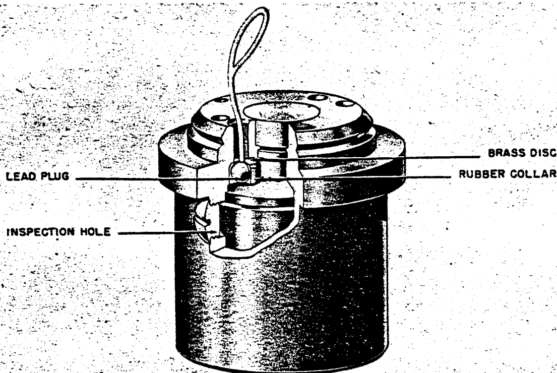
Figure 178—(89) Clockwork Aerial Burst Fuze
