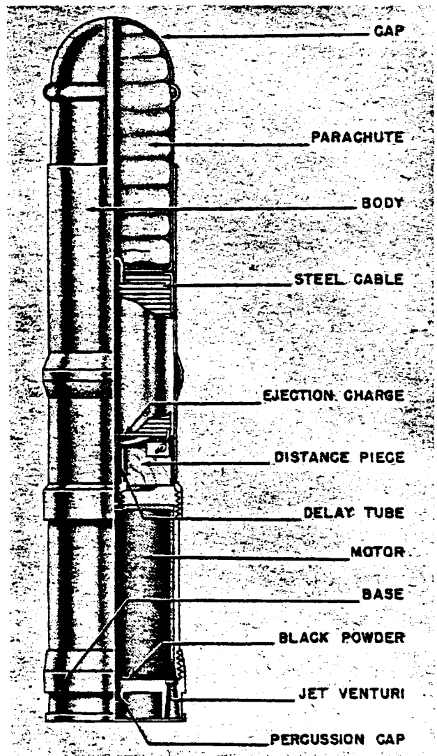
Figure 209—8.6-cm Antiaircraft Rocket (Naval)
