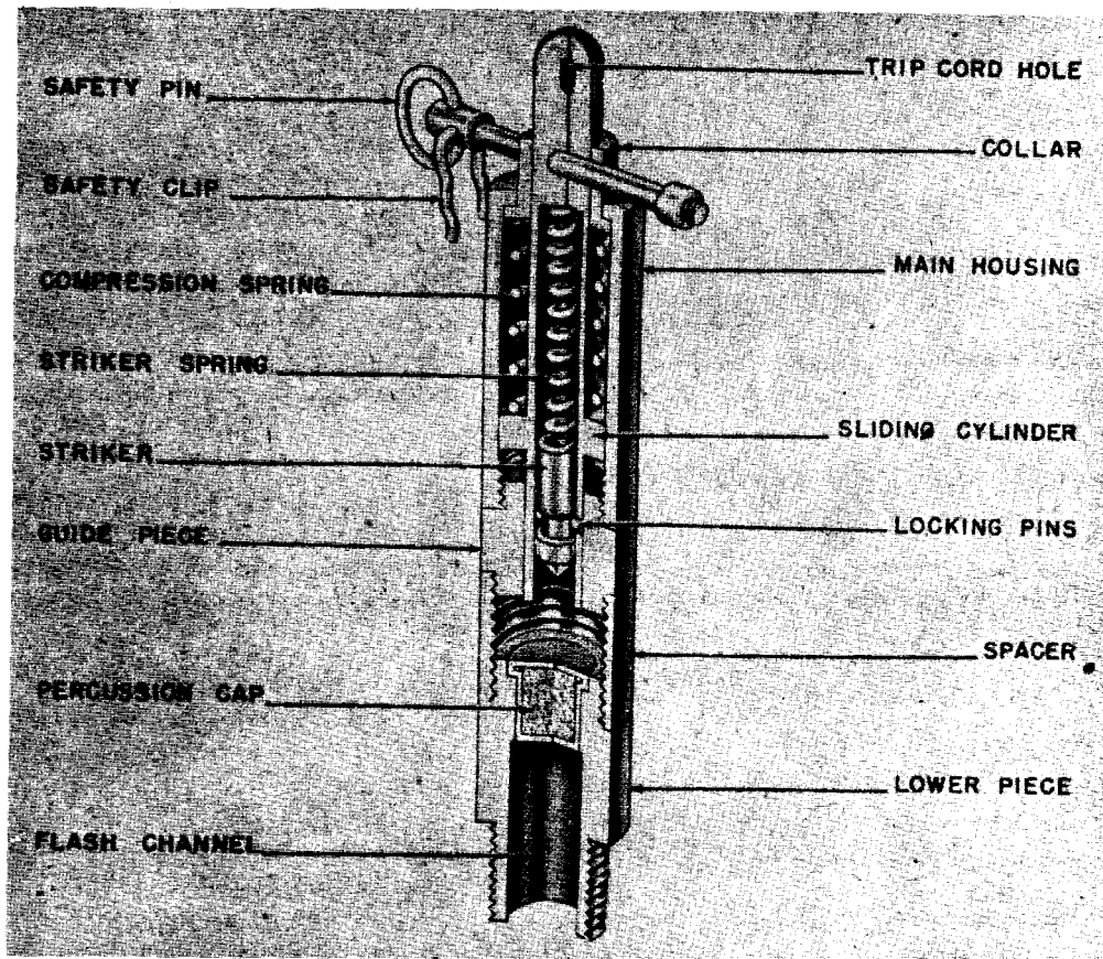
Figure 256—Z. Z. 35 Pull Igniter
