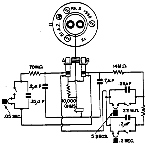
Figure 164—(38) Electrical Impact Fuze
