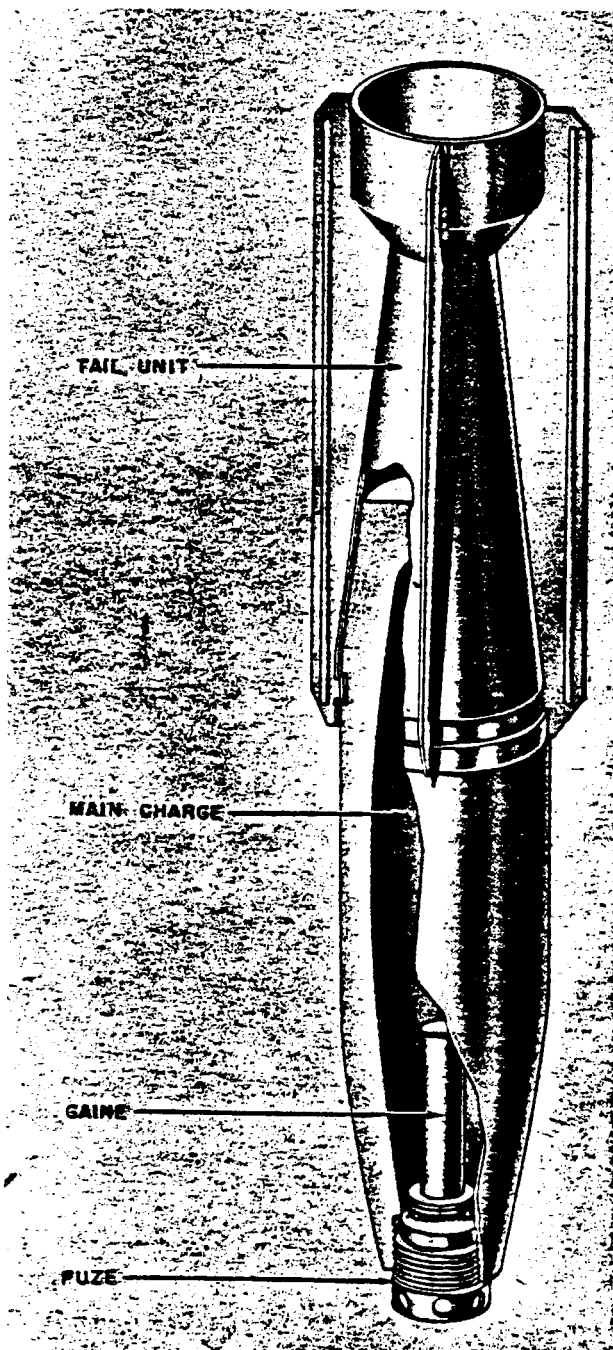
Figure 45—SD 15-Kg Converted German Shell Bomb
