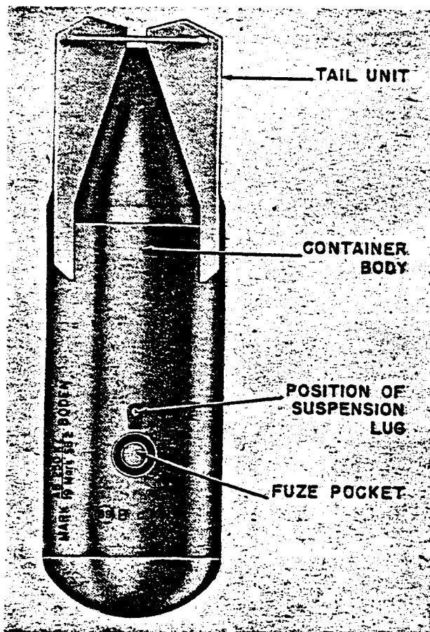
Figure 108—AB 250 KZ Boden Container
