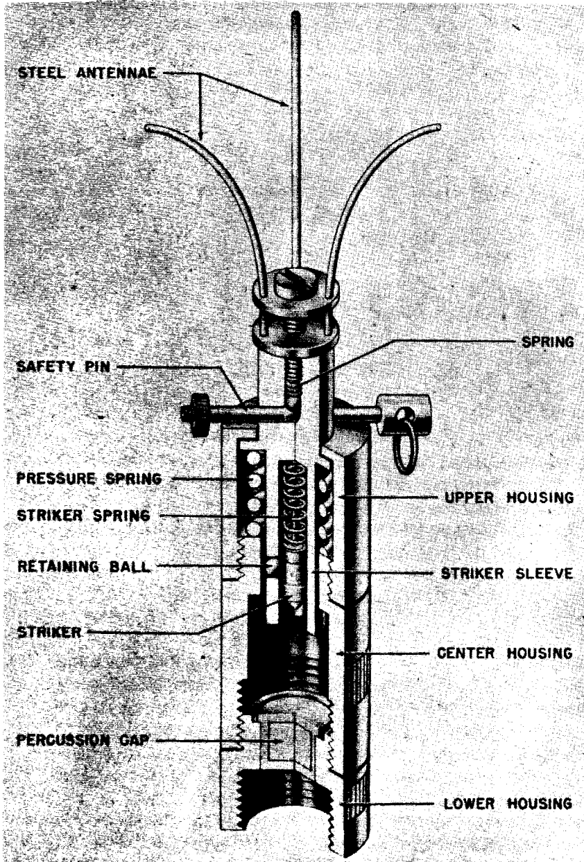
Figure 267—S. Mi. Z. 35 Pressure Igniter
