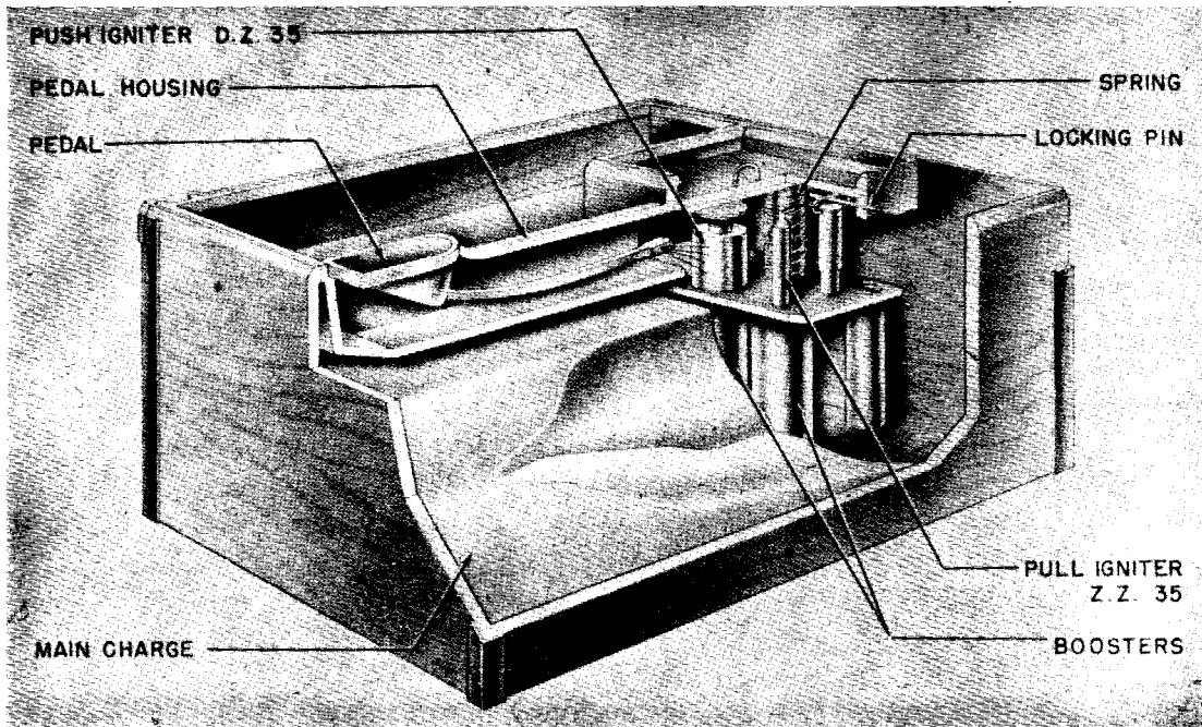
Figure 229—Heavy Antitank Mine
