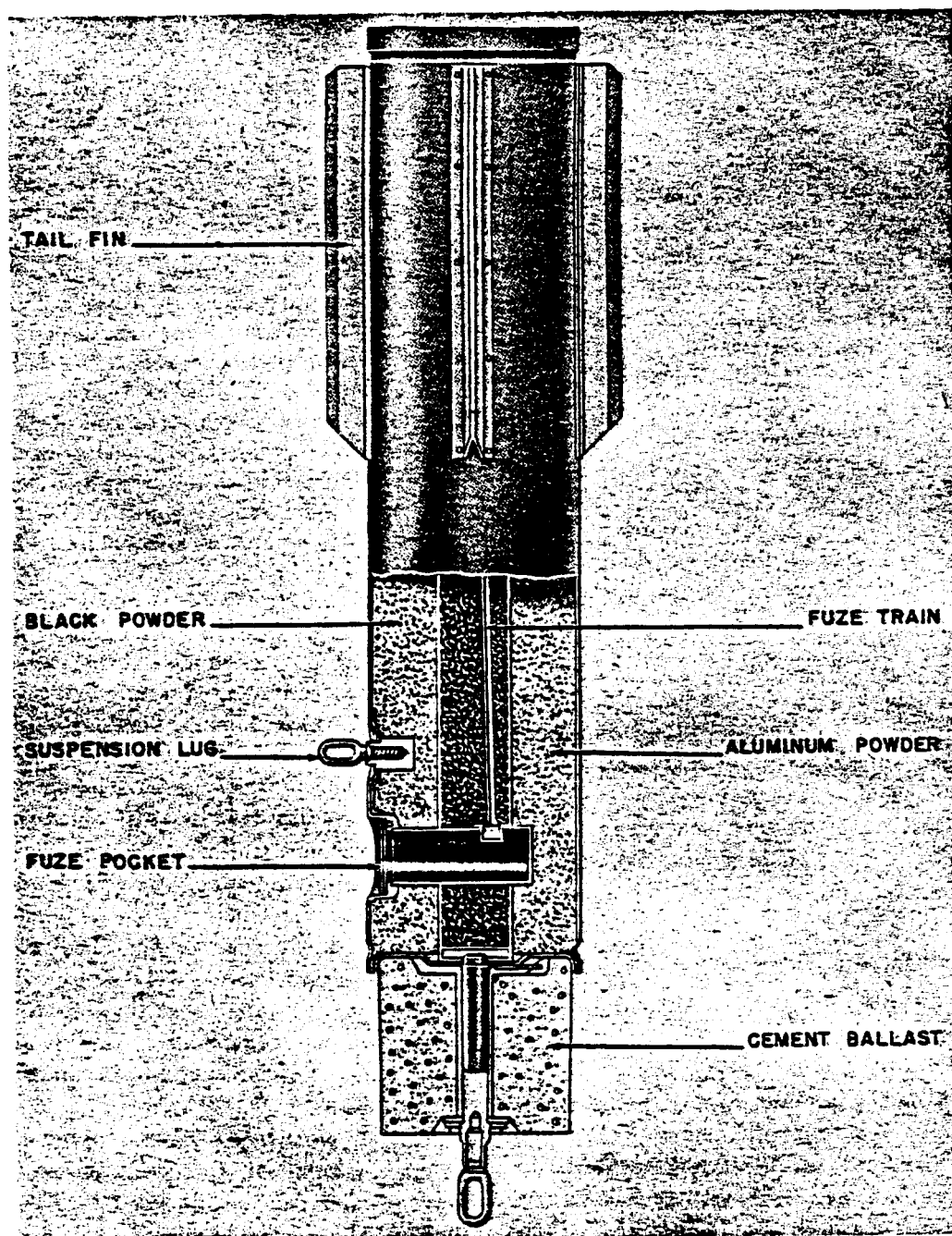
Figure 87—BLC 50/A Photoflash Bomb
