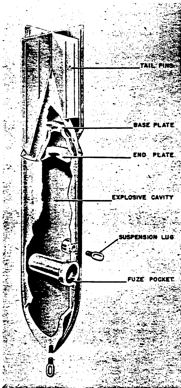
Figure 9—SC 50 Bi Bomb
