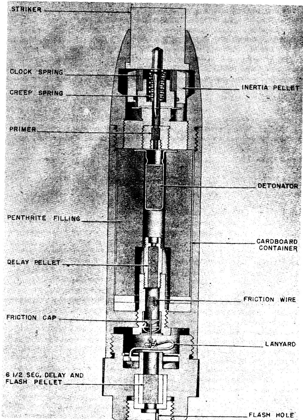
Figure 301—Hand or Rifle Grenade
