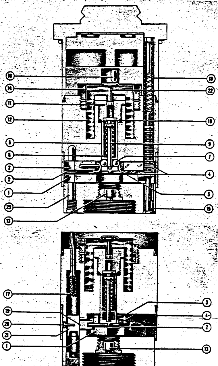
Figure 156A—(57) Electrical Chemical Time Fuze
