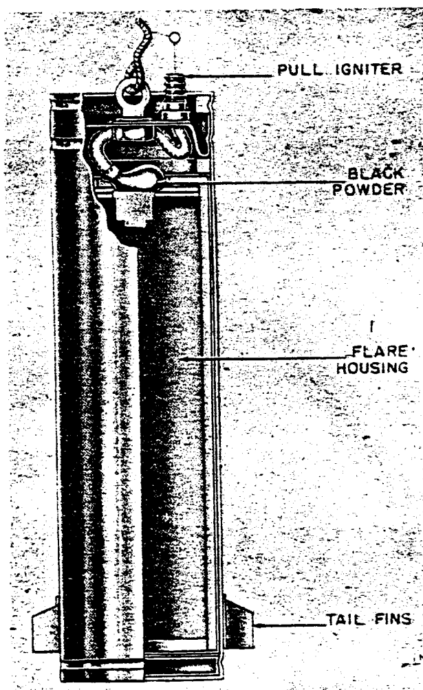
Figure 88—Target Indicator (Red)
