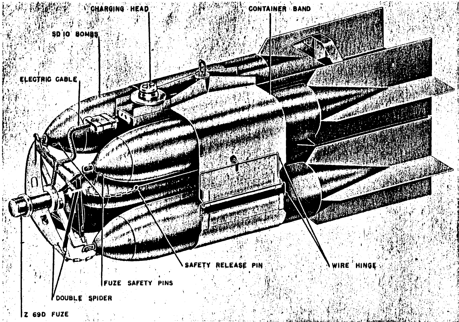
Figure 95—BDE 10 Container
