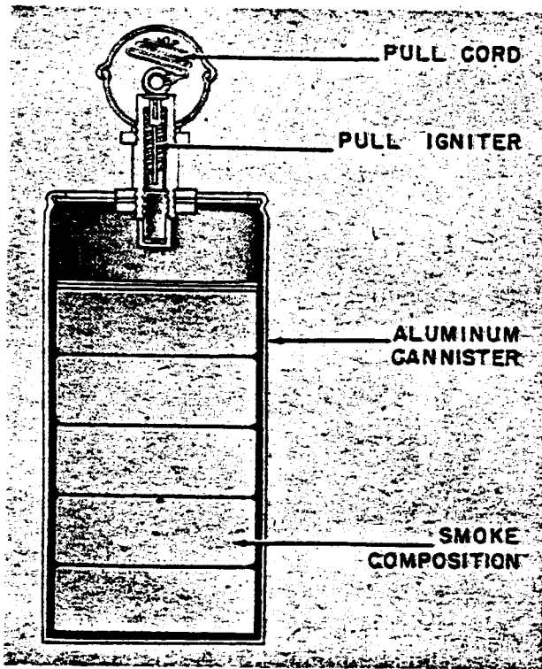
Figure 83—Smoke Signal Flare
